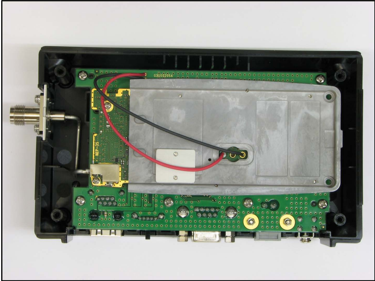
Photograph 16: Metal Base Removed
