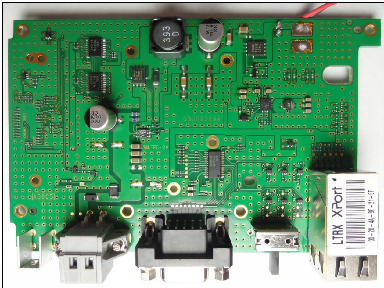
Photograph 11: Interface Board Top View
