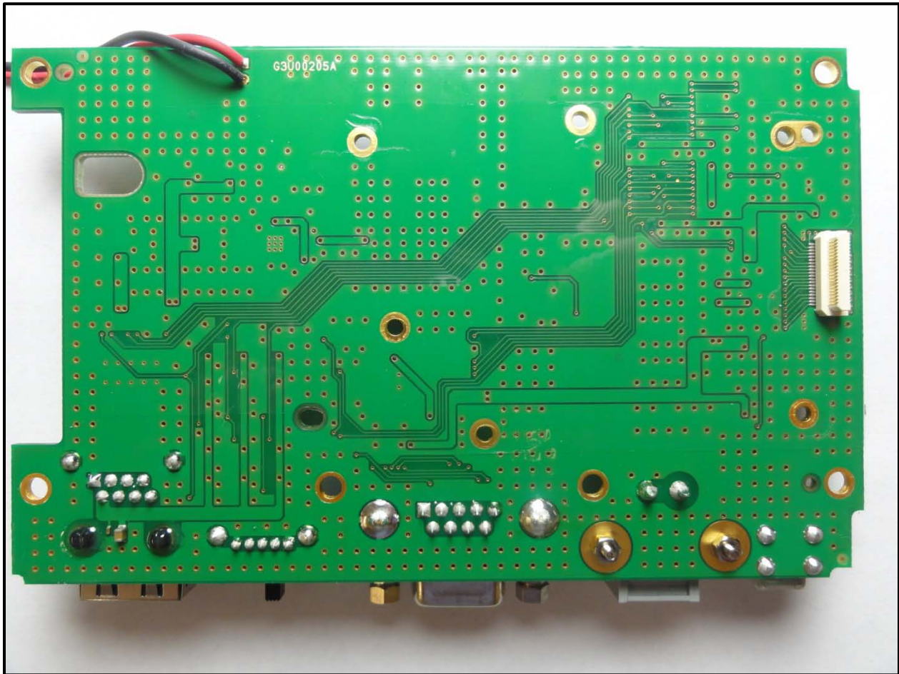
Photograph 12: Interface Board Bottom View
