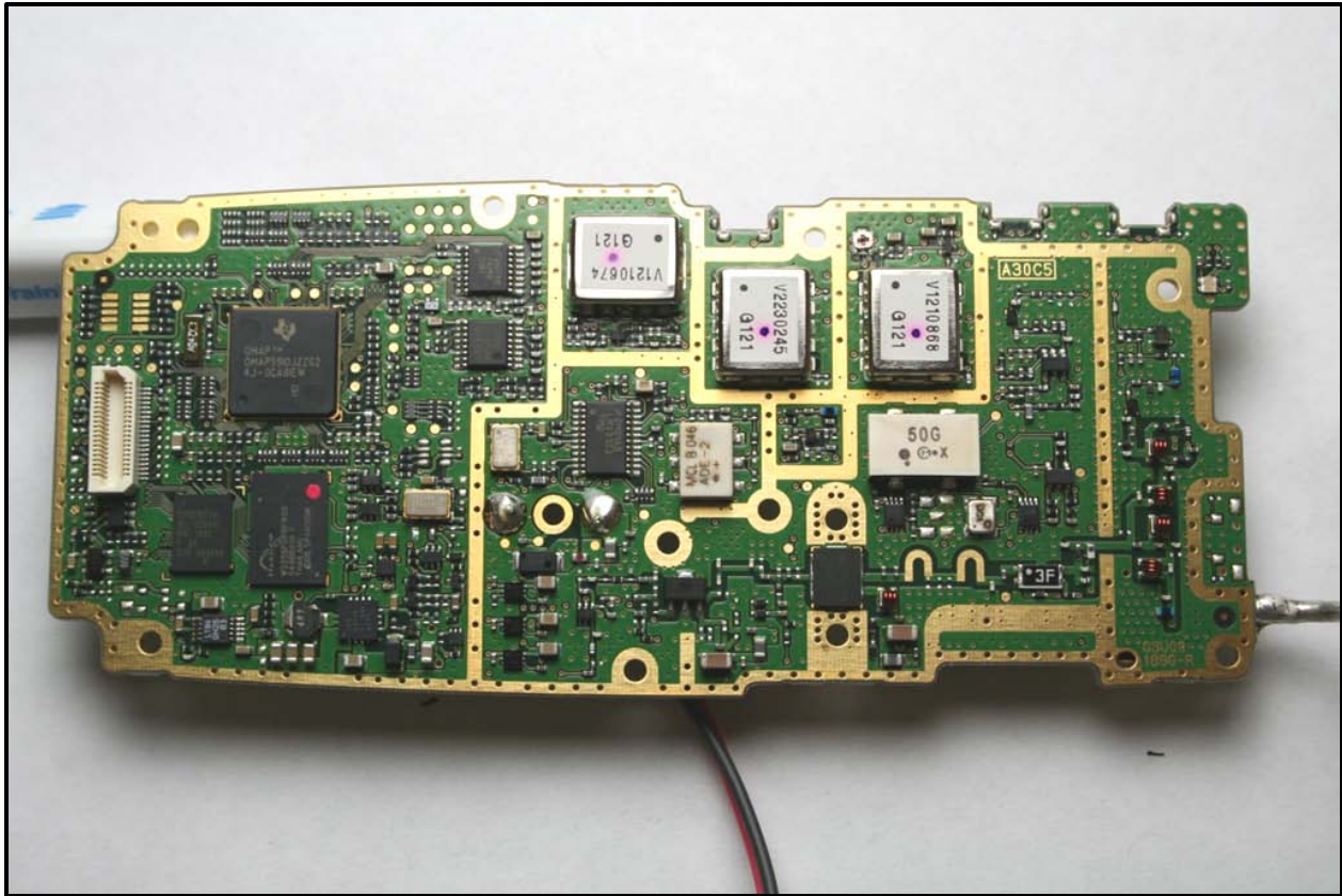
Photograph 9: Main Board Top View
