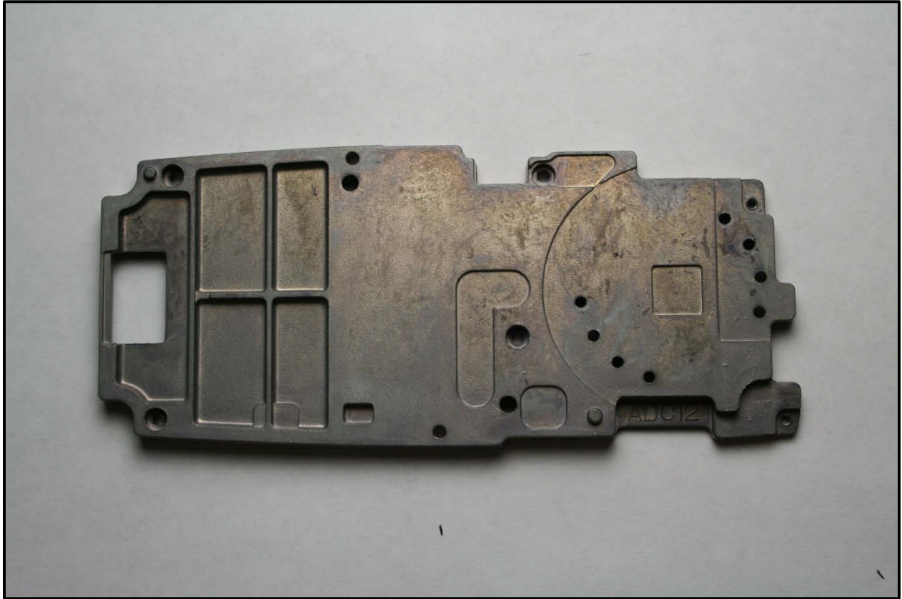
Photograph 13: RF Shield Top View
