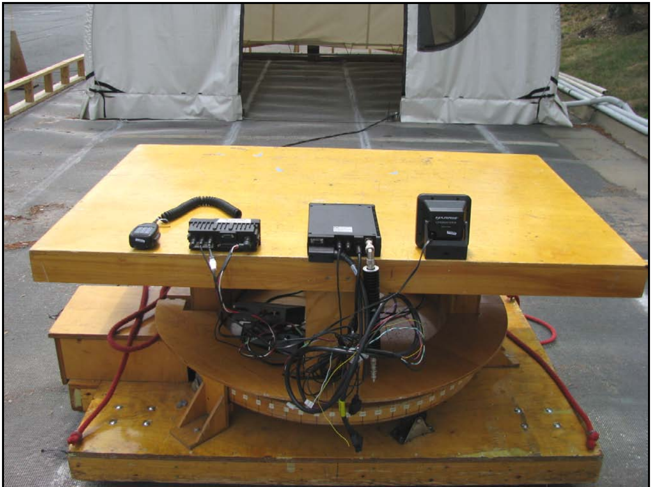
Photograph 5: Radiated Emissions – Back View
