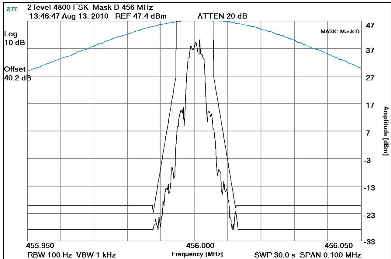
Plot 8-28: Occupied Bandwidth – 456 MHz; 2-Level 4800 FSK; (Mask D)
