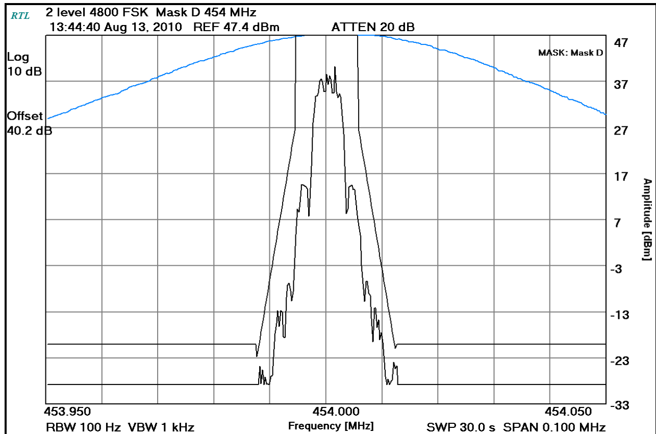
Plot 8-27: Occupied Bandwidth – 454 MHz; 2-Level 4800 FSK; (Mask D)
