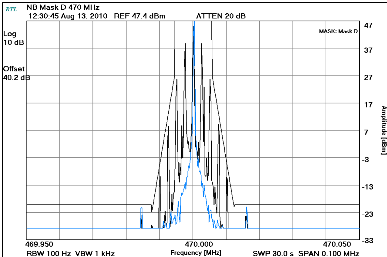
Plot 8-11: Occupied Bandwidth – 470 MHz; Analog NB (Mask D)
