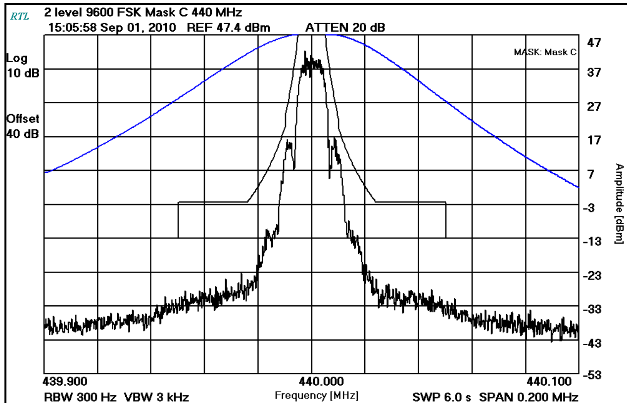
Plot 8-13: Occupied Bandwidth – 440 MHz; 2-Level 9600 FSK WB (Mask C)
