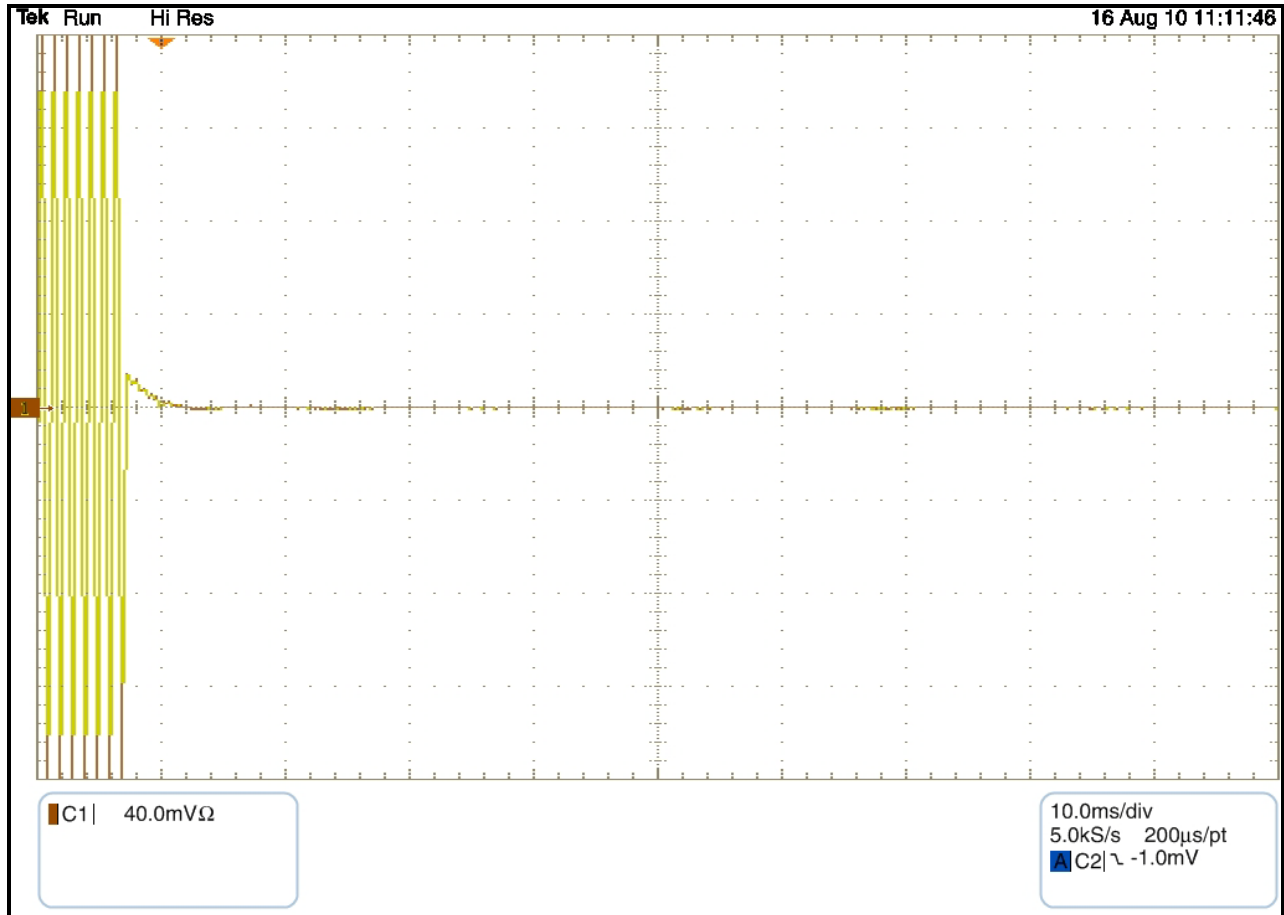
Plot 13-5: Transient Frequency Behavior – 454 MHz; High Power; Wide Band; Carrier On Time
