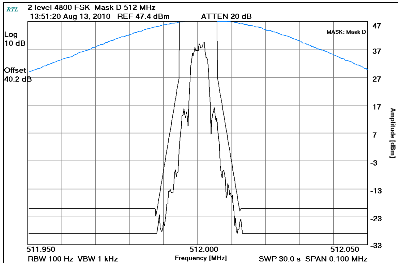
Plot 8-30: Occupied Bandwidth – 512 MHz; 2-Level 4800 FSK; (Mask D)
