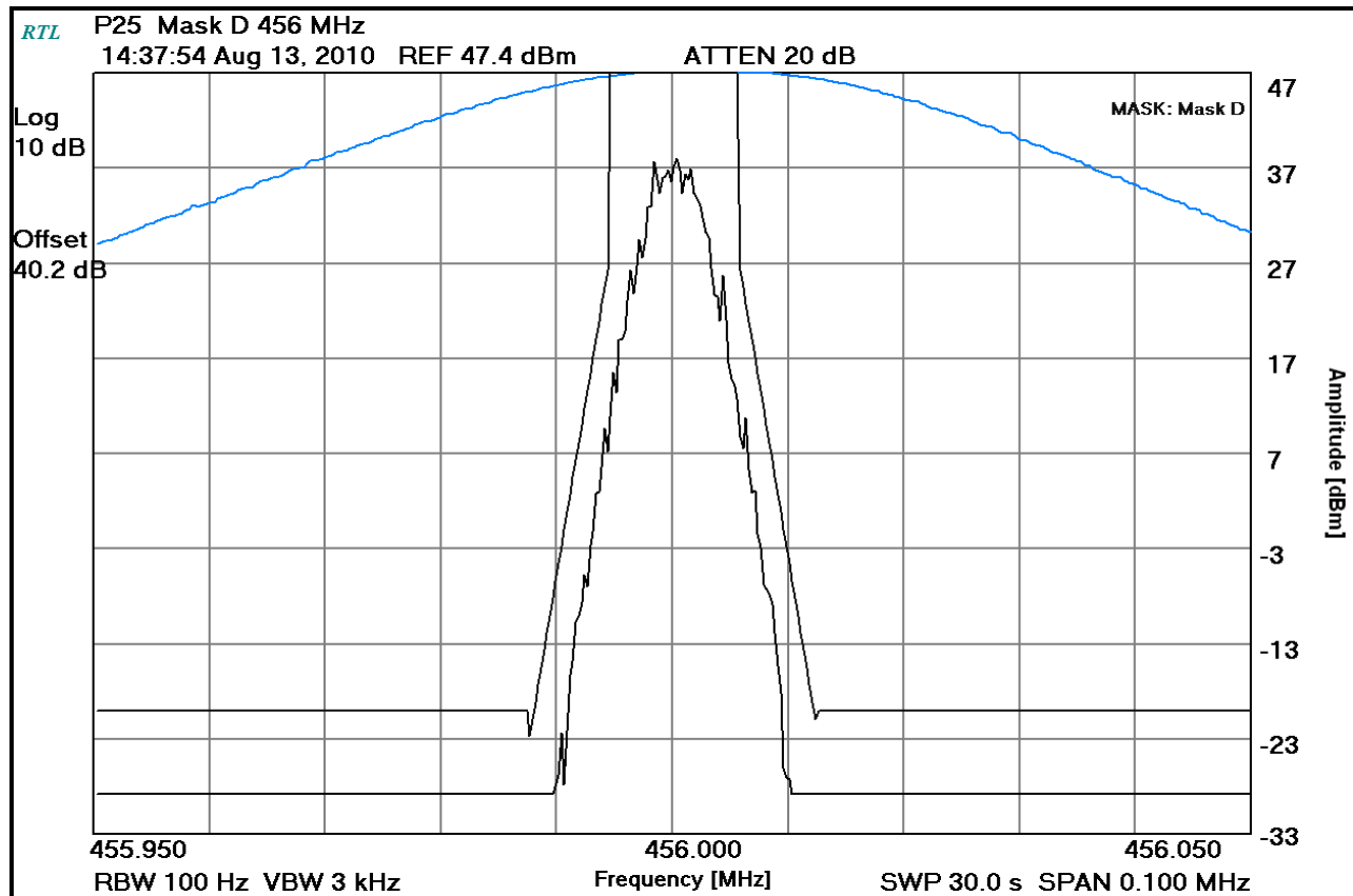
Plot 8-46: Occupied Bandwidth – 456 MHz; P25; (Mask D)
