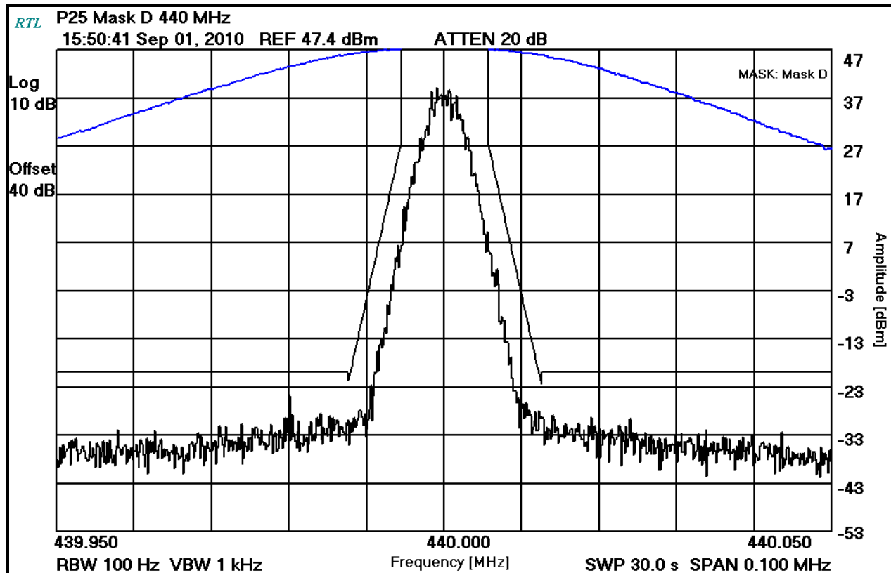
Plot 8-43: Occupied Bandwidth – 440 MHz; P25; (Mask D)
