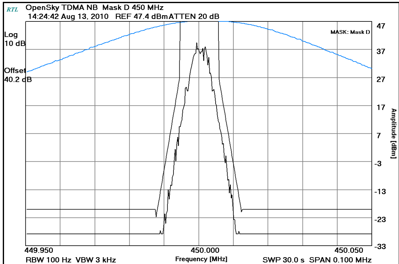
Plot 8-38: Occupied Bandwidth – 450 MHz; TDMA NB; (Mask D)
