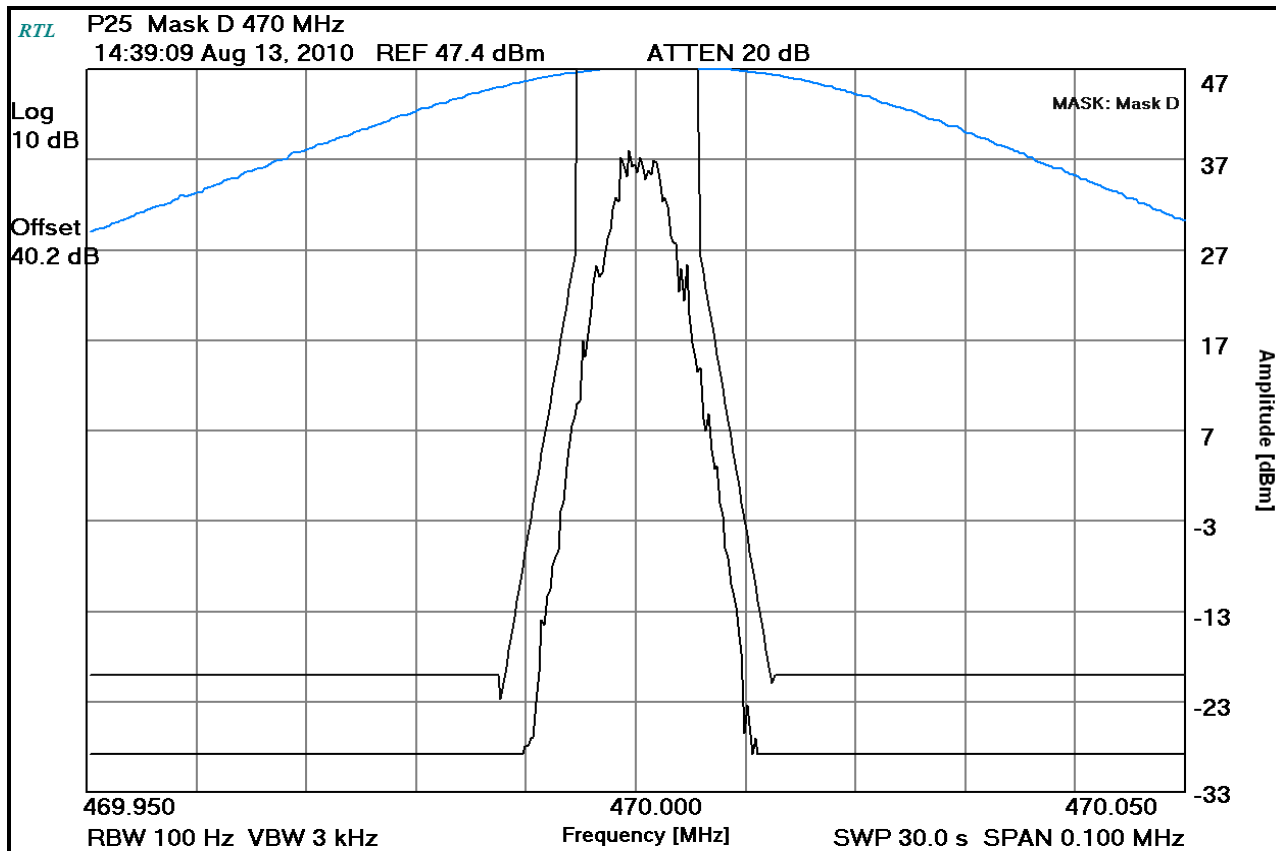
Plot 8-47: Occupied Bandwidth – 470 MHz; P25; (Mask D)
