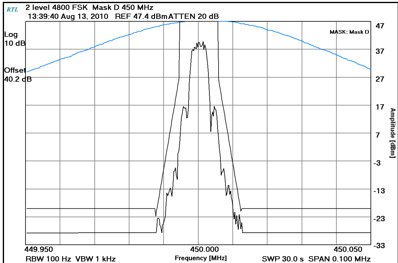
Plot 8-26: Occupied Bandwidth – 450 MHz; 2-Level 4800 FSK; (Mask D)
