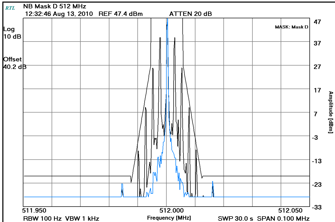
Plot 8-12: Occupied Bandwidth – 512 MHz; Analog NB (Mask D)
