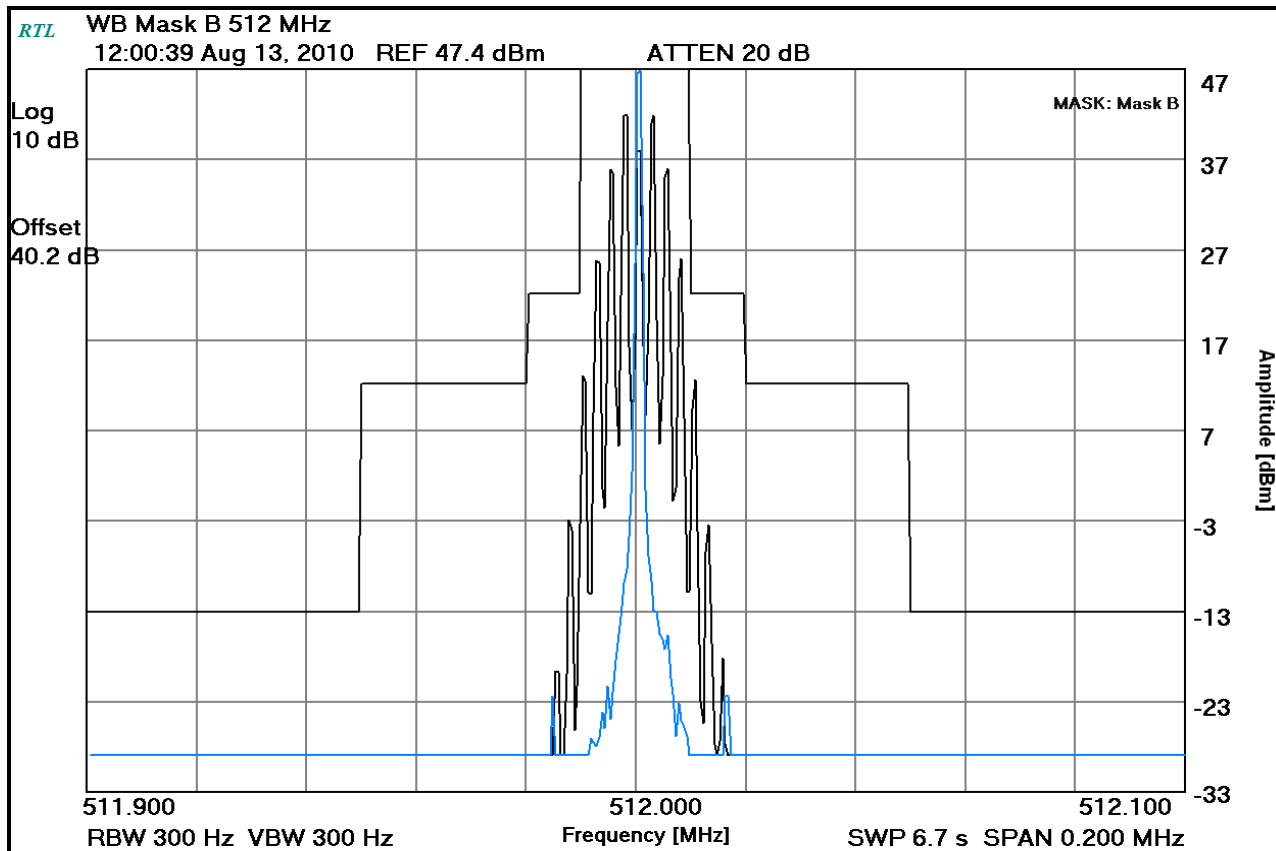
Plot 8-6: Occupied Bandwidth – 512 MHz; Analog WB (Mask B)
