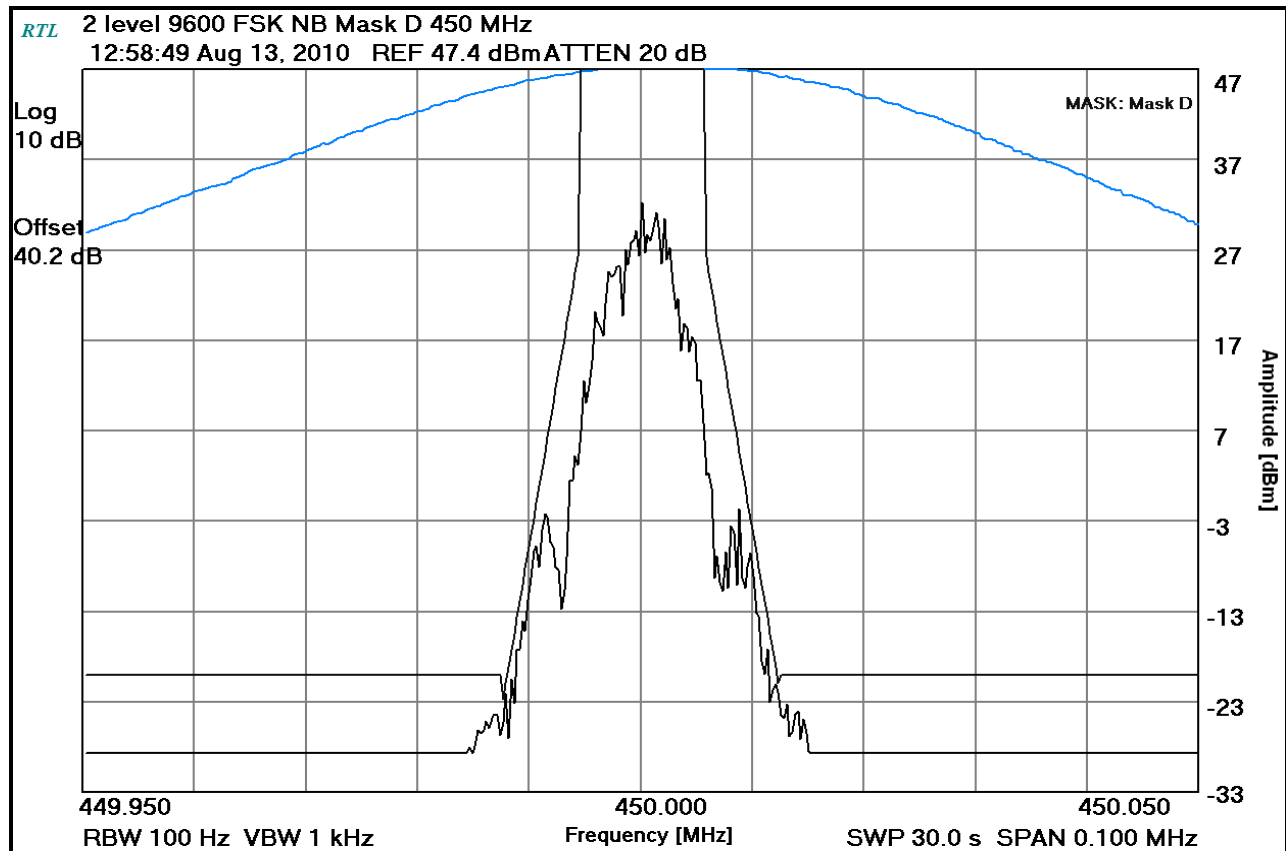
Plot 8-20: Occupied Bandwidth – 450 MHz; 2-Level 9600 FSK NB (Mask D)
