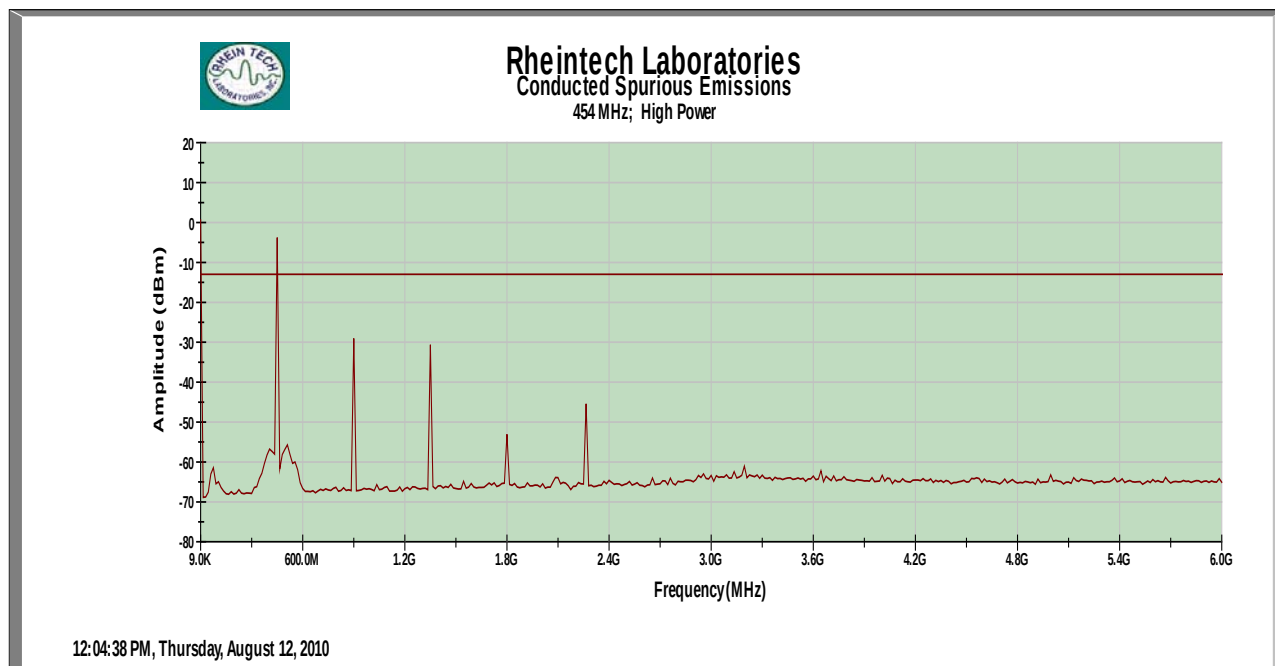
Plot 6-3: Conducted Spurious – 454 MHz – Analog High Power
