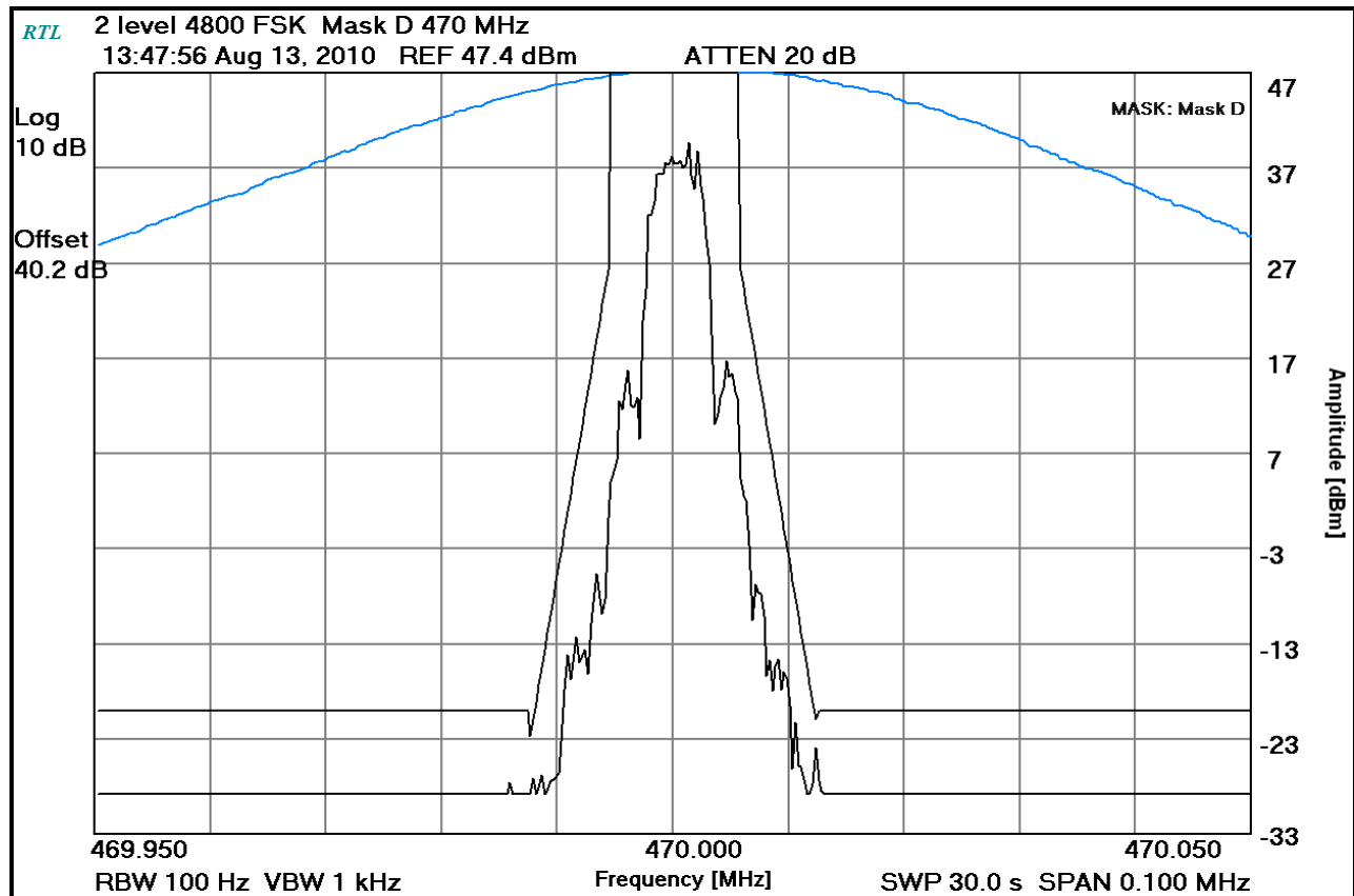
Plot 8-29: Occupied Bandwidth – 470 MHz; 2-Level 4800 FSK; (Mask D)
