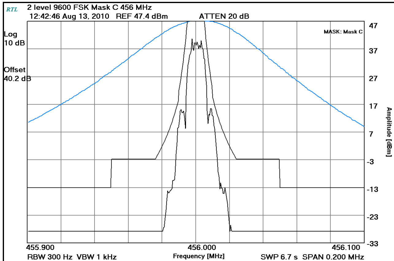
Plot 8-16: Occupied Bandwidth – 456 MHz; 2-Level 9600 FSK WB (Mask C)
