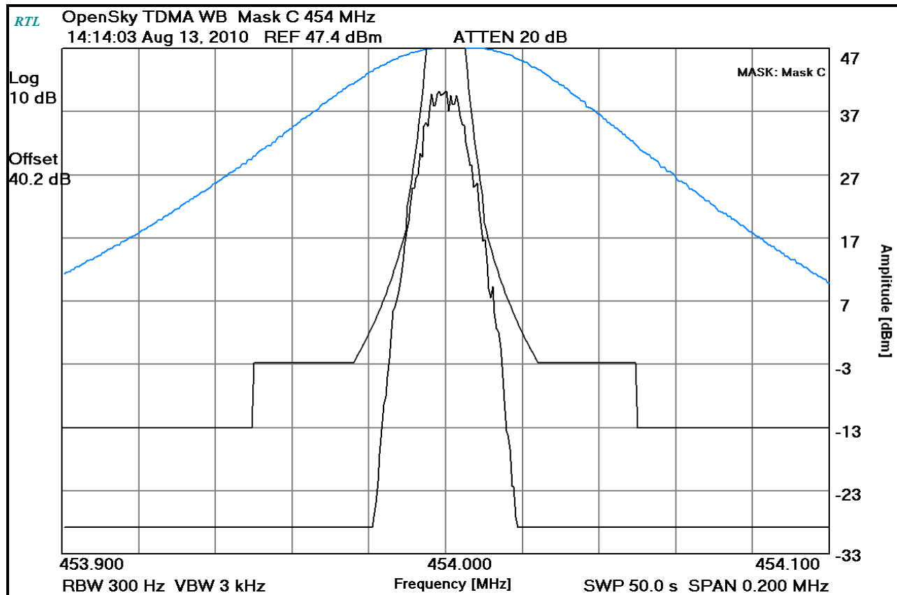
Plot 8-33: Occupied Bandwidth – 454 MHz; TDMA WB; (Mask C)
