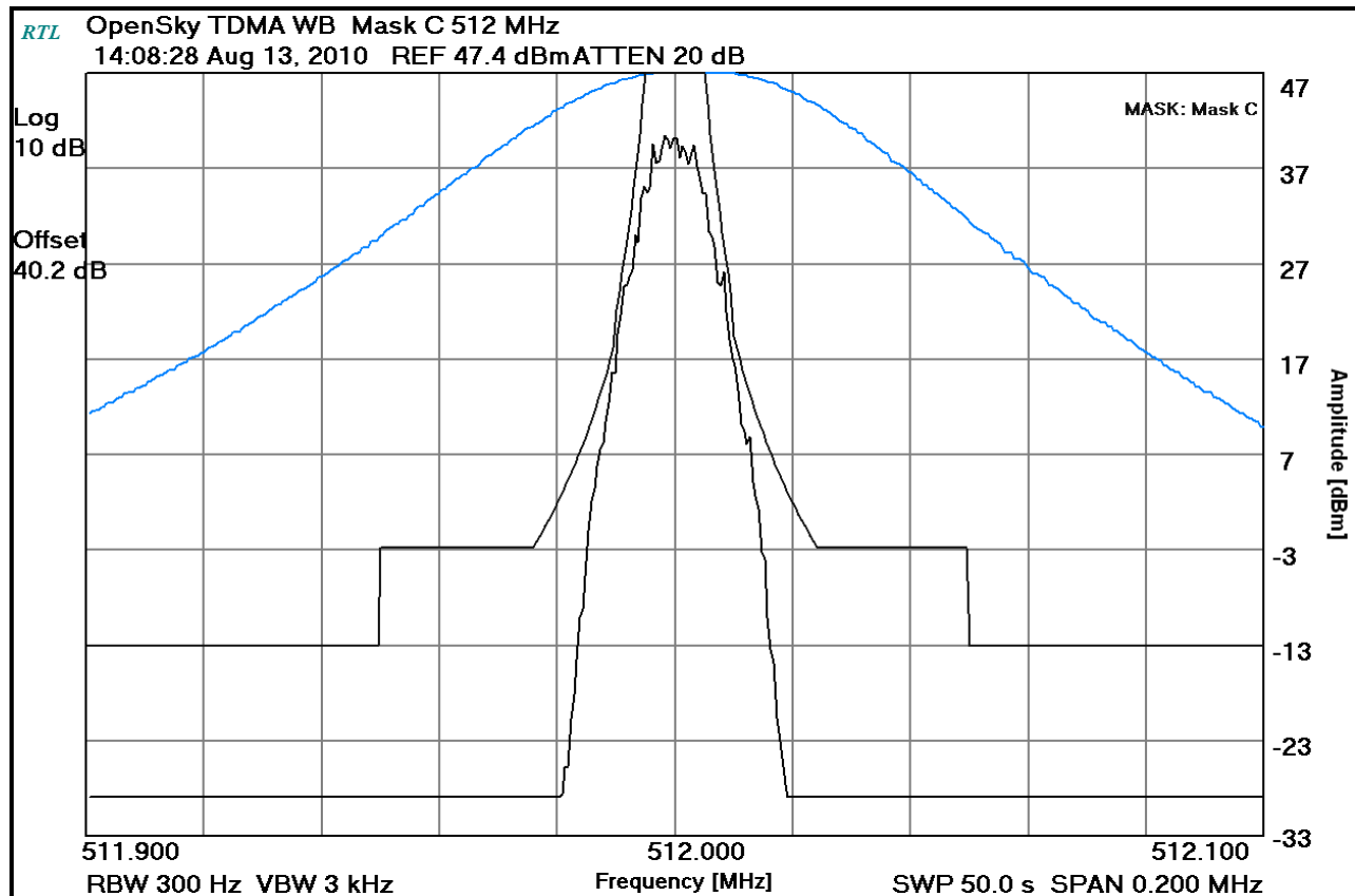
Plot 8-36: Occupied Bandwidth – 512 MHz; TDMA WB; (Mask C)
