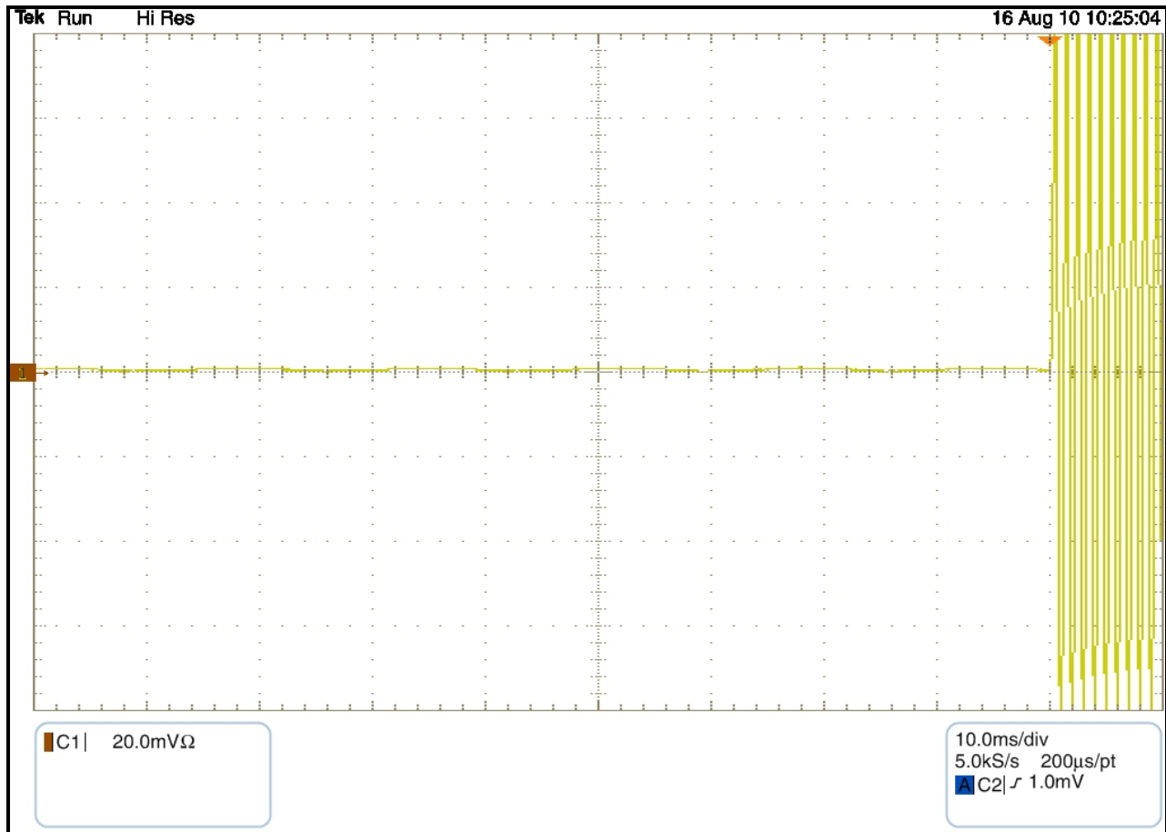
Plot 13-12: Transient Frequency Behavior – 456 MHz; High Power; Narrow Band; Carrier Off Time
