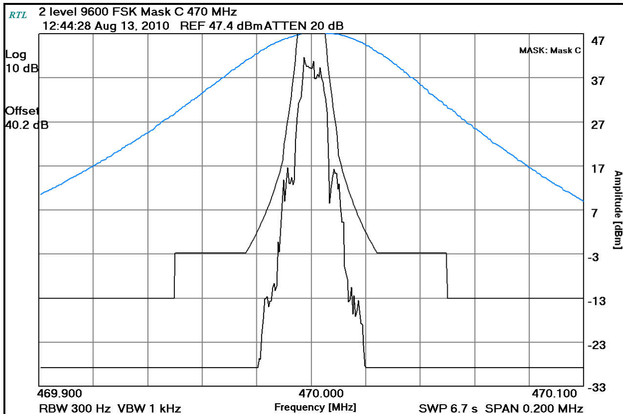
Plot 8-17: Occupied Bandwidth – 470 MHz; 2-Level 9600 FSK WB (Mask C)
