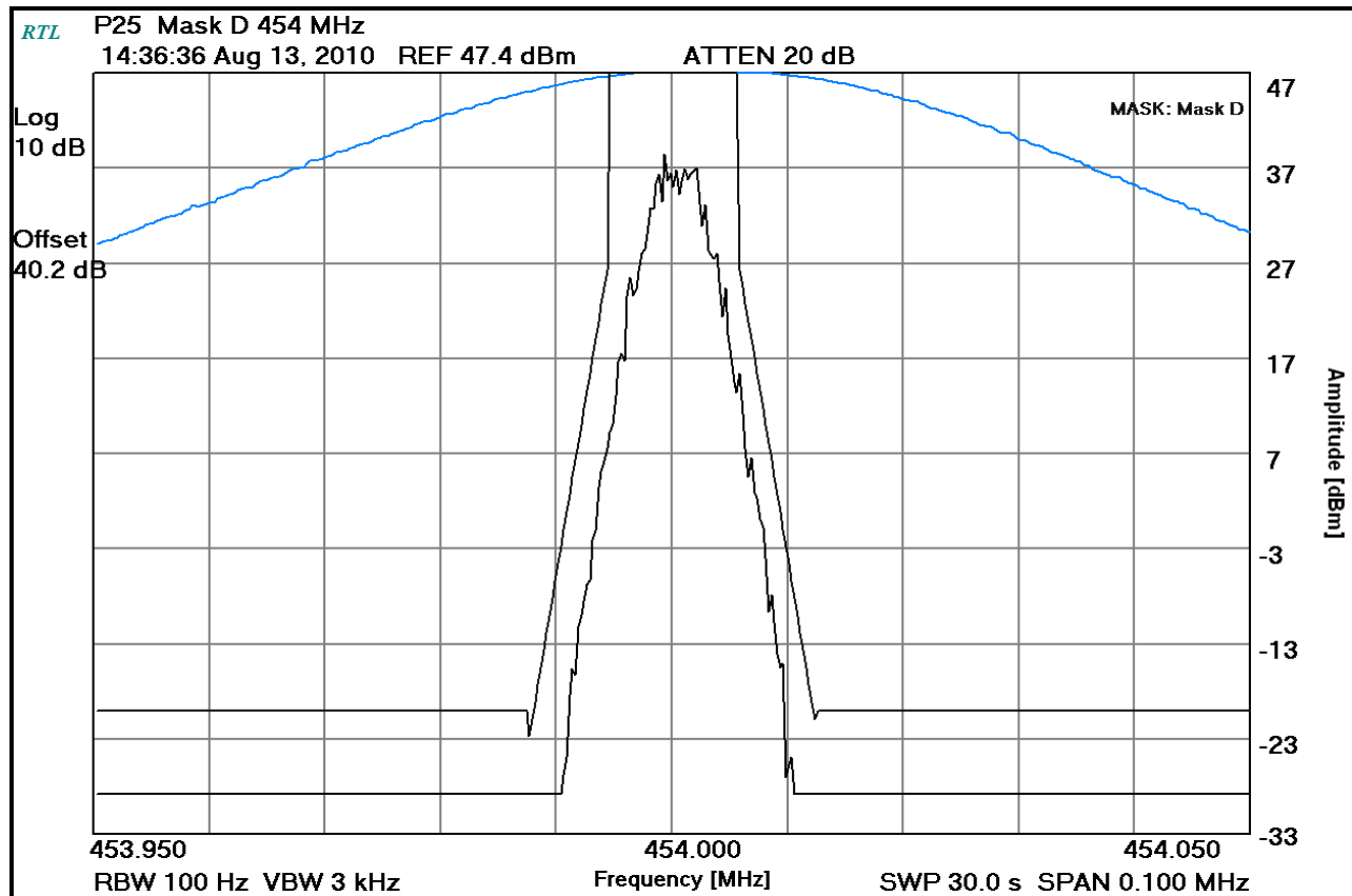
Plot 8-45: Occupied Bandwidth – 454 MHz; P25; (Mask D)
