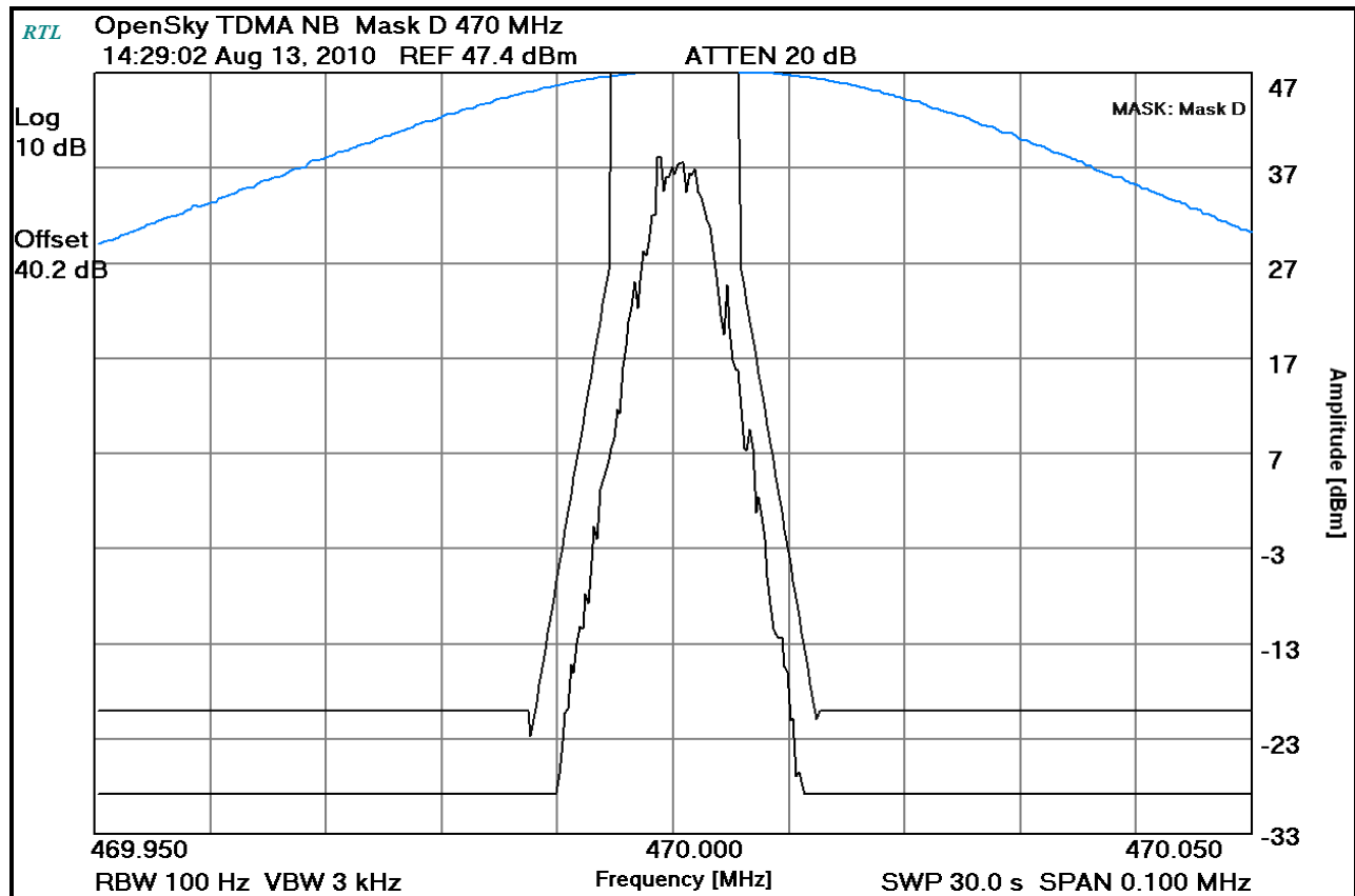
Plot 8-41: Occupied Bandwidth – 470 MHz; TDMA NB; (Mask D)
