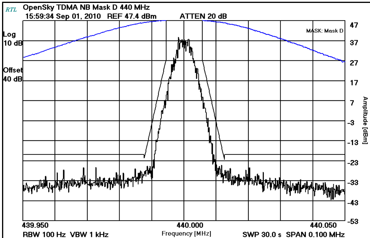
Plot 8-37: Occupied Bandwidth – 440 MHz; TDMA NB; (Mask D)
