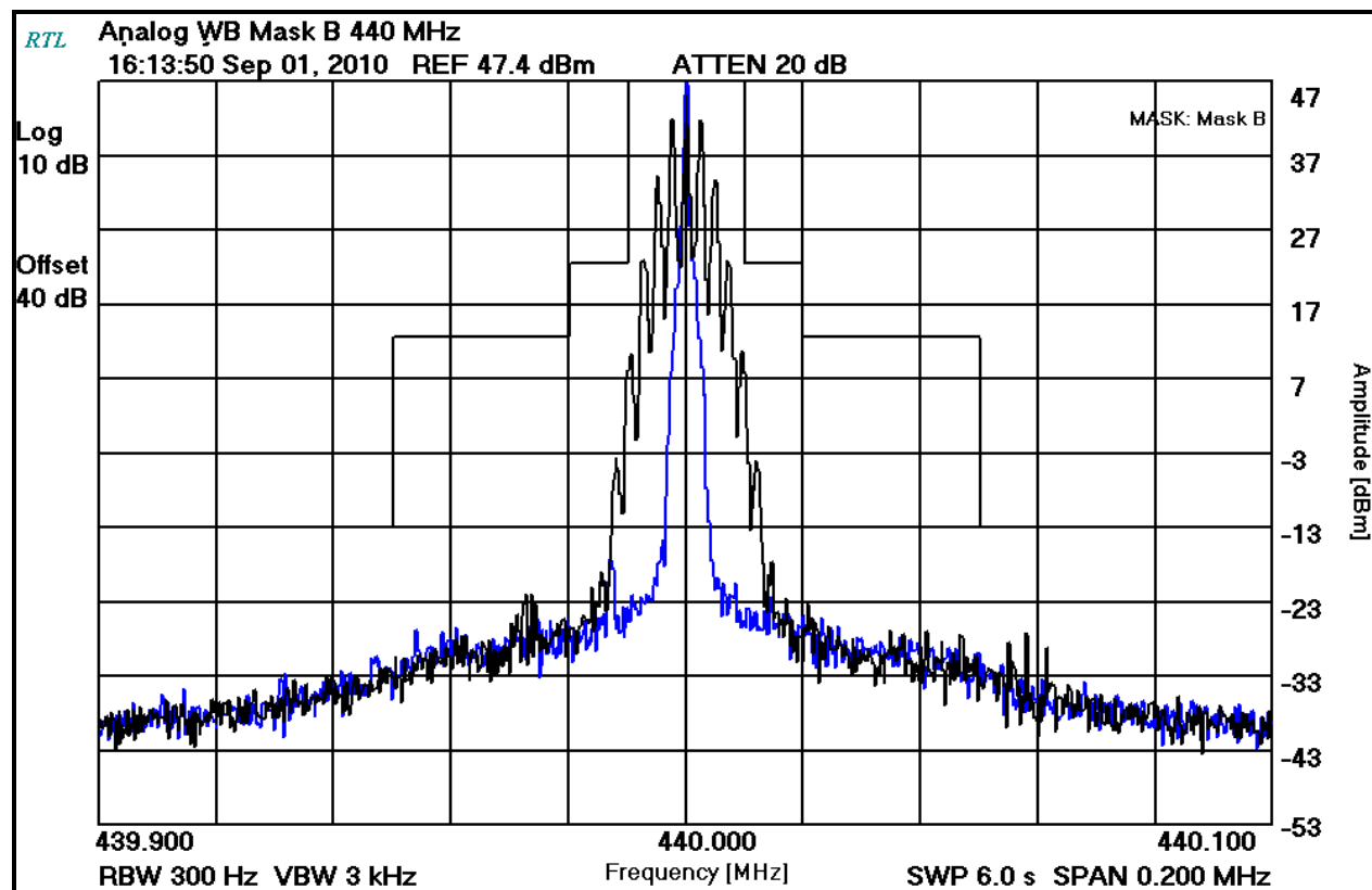
Plot 8-1: Occupied Bandwidth – 440 MHz; Analog WB (Mask B)
