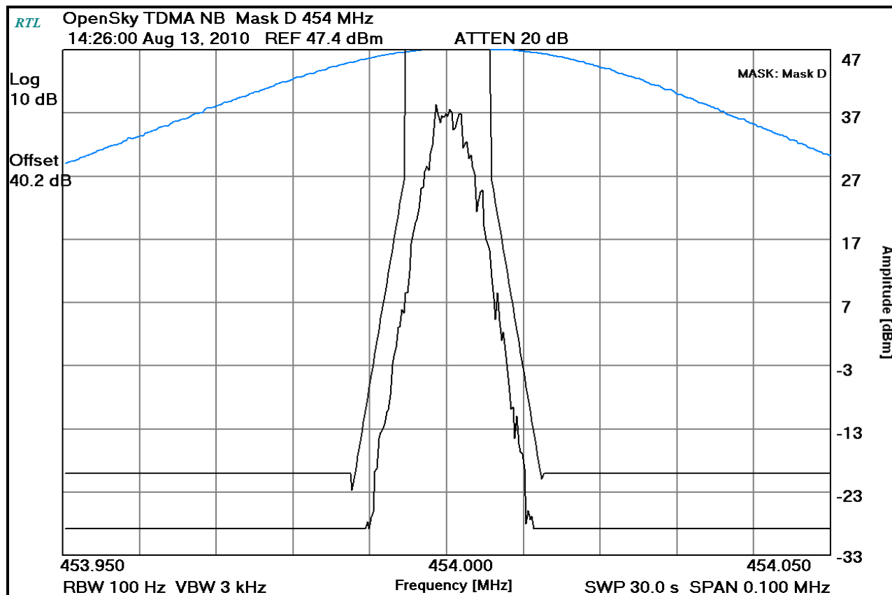
Plot 8-39: Occupied Bandwidth – 454 MHz; TDMA NB; (Mask D)
