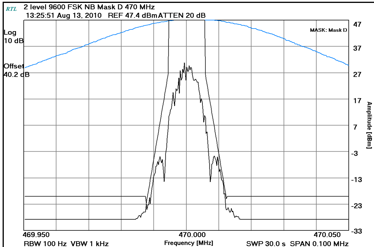
Plot 8-23: Occupied Bandwidth – 470 MHz; 2-Level 9600 FSK NB (Mask D)
