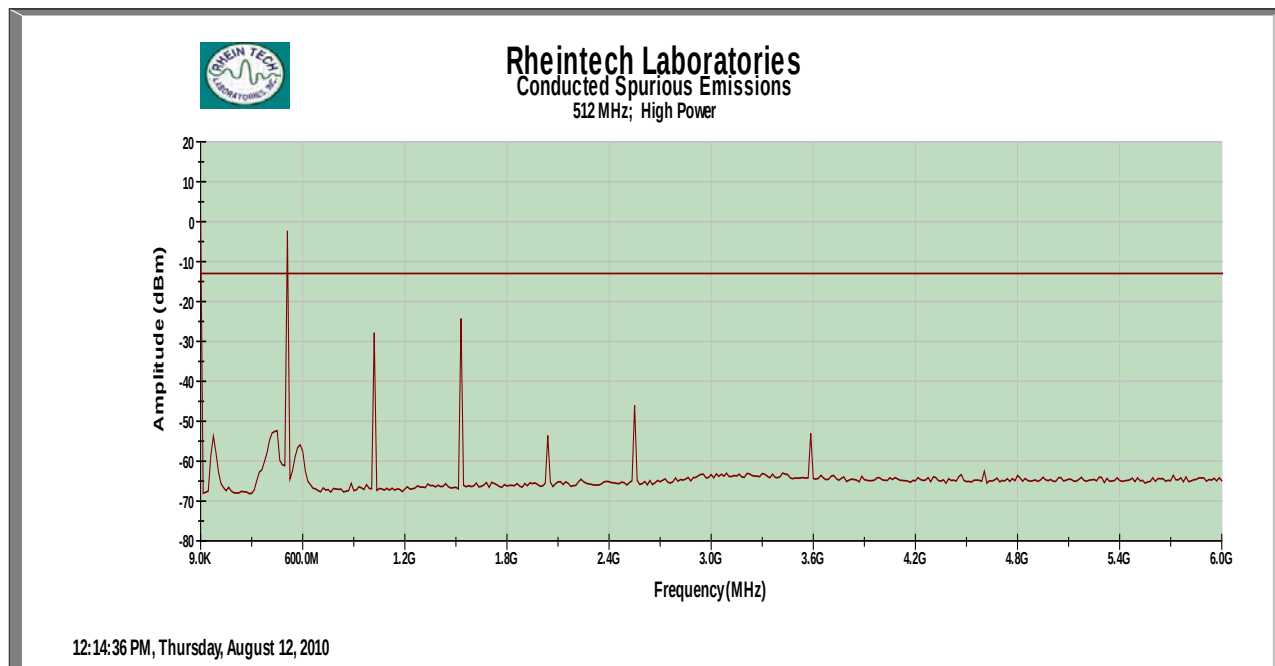
Plot 6-6: Conducted Spurious – 512 MHz – Analog High Power
