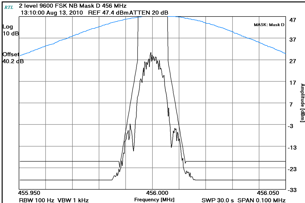
Plot 8-22: Occupied Bandwidth – 456 MHz; 2-Level 9600 FSK NB (Mask D)
