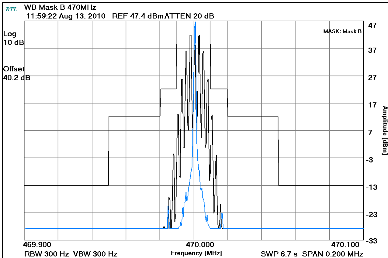
Plot 8-5: Occupied Bandwidth – 470 MHz; Analog WB (Mask B)
