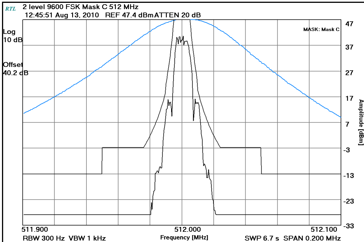
Plot 8-18: Occupied Bandwidth – 512 MHz; 2-Level 9600 FSK WB (Mask C)
