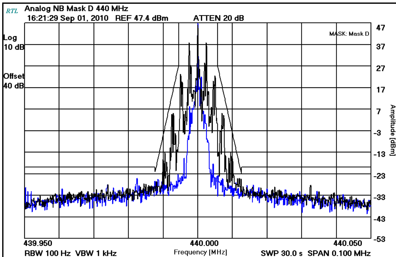
Plot 8-7: Occupied Bandwidth – 440 MHz; Analog NB (Mask D)
