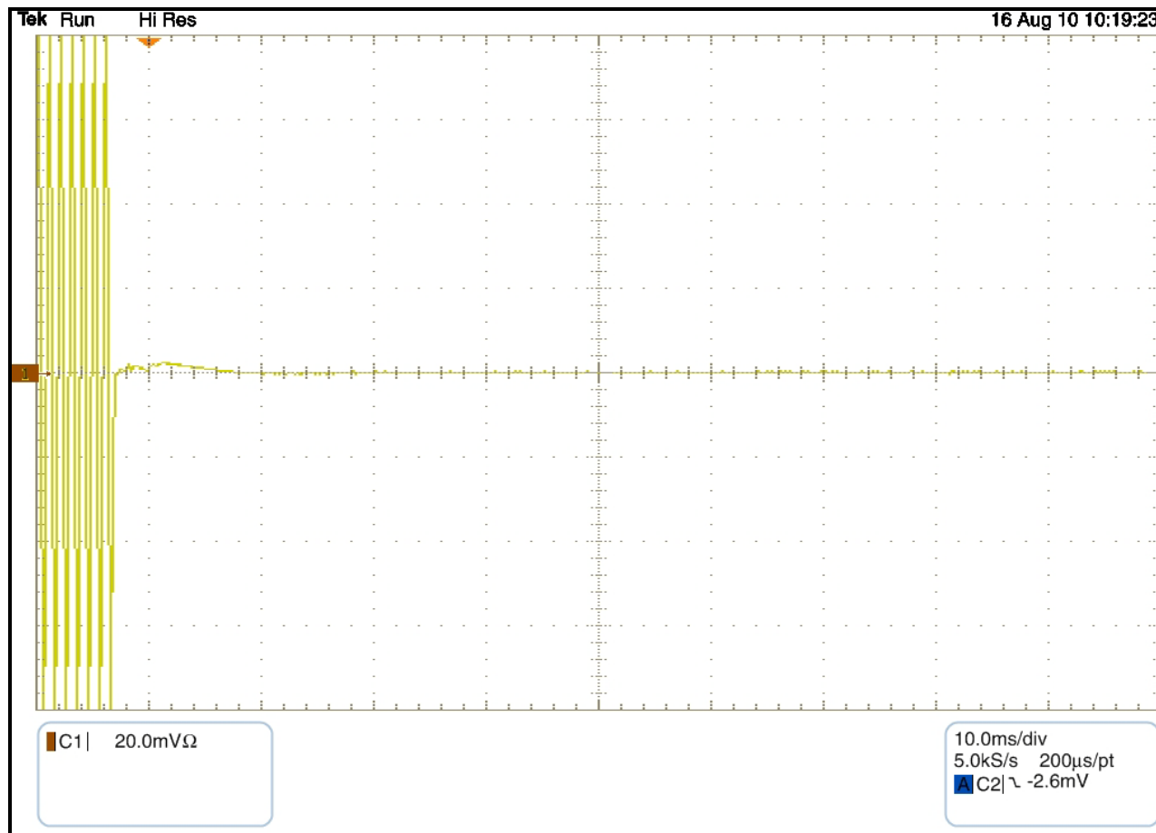
Plot 13-7: Transient Frequency Behavior – 454 MHz; High Power; Narrow Band; Carrier On Time
