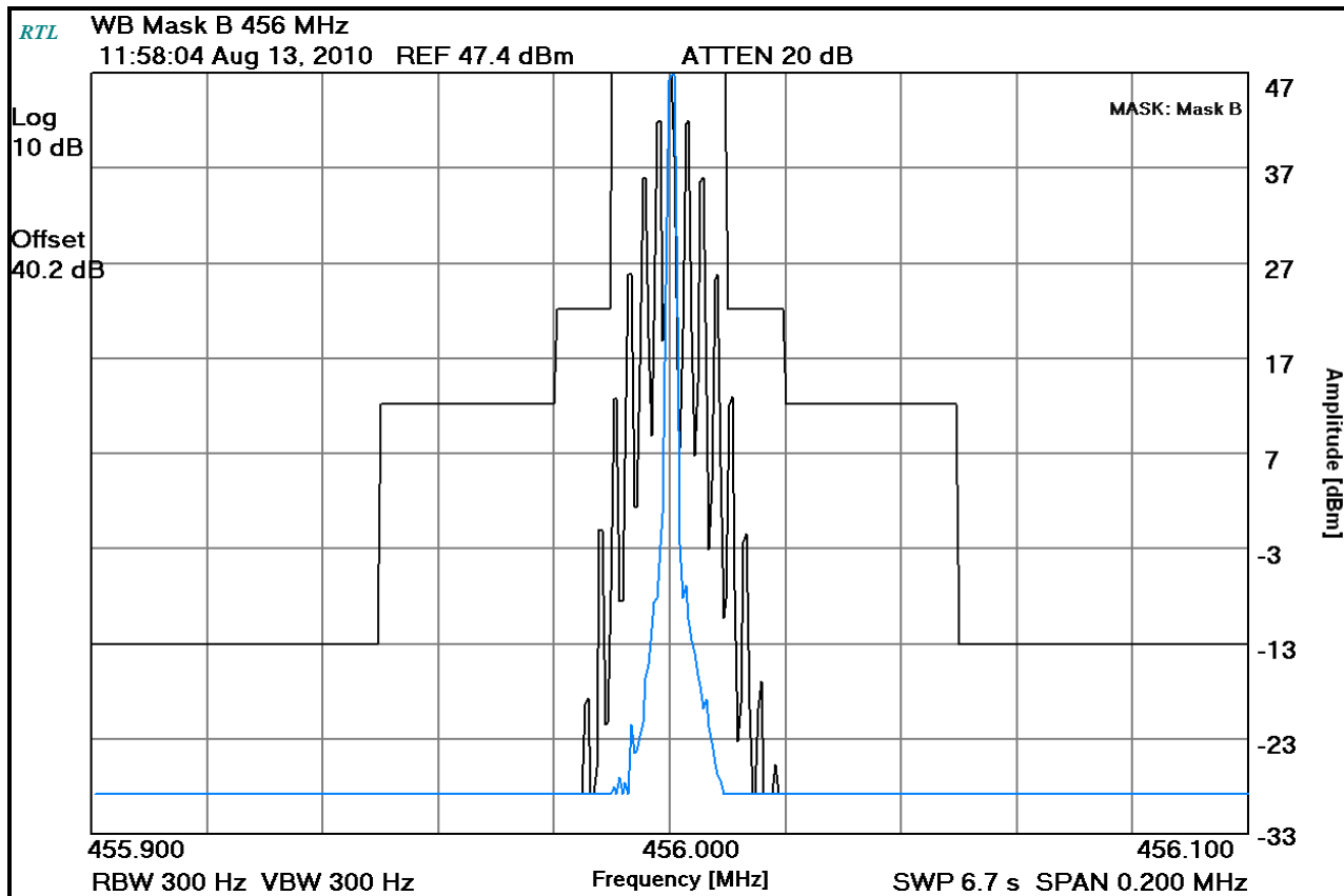
Plot 8-4: Occupied Bandwidth – 456 MHz; Analog WB (Mask B)
