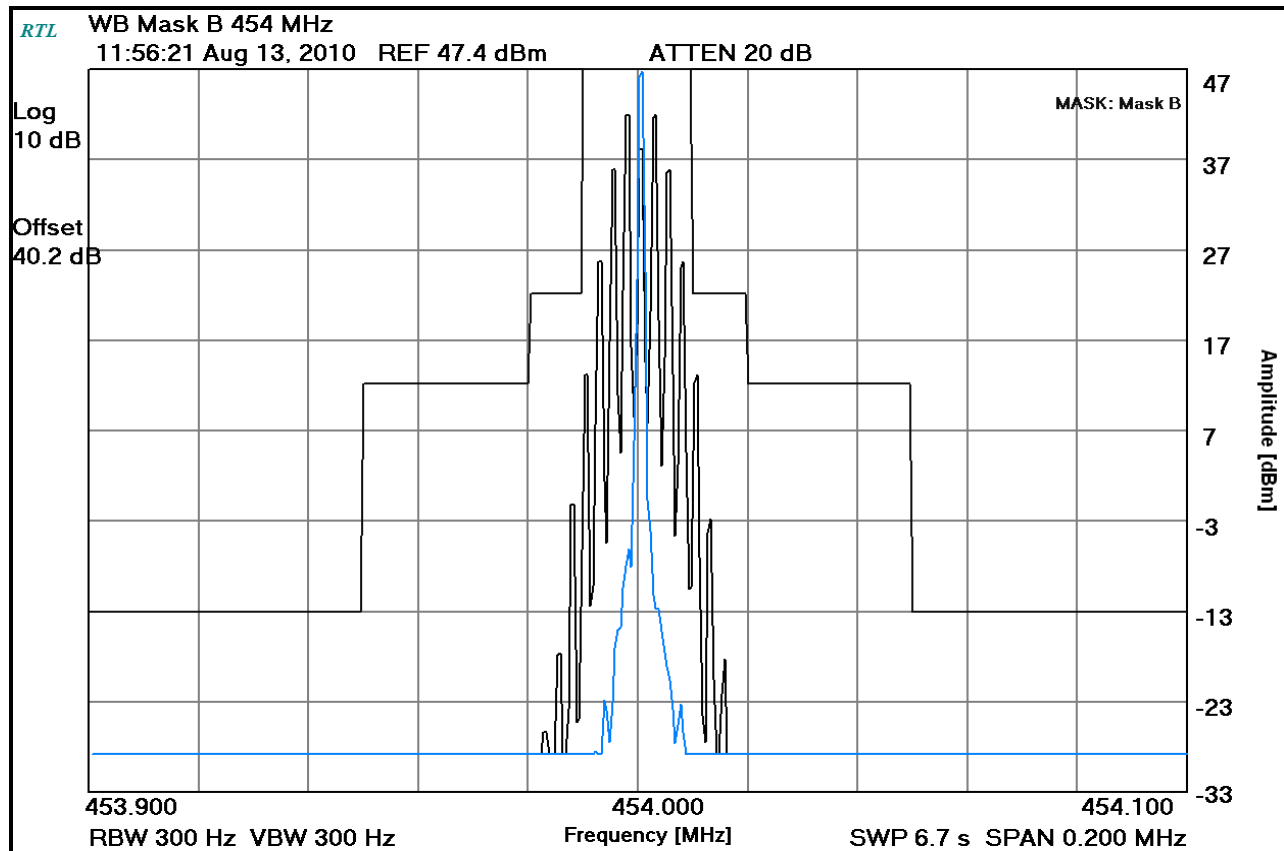
Plot 8-3: Occupied Bandwidth – 454 MHz; Analog WB (Mask B)
