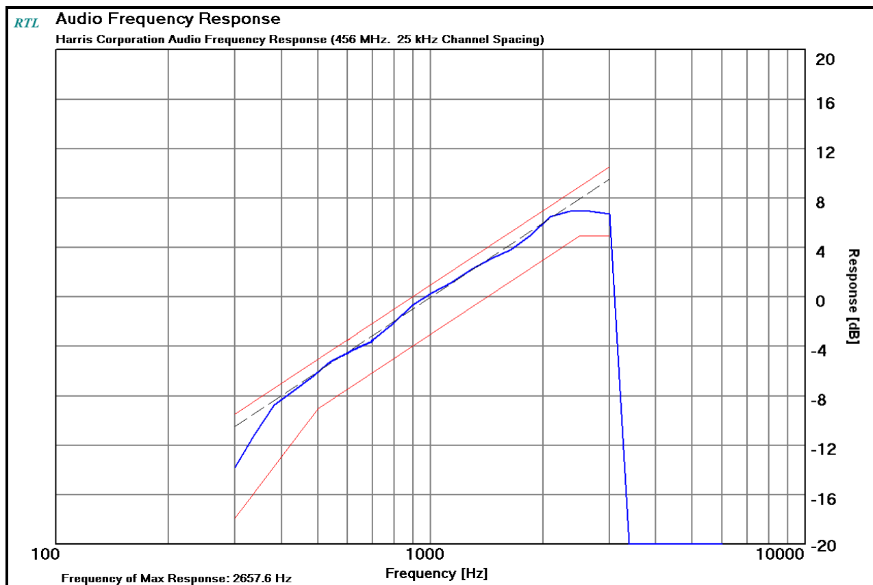
Plot 10-1: Modulation Characteristics - Audio Frequency Response
