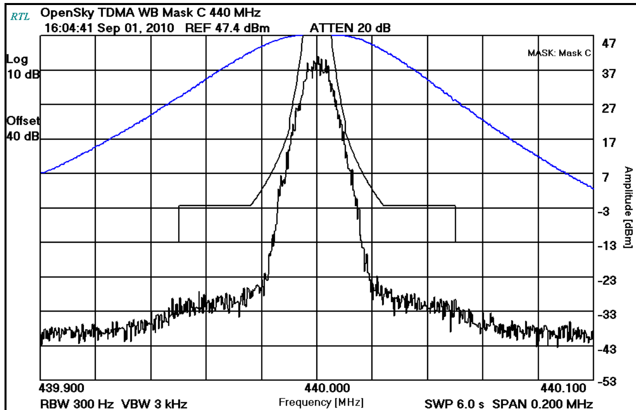
Plot 8-31: Occupied Bandwidth – 440 MHz; TDMA WB; (Mask C)
