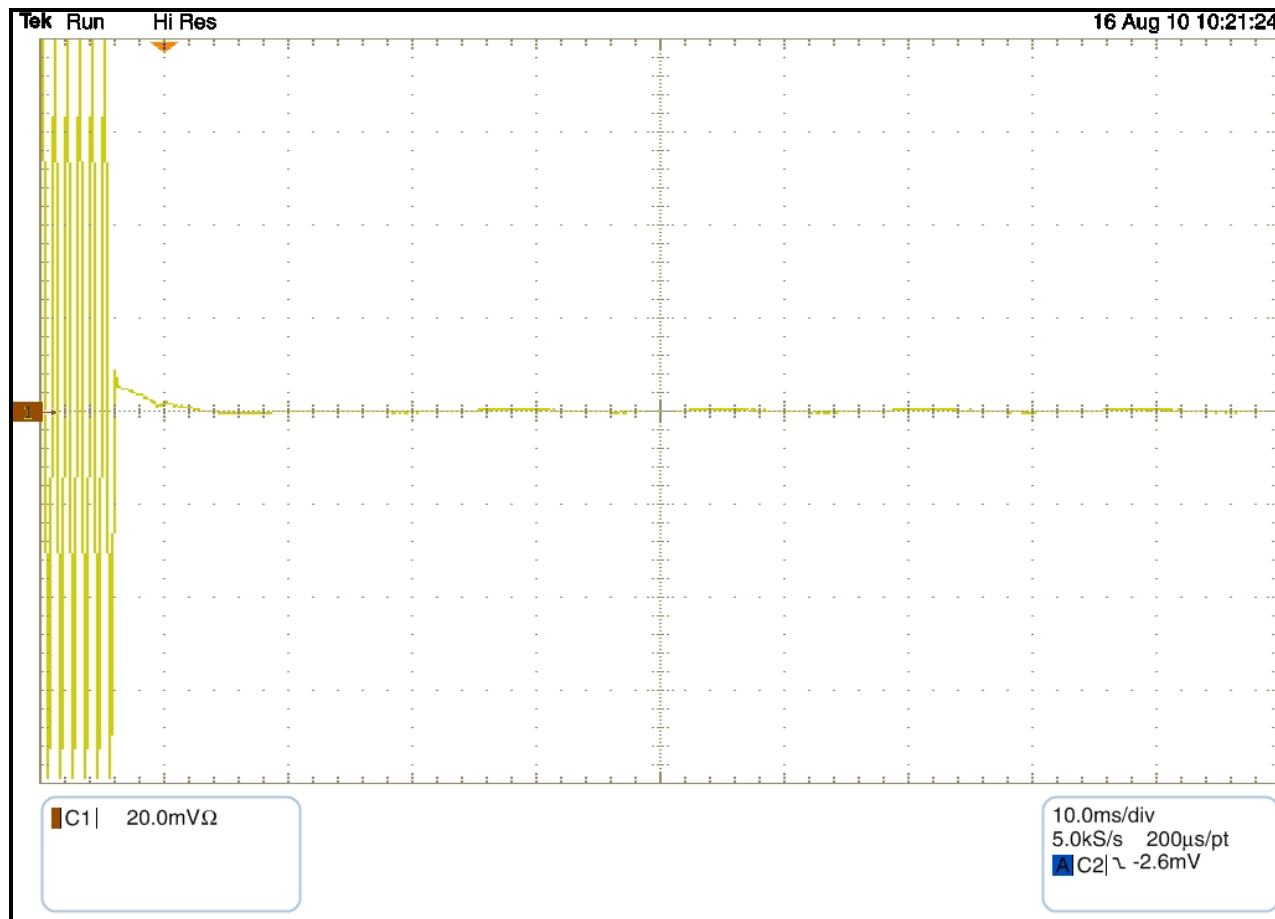
Plot 13-19: Transient Frequency Behavior – 512 MHz; High Power; Narrow Band; Carrier On Time
