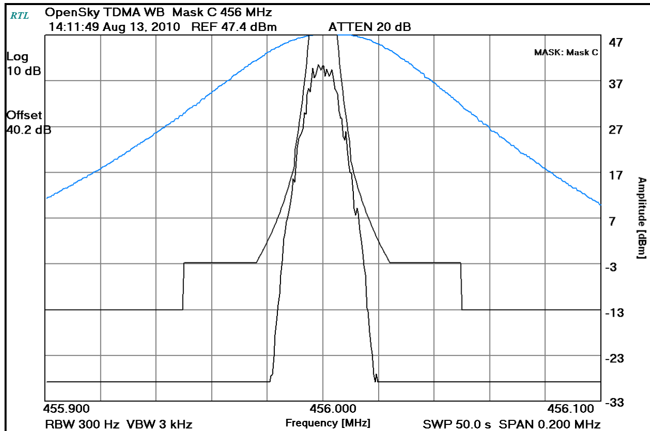
Plot 8-34: Occupied Bandwidth – 456 MHz; TDMA WB; (Mask C)
