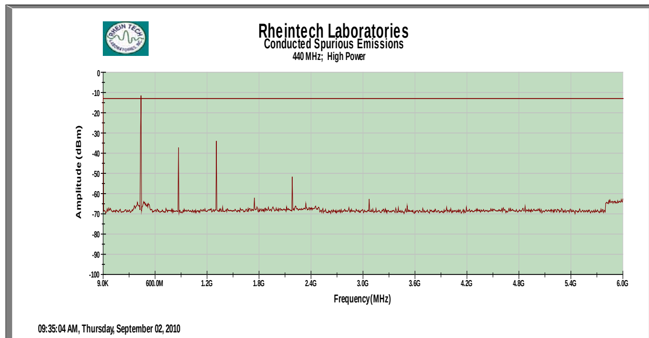
Plot 6-1: Conducted Spurious - 440 MHz - Analog High Power
