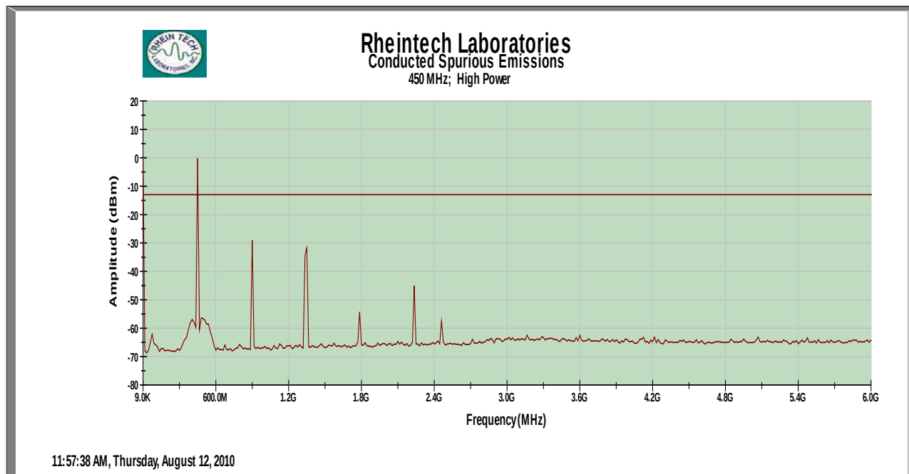
Plot 6-2: Conducted Spurious - 450 MHz - Analog High Power
