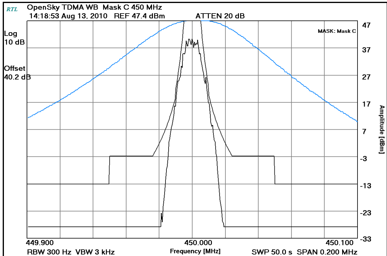
Plot 8-32: Occupied Bandwidth – 450 MHz; TDMA WB; (Mask C)
