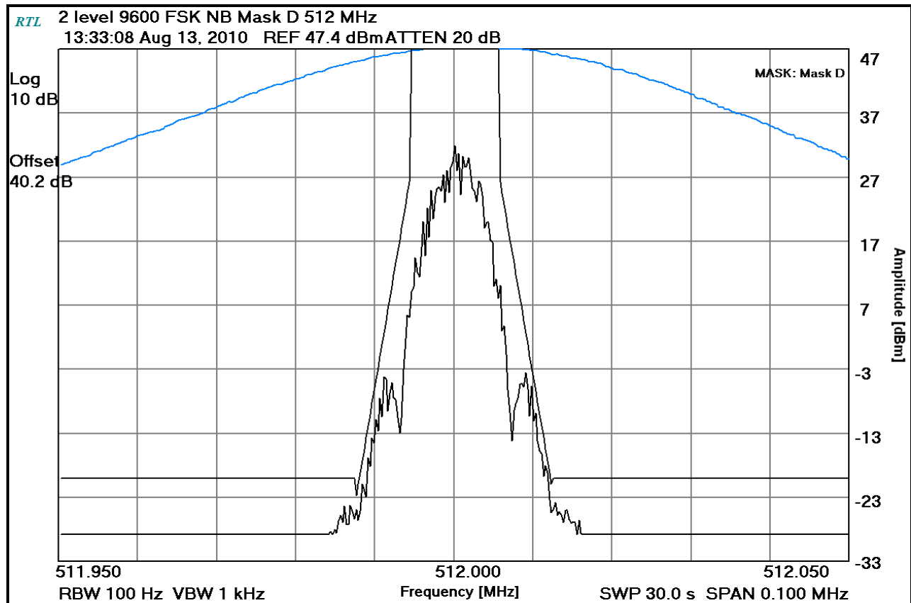
Plot 8-24: Occupied Bandwidth – 512 MHz; 2-Level 9600 FSK NB (Mask D)
