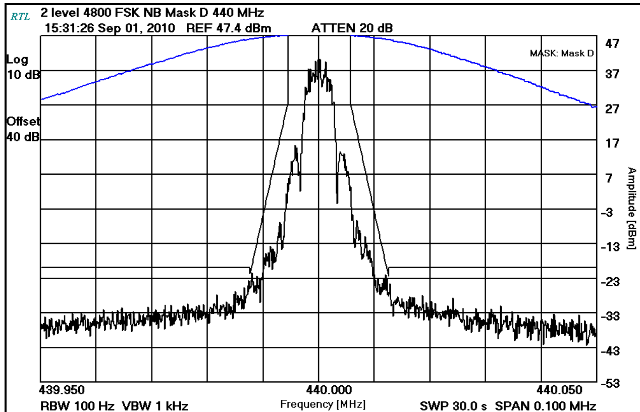
Plot 8-25: Occupied Bandwidth – 440 MHz; 2-Level 4800 FSK; (Mask D)
