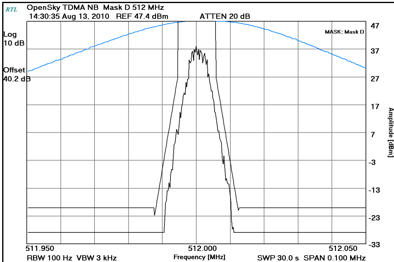
Plot 8-42: Occupied Bandwidth – 512 MHz; TDMA NB; (Mask D)
