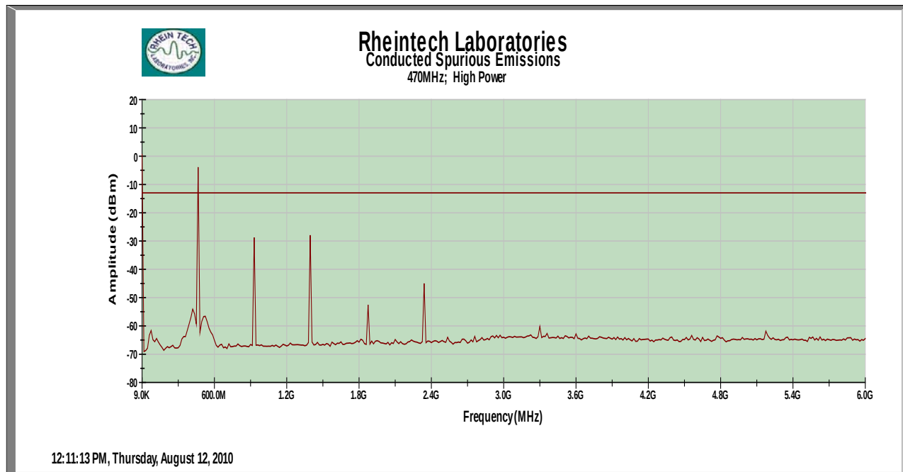
Plot 6-5: Conducted Spurious – 470 MHz – Analog High Power
