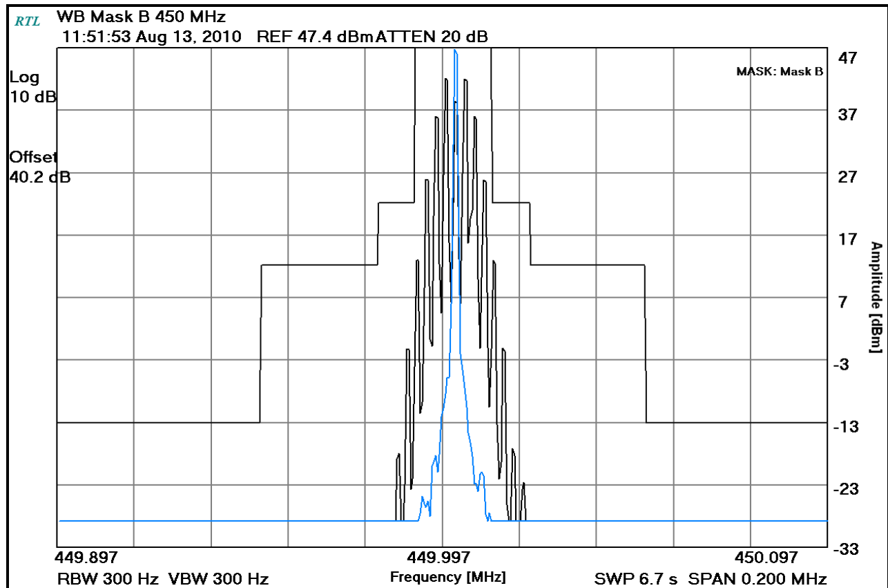
Plot 8-2: Occupied Bandwidth – 450 MHz; Analog WB (Mask B)
