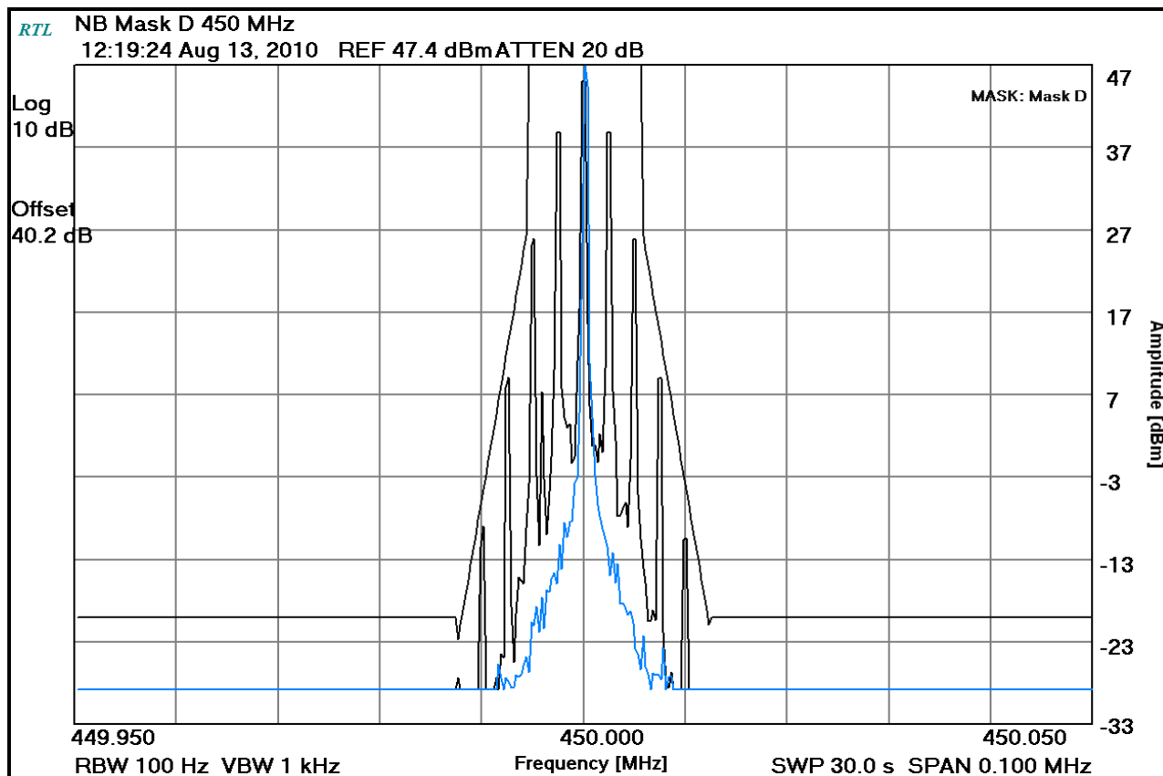
Plot 8-8: Occupied Bandwidth – 450 MHz; Analog NB (Mask D)
