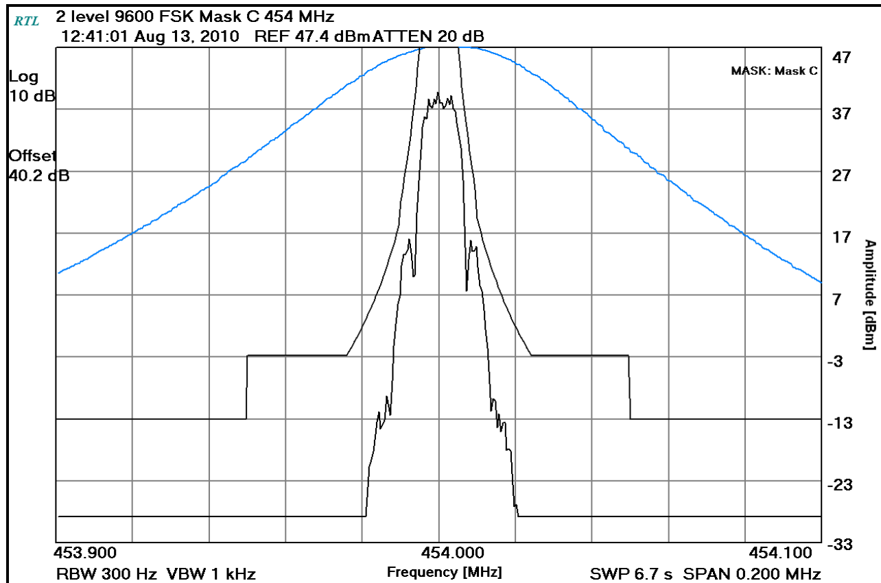
Plot 8-15: Occupied Bandwidth – 454 MHz; 2-Level 9600 FSK WB (Mask C)
