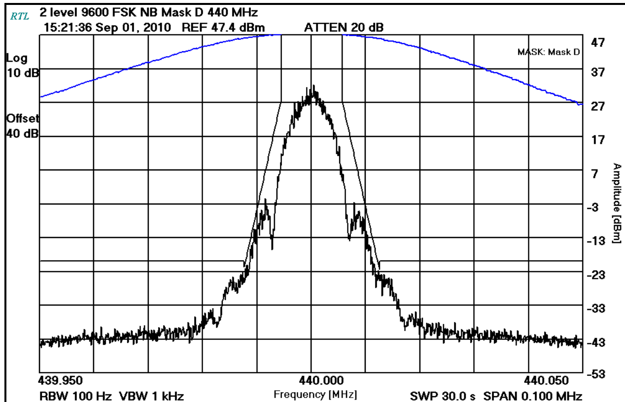
Plot 8-19: Occupied Bandwidth – 440 MHz; 2-Level 9600 FSK NB (Mask D)
