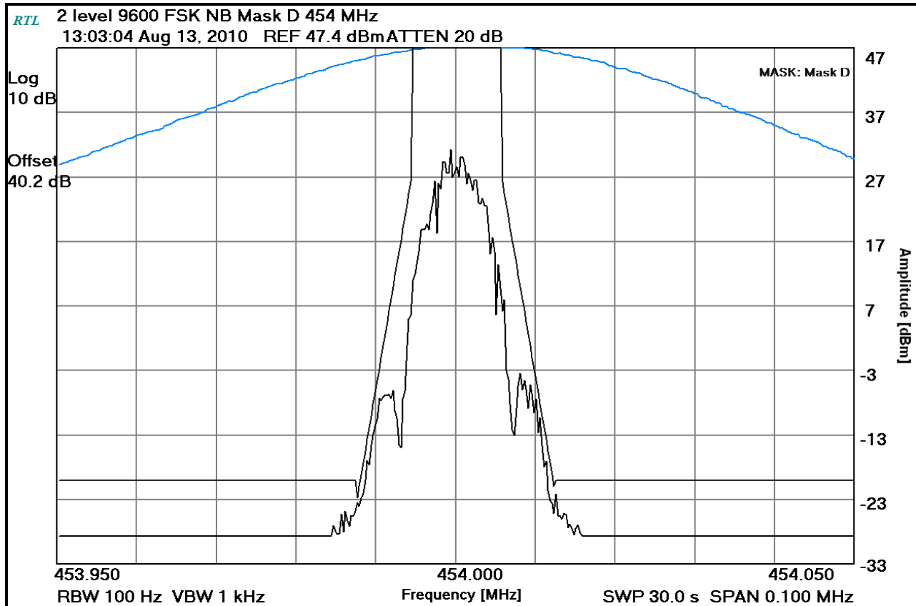
Plot 8-21: Occupied Bandwidth – 454 MHz; 2-Level 9600 FSK NB (Mask D)
