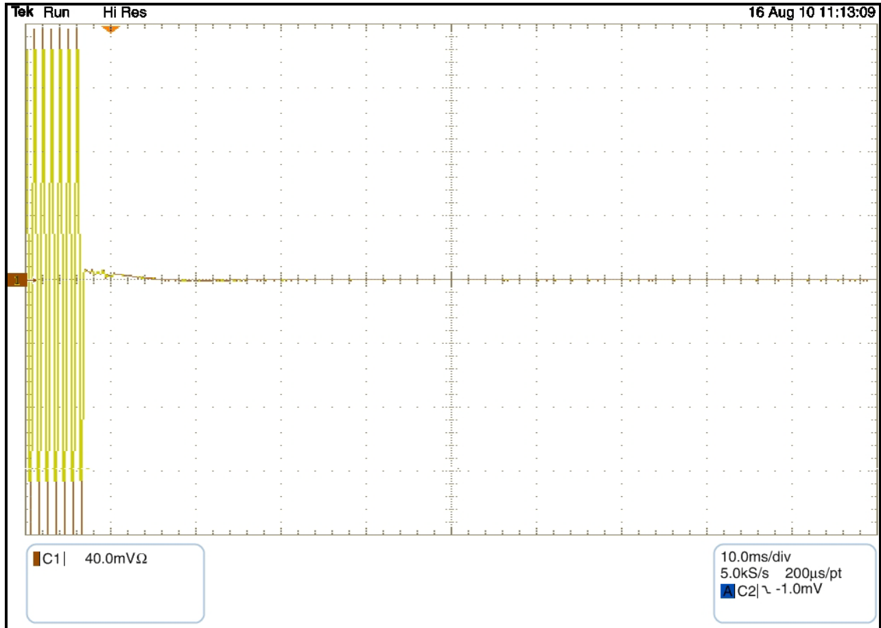
Plot 13-13: Transient Frequency Behavior – 470 MHz; High Power; Wide Band; Carrier On Time
