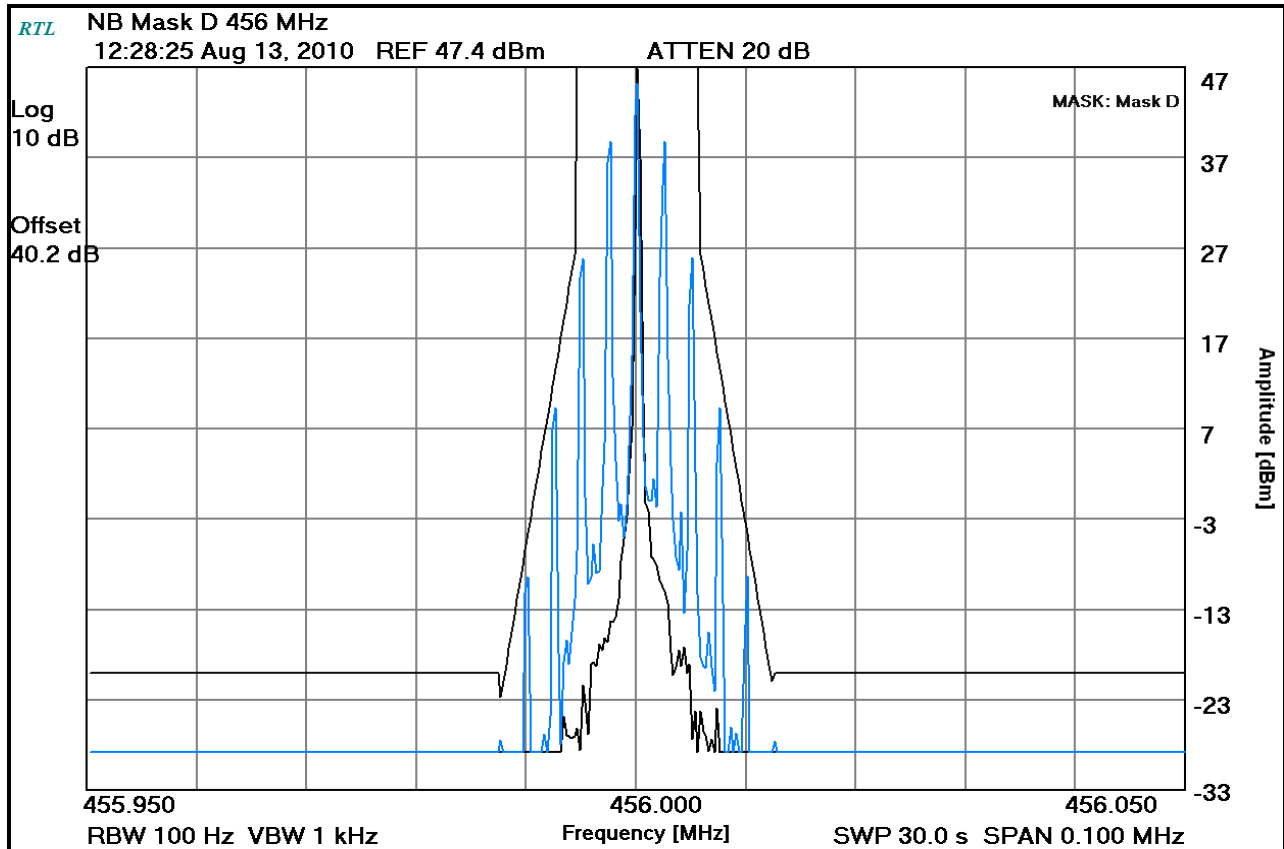
Plot 8-10: Occupied Bandwidth – 456 MHz; Analog NB (Mask D)
