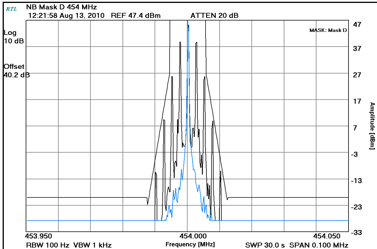
Plot 8-9: Occupied Bandwidth – 454 MHz; Analog NB (Mask D)
