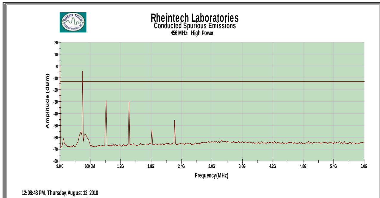
Plot 6-4: Conducted Spurious – 456 MHz – Analog High Power
