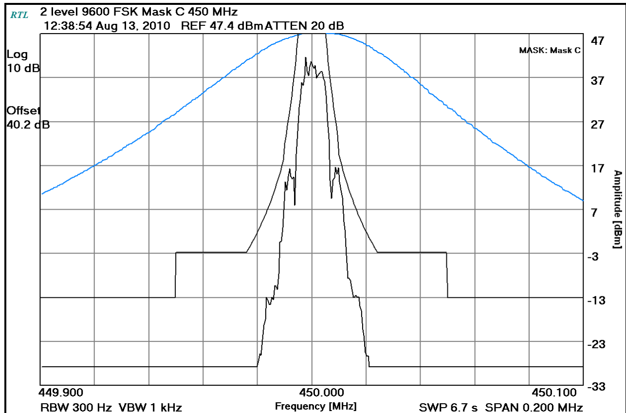
Plot 8-14: Occupied Bandwidth – 450 MHz; 2-Level 9600 FSK WB (Mask C)
