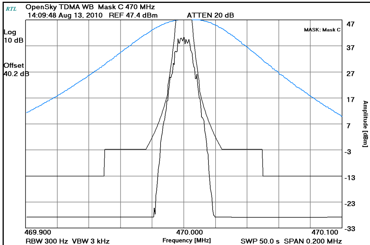
Plot 8-35: Occupied Bandwidth – 470 MHz; TDMA WB; (Mask C)
