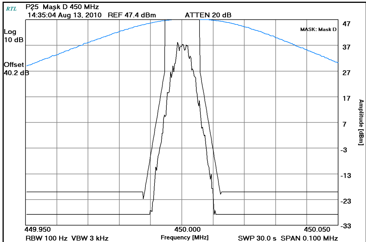
Plot 8-44: Occupied Bandwidth – 450 MHz; P25; (Mask D)
