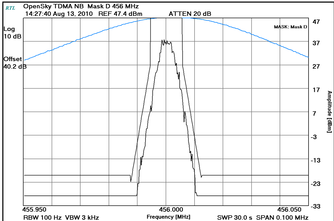
Plot 8-40: Occupied Bandwidth – 456 MHz; TDMA NB; (Mask D)
