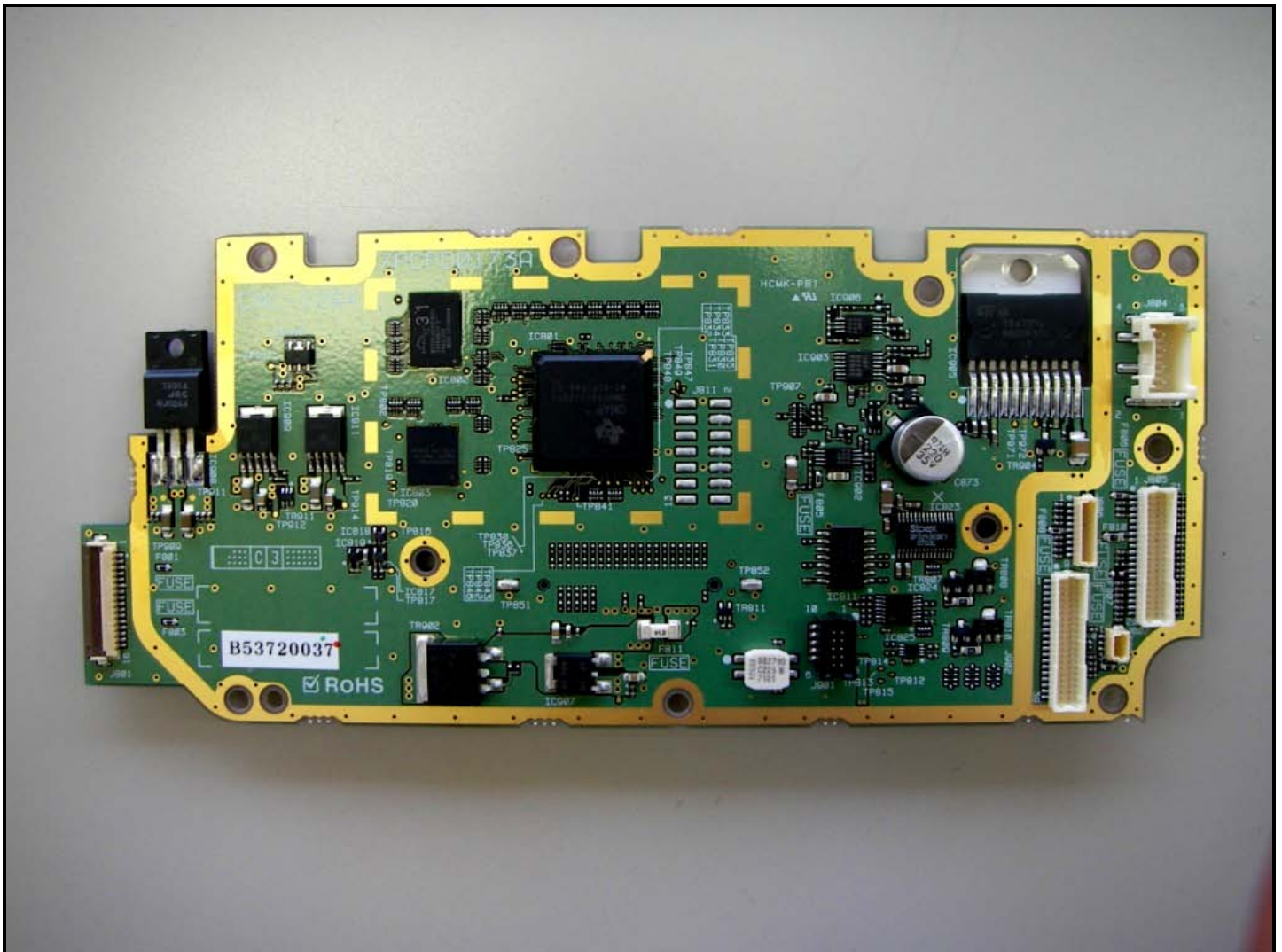
Photograph 17: PK Board – Component Side
