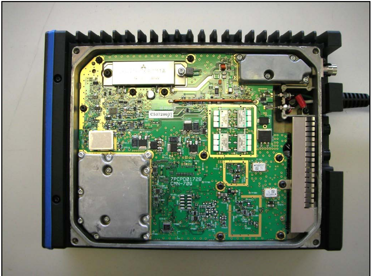
Photograph 13: Bottom Cover and Shield Removed
