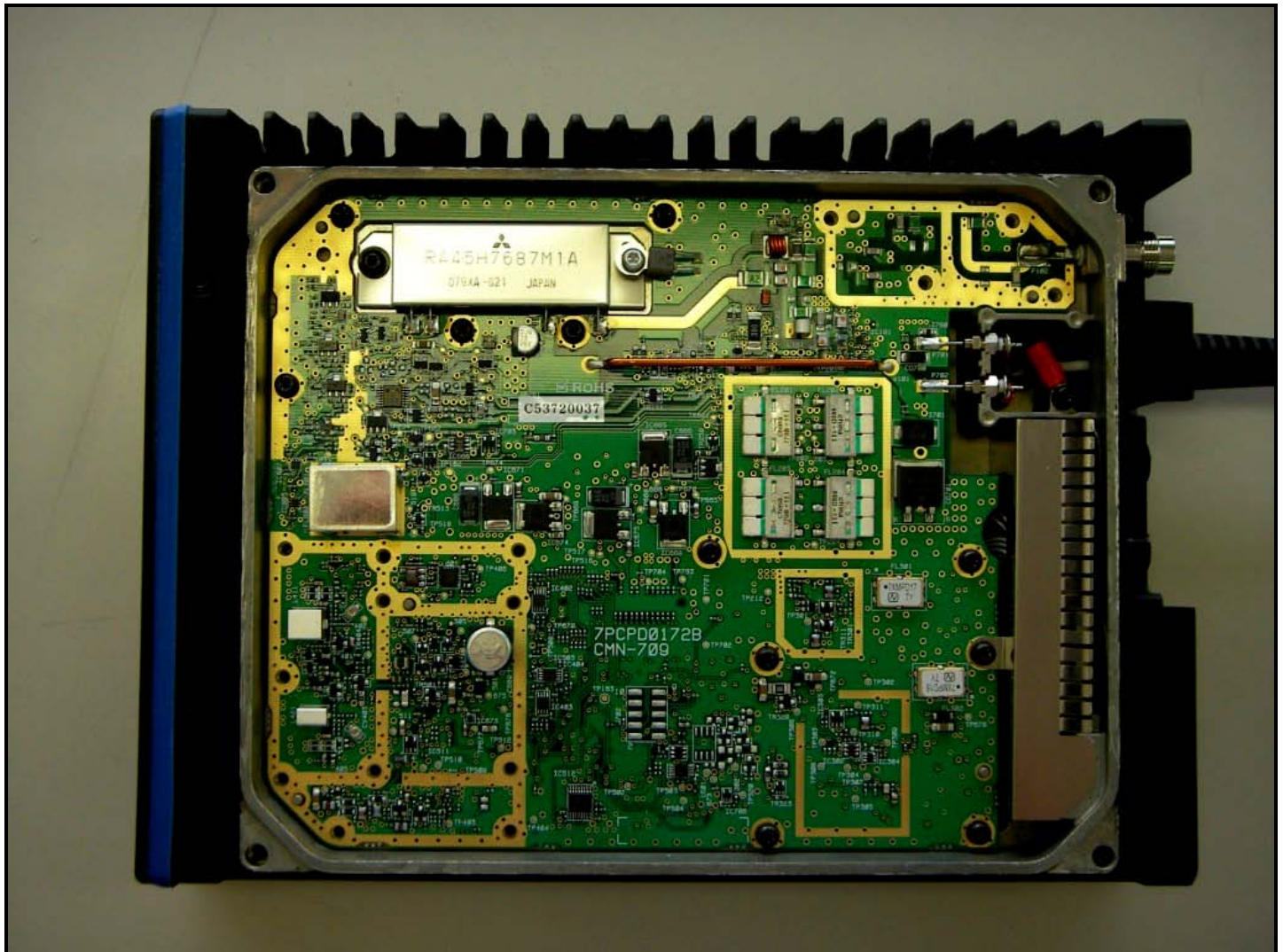
Photograph 14: Bottom Cover and Shields Removed
