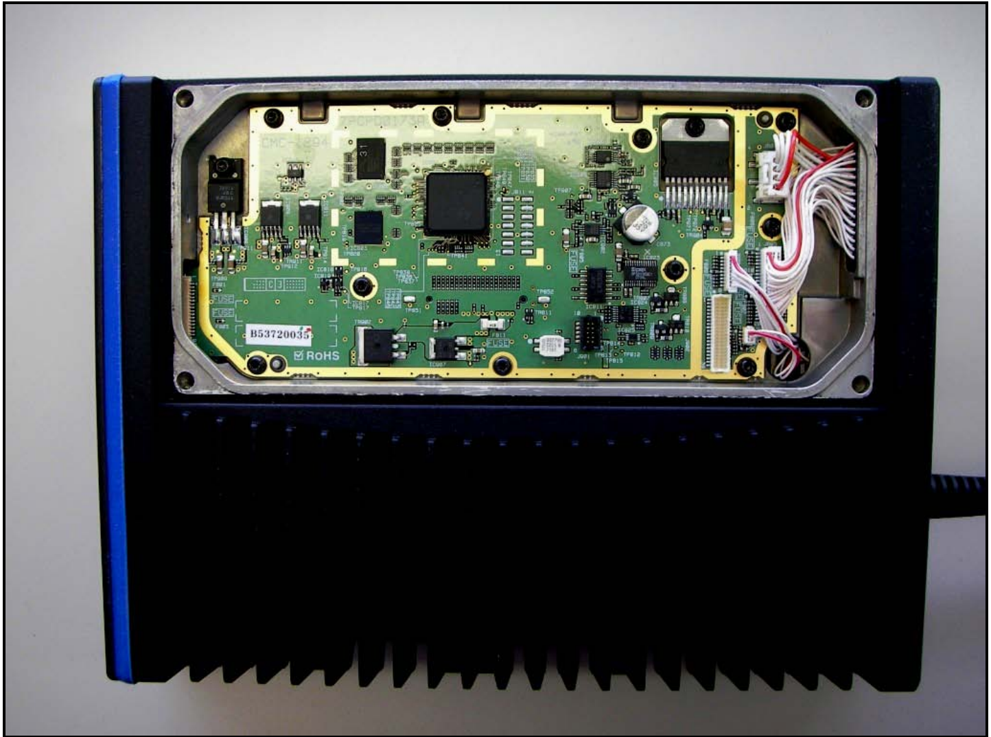
Photograph 11: Top View without Cover
