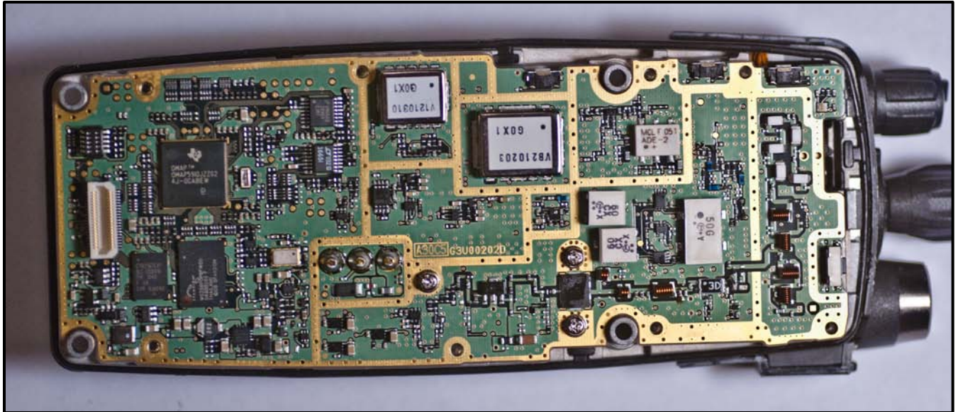
Photograph 5: Main PWB in Unit
