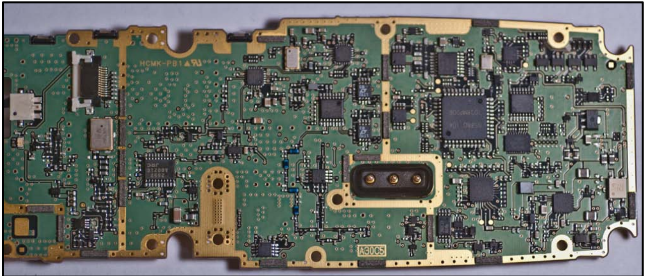
Photograph 6: Main PWB – Side 1
