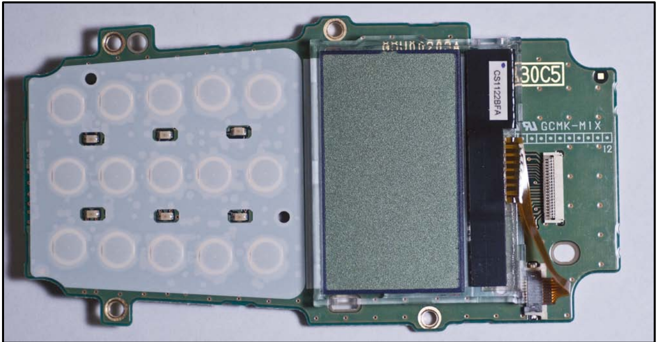
Photograph 10: Interface PWB – LCD Side
