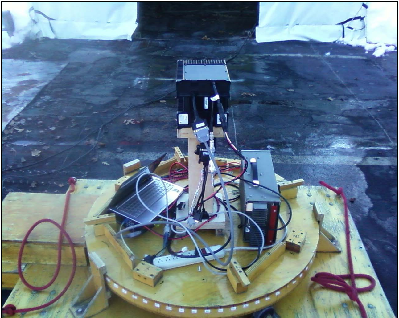
Photograph 35: Radiated Emissions (Rear View)
