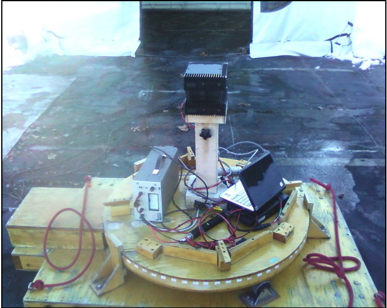
Photograph 34: Radiated Emissions (Front View)
