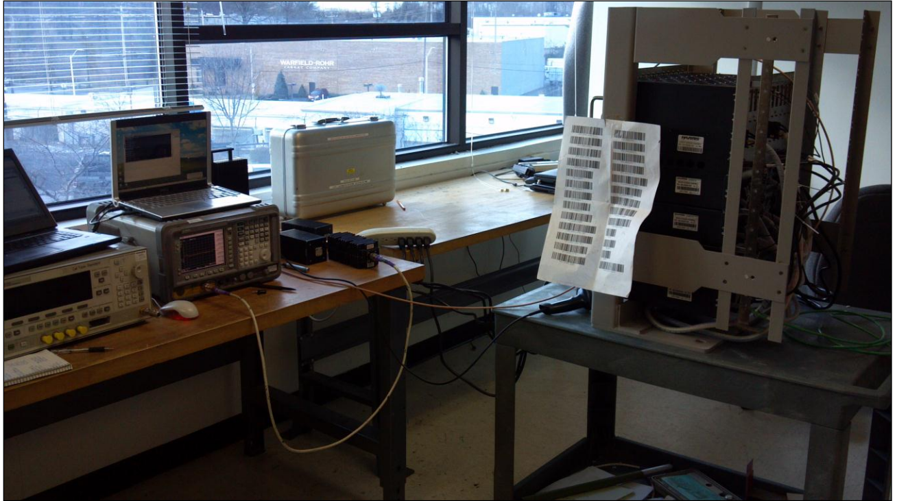
Photograph 3. Conducted Spurious Emissions, Test Setup
