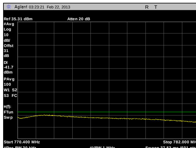
Plot 111. Adjacent Channel Power, Channel 770, 400 kHz – 12 MHz. C4FM, 10 W
