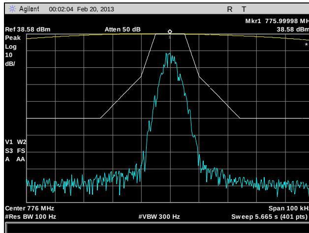
Plot 19. Emission Mask, 776 MHz, C4FM, 10 W
