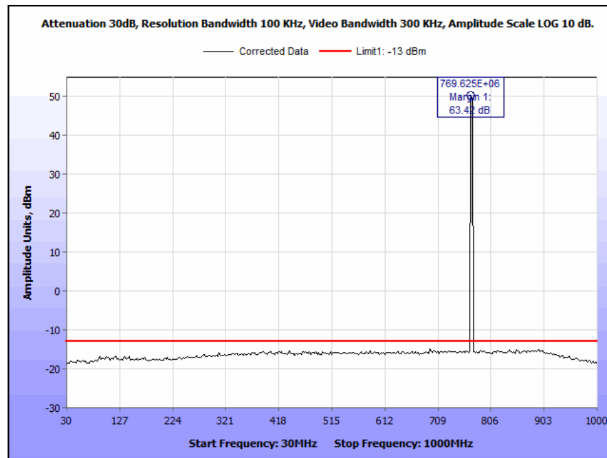
Plot 65. Conducted Spurious Emissions, 770 MHz, HDQPSK, 100 W, 30 MHz – 1 GHz
