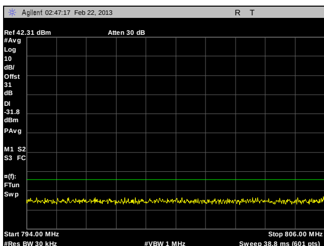
Plot 163. Adjacent Channel Power, Channel 776, Paired Receive Band, CQPSK, 100 W
