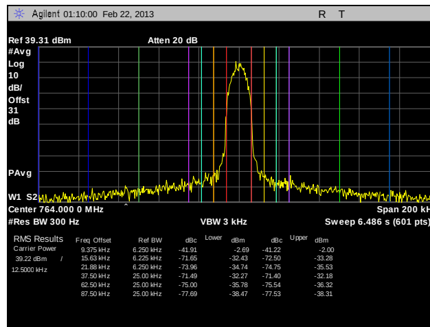
Plot 84. Adjacent Channel Power, Channel 764, CQPSK, 10 W, 1
