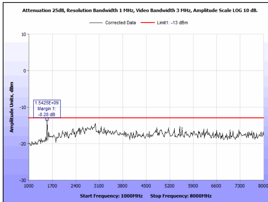
Plot 64. Conducted Spurious Emissions, 770 MHz, CQPSK, 100 W, 1 GHz – 8 GHz
