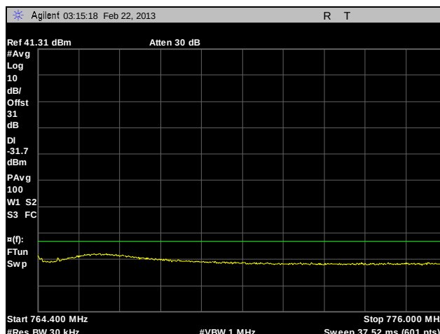
Plot 96. Adjacent Channel Power, Channel 764, 400 kHz – 12 MHz. C4FM, 100 W
