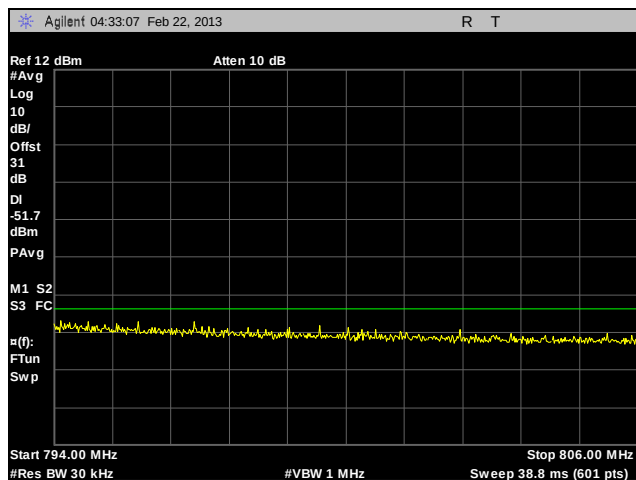
Plot 108. Adjacent Channel Power, Channel 764, Paired Receive Band, HDQPSK, 100 W
