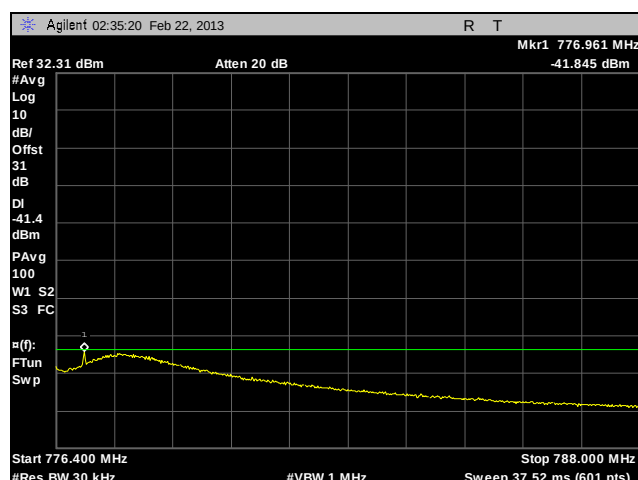
Plot 151. Adjacent Channel Power, Channel 776, 400 kHz – 12 MHz, HDQPSK, 10 W
