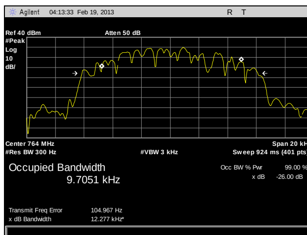
Plot 26. Occupied Bandwidth, 764 MHz, CQPSK, 10 W
