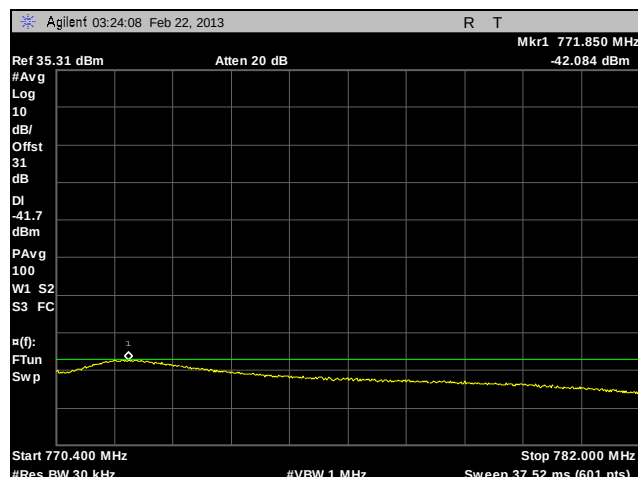
Plot 116. Adjacent Channel Power, Channel 770, 400 kHz – 12 MHz, CQPSK, 10 W
