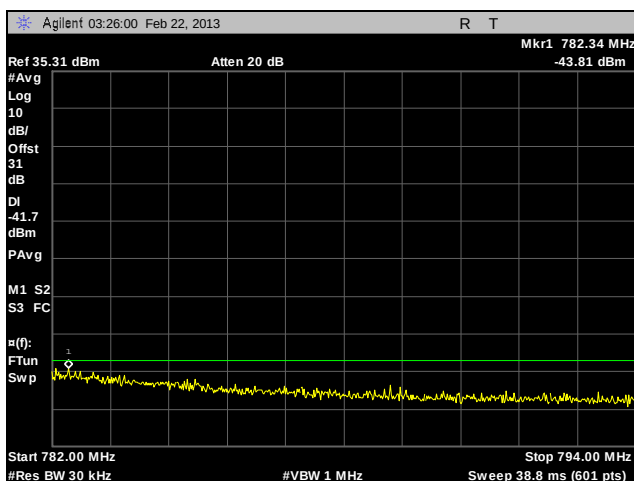
Plot 112. Adjacent Channel Power, Channel 770, 12 MHz – Paired Receive Band, C4FM, 10 W
