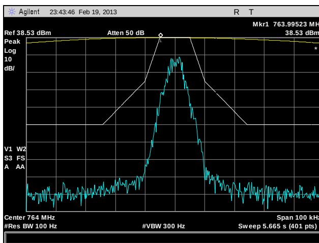
Plot 7. Emission Mask, 764 MHz, C4FM, 10 W
