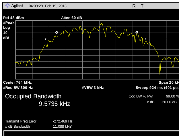
Plot 30. Occupied Bandwidth, 764 MHz, HDQPSK, 100 W
