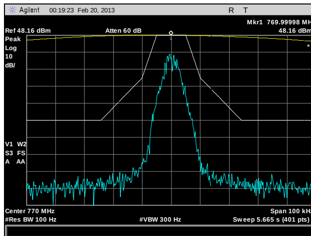
Plot 16. Emission Mask, 770 MHz, C4FM, 100 W
