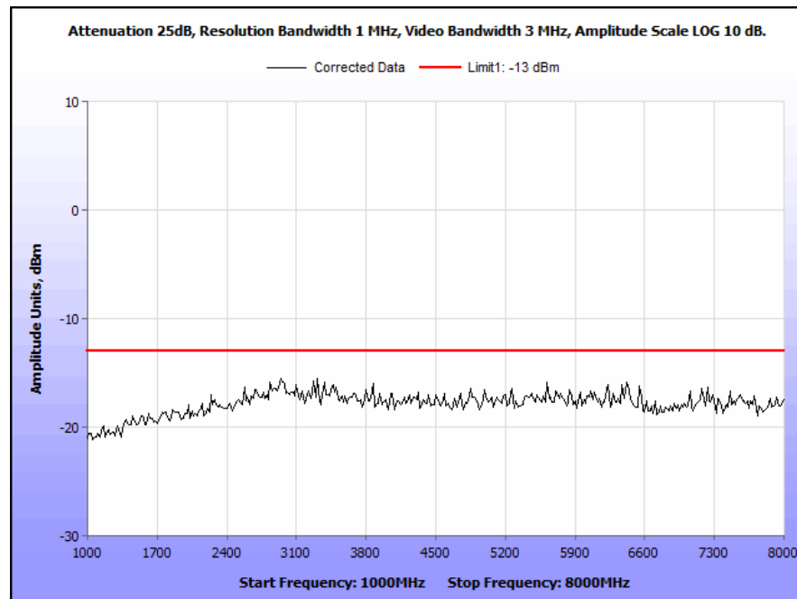
Plot 46. Conducted Spurious Emissions, 764 MHz, CQPSK, 10 W, 1 GHz – 8 GHz
