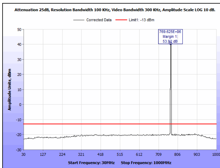
Plot 57. Conducted Spurious Emissions, 770 MHz, CQPSK, 10 W, 30 MHz – 1 GHz
