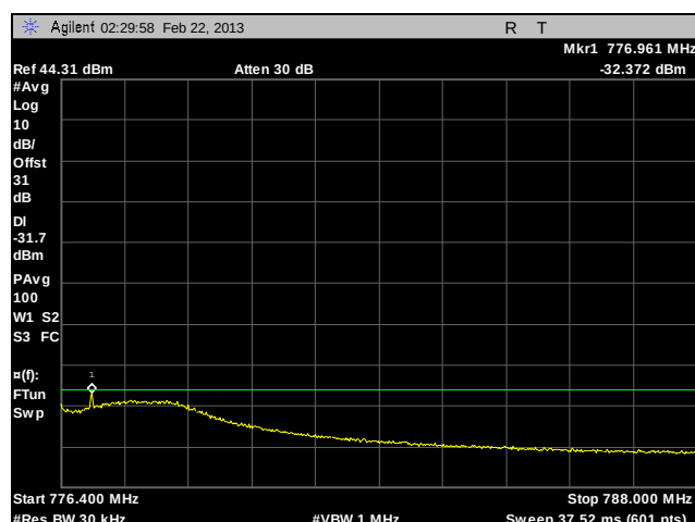
Plot 161. Adjacent Channel Power, Channel 776, 400 kHz – 12 MHz, CQPSK, 100 W
