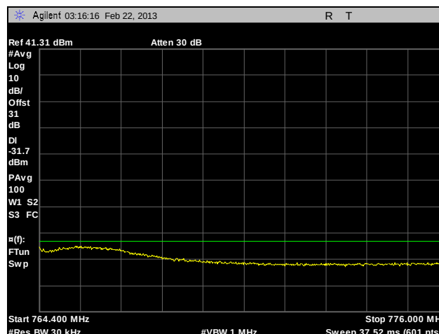
Plot 106. Adjacent Channel Power, Channel 764, 400 kHz – 12 MHz, HDQPSK, 100 W
