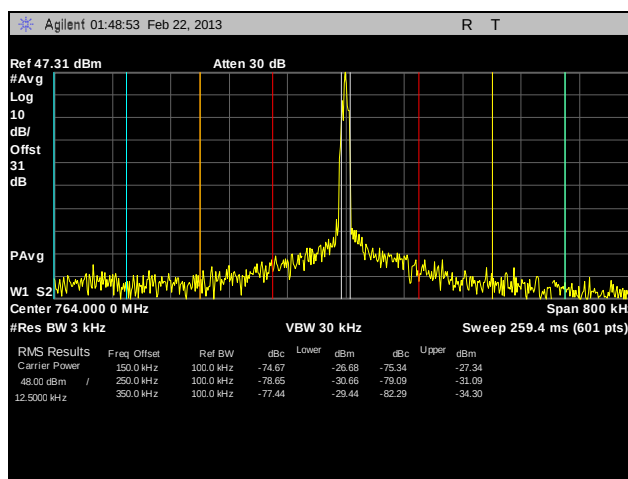
Plot 95. Adjacent Channel Power, Channel 764, C4FM, 100 W, 2
