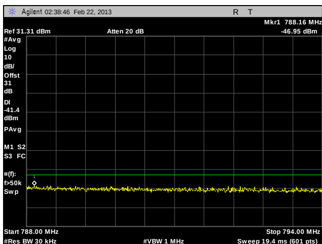
Plot 142. Adjacent Channel Power, Channel 776, 12 MHz – Paired Receive Band, C4FM, 10 W
