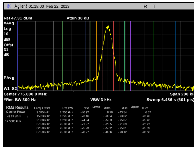
Plot 154. Adjacent Channel Power, Channel 776, C4FM, 100 W, 1
