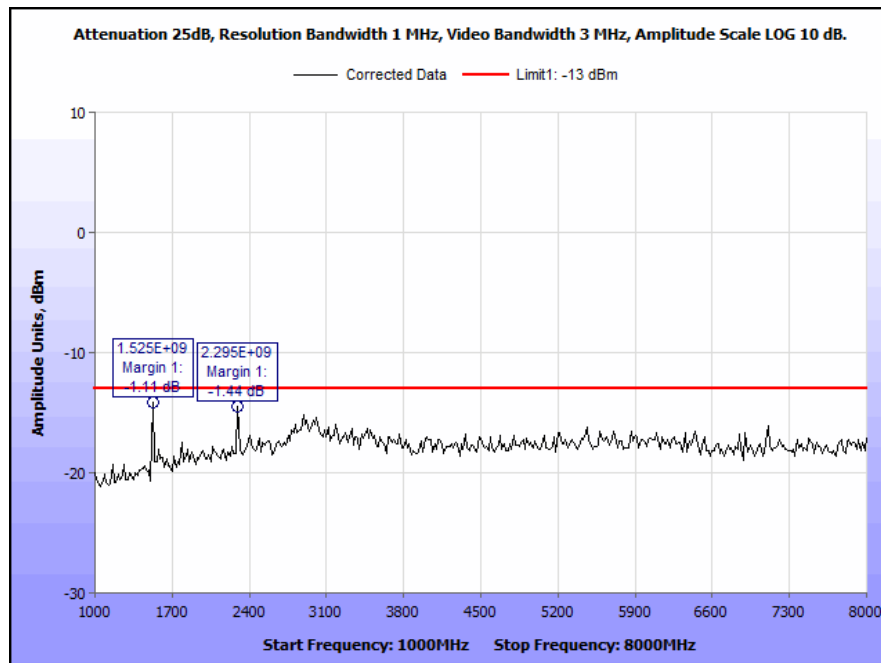
Plot 54. Conducted Spurious Emissions, 764 MHz, HDQPSK, 100 W, 1 GHz – 8 GHz
