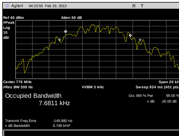
Plot 37. Occupied Bandwidth, 776 MHz, C4FM, 10 W
