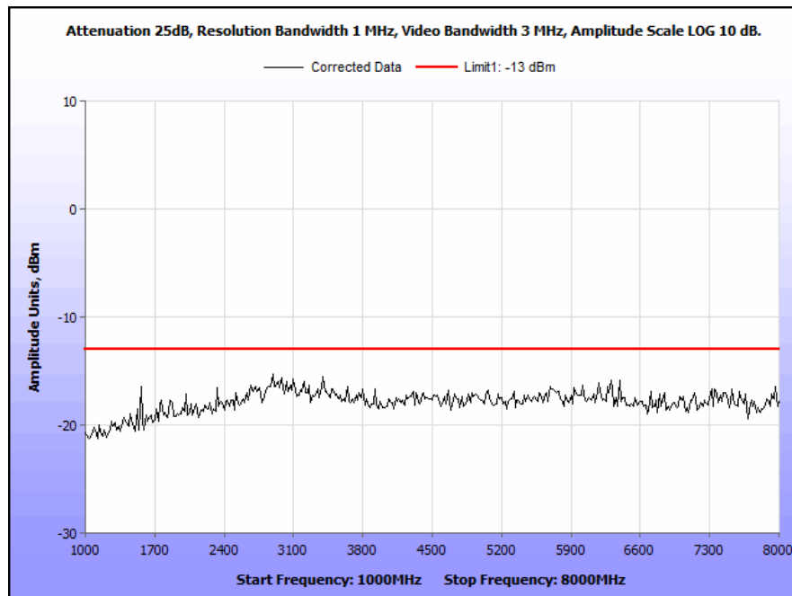
Plot 74. Conducted Spurious Emissions, 776 MHz, C4FM, 100 W, 1 GHz – 8 GHz
