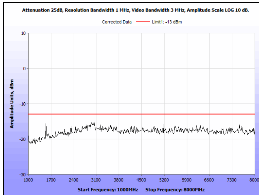
Plot 62. Conducted Spurious Emissions, 770 MHz, C4FM, 100 W, 1 GHz – 8 GHz
