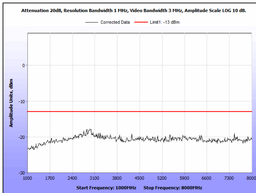
Plot 58. Conducted Spurious Emissions, 770 MHz, CQPSK, 10 W, 1 GHz – 8 GHz
