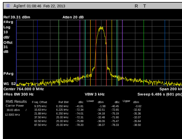
Plot 89. Adjacent Channel Power, Channel 764, HDQPSK, 10 W, 1
