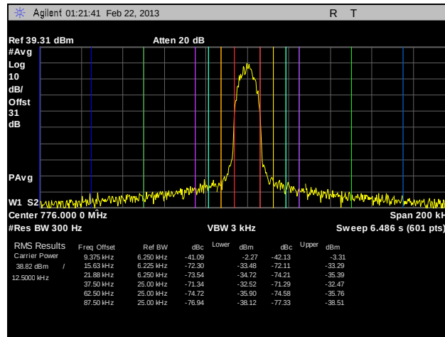
Plot 144. Adjacent Channel Power, Channel 776, CQPSK, 10 W, 1
