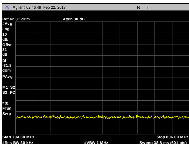
Plot 158. Adjacent Channel Power, Channel 776, Paired Receive Band, C4FM, 100 W
