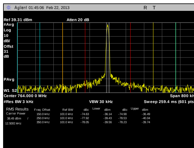
Plot 90. Adjacent Channel Power, Channel 764, HDQPSK, 10 W, 2
