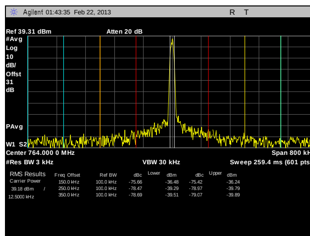
Plot 85. Adjacent Channel Power, Channel 764, CQPSK, 10 W, 2
