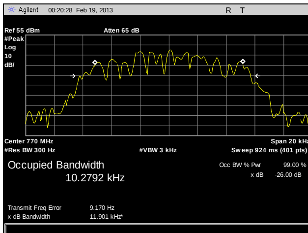
Plot 36. Occupied Bandwidth, 770 MHz, HDQPSK, 100 W
