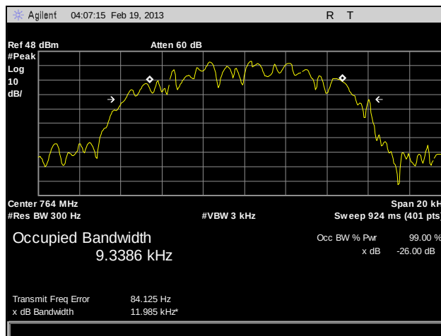
Plot 29. Occupied Bandwidth, 764 MHz, CQPSK, 100 W
