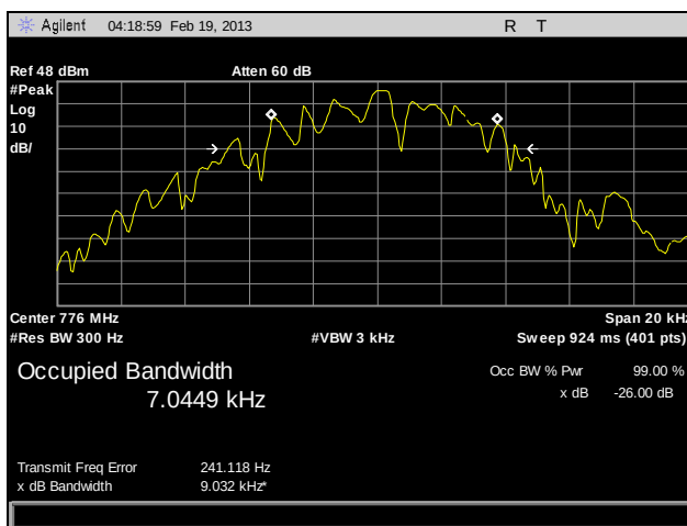
Plot 40. Occupied Bandwidth, 776 MHz, C4FM, 100 W
