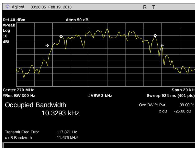
Plot 33. Occupied Bandwidth, 770 MHz, HDQPSK, 10 W
