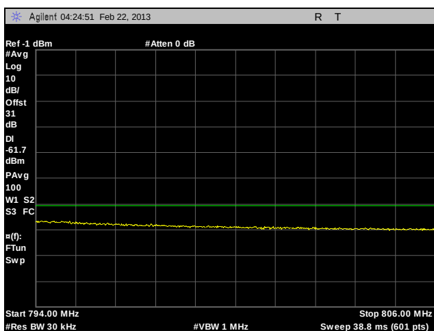
Plot 113. Adjacent Channel Power, Channel 770, Paired Receive Band, C4FM, 10 W
