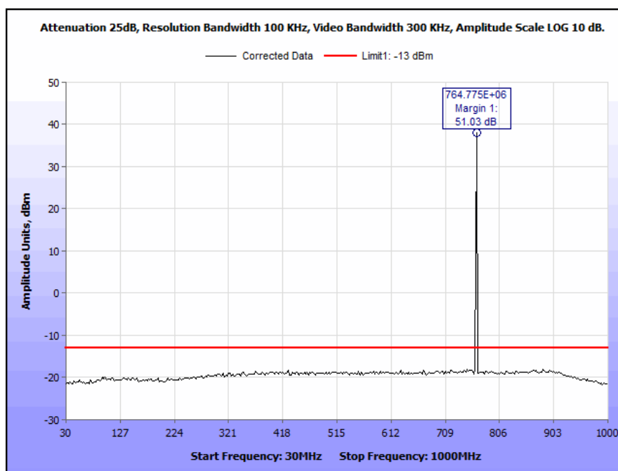
Plot 43. Conducted Spurious Emissions, 764 MHz, C4FM, 10 W, 30 MHz – 1 GHz
