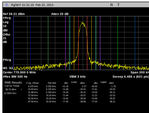
Plot 114. Adjacent Channel Power, Channel 770, CQPSK, 10 W, 1
