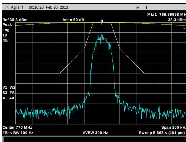
Plot 14. Emission Mask, 770 MHz, CQPSK, 10 W
