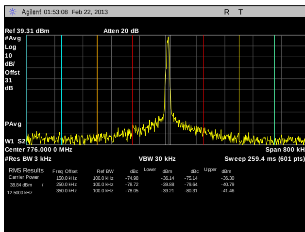
Plot 140. Adjacent Channel Power, Channel 776, C4FM, 10 W, 2
