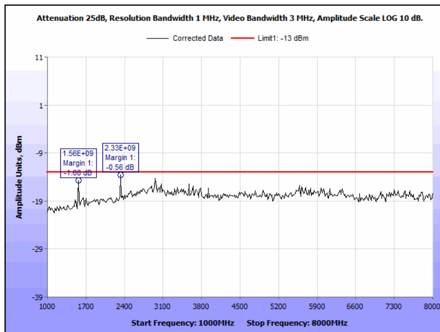
Plot 78. Conducted Spurious Emissions, 776 MHz, HDQPSK, 100 W, 1 GHz – 8 GHz
