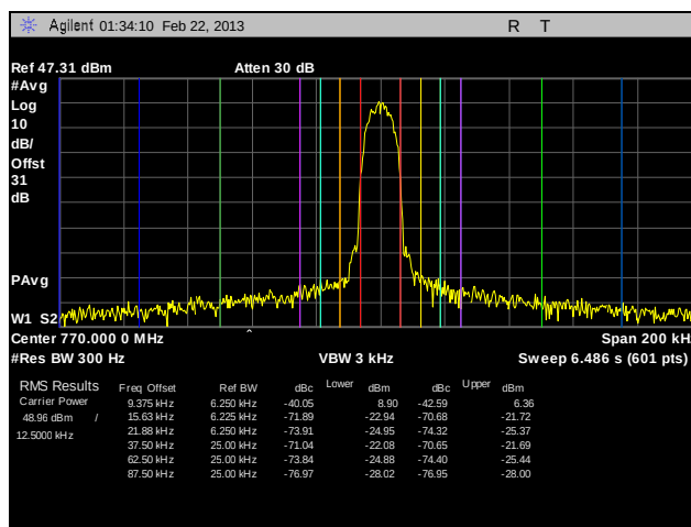
Plot 129. Adjacent Channel Power, Channel 770, CQPSK, 100 W, 1
