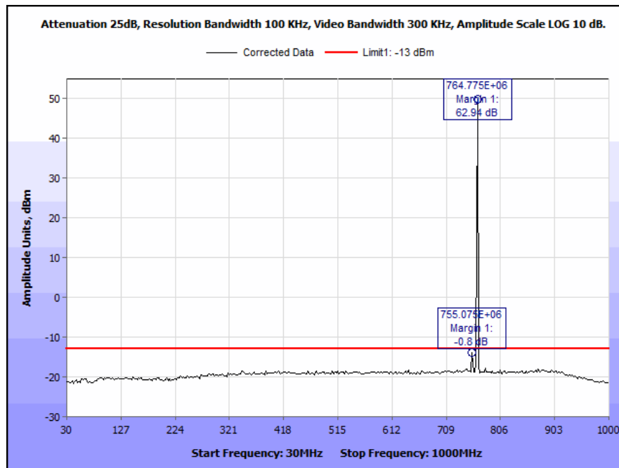
Plot 53. Conducted Spurious Emissions, 764 MHz, HDQPSK, 100 W, 30 MHz – 1 GHz
