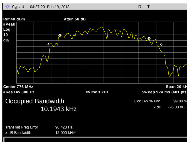
Plot 39. Occupied Bandwidth, 776 MHz, HDQPSK, 10 W
