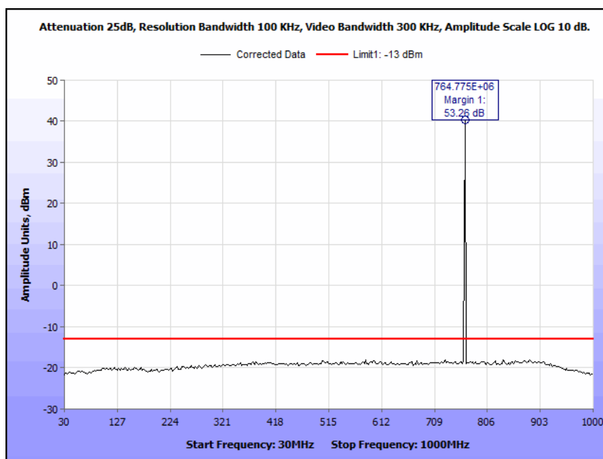
Plot 47. Conducted Spurious Emissions, 764 MHz, HDQPSK, 10 W, 30 MHz – 1 GHz
