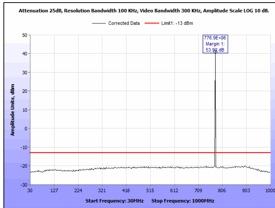
Plot 69. Conducted Spurious Emissions, 776 MHz, CQPSK, 10 W, 30 MHz – 1 GHz
