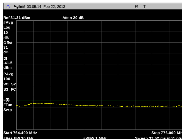
Plot 81. Adjacent Channel Power, Channel 764, 400 kHz – 12 MHz. C4FM, 10 W
