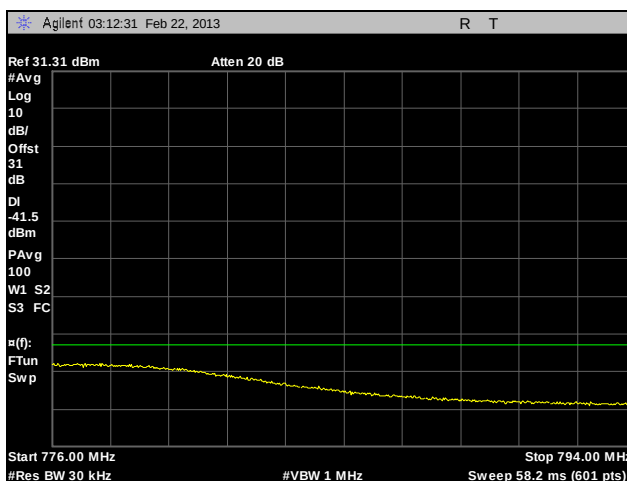
Plot 92. Adjacent Channel Power, Channel 764, 12 MHz – Paired Receive Band, HDQPSK, 10 W
