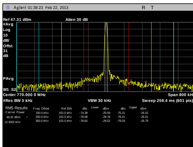
Plot 130. Adjacent Channel Power, Channel 770, CQPSK, 100 W, 2
