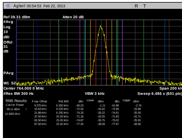
Plot 79. Adjacent Channel Power, Channel 764, C4FM, 10 W, 1
