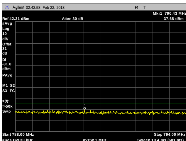
Plot 157. Adjacent Channel Power, Channel 776, 12 MHz – Paired Receive Band, C4FM, 100 W
