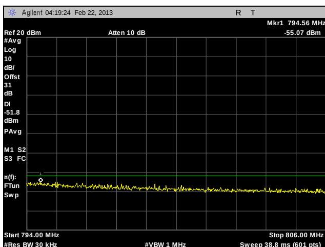
Plot 133. Adjacent Channel Power, Channel 770, Paired Receive Band, CQPSK, 100 W
