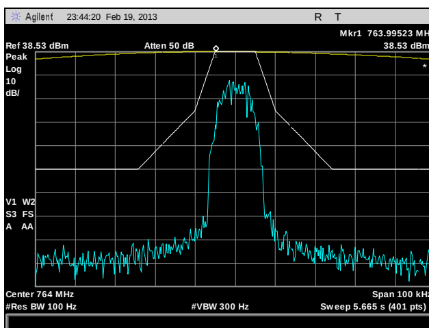
Plot 8. Emission Mask, 764 MHz, CQPSK, 10 W
