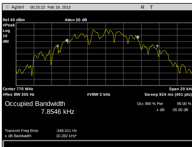
Plot 31. Occupied Bandwidth, 770 MHz, C4FM, 10 W
