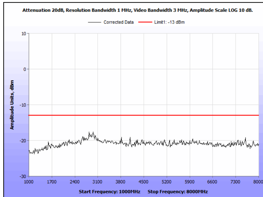
Plot 56. Conducted Spurious Emissions, 770 MHz, C4FM, 10 W, 1 GHz – 8 GHz
