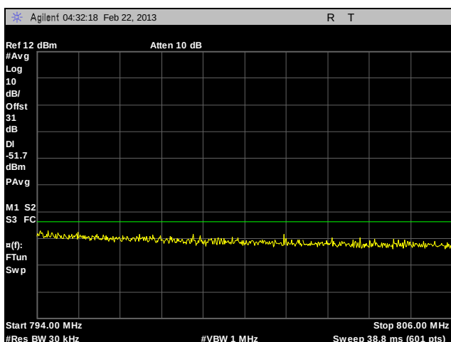
Plot 103. Adjacent Channel Power, Channel 764, Paired Receive Band, CQPSK, 100 W
