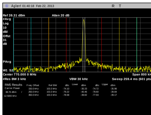
Plot 115. Adjacent Channel Power, Channel 770, CQPSK, 10 W, 2
