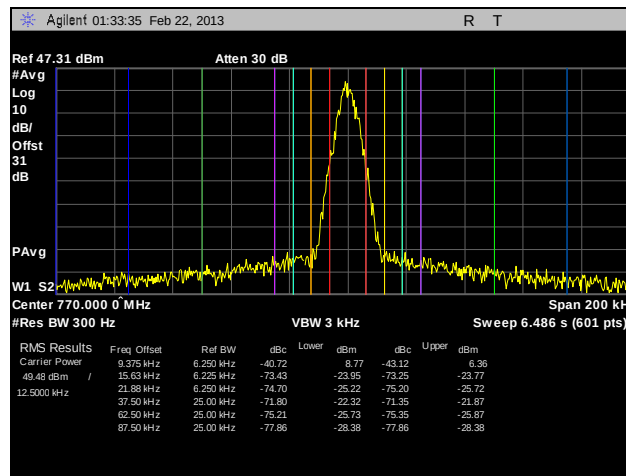
Plot 124. Adjacent Channel Power, Channel 770, C4FM, 100 W, 1
