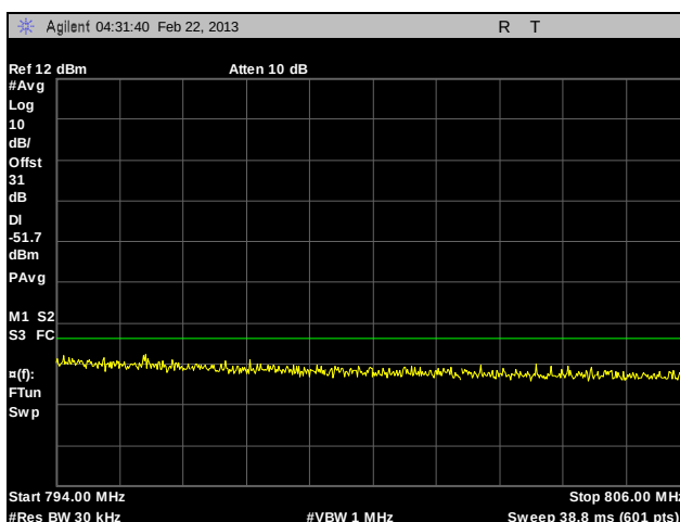
Plot 98. Adjacent Channel Power, Channel 764, Paired Receive Band, C4FM, 100 W
