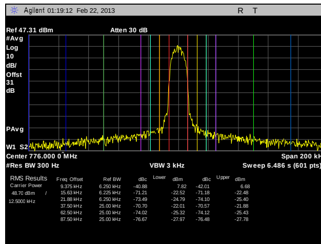
Plot 159. Adjacent Channel Power, Channel 776, CQPSK, 100 W, 1
