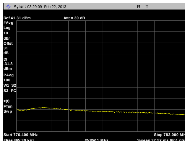
Plot 126. Adjacent Channel Power, Channel 770, 400 kHz – 12 MHz. C4FM, 100 W
