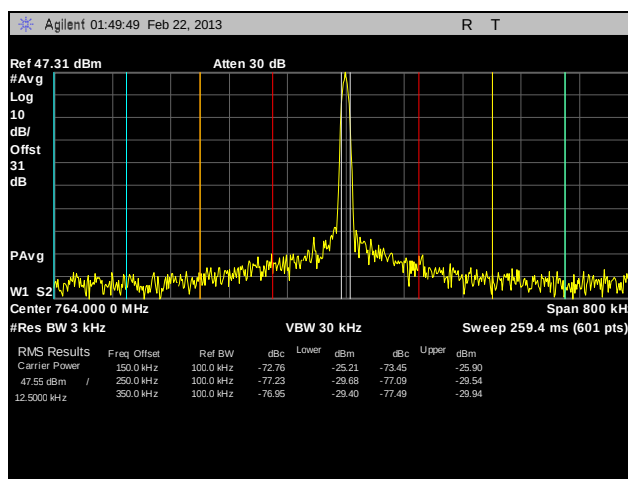
Plot 100. Adjacent Channel Power, Channel 764, CQPSK, 100 W, 2
