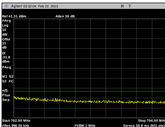
Plot 132. Adjacent Channel Power, Channel 770, 12 MHz – Paired Receive Band, CQPSK, 100 W
