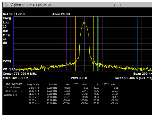
Plot 149. Adjacent Channel Power, Channel 776, HDQPSK, 10 W, 1
