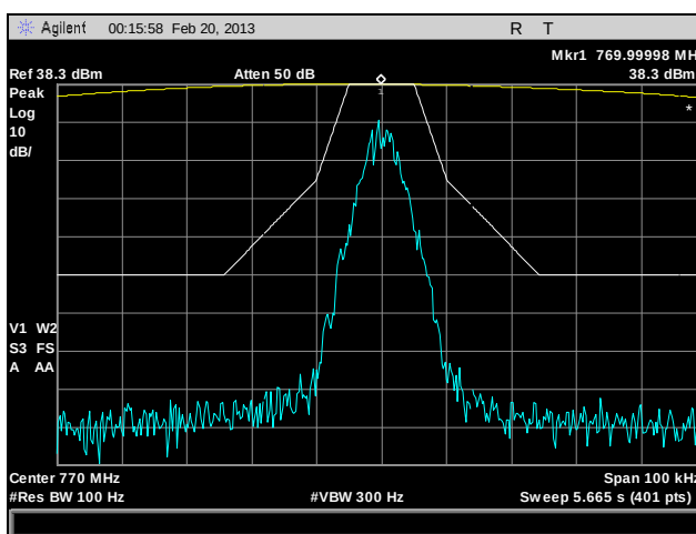
Plot 13. Emission Mask, 770 MHz, C4FM, 10 W
