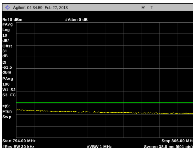
Plot 83. Adjacent Channel Power, Channel 764, Paired Receive Band, C4FM, 10 W
