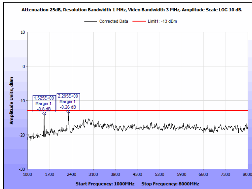
Plot 52. Conducted Spurious Emissions, 764 MHz, CQPSK, 100 W, 1 GHz – 8 GHz
