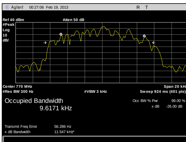
Plot 32. Occupied Bandwidth, 770 MHz, CQPSK, 10 W
