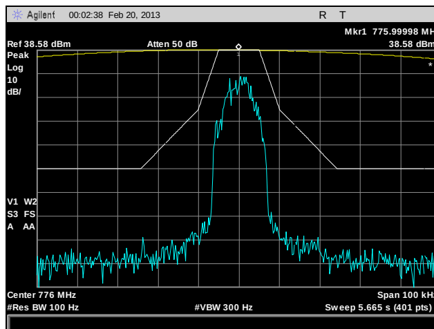
Plot 20. Emission Mask, 776 MHz, CQPSK, 10 W
