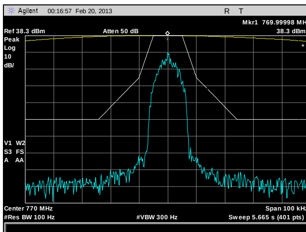
Plot 15. Emission Mask, 770 MHz, HDQPSK, 10 W
