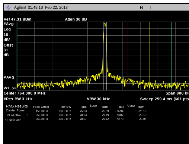
Plot 105. Adjacent Channel Power, Channel 764, HDQPSK, 100 W, 2
