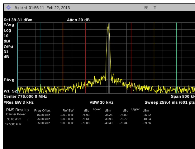
Plot 150. Adjacent Channel Power, Channel 776, HDQPSK, 10 W, 2
