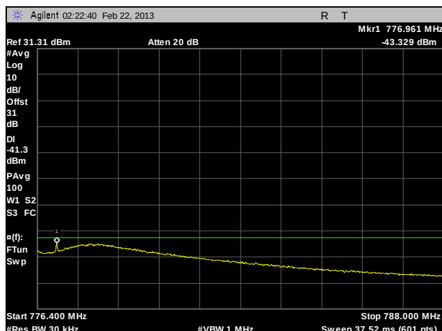
Plot 141. Adjacent Channel Power, Channel 776, 400 kHz – 12 MHz. C4FM, 10 W
