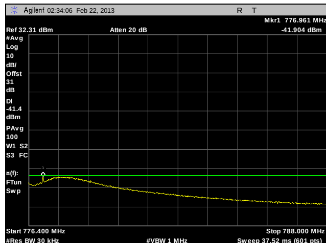
Plot 146. Adjacent Channel Power, Channel 776, 400 kHz – 12 MHz, CQPSK, 10 W
