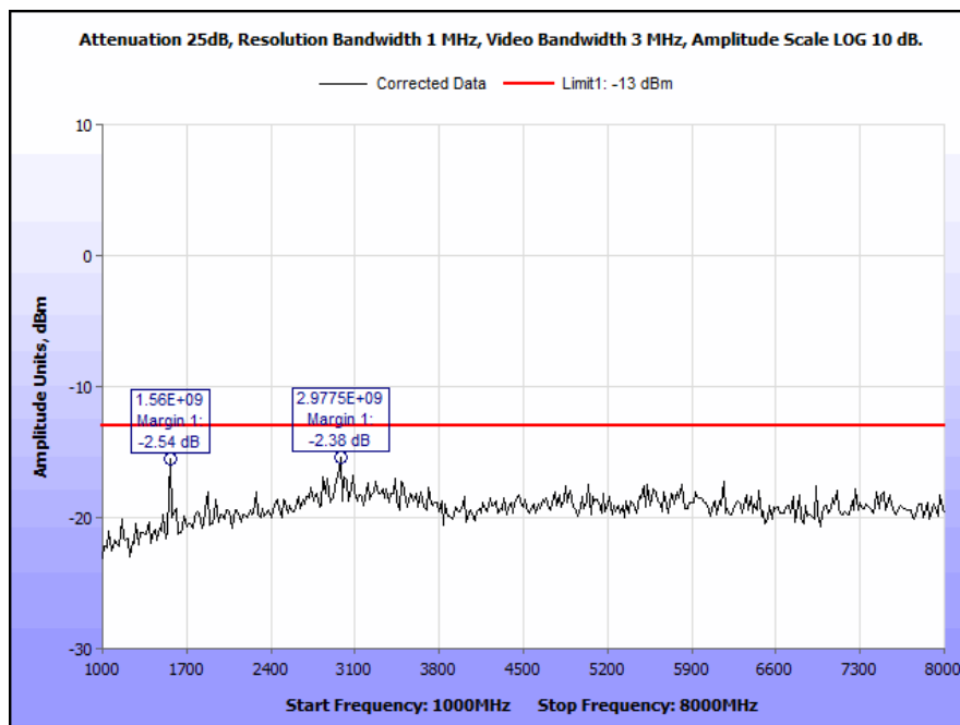
Plot 76. Conducted Spurious Emissions, 776 MHz, CQPSK, 100 W, 1 GHz – 8 GHz
