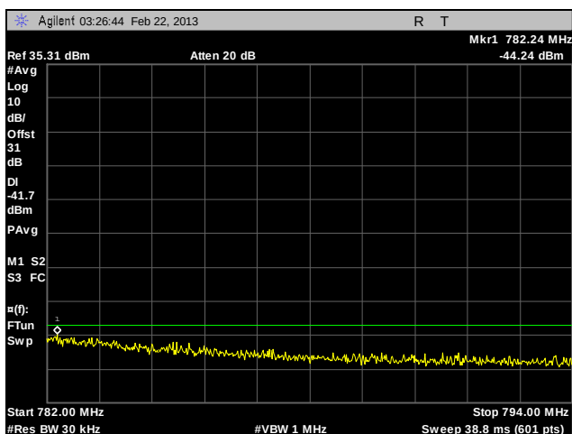
Plot 117. Adjacent Channel Power, Channel 770, 12 MHz – Paired Receive Band, CQPSK, 10 W
