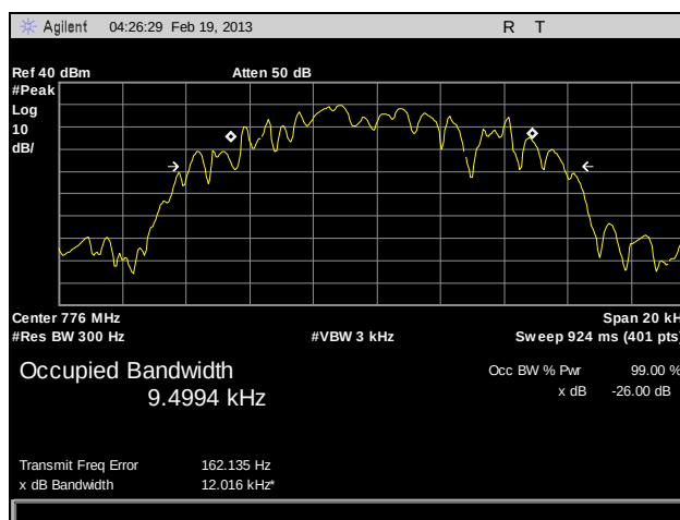
Plot 38. Occupied Bandwidth, 776 MHz, CQPSK, 10 W
