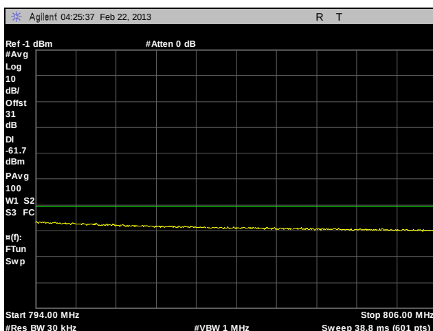
Plot 118. Adjacent Channel Power, Channel 770, Paired Receive Band, CQPSK, 10 W
