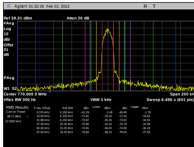
Plot 119. Adjacent Channel Power, Channel 770, HDQPSK, 10 W, 1
