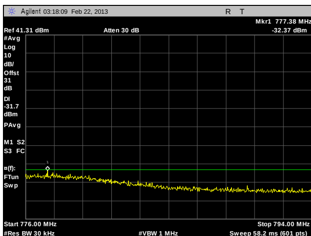
Plot 102. Adjacent Channel Power, Channel 764, 12 MHz – Paired Receive Band, CQPSK, 100 W
