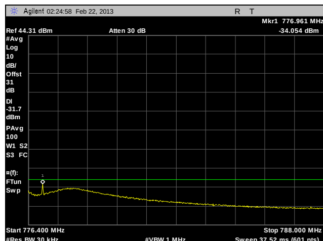
Plot 156. Adjacent Channel Power, Channel 776, 400 kHz – 12 MHz. C4FM, 100 W
