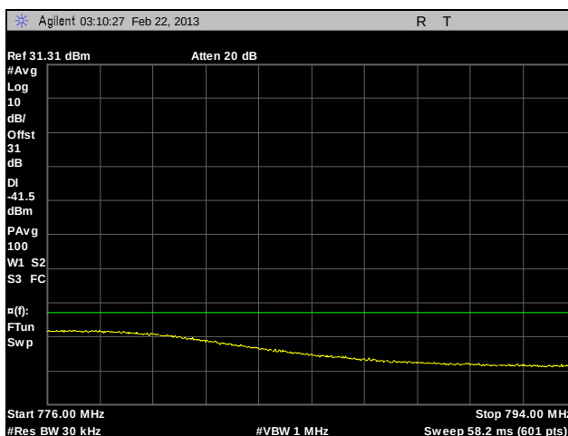
Plot 82. Adjacent Channel Power, Channel 764, 12 MHz – Paired Receive Band, C4FM, 10 W
