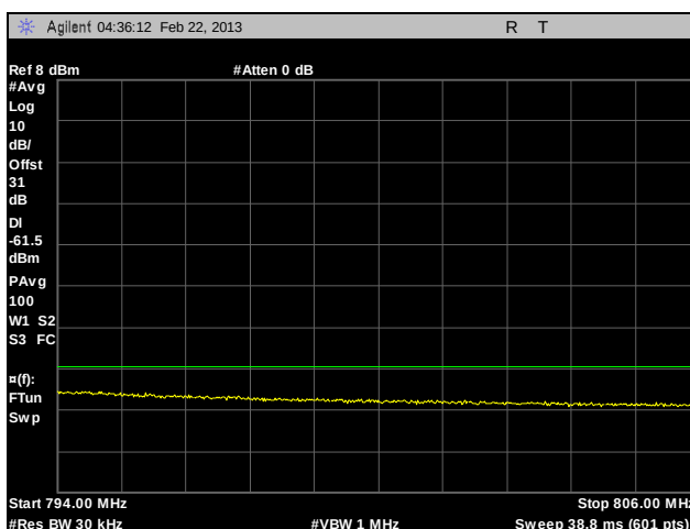
Plot 93. Adjacent Channel Power, Channel 764, Paired Receive Band, HDQPSK, 10 W
