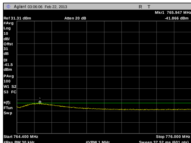
Plot 86. Adjacent Channel Power, Channel 764, 400 kHz – 12 MHz, CQPSK, 10 W
