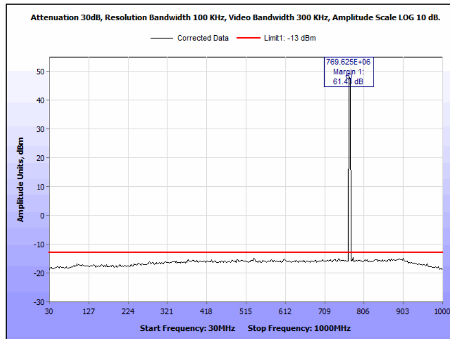
Plot 61. Conducted Spurious Emissions, 770 MHz, C4FM, 100 W, 30 MHz – 1 GHz
