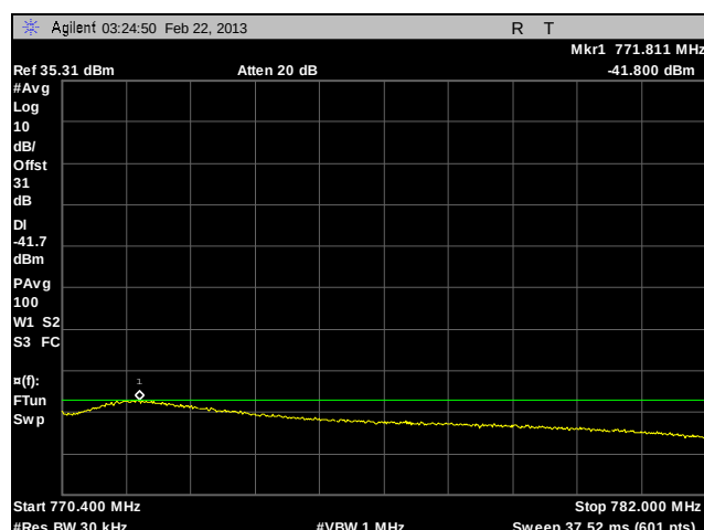
Plot 121. Adjacent Channel Power, Channel 770, 400 kHz – 12 MHz, HDQPSK, 10 W
