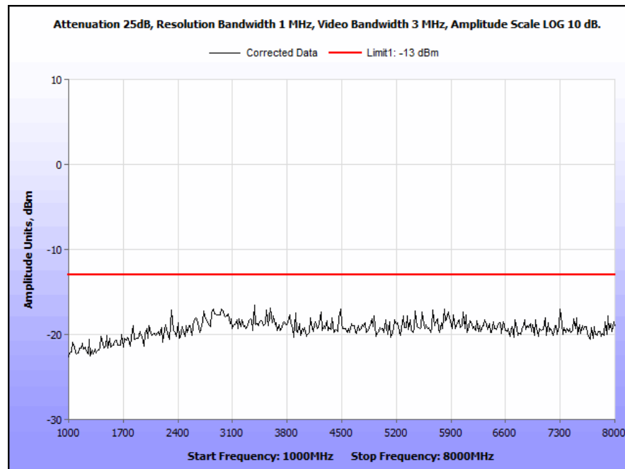
Plot 66. Conducted Spurious Emissions, 770 MHz, HDQPSK, 100 W, 1 GHz – 8 GHz
