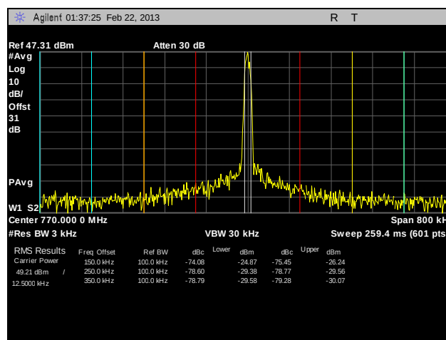
Plot 125. Adjacent Channel Power, Channel 770, C4FM, 100 W, 2
