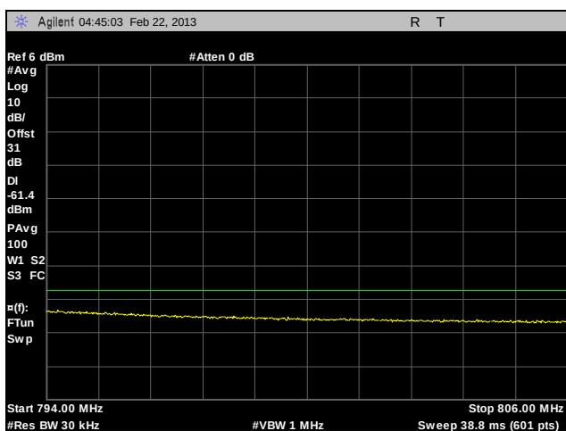
Plot 148. Adjacent Channel Power, Channel 776, Paired Receive Band, CQPSK, 10 W
