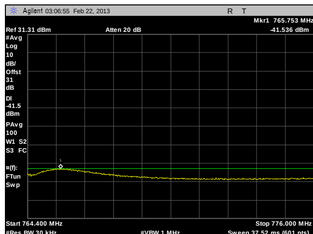
Plot 91. Adjacent Channel Power, Channel 764, 400 kHz – 12 MHz, HDQPSK, 10 W
