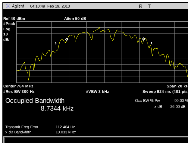
Plot 25. Occupied Bandwidth, 764 MHz, C4FM, 10 W
