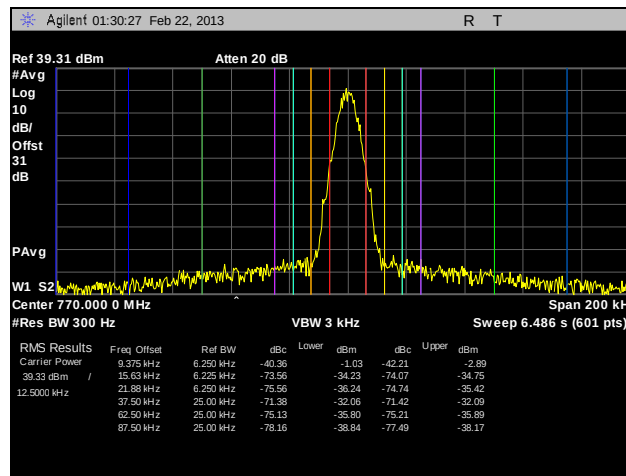
Plot 109. Adjacent Channel Power, Channel 770, C4FM, 10 W, 1
