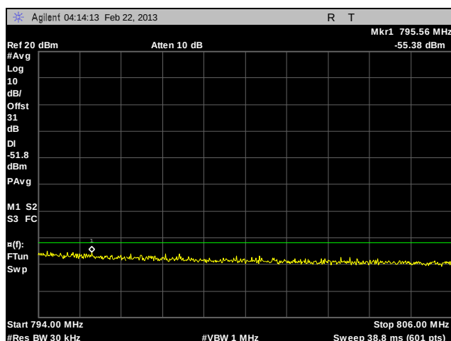
Plot 128. Adjacent Channel Power, Channel 770, Paired Receive Band, C4FM, 100 W
