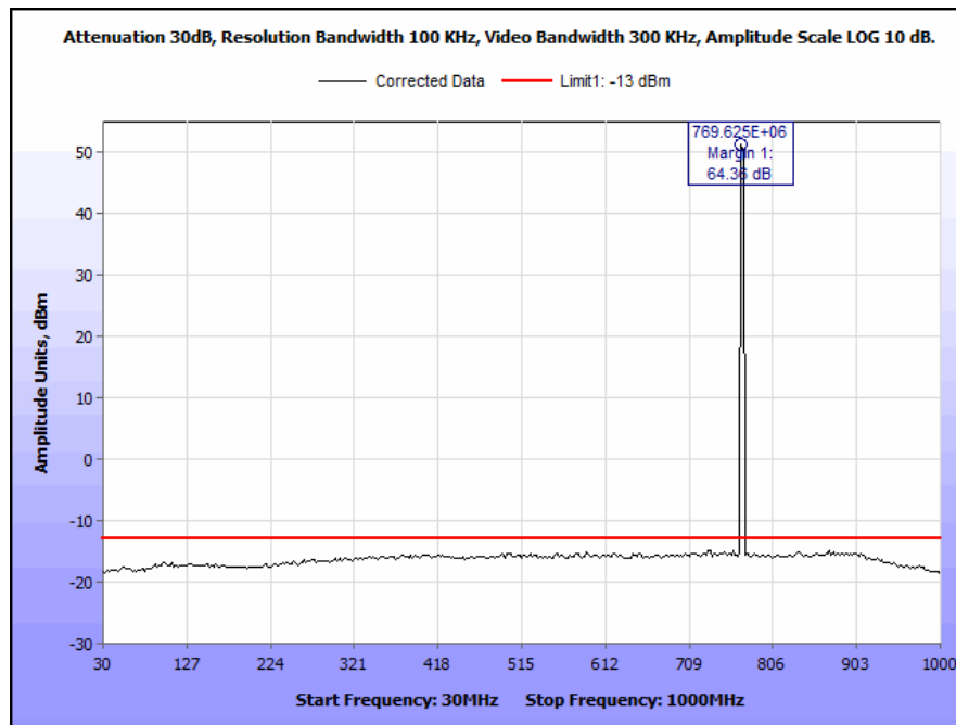
Plot 63. Conducted Spurious Emissions, 770 MHz, CQPSK, 100 W, 30 MHz – 1 GHz
