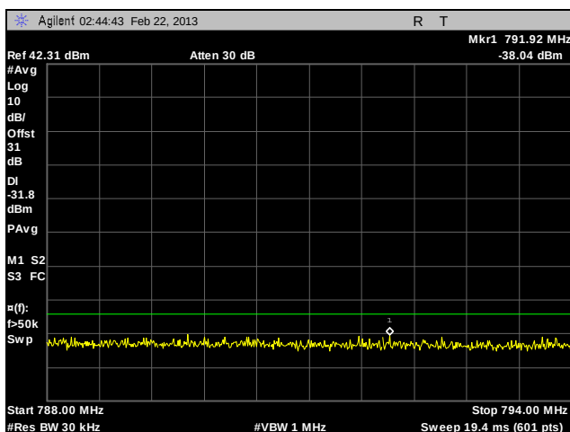
Plot 167. Adjacent Channel Power, Channel 776, 12 MHz – Paired Receive Band, HDQPSK, 100 W
