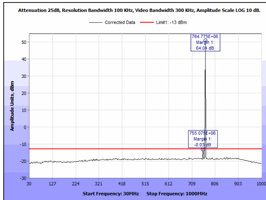
Plot 51. Conducted Spurious Emissions, 764 MHz, CQPSK, 100 W, 30 MHz – 1 GHz
