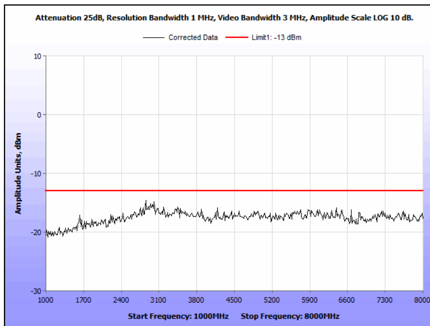
Plot 44. Conducted Spurious Emissions, 764 MHz, C4FM, 10 W, 1 GHz – 8 GHz
