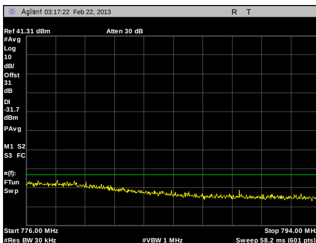
Plot 97. Adjacent Channel Power, Channel 764, 12 MHz – Paired Receive Band, C4FM, 100 W
