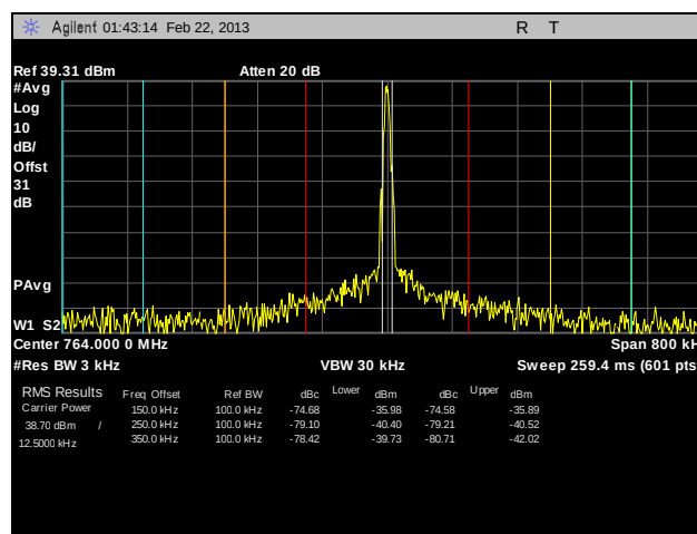
Plot 80. Adjacent Channel Power, Channel 764, C4FM, 10 W, 2
