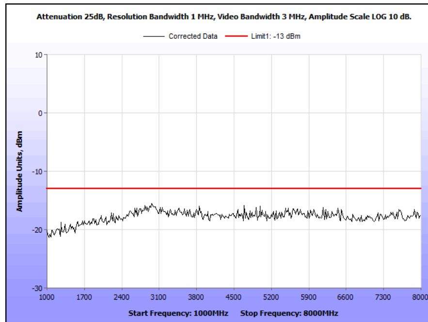
Plot 68. Conducted Spurious Emissions, 776 MHz, C4FM, 10 W, 1 GHz – 8 GHz
