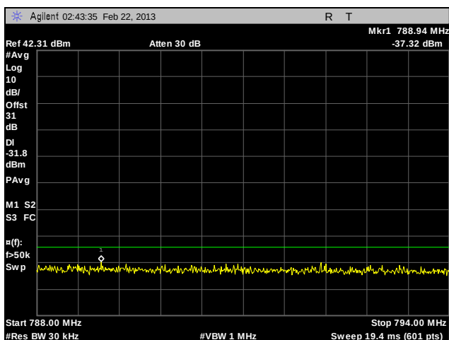
Plot 162. Adjacent Channel Power, Channel 776, 12 MHz – Paired Receive Band, CQPSK, 100 W
