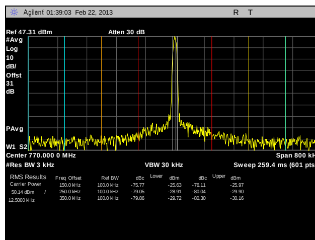
Plot 135. Adjacent Channel Power, Channel 770, HDQPSK, 100 W, 2
