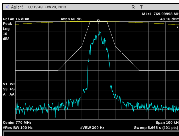
Plot 17. Emission Mask, 770 MHz, CQPSK, 100 W
