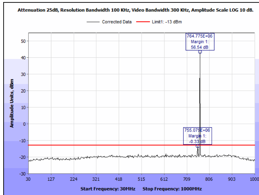
Plot 49. Conducted Spurious Emissions, 764 MHz, C4FM, 100 W, 30 MHz – 1 GHz
