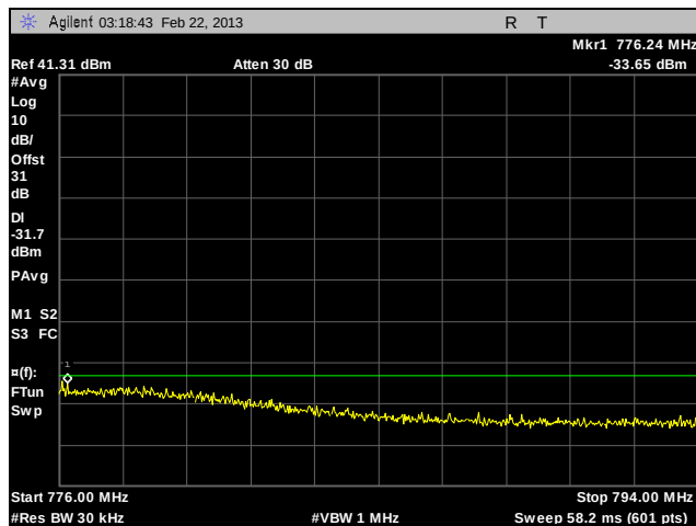
Plot 107. Adjacent Channel Power, Channel 764, 12 MHz – Paired Receive Band, HDQPSK, 100 W
