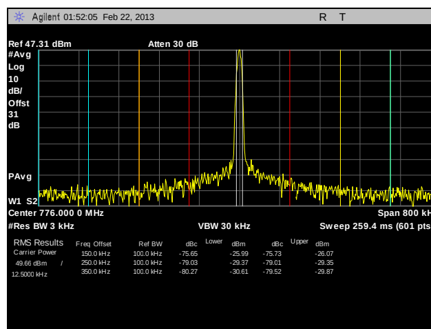
Plot 160. Adjacent Channel Power, Channel 776, CQPSK, 100 W, 2
