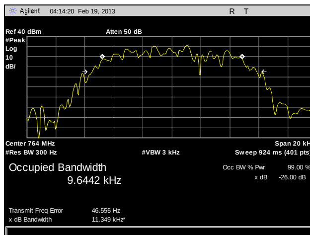
Plot 27. Occupied Bandwidth, 764 MHz, HDQPSK, 10 W
