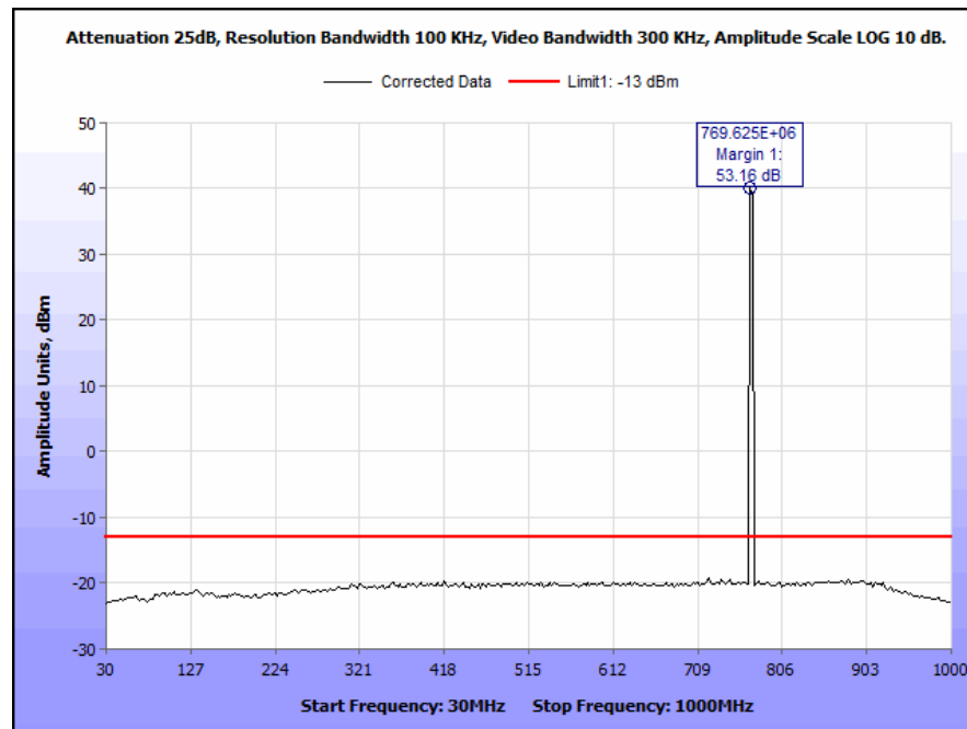
Plot 59. Conducted Spurious Emissions, 770 MHz, HDQPSK, 10 W, 30 MHz – 1 GHz
