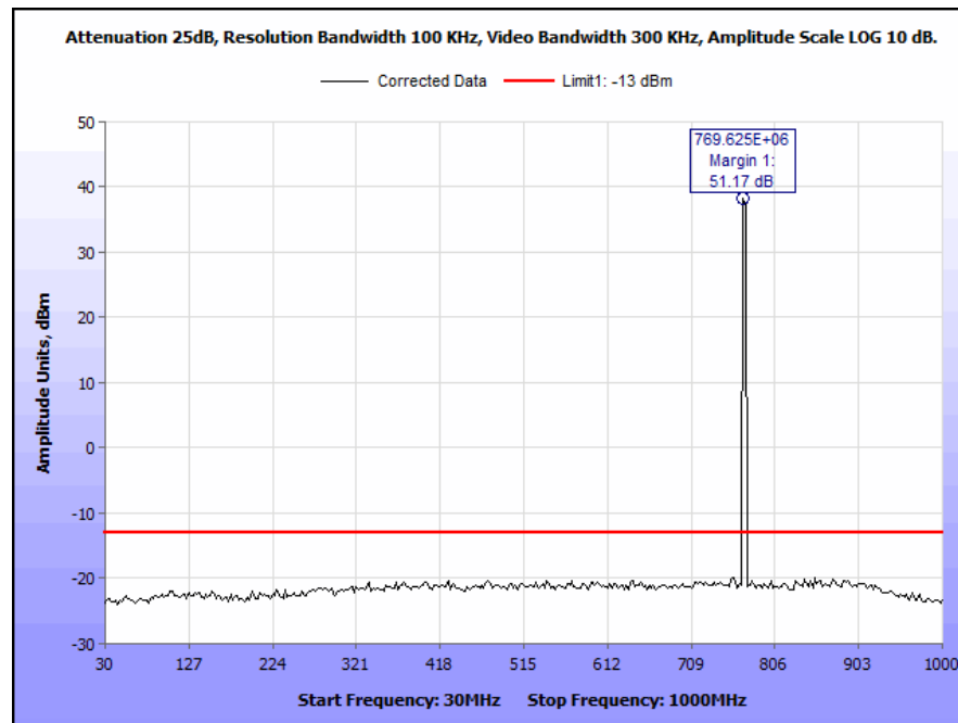
Plot 55. Conducted Spurious Emissions, 770 MHz, C4FM, 10 W, 30 MHz – 1 GHz
