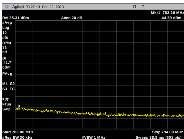
Plot 122. Adjacent Channel Power, Channel 770, 12 MHz – Paired Receive Band, HDQPSK, 10 W
