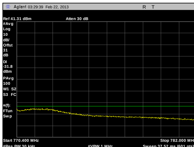
Plot 131. Adjacent Channel Power, Channel 770, 400 kHz – 12 MHz, CQPSK, 100 W
