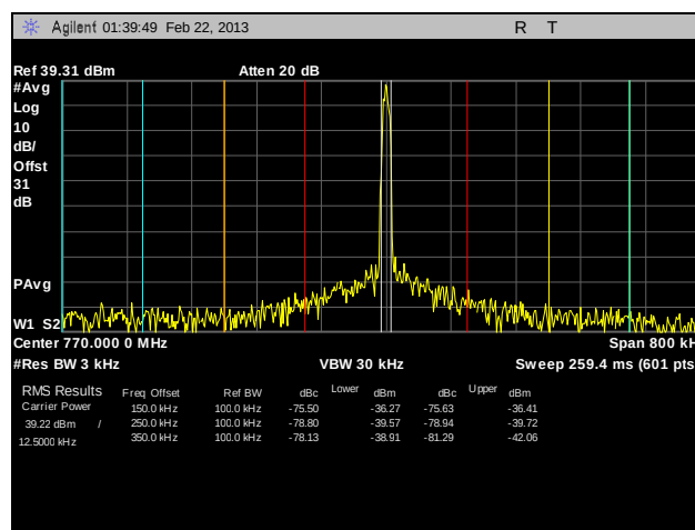
Plot 110. Adjacent Channel Power, Channel 770, C4FM, 10 W, 2
