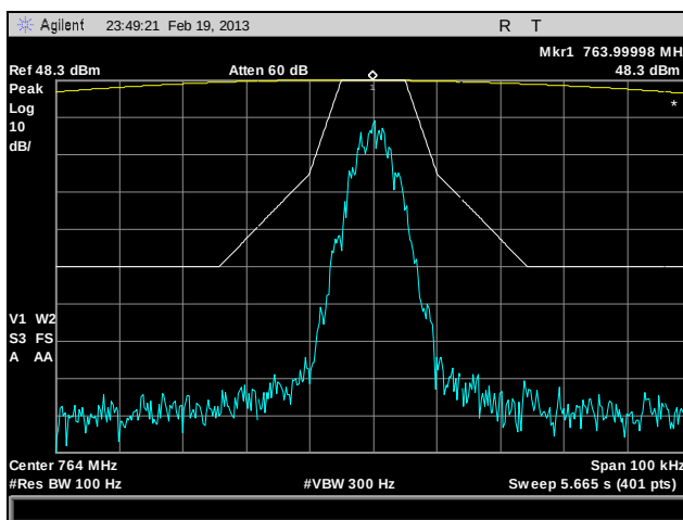
Plot 10. Emission Mask, 764 MHz, C4FM, 100 W
