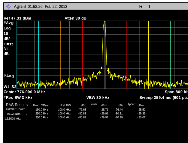
Plot 165. Adjacent Channel Power, Channel 776, HDQPSK, 100 W, 2
