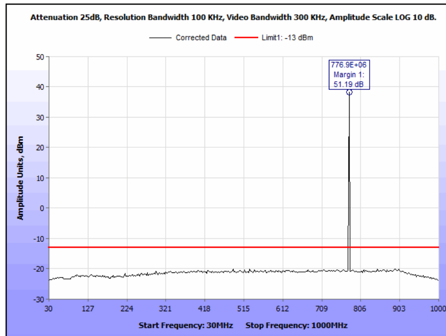
Plot 67. Conducted Spurious Emissions, 776 MHz, C4FM, 10 W, 30 MHz – 1 GHz
