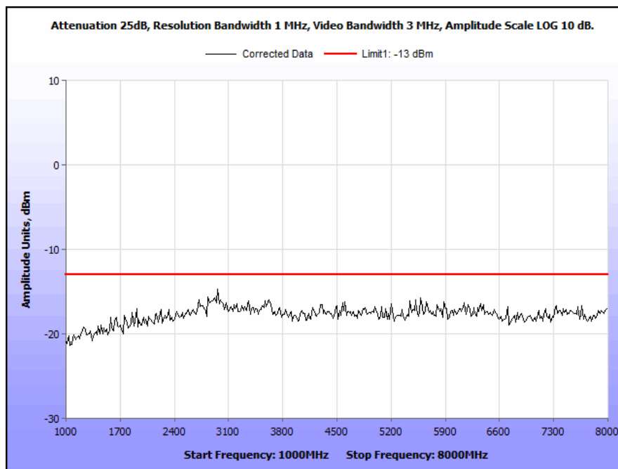
Plot 48. Conducted Spurious Emissions, 764 MHz, HDQPSK, 10 W, 1 GHz – 8 GHz
