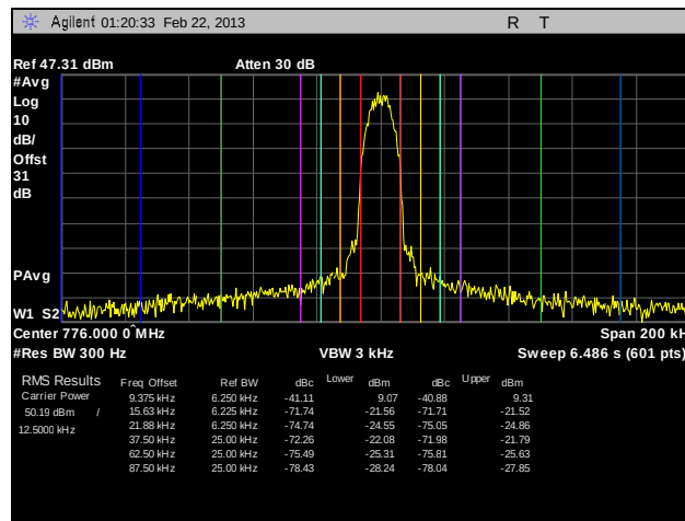
Plot 164. Adjacent Channel Power, Channel 776, HDQPSK, 100 W, 1
