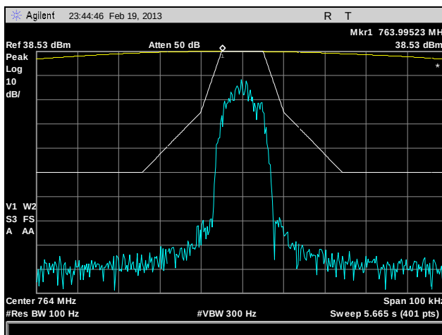
Plot 9. Emission Mask, 764 MHz, HDQPSK, 10 W
