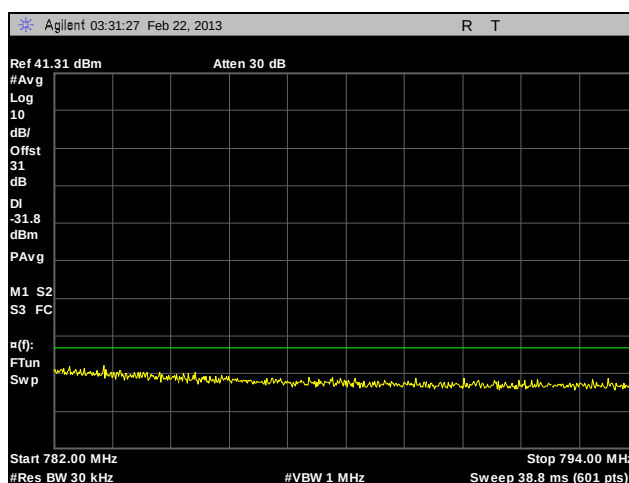
Plot 127. Adjacent Channel Power, Channel 770, 12 MHz – Paired Receive Band, C4FM, 100 W
