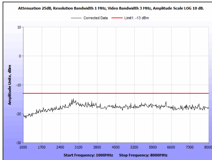
Plot 70. Conducted Spurious Emissions, 776 MHz, CQPSK, 10 W, 1 GHz – 8 GHz
