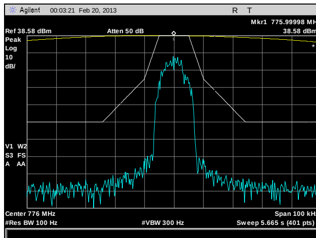
Plot 21. Emission Mask, 776 MHz, HDQPSK, 10 W
