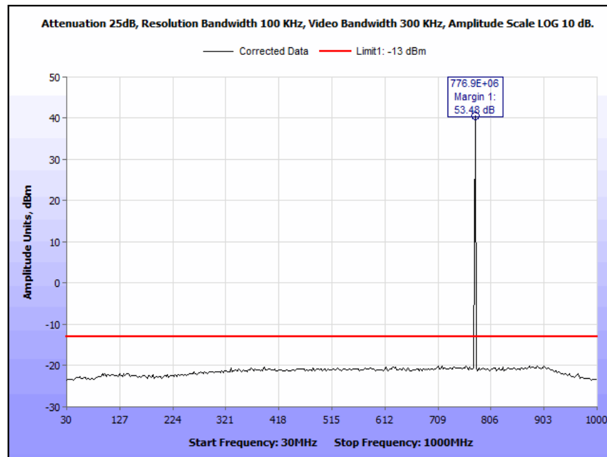
Plot 71. Conducted Spurious Emissions, 776 MHz, HDQPSK, 10 W, 30 MHz – 1 GHz
