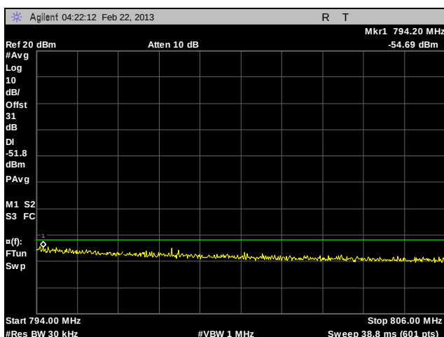
Plot 138. Adjacent Channel Power, Channel 770, Paired Receive Band, HDQPSK, 100 W
