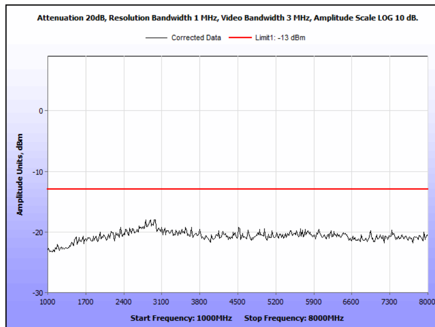
Plot 60. Conducted Spurious Emissions, 770 MHz, HDQPSK, 10 W, 1 GHz – 8 GHz
