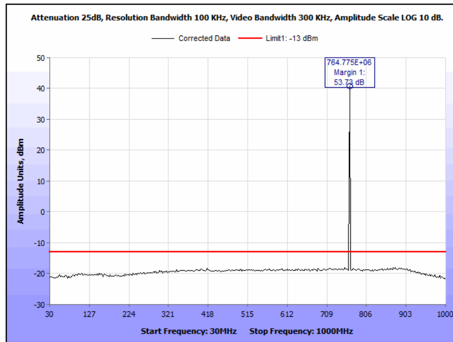
Plot 45. Conducted Spurious Emissions, 764 MHz, CQPSK, 10 W, 30 MHz – 1 GHz
