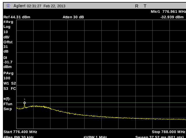
Plot 166. Adjacent Channel Power, Channel 776, 400 kHz – 12 MHz, HDQPSK, 100 W
