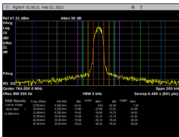
Plot 99. Adjacent Channel Power, Channel 764, CQPSK, 100 W, 1
