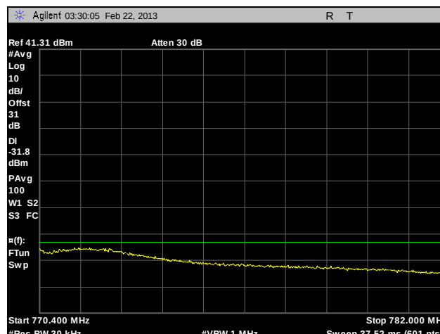
Plot 136. Adjacent Channel Power, Channel 770, 400 kHz – 12 MHz, HDQPSK, 100 W
