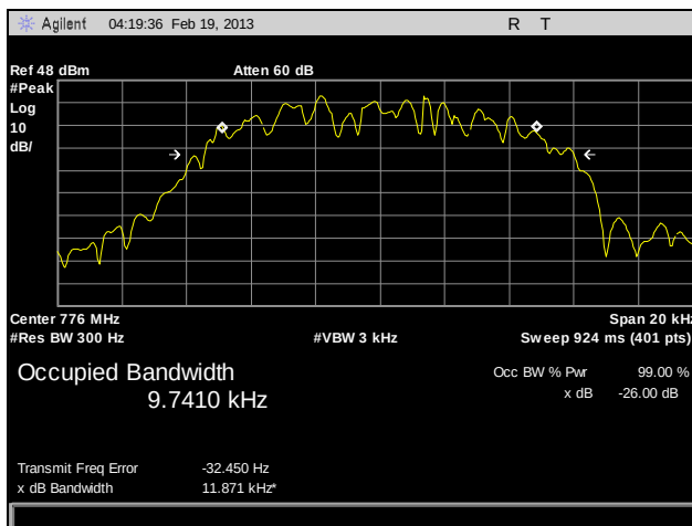
Plot 41. Occupied Bandwidth, 776 MHz, CQPSK, 100 W
