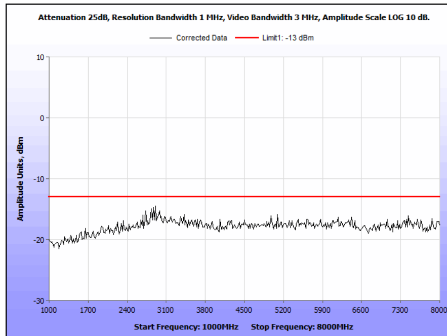
Plot 72. Conducted Spurious Emissions, 776 MHz, HDQPSK, 10 W, 1 GHz – 8 GHz
