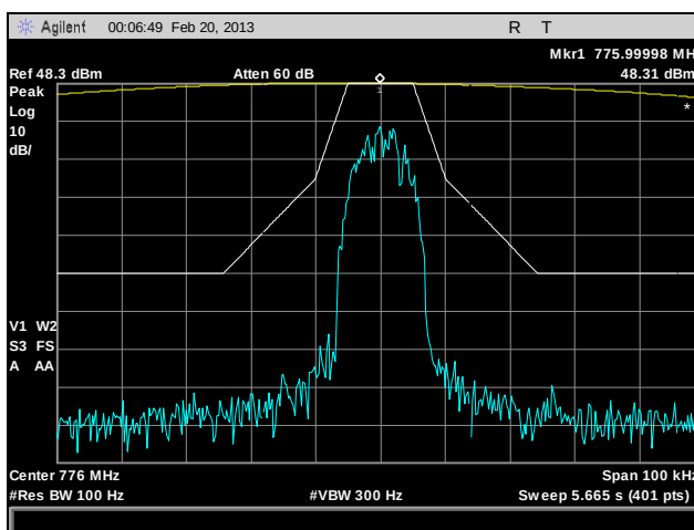
Plot 23. Emission Mask, 776 MHz, CQPSK, 100 W
