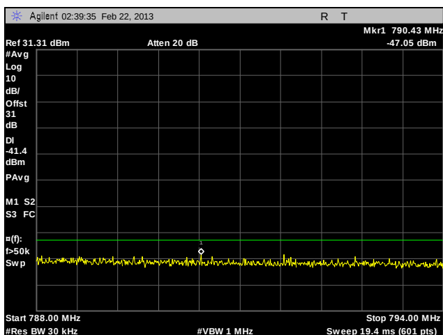
Plot 147. Adjacent Channel Power, Channel 776, 12 MHz – Paired Receive Band, CQPSK, 10 W
