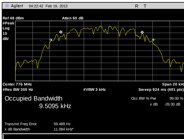
Plot 42. Occupied Bandwidth, 776 MHz, HDQPSK, 100 W
