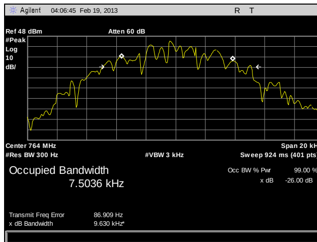
Plot 28. Occupied Bandwidth, 764 MHz, C4FM, 100 W
