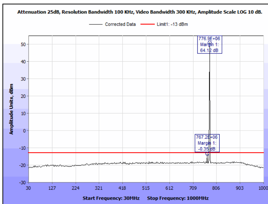
Plot 75. Conducted Spurious Emissions, 776 MHz, CQPSK, 100 W, 30 MHz – 1 GHz
