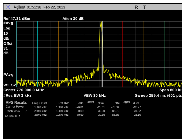
Plot 155. Adjacent Channel Power, Channel 776, C4FM, 100 W, 2
