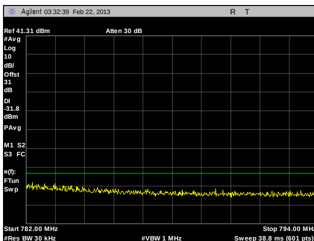
Plot 137. Adjacent Channel Power, Channel 770, 12 MHz – Paired Receive Band, HDQPSK, 100 W
