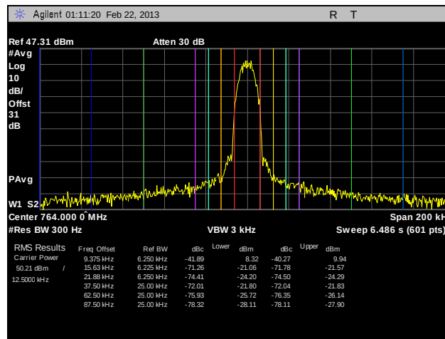
Plot 104. Adjacent Channel Power, Channel 764, HDQPSK, 100 W, 1
