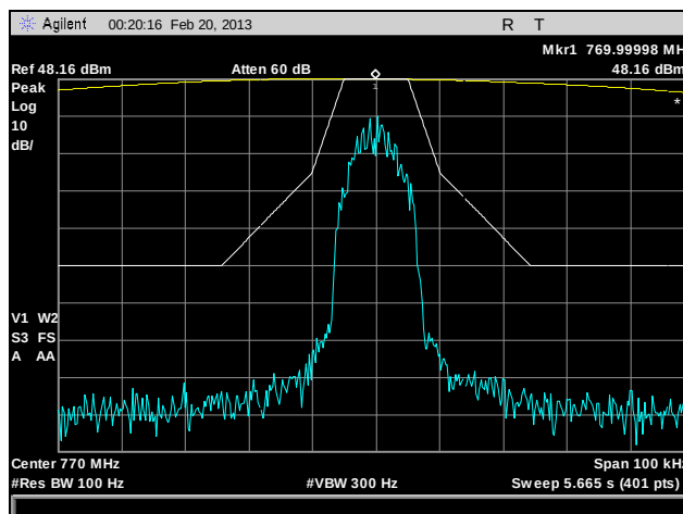
Plot 18. Emission Mask, 770 MHz, HDQPSK, 100 W
