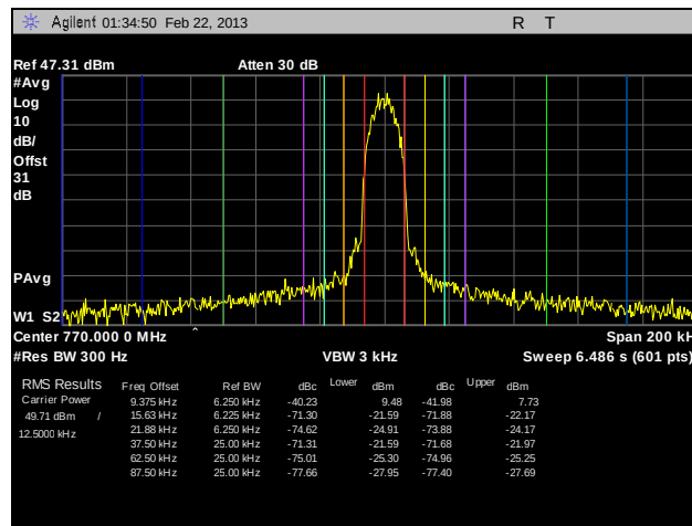
Plot 134. Adjacent Channel Power, Channel 770, HDQPSK, 100 W, 1
