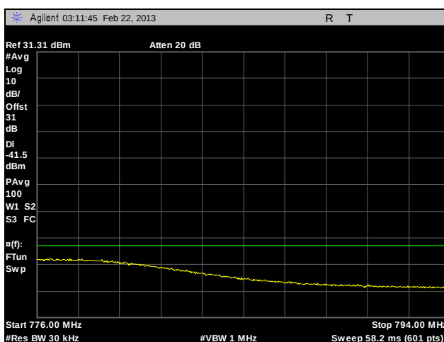
Plot 87. Adjacent Channel Power, Channel 764, 12 MHz – Paired Receive Band, CQPSK, 10 W
