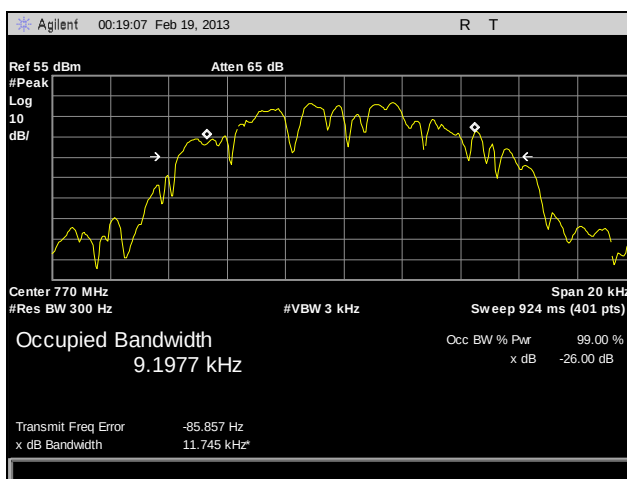
Plot 35. Occupied Bandwidth, 770 MHz, CQPSK, 100 W
