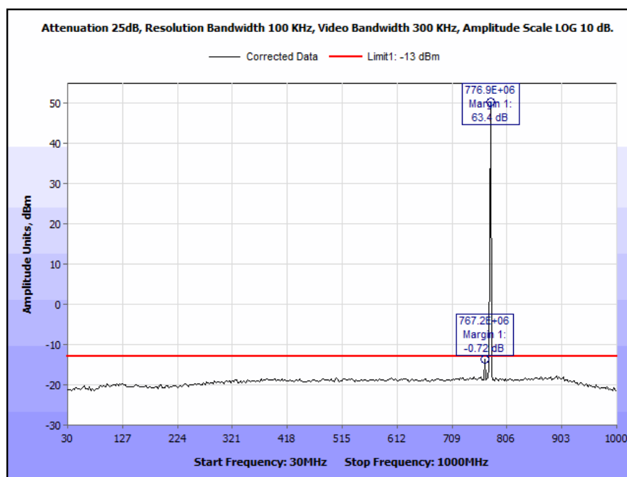
Plot 77. Conducted Spurious Emissions, 776 MHz, HDQPSK, 100 W, 30 MHz – 1 GHz
