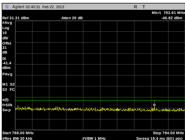
Plot 152. Adjacent Channel Power, Channel 776, 12 MHz – Paired Receive Band, HDQPSK, 10 W
