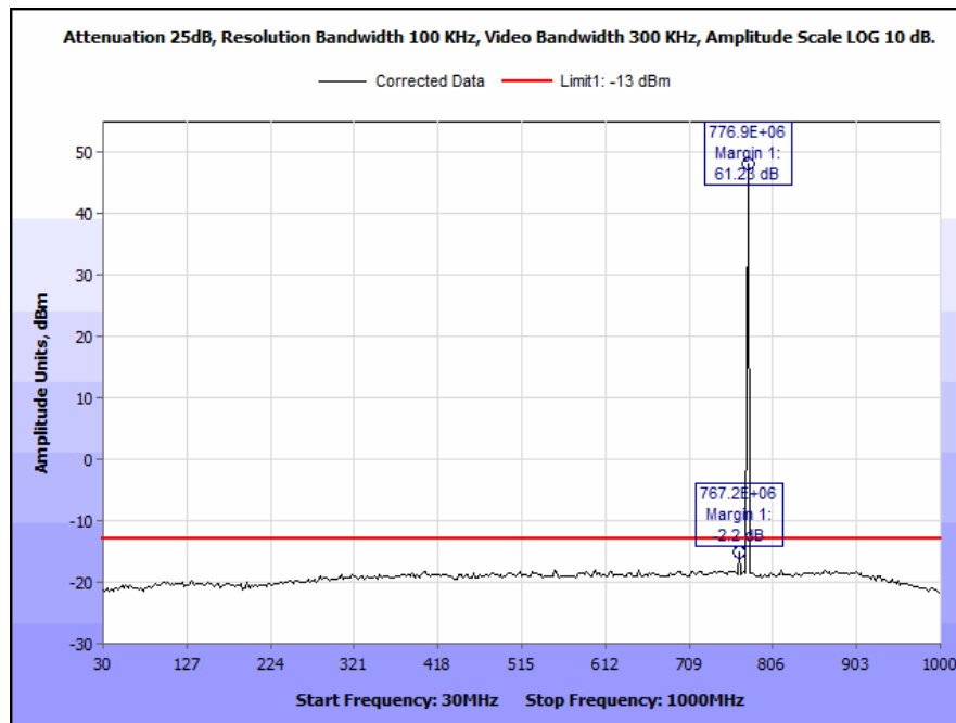
Plot 73. Conducted Spurious Emissions, 776 MHz, C4FM, 100 W, 30 MHz – 1 GHz
