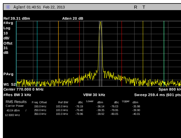
Plot 120. Adjacent Channel Power, Channel 770, HDQPSK, 10 W, 2
