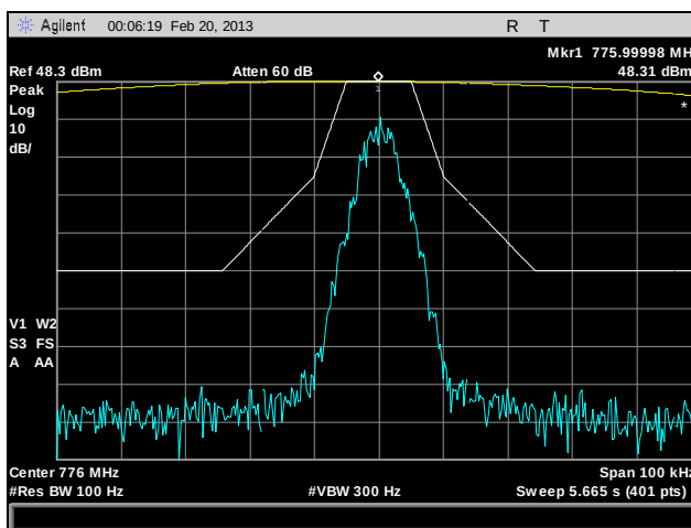
Plot 22. Emission Mask, 776 MHz, C4FM, 100 W
