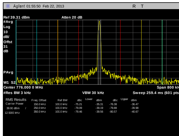
Plot 145. Adjacent Channel Power, Channel 776, CQPSK, 10 W, 2
