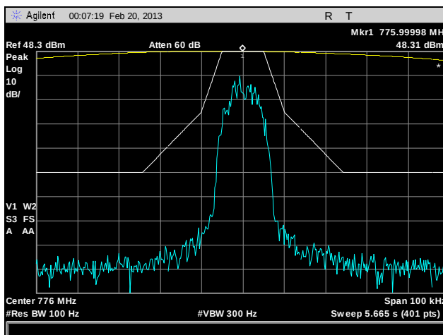
Plot 24. Emission Mask, 776 MHz, HDQPSK, 100 W
