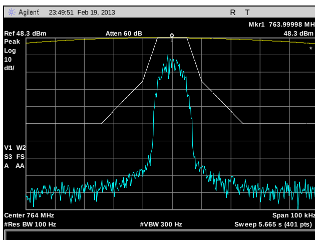
Plot 11. Emission Mask, 764 MHz, CQPSK, 100 W
