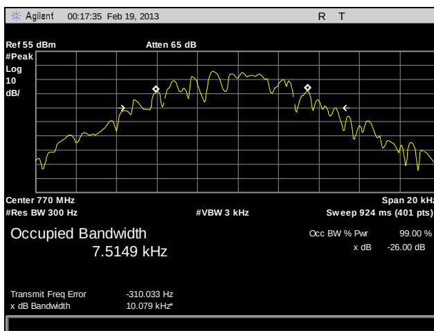
Plot 34. Occupied Bandwidth, 770 MHz, C4FM, 100 W
