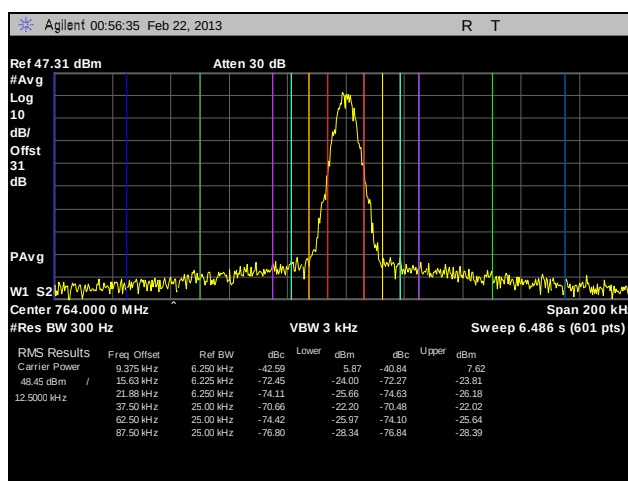
Plot 94. Adjacent Channel Power, Channel 764, C4FM, 100 W, 1
