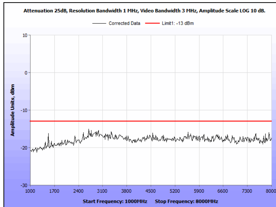
Plot 50. Conducted Spurious Emissions, 764 MHz, C4FM, 100 W, 1 GHz – 8 GHz
