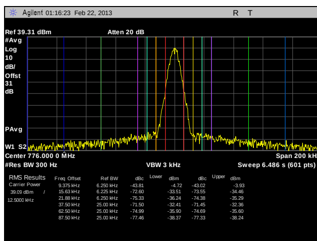
Plot 139. Adjacent Channel Power, Channel 776, C4FM, 10 W, 1
