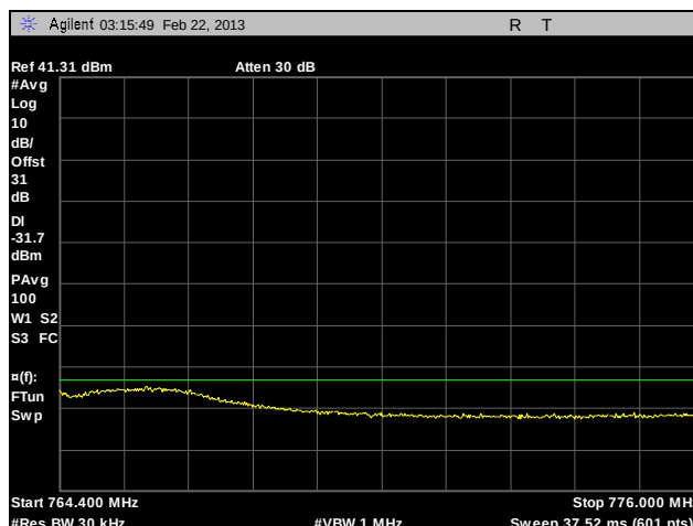
Plot 101. Adjacent Channel Power, Channel 764, 400 kHz – 12 MHz, CQPSK, 100 W
