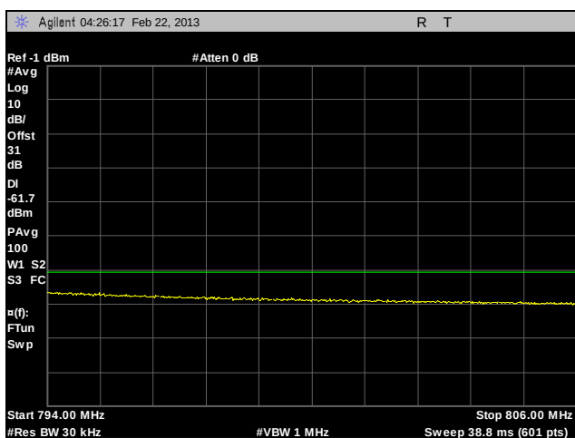
Plot 123. Adjacent Channel Power, Channel 770, Paired Receive Band, HDQPSK, 10 W
