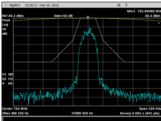
Plot 12. Emission Mask, 764 MHz, HDQPSK, 100 W
