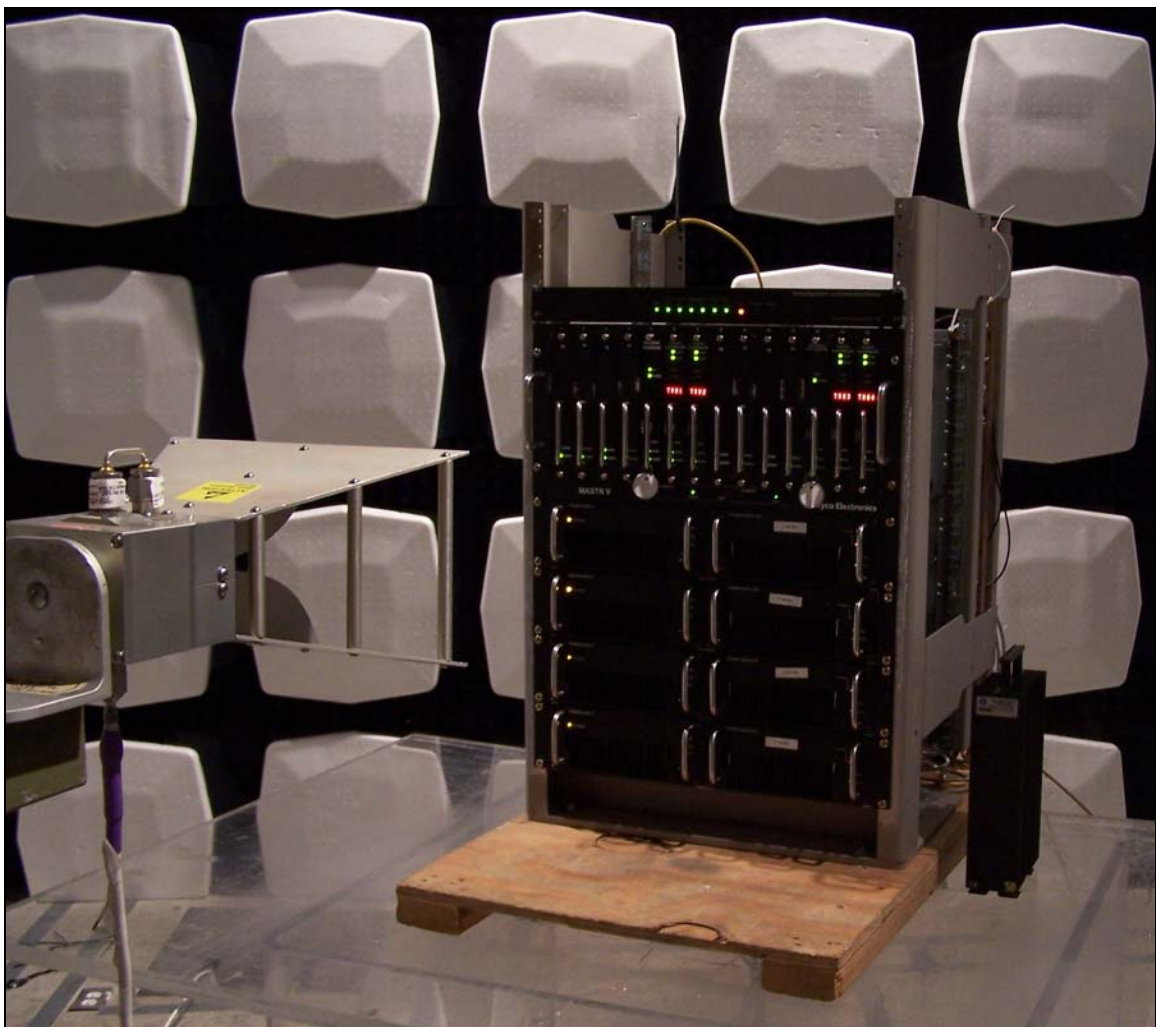
Photograph 2. Radiated Spurious Emissions Test Setup
