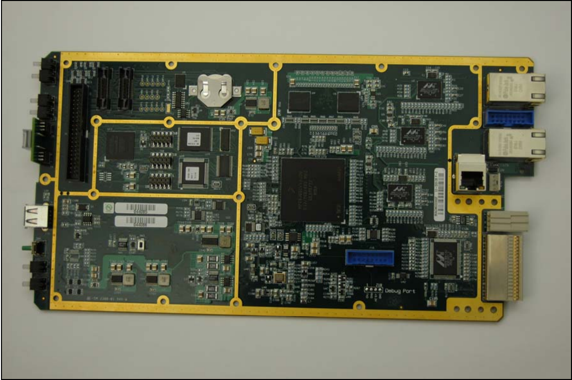
Photograph 21. Traffic Controller - Top Side
