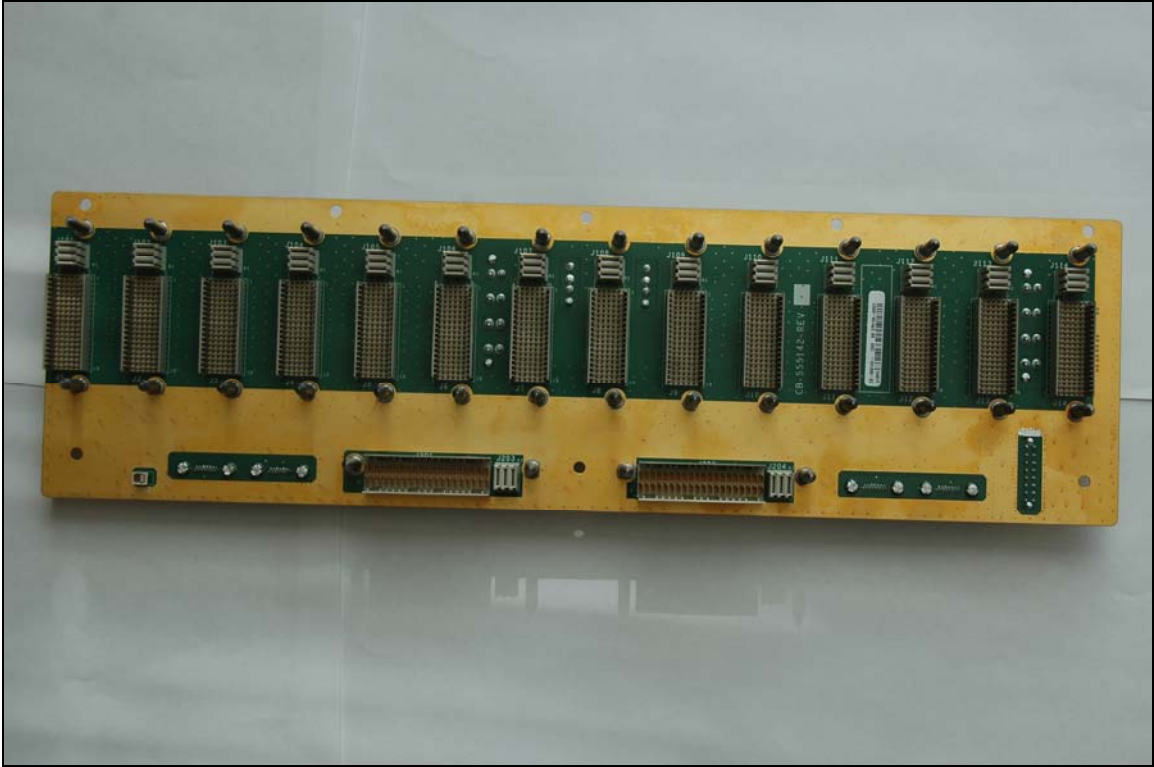
Photograph 1. Backplane - Top Side
