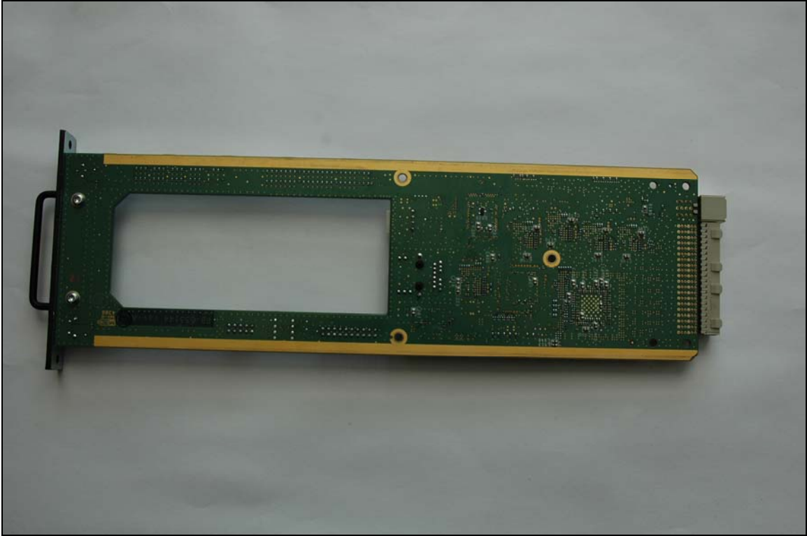
Photograph 11. E-Switch - Bottom Side
