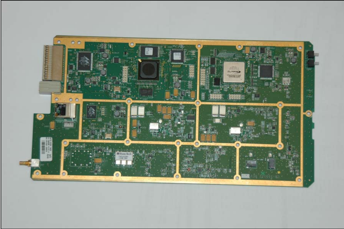
Photograph 23. Transmit Module - Top Side
