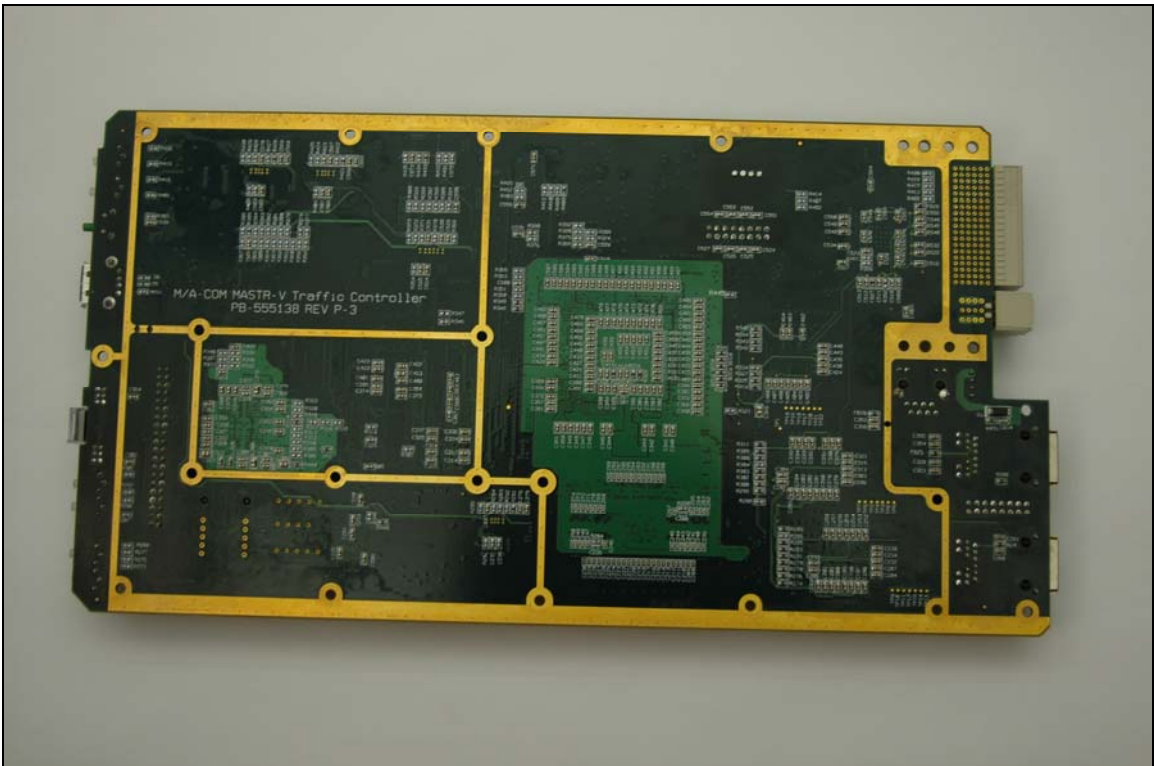
Photograph 20. Traffic Controller - Bottom Side
