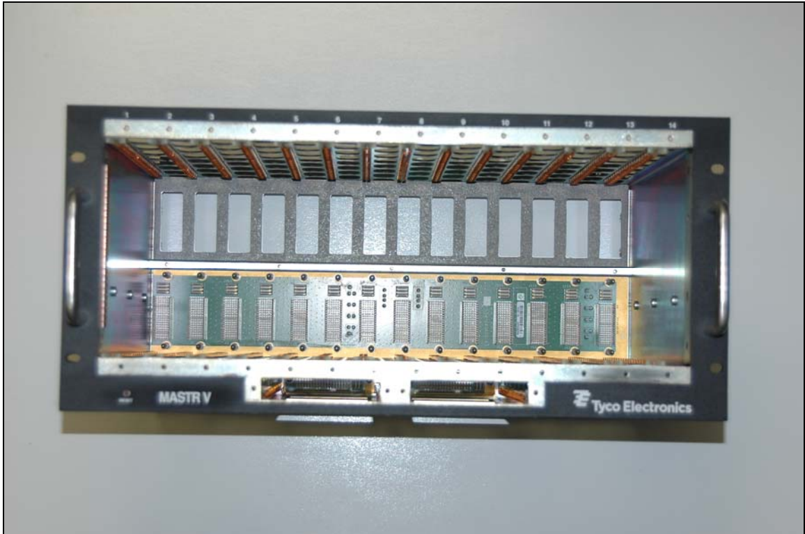
Photograph 7. Chassis – Front
