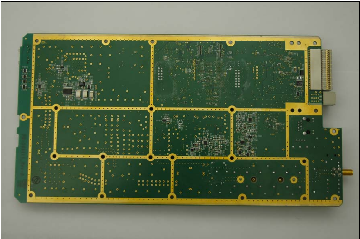
Photograph 18. Receiver Module - Bottom Side
