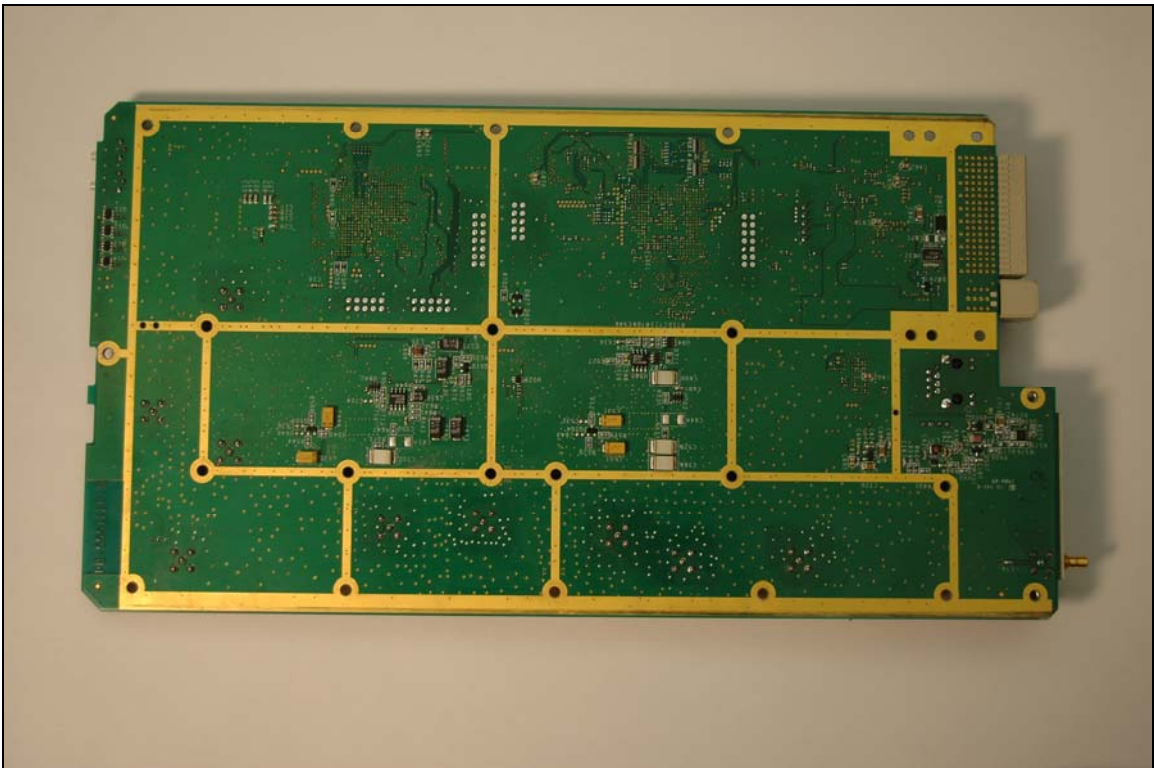
Photograph 22. Transmit Module - Bottom Side
