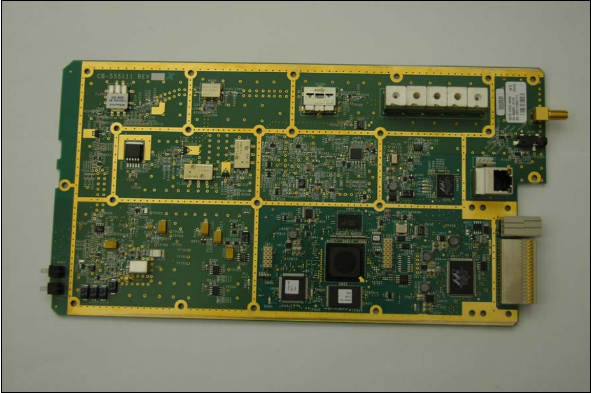
Photograph 19. Receiver Module - Top Side
