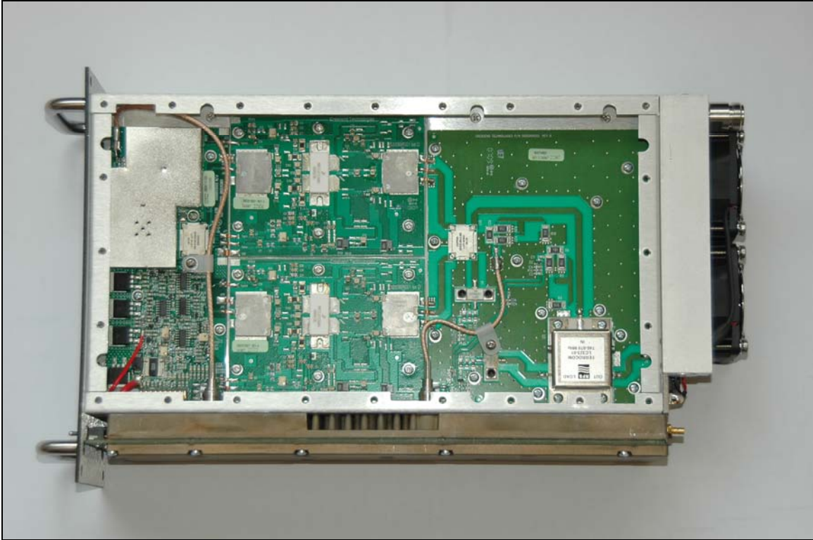
Photograph 15. Power Amplifier
