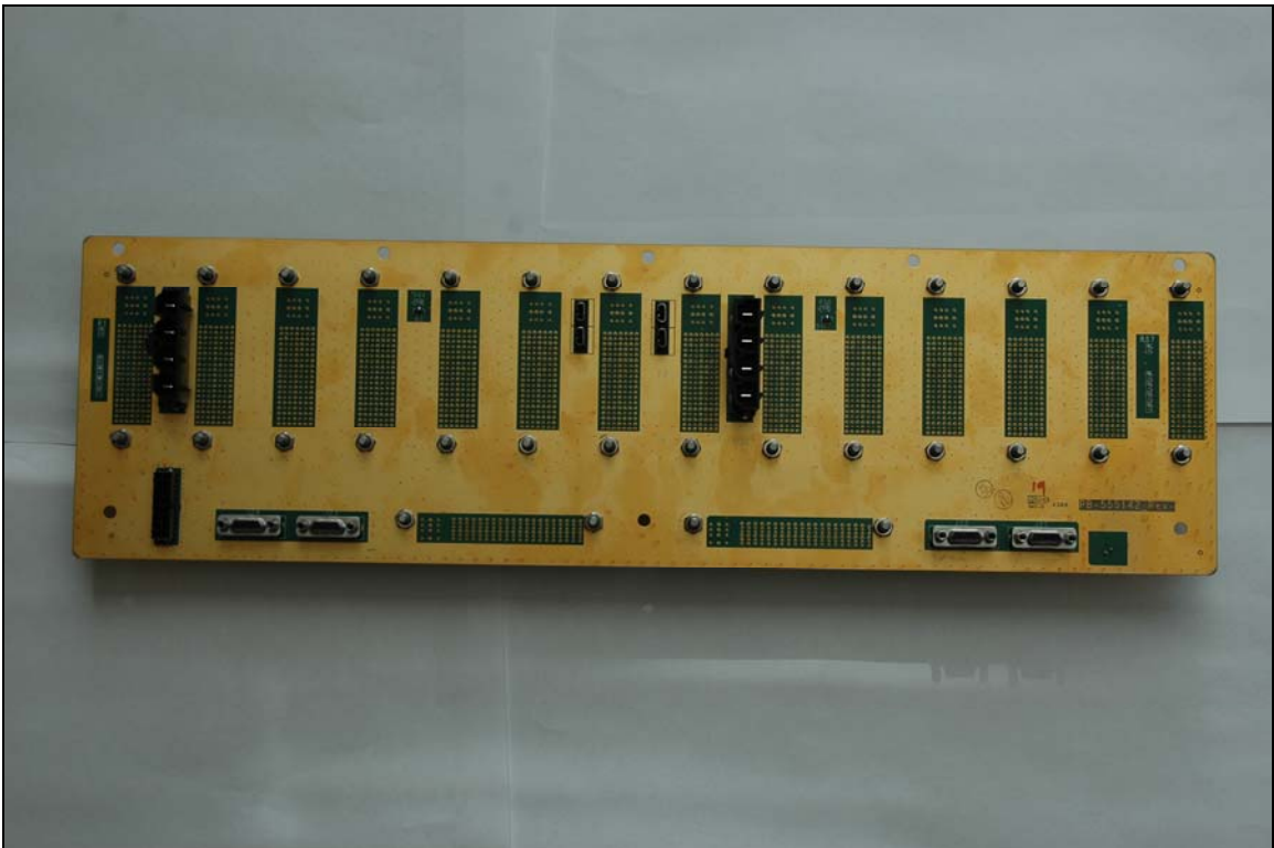
Photograph 2. Backplane Bottom Side
