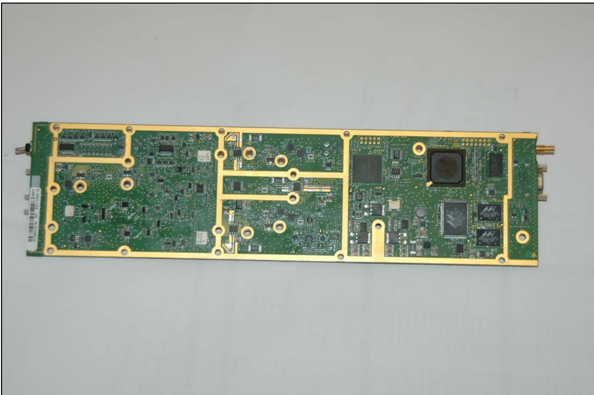
Photograph 14. Linearizer - Top Side
