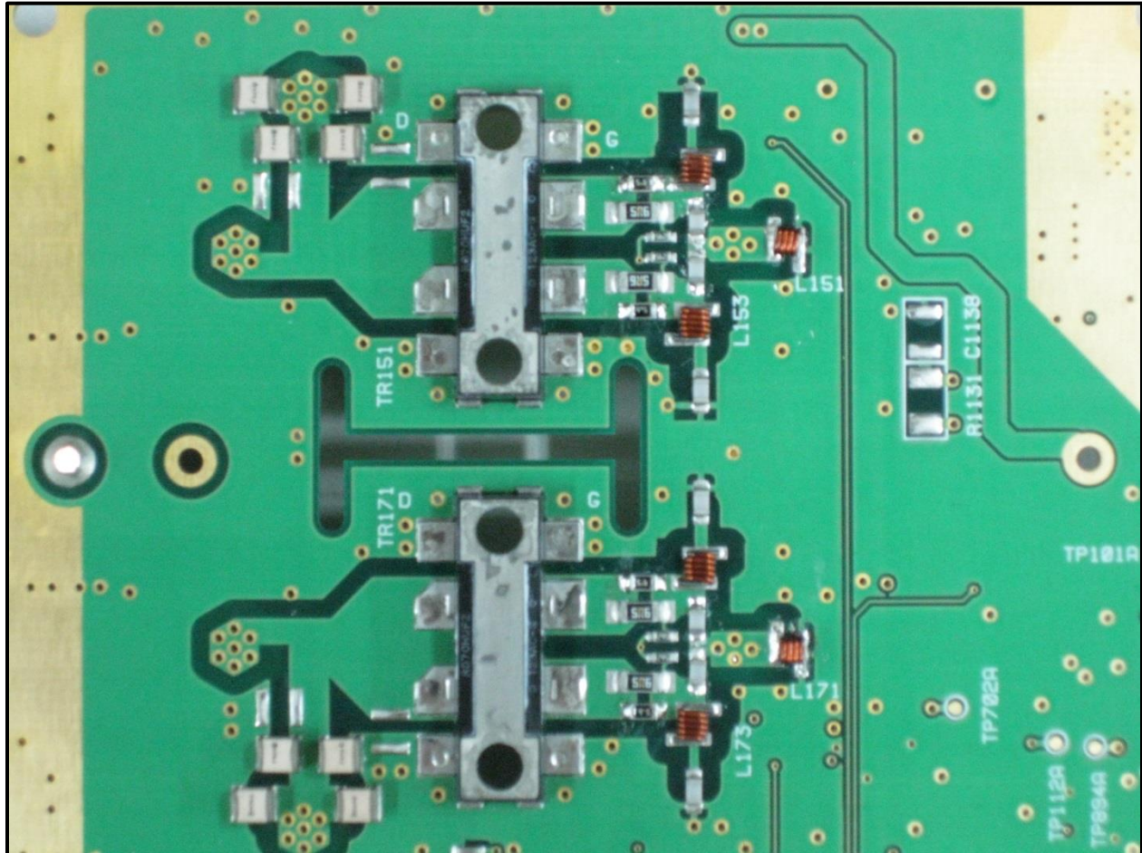
Photograph 2: RF Processor Board Solder Change Final AMP
