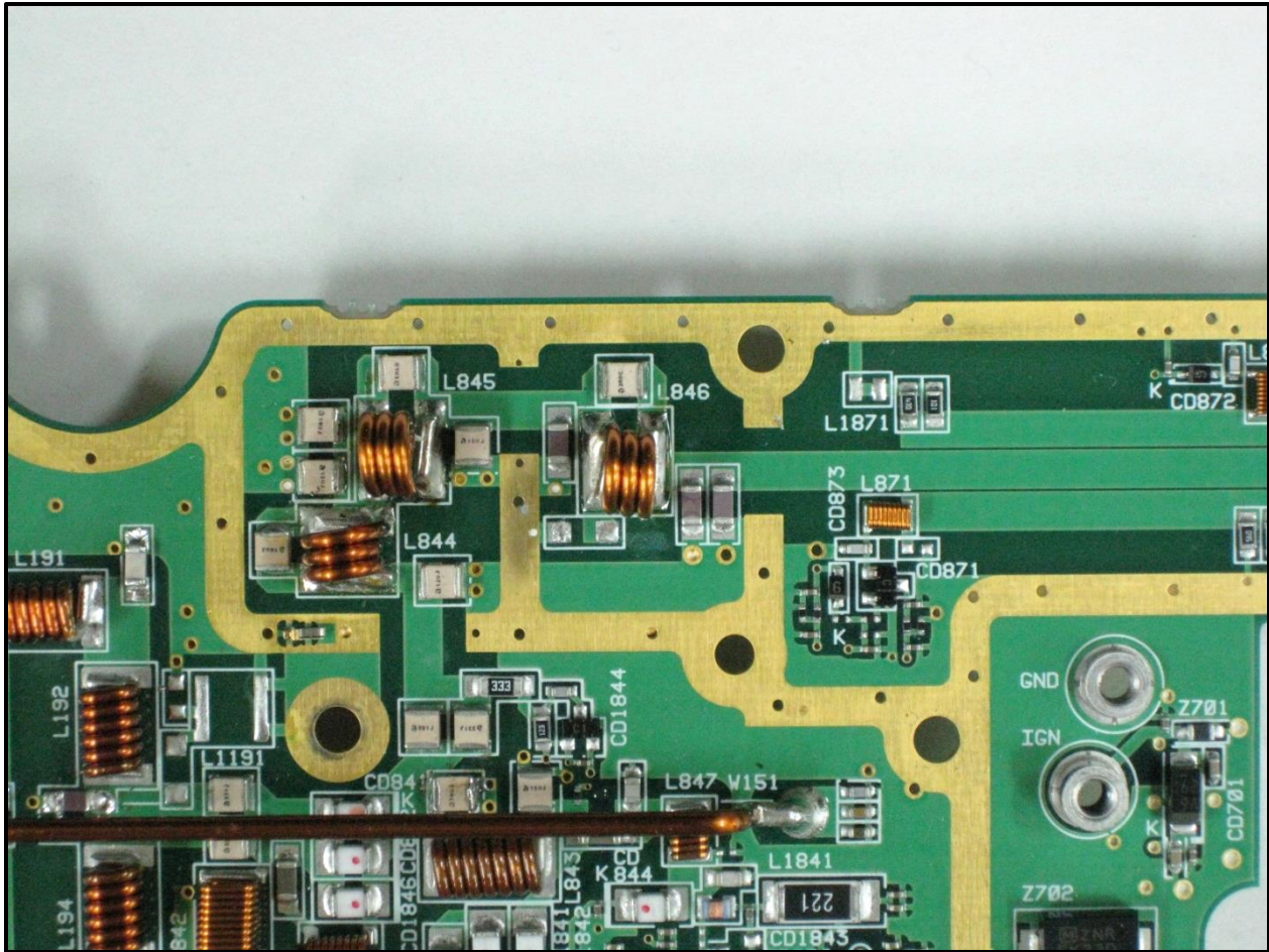
Photograph 1: RF Processor Board Component Change LPF
