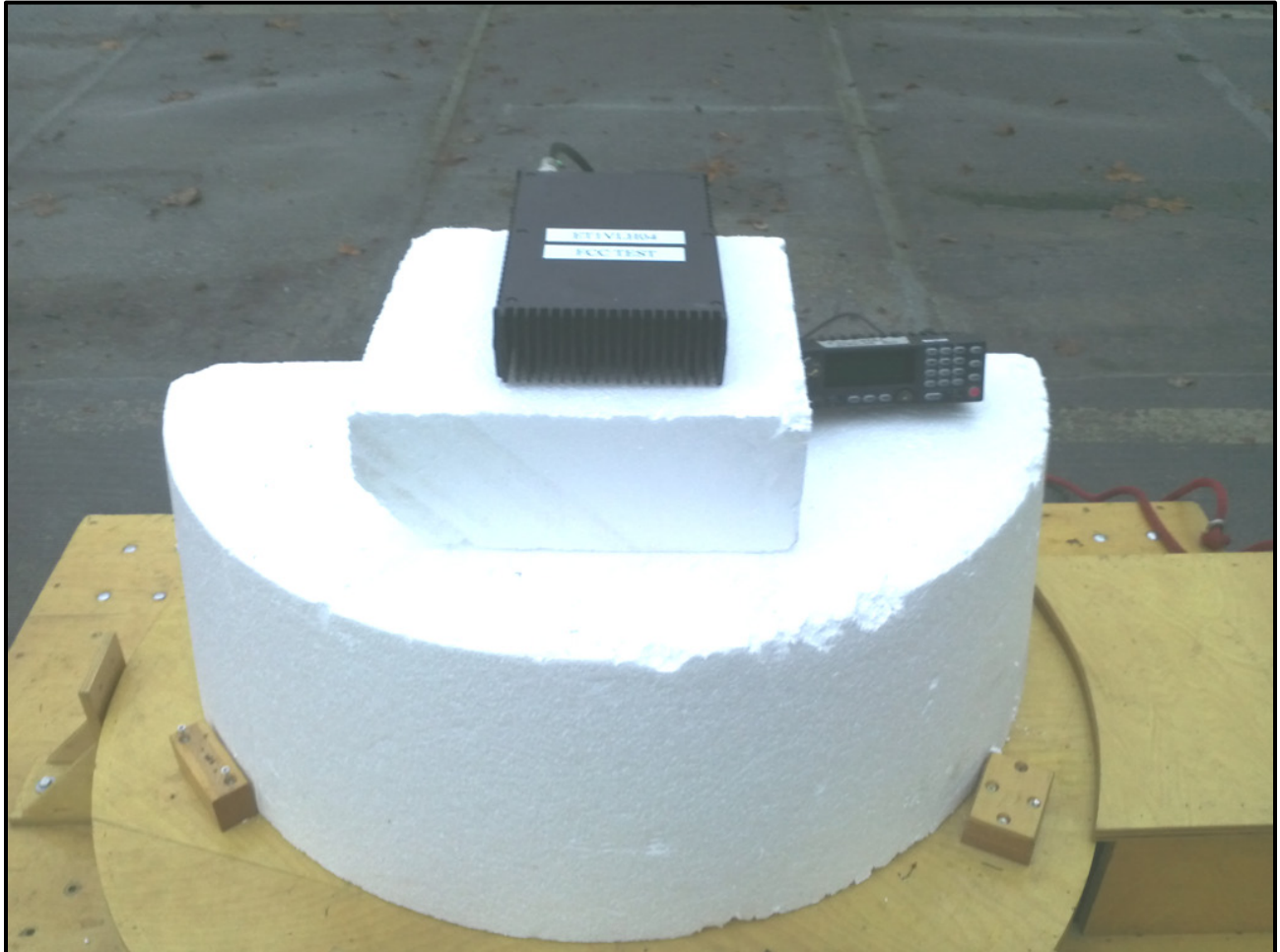
Photograph 5: Radiated Emissions – Front View
