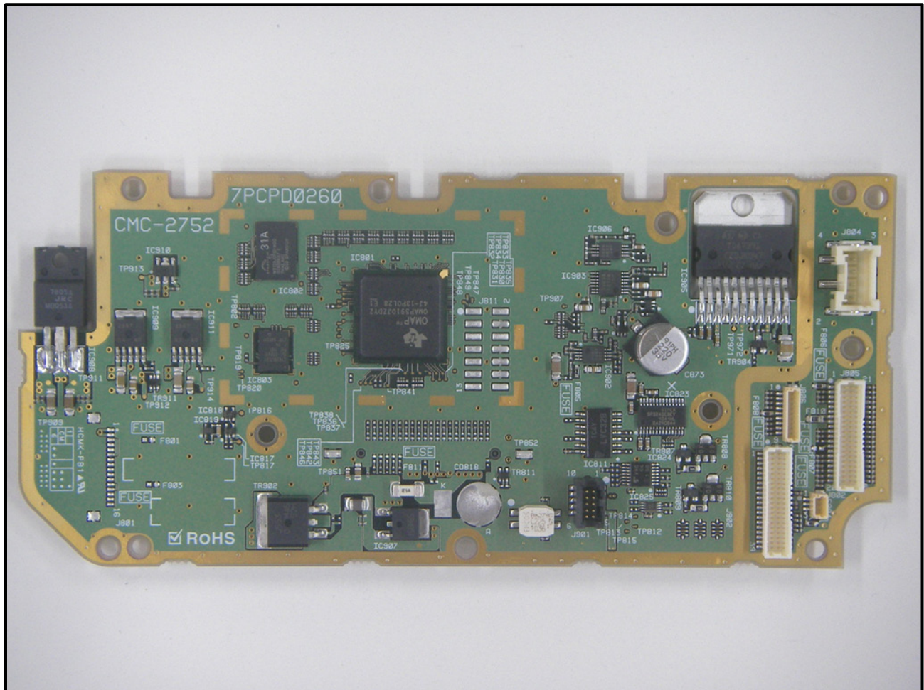
Photograph 18: PK Board – Component Side
