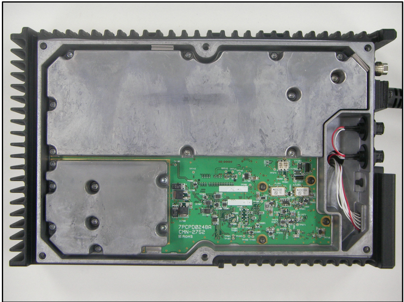
Photograph 14: Bottom Cover Removed
