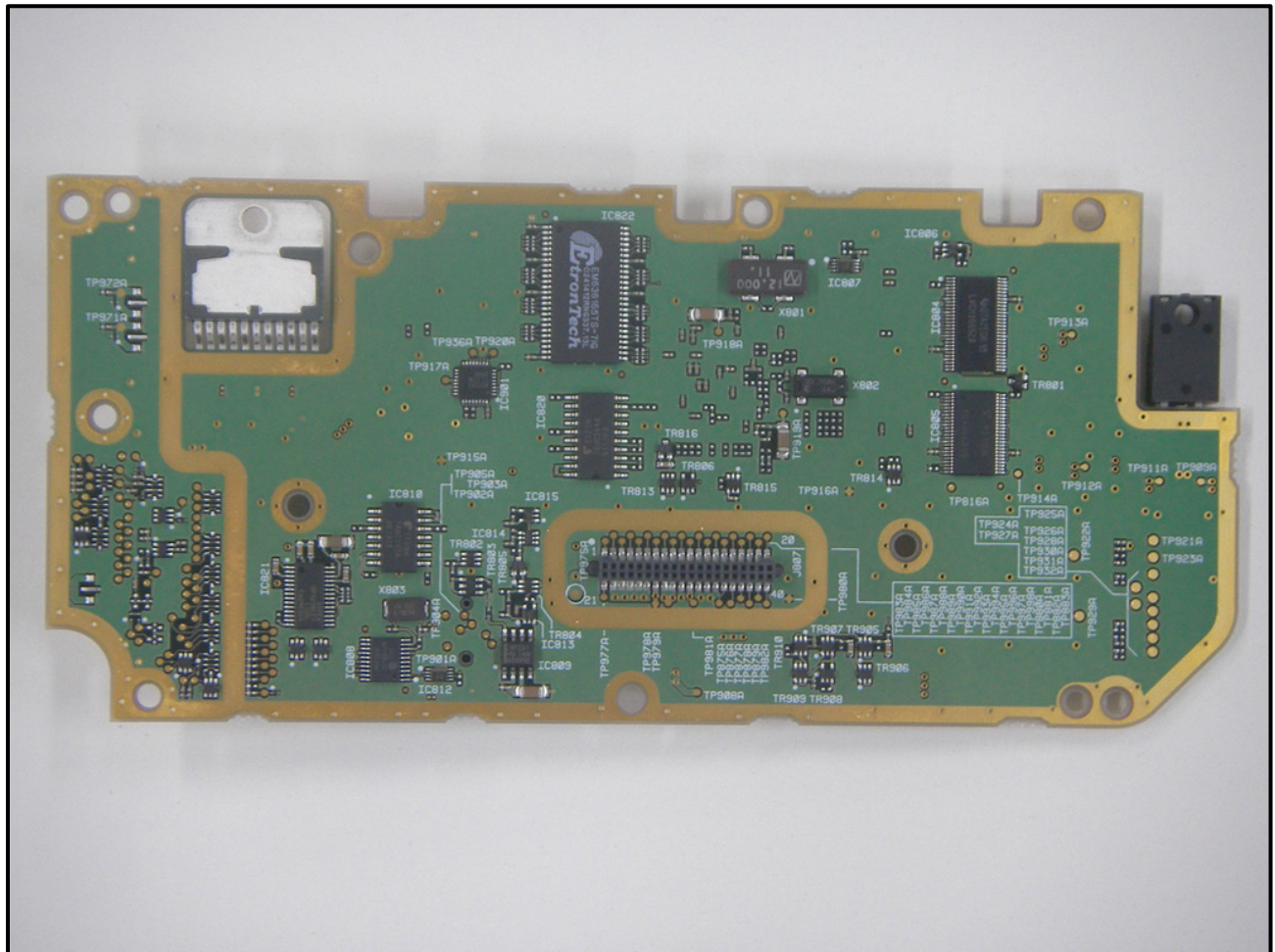
Photograph 19: PK Board – Solder Side
