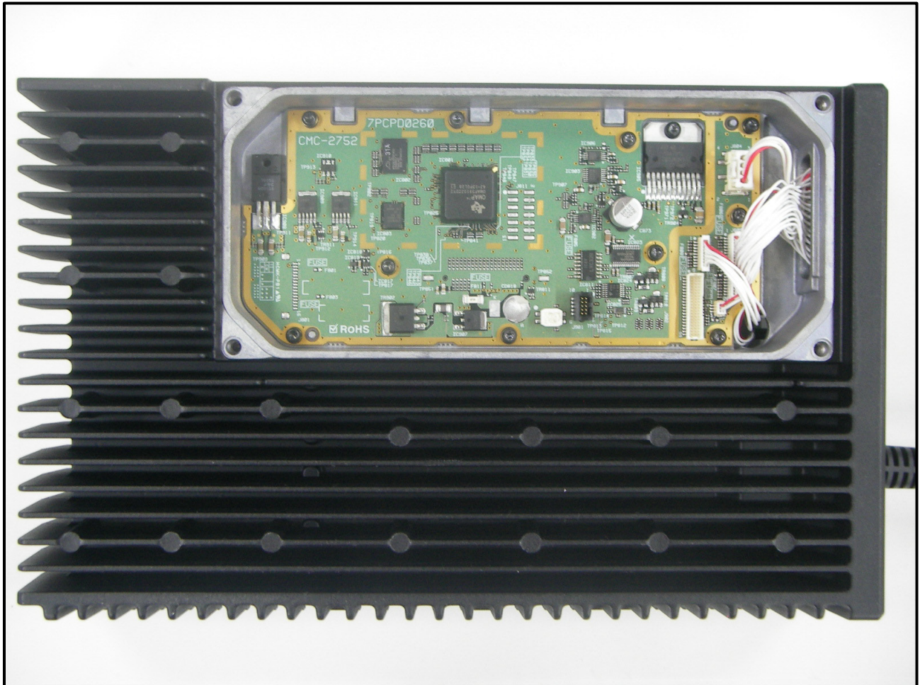
Photograph 13: Top Cover Removed
