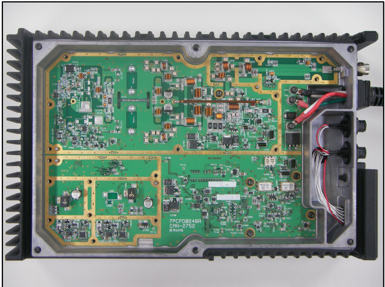
Photograph 15: Bottom Cover and Shield Removed
