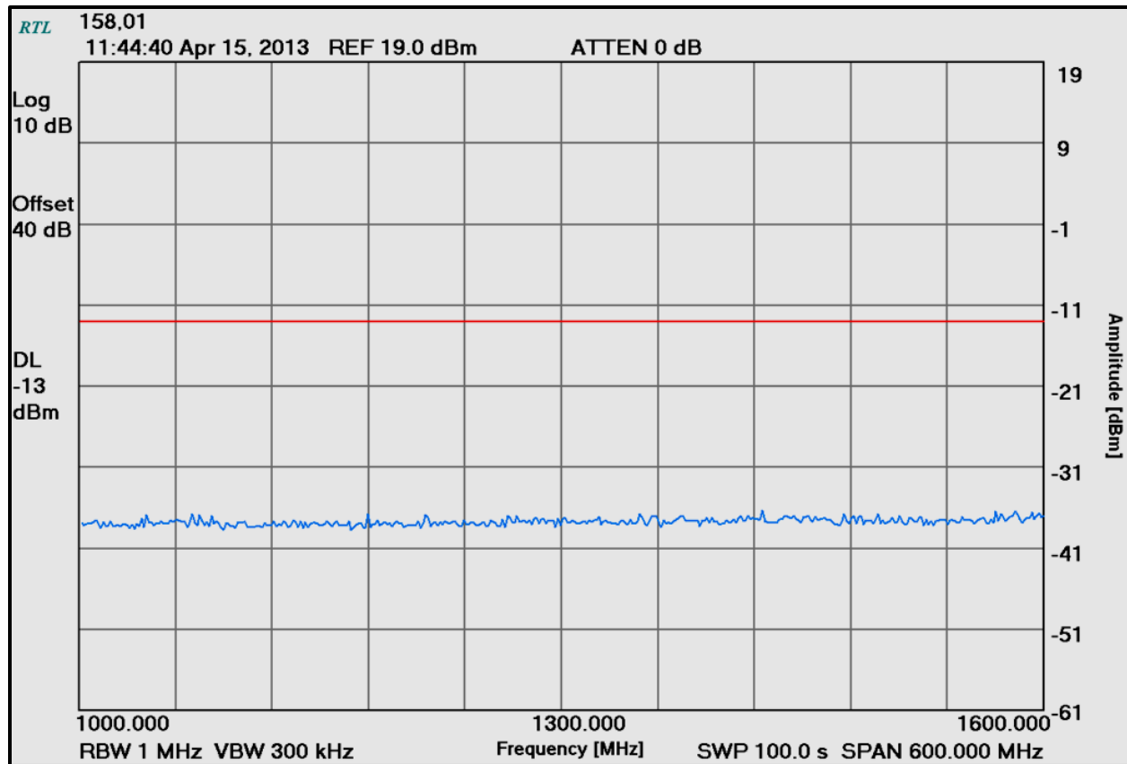
Plot 4-2: Conducted Spurious Emissions - 158.01 MHz; 1 GHz – 1.6 GHz
