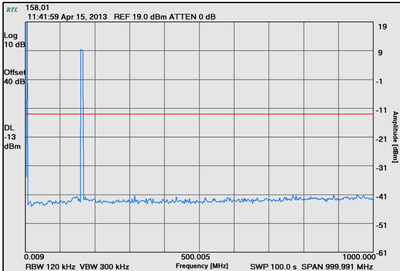
Plot 4-1: Conducted Spurious Emissions - 158.01 MHz; 9 kHz - 1 GHz
