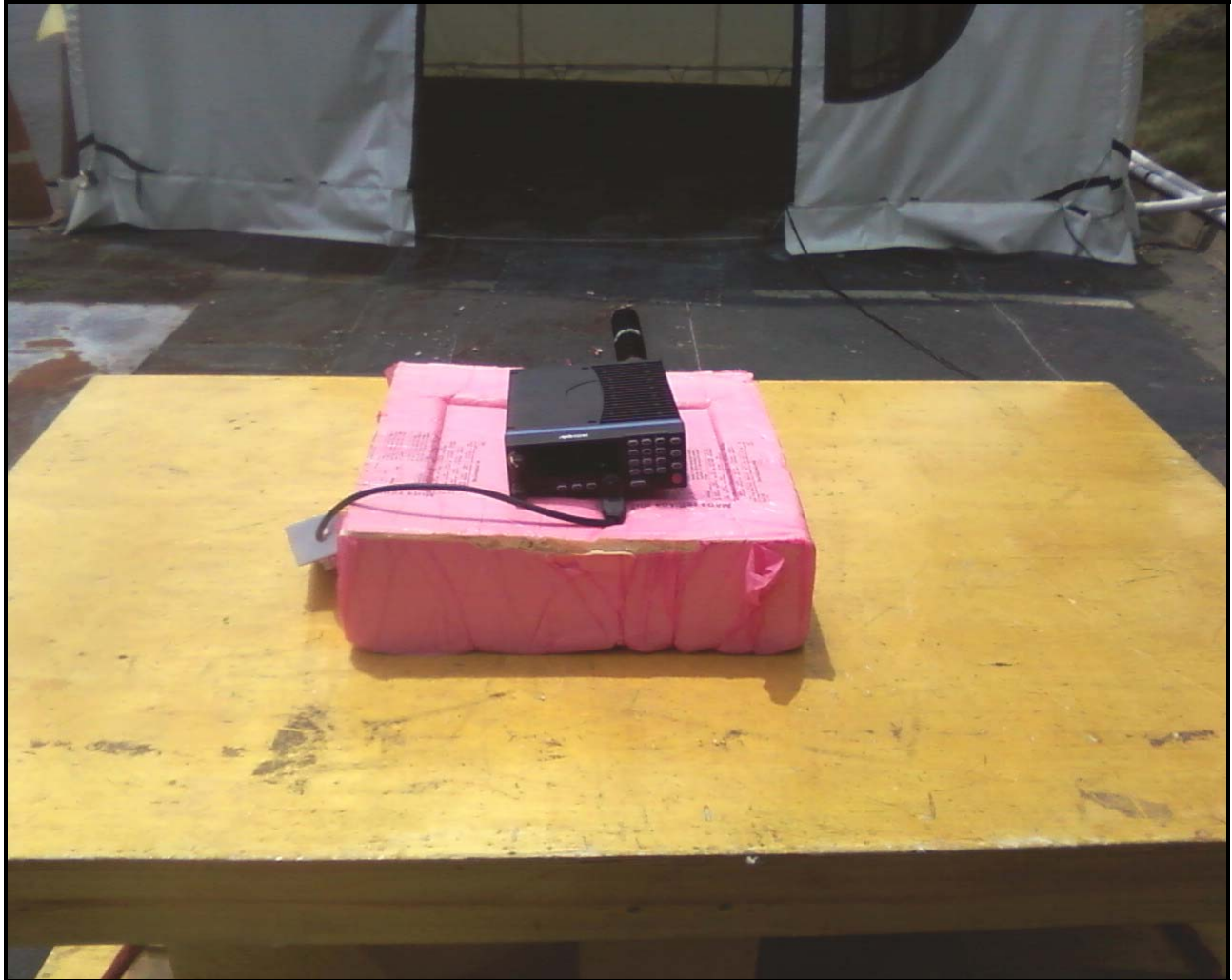
Photograph 4: Radiated Emissions – Front View
