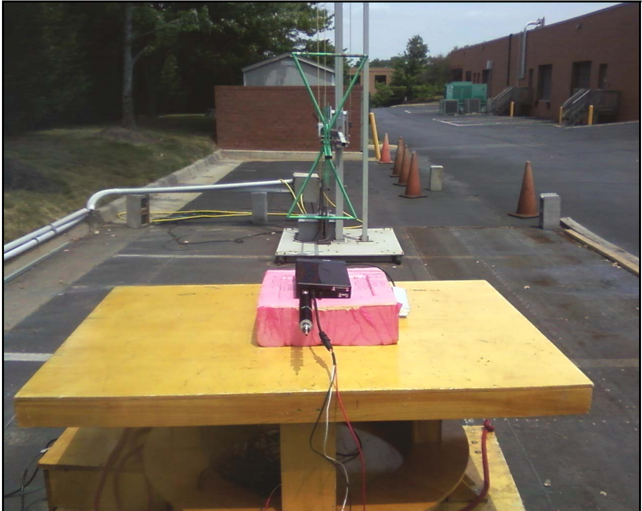
Photograph 5: Radiated Emissions – Back View
