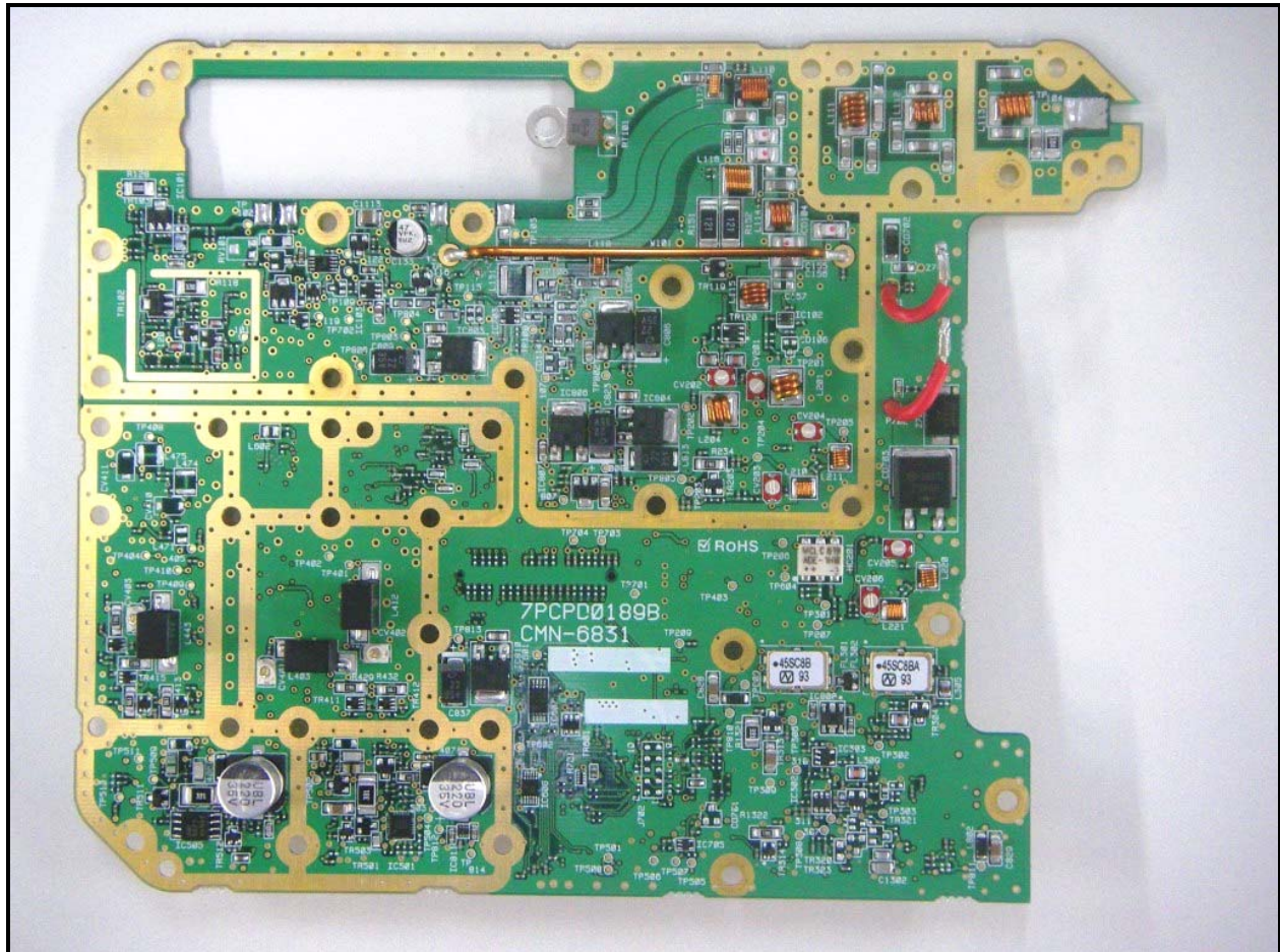
Photograph 29: RF Processor Board Component Side Complete
