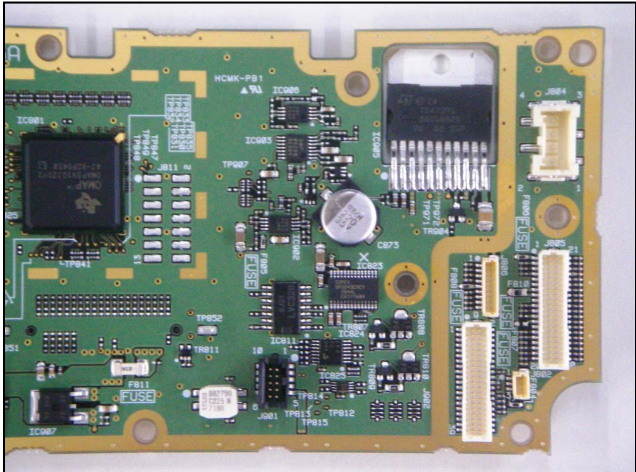
Photograph 25: PK Board Component Side Right
