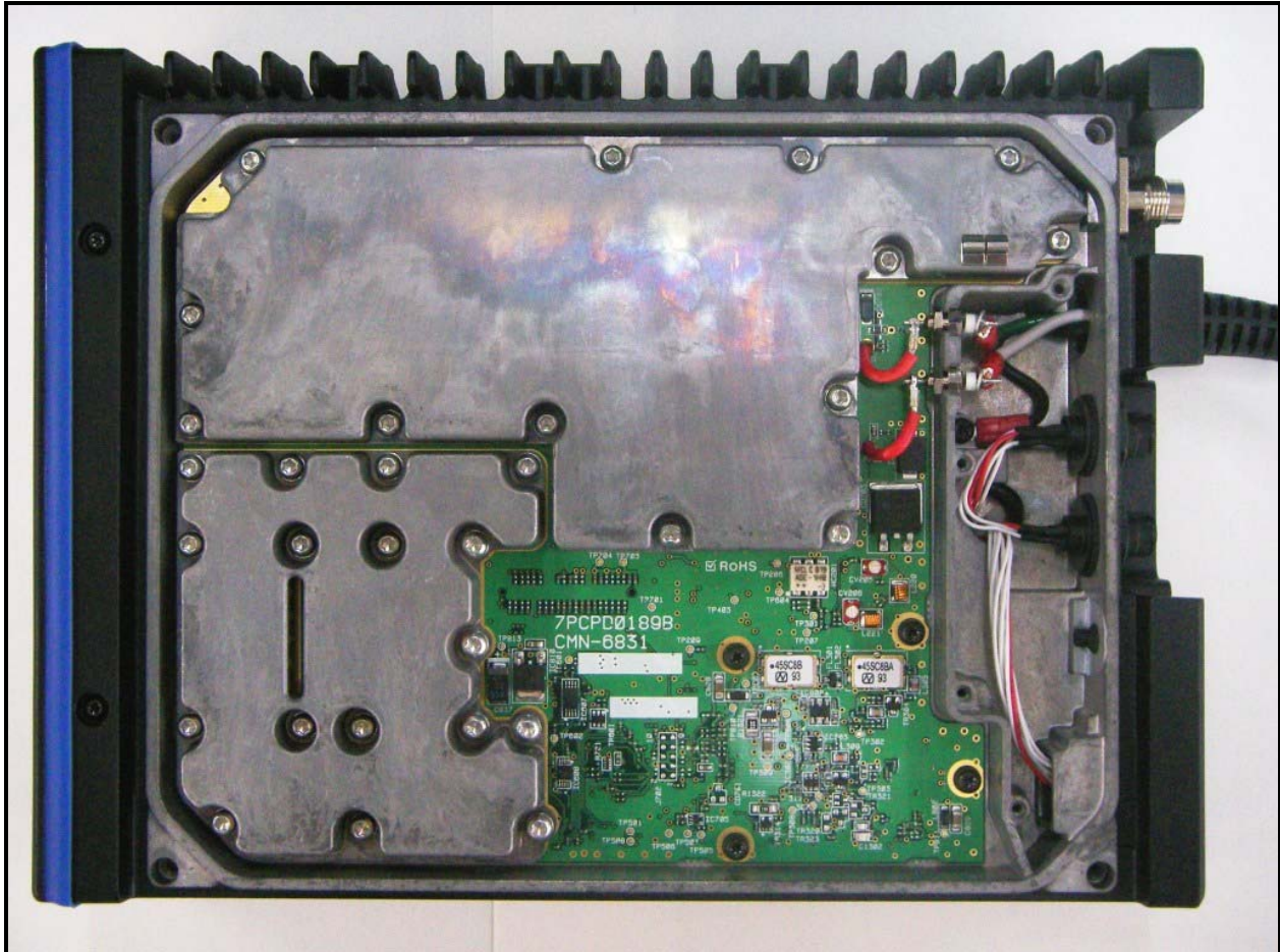
Photograph 21: Bottom Cover Removed
