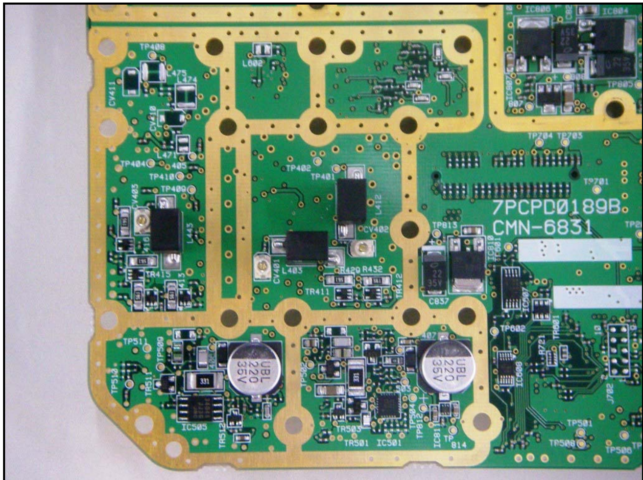
Photograph 30: RF Processor Board Component Side Lower Left
