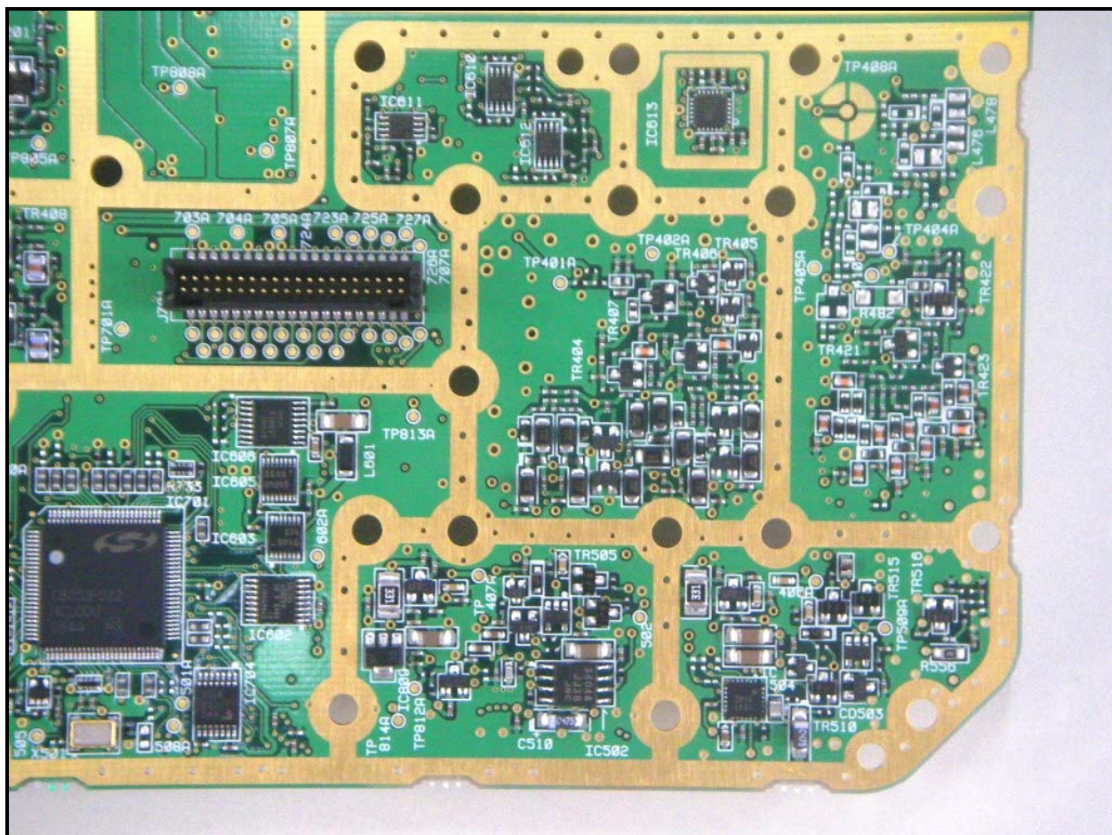
Photograph 35: RF Processor Board Solder Side Lower Right
