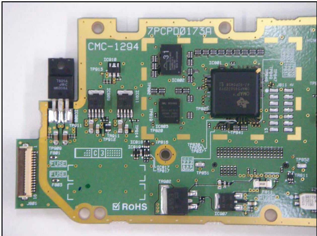
Photograph 24: PK Board Component Side Left
