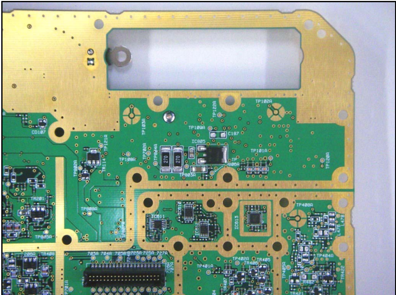
Photograph 37: RF Processor Board Solder Side Upper Right
