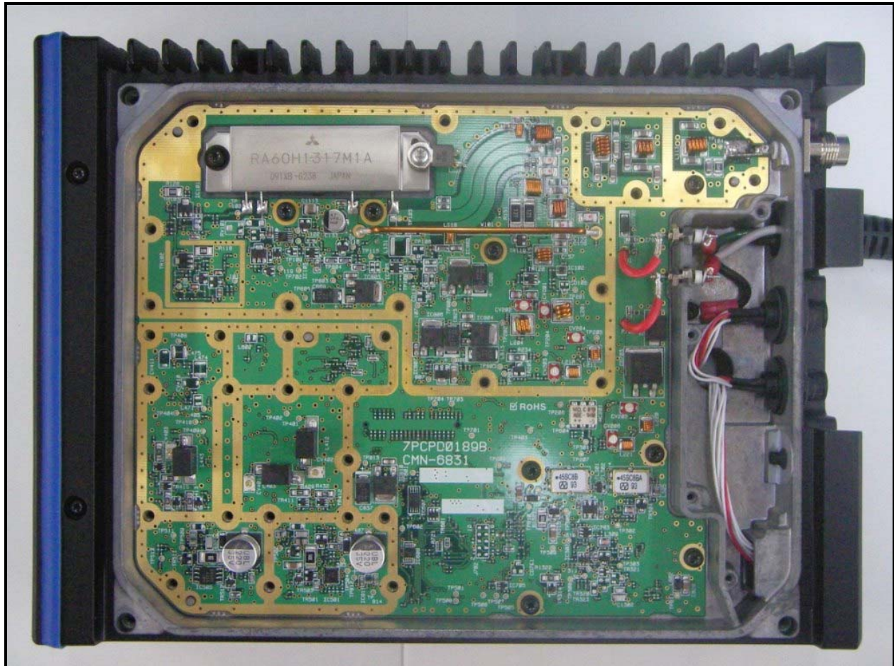
Photograph 22: Bottom Cover and Shield Removed
