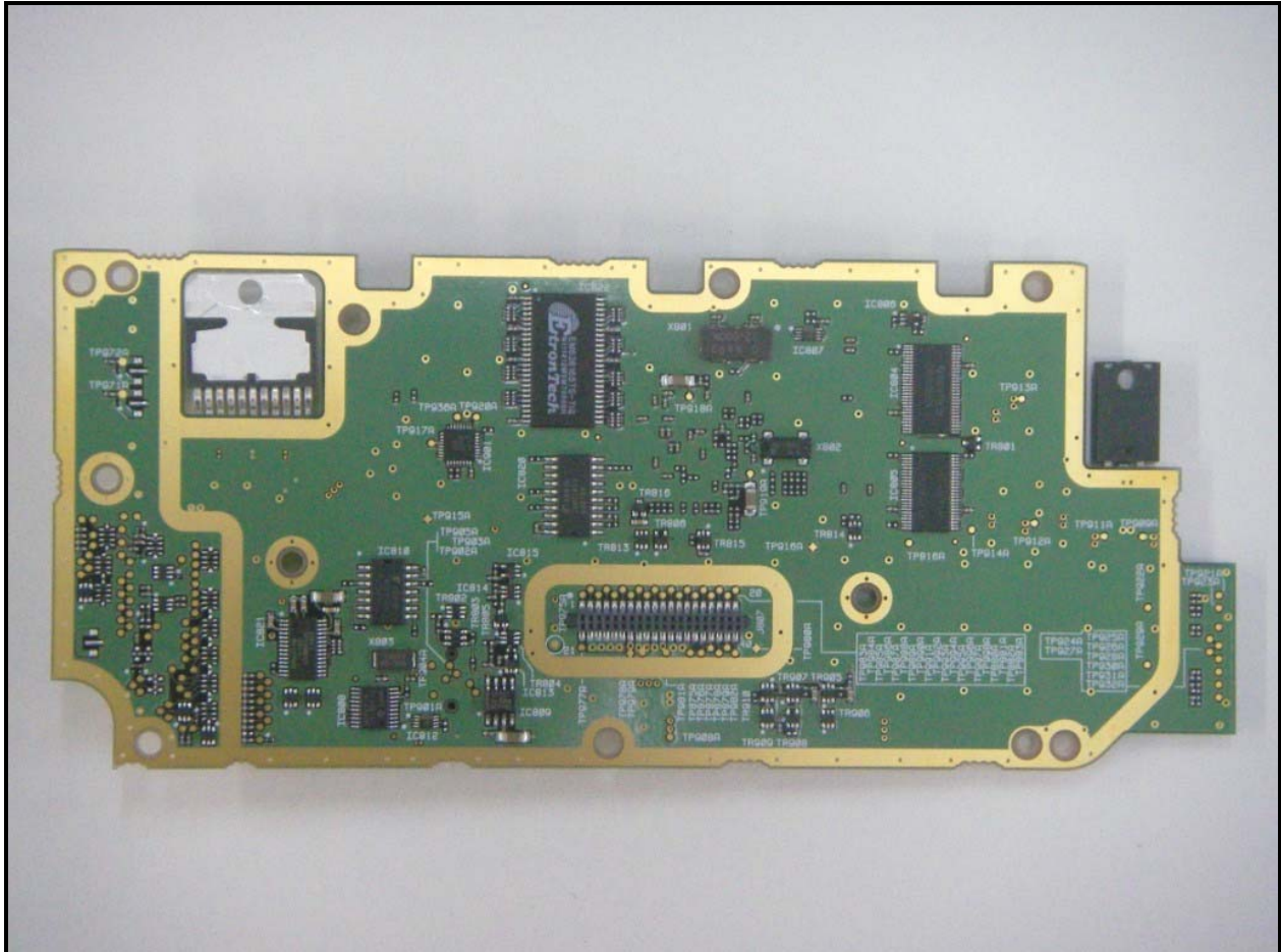
Photograph 26: PK Board Solder Side Complete
