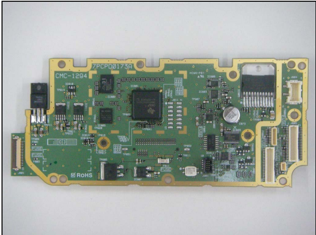
Photograph 23: PK Board Component Side Complete
