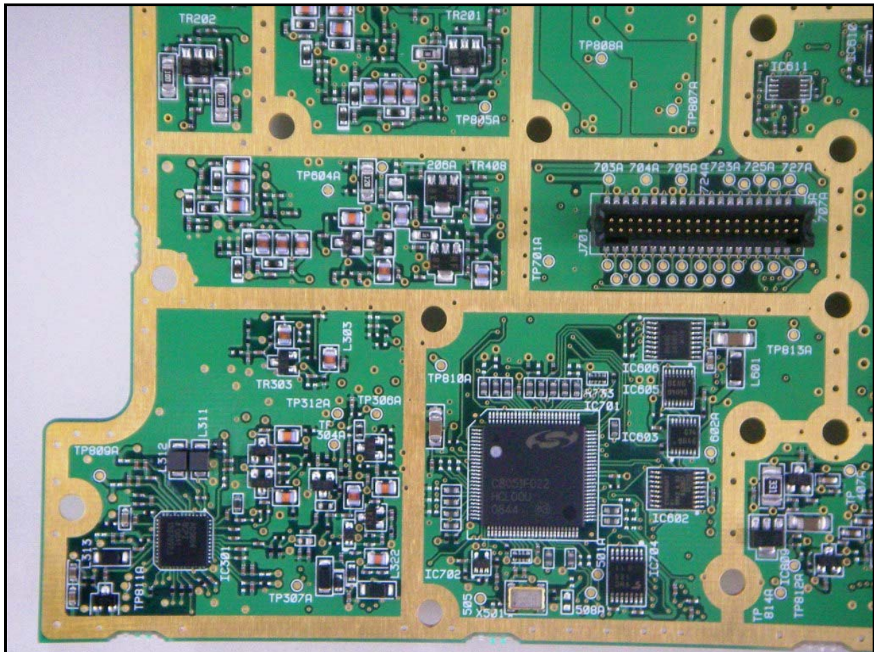
Photograph 34: RF Processor Board Solder Side Lower Left
