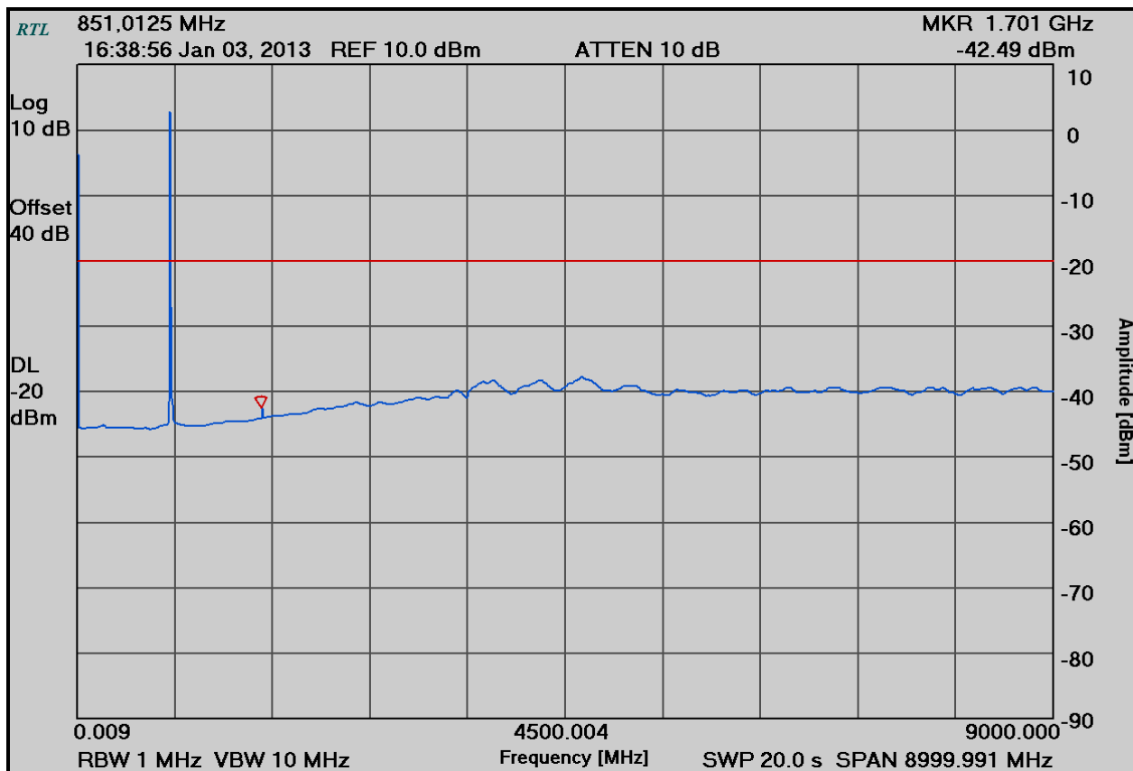
Plot 5-10: Conducted Spurious Emissions – H-CPM TDMA; 851.0125 MHz
