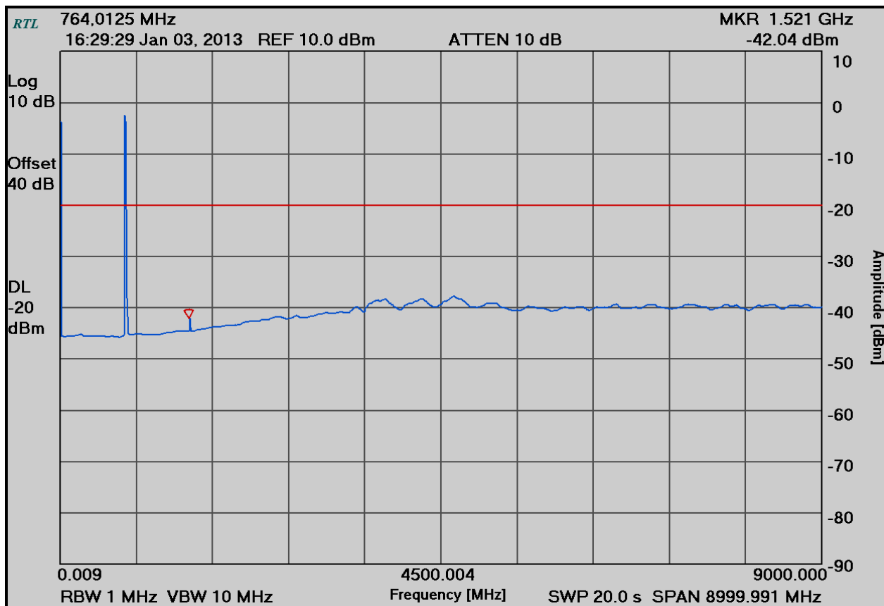
Plot 5-1: Conducted Spurious Emissions – H-CPM TDMA; 764.0125 MHz
