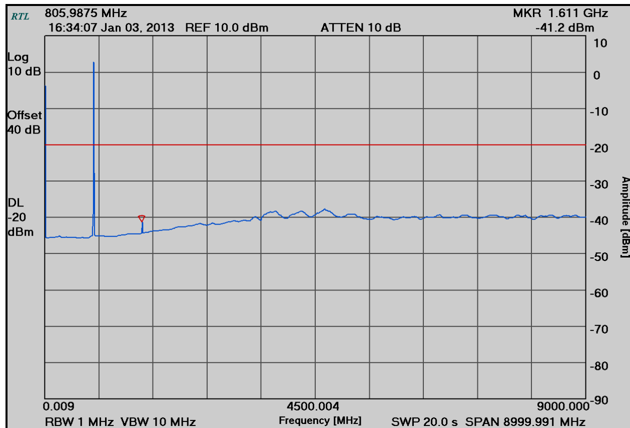
Plot 5-6: Conducted Spurious Emissions – H-CPM TDMA; 805.9875 MHz
