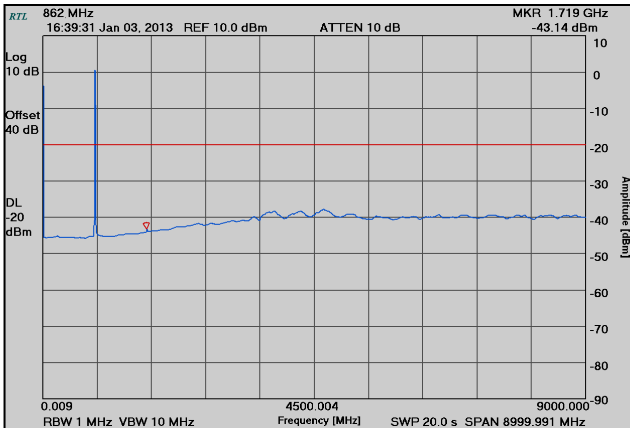
Plot 5-11: Conducted Spurious Emissions – H-CPM TDMA; 862.0000 MHz
