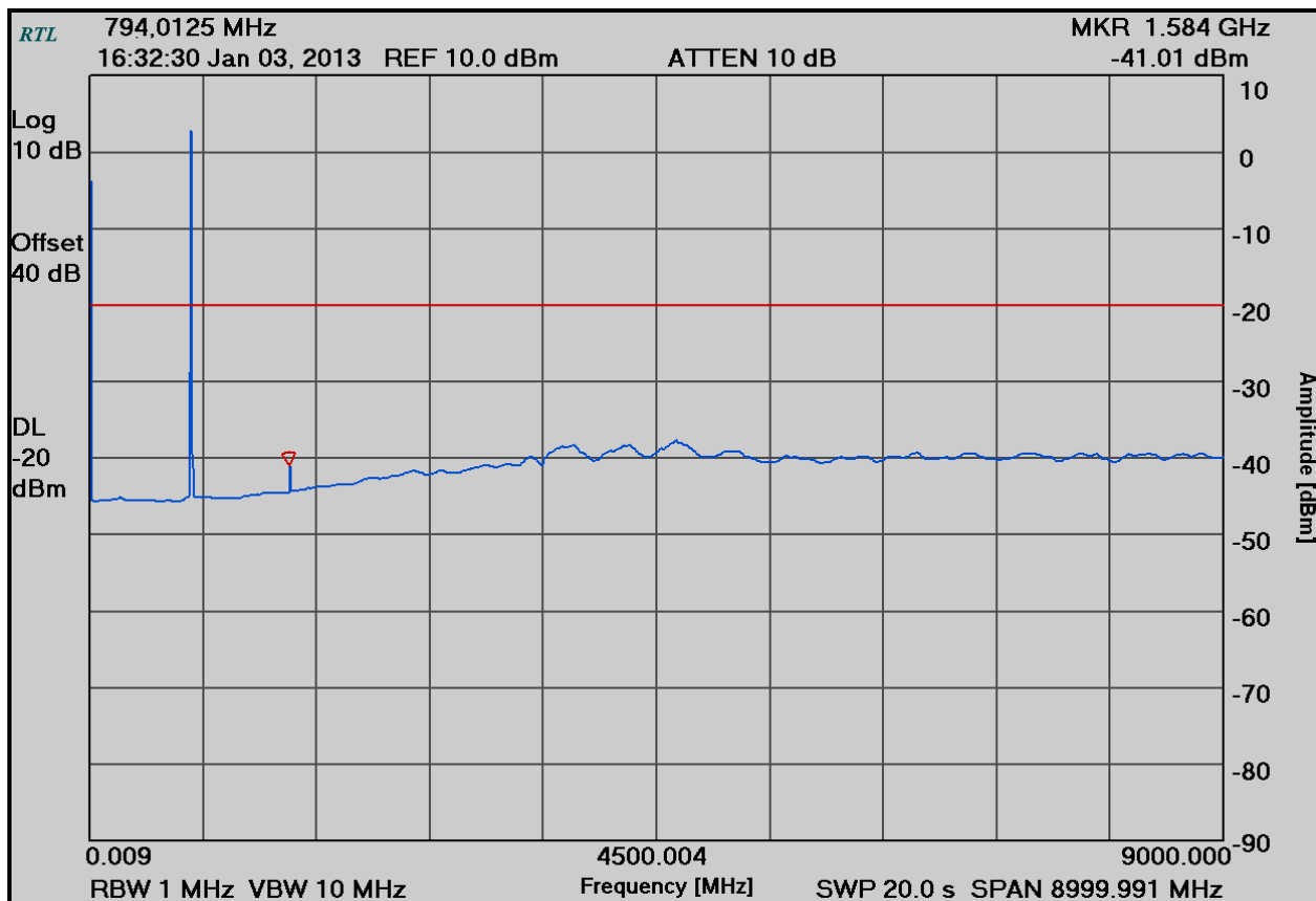
Plot 5-4: Conducted Spurious Emissions – H-CPM TDMA; 794.0125 MHz
