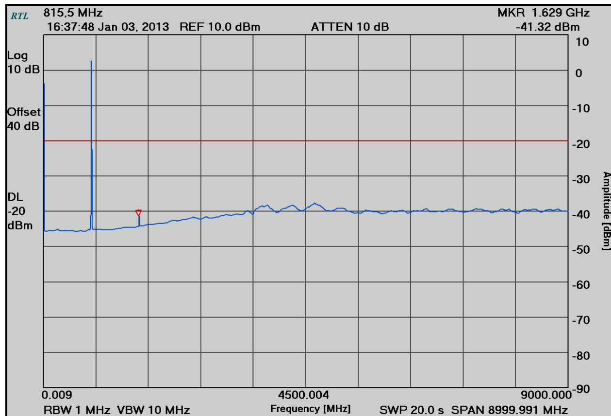
Plot 5-8: Conducted Spurious Emissions – H-CPM TDMA; 815.5000 MHz
