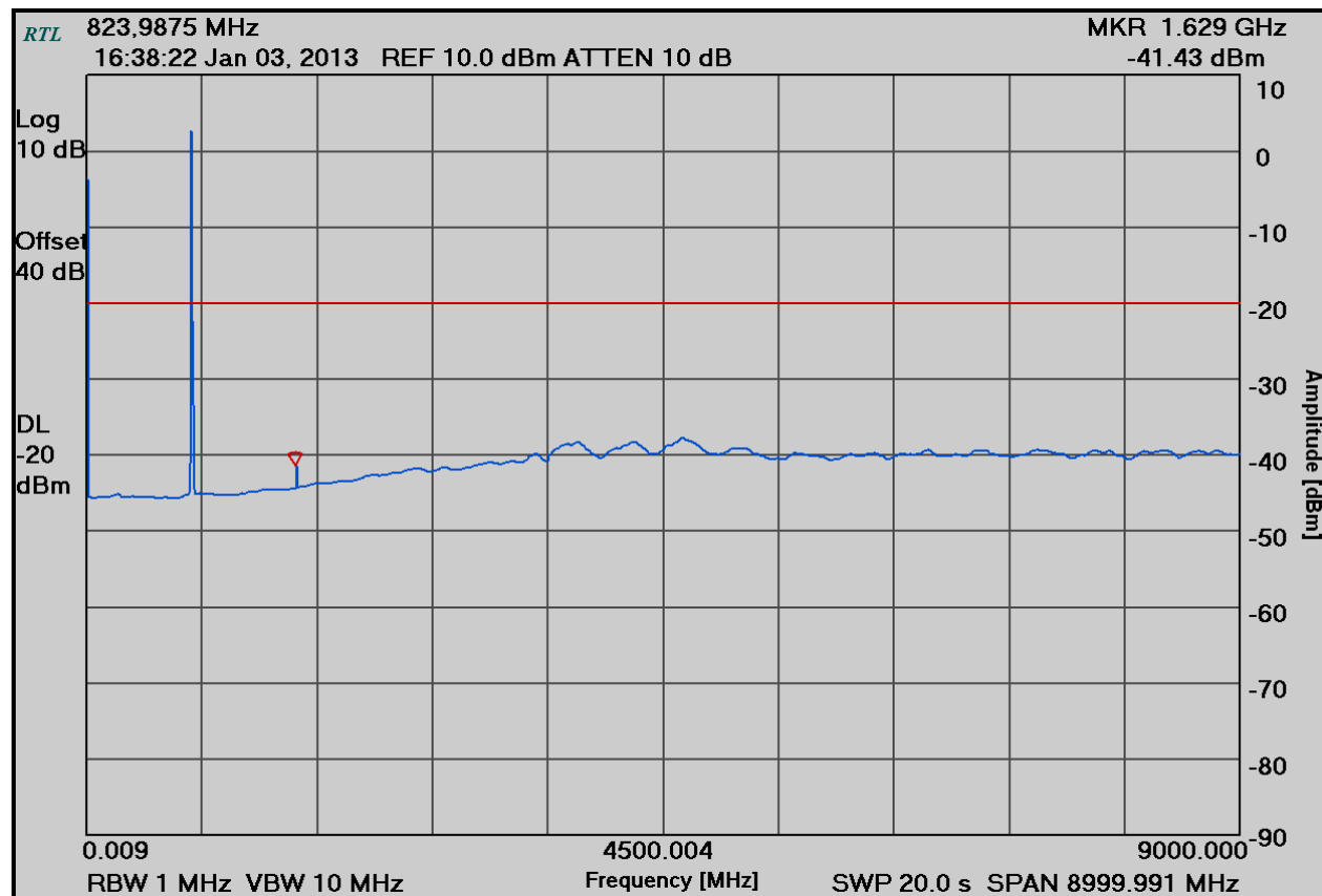
Plot 5-9: Conducted Spurious Emissions – H-CPM TDMA; 823.9875 MHz
