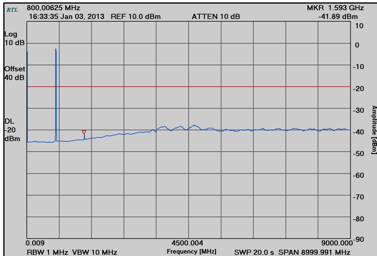
Plot 5-5: Conducted Spurious Emissions – H-CPM TDMA; 800.00625 MHz
