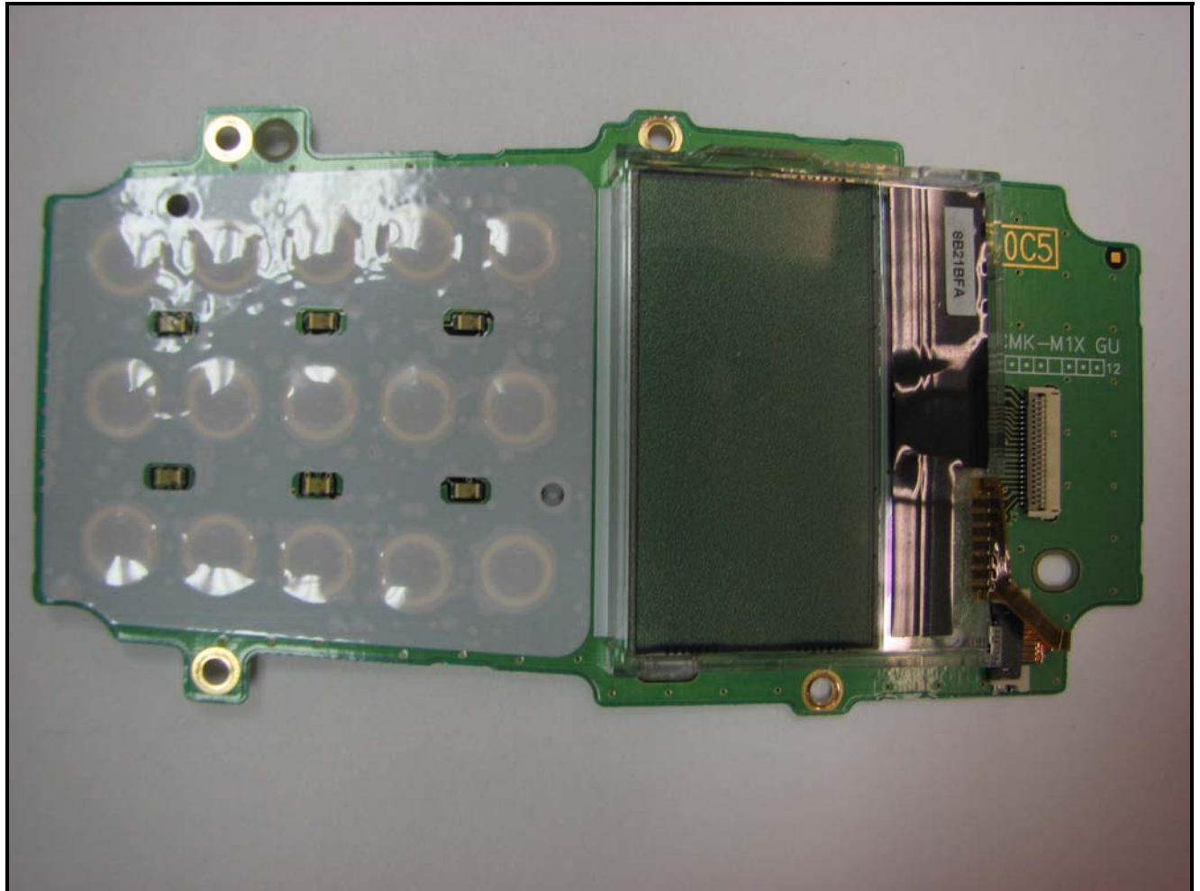
Photograph 16: Interface PWB LCD Side
