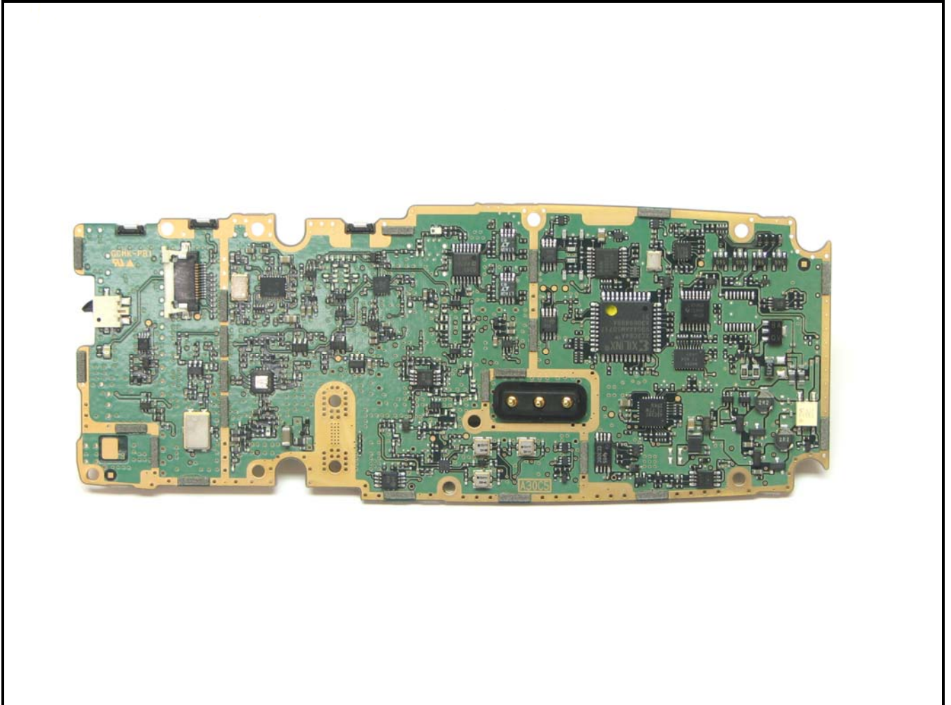
Photograph 13: Main PWB Side 1
