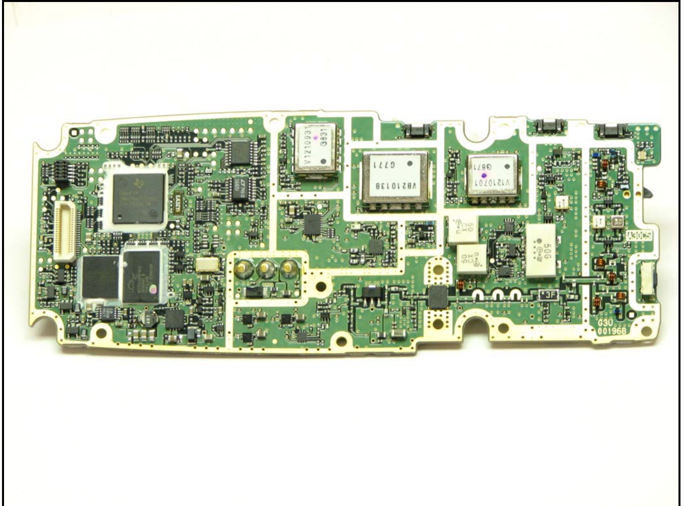
Photograph 14: Main PWB Side 2
