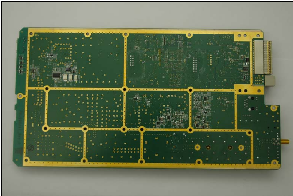
Photograph 12. Receiver Module Bottom
