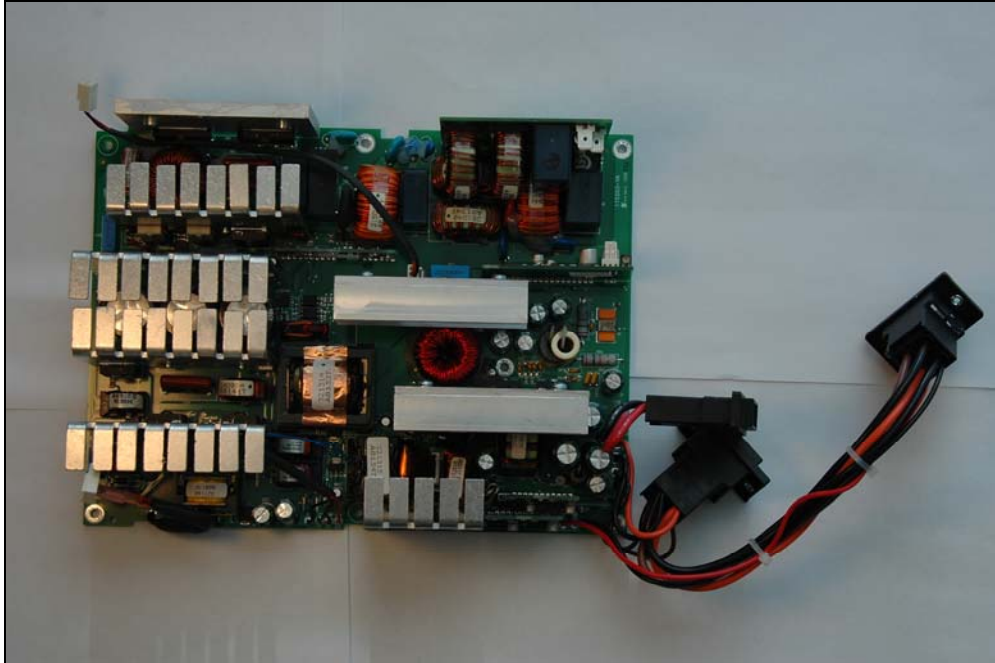
Photograph 11. Power Supply Top
