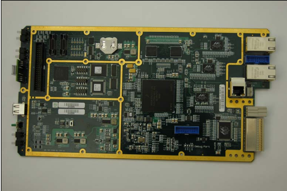
Photograph 15. Traffic Controller Top
