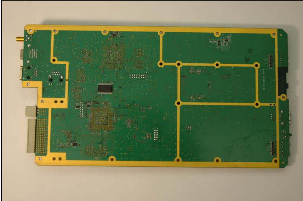
Photograph 3. Baseband Module Bottom
