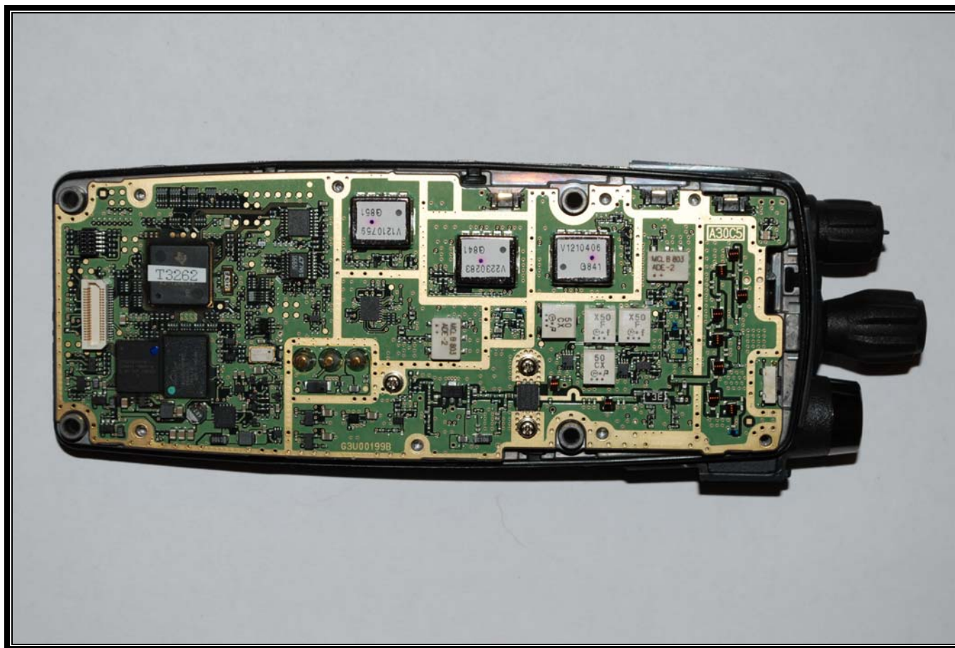
Photograph 12: P7300 Main PWB in Unit
