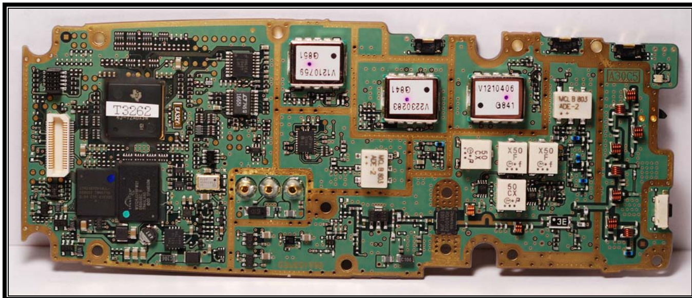
Photograph 13: P7300 Main PWB Front View
