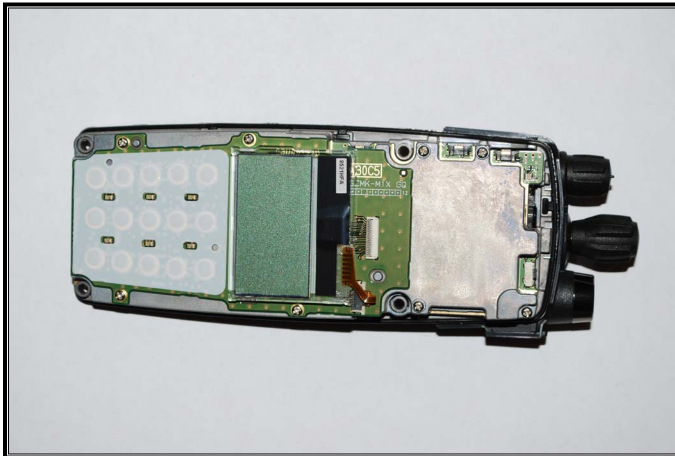
Photograph 15: P7300 Interface PWB in Unit
