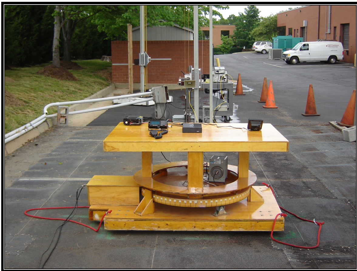
Photograph 6: Radiated Spurious Emissions – Front View
