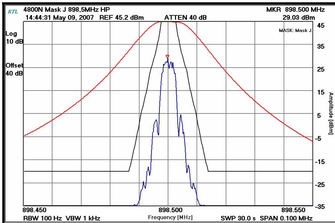
Plot 7-5: Occupied Bandwidth – 898.500 MHz; Mask J; 2-level FSK; 4800 BPS
