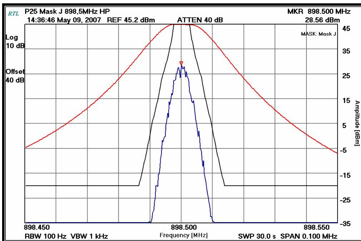
Plot 7-7: Occupied Bandwidth – 898.500 MHz; Mask J; 4-level FSK (P25 mode); 4800 SPS
