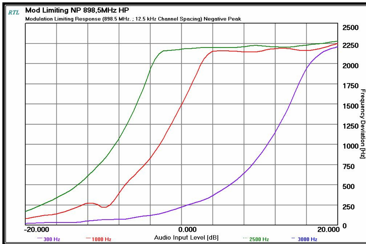
Plot 11-2: Modulation Characteristics – Modulation Limiting: 898.500 MHz; Narrow Band; Negative Peak
