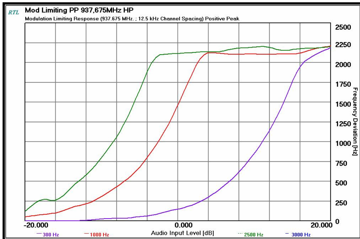
Plot 11-3: Modulation Characteristics – Modulation Limiting: 937.675 MHz; Narrow Band; Positive Peak
