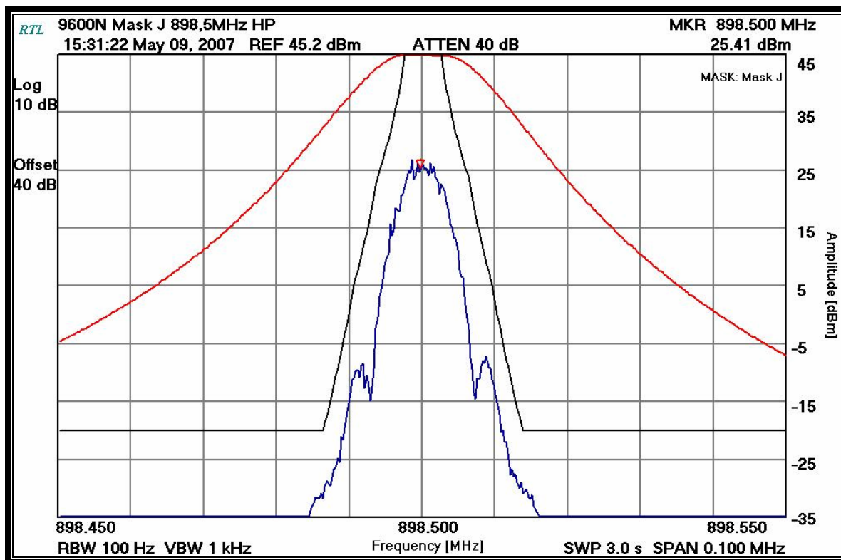
Plot 7-3: Occupied Bandwidth – 898.500 MHz; Mask J; 2-level FSK; 9600 BPS
