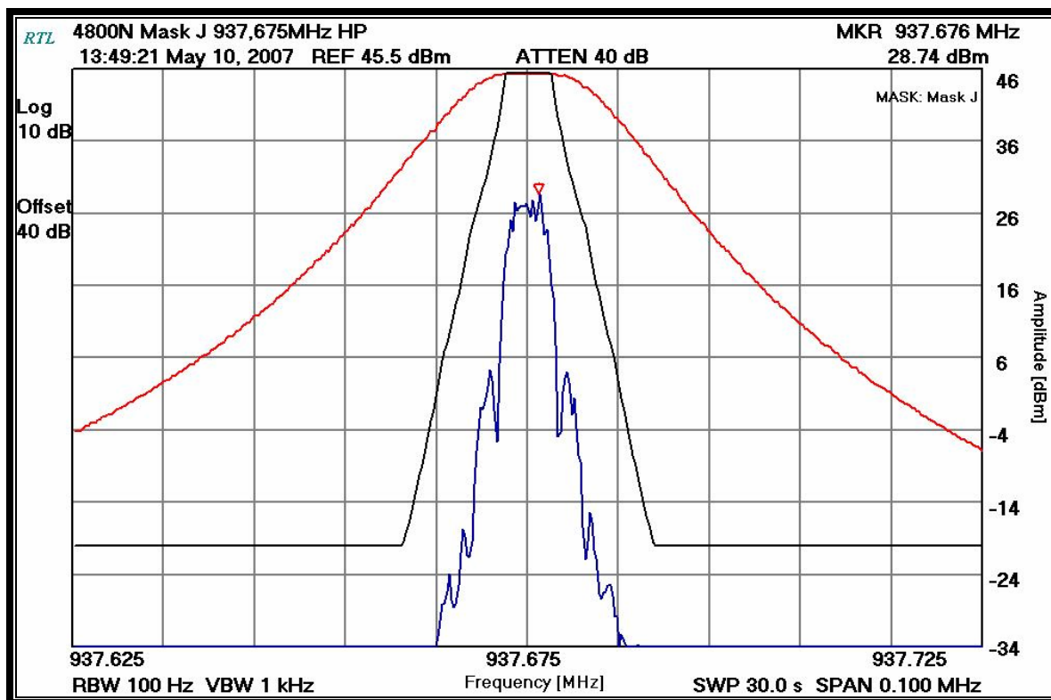
Plot 7-6: Occupied Bandwidth – 937.675 MHz; Mask J; 2-level FSK; 4800 BPS
