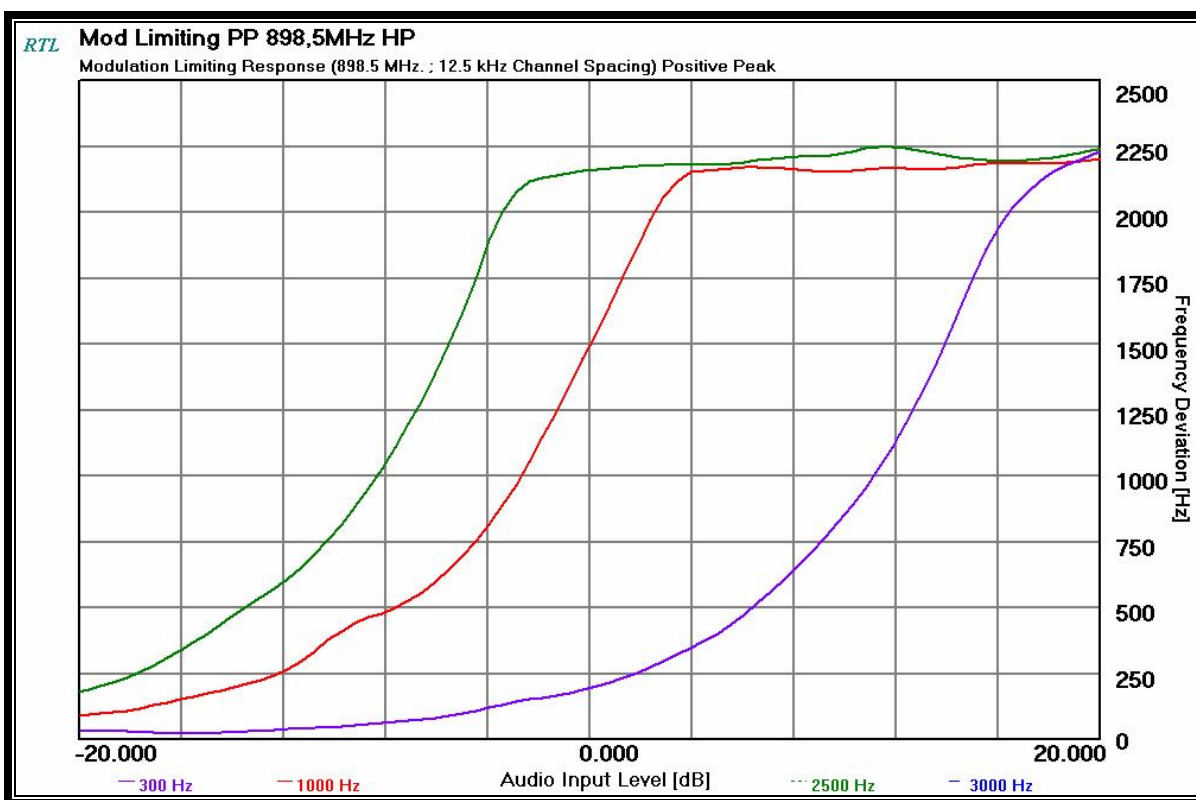
Plot 11-1: Modulation Characteristics – Modulation Limiting: 898.500 MHz; Narrow Band; Positive Peak
