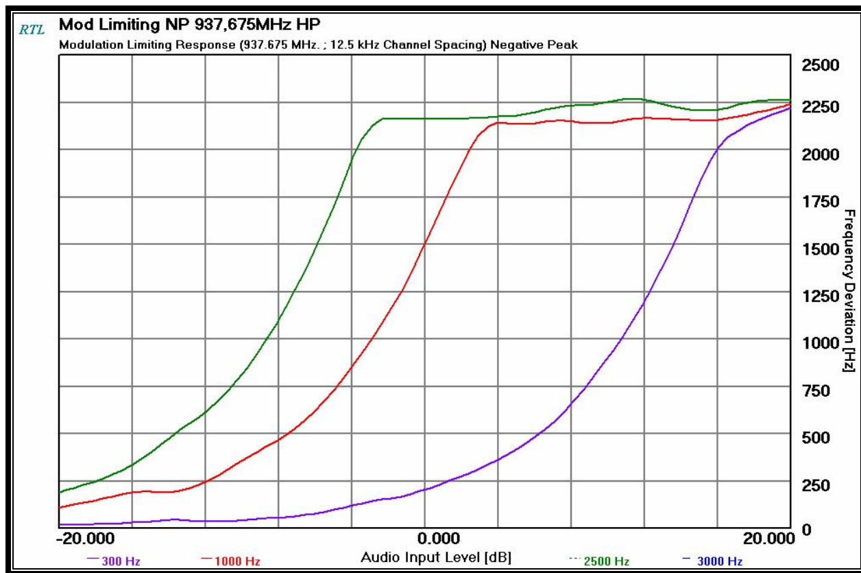
Plot 11-4: Modulation Characteristics – Modulation Limiting: 937.675 MHz; Narrow Band; Negative Peak
