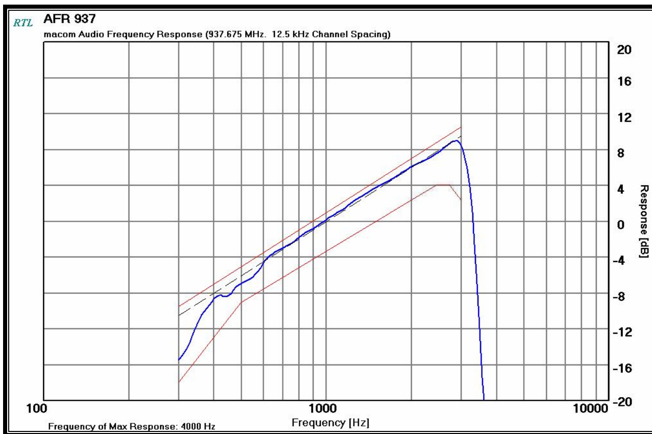
Plot 9-2: Modulation Characteristics - Audio Frequency Response; 937.675 MHz
