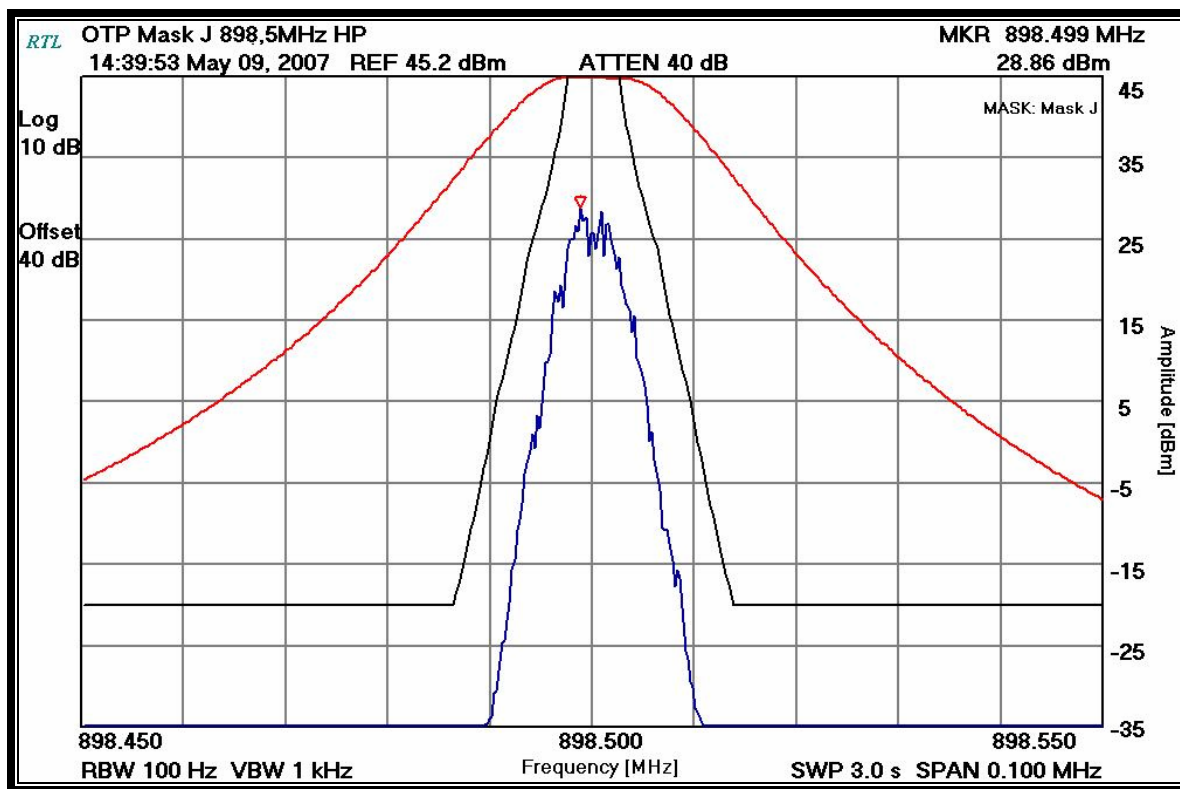
Plot 7-9: Occupied Bandwidth – 898.500 MHz; Mask J; 4-level FSK (NB OTP mode); 4800 SPS
