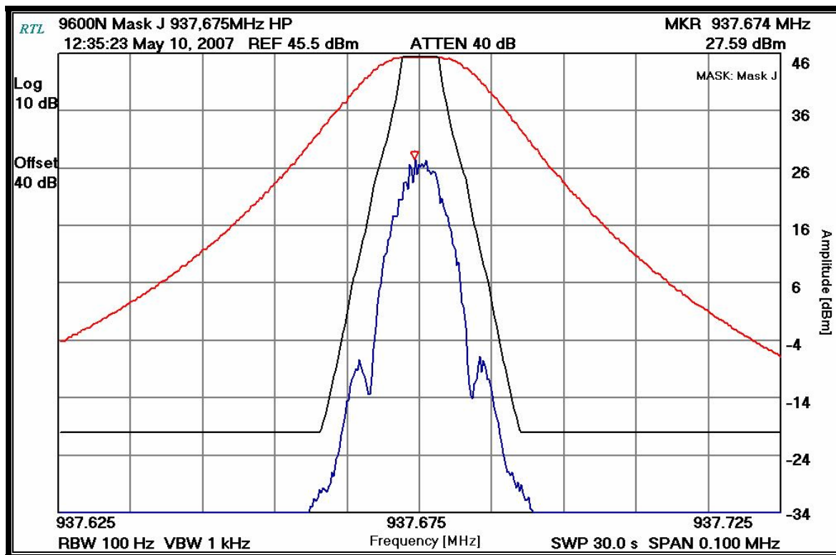
Plot 7-4: Occupied Bandwidth – 937.675 MHz; Mask J; 2-level FSK; 9600 BPS
