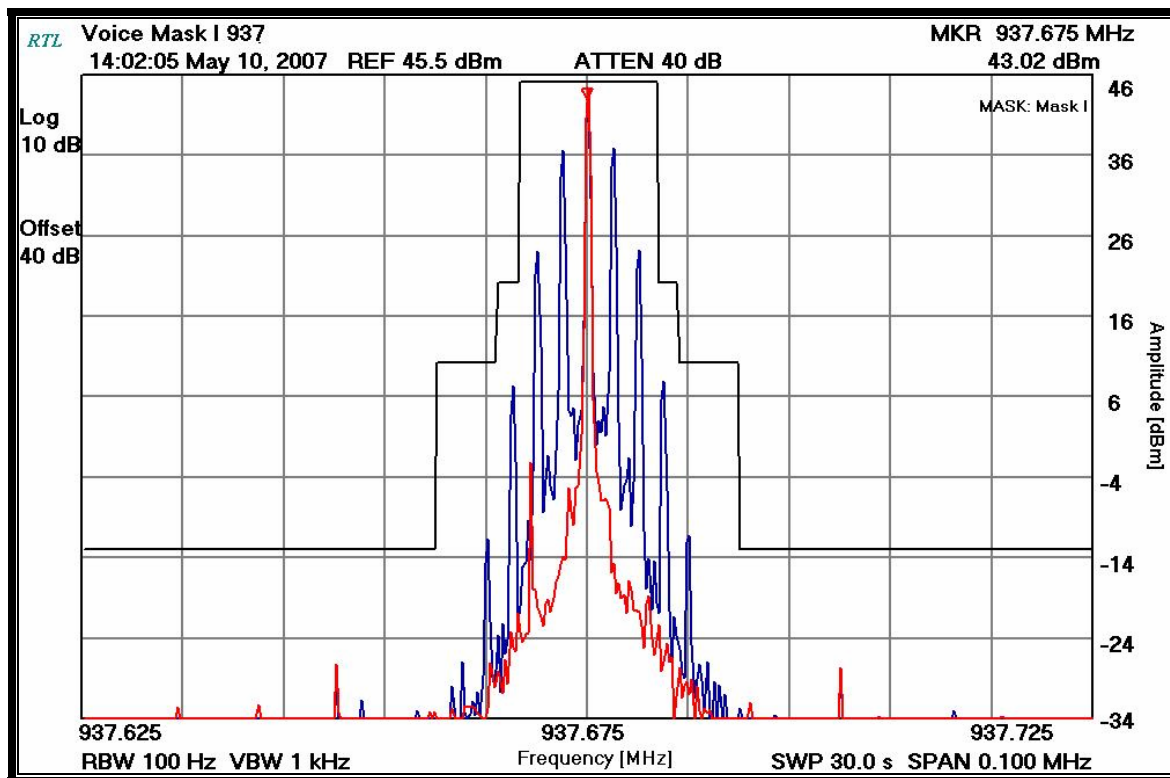
Plot 7-2: Occupied Bandwidth – 937.675 MHz; Mask I; Analog; High Power
