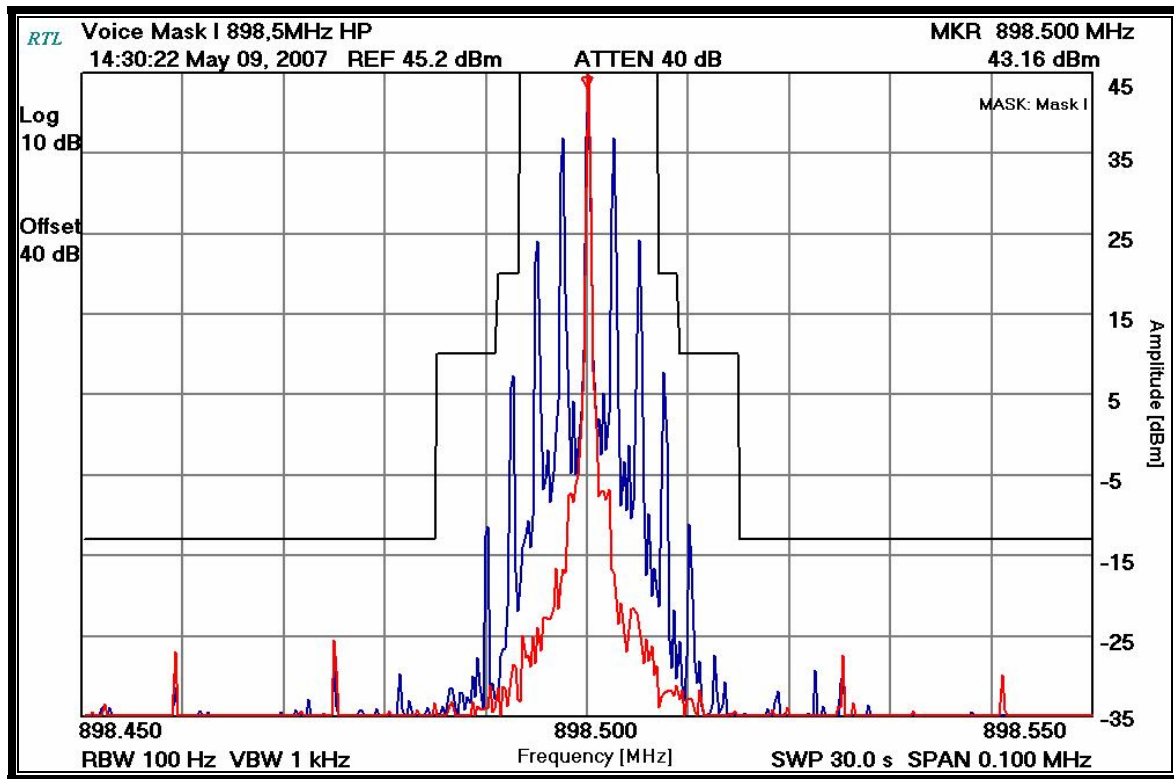
Plot 7-1: Occupied Bandwidth – 898.500 MHz; Mask I; Analog; High Power
