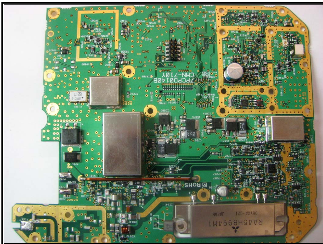
Photograph 13: RF Board Top View
