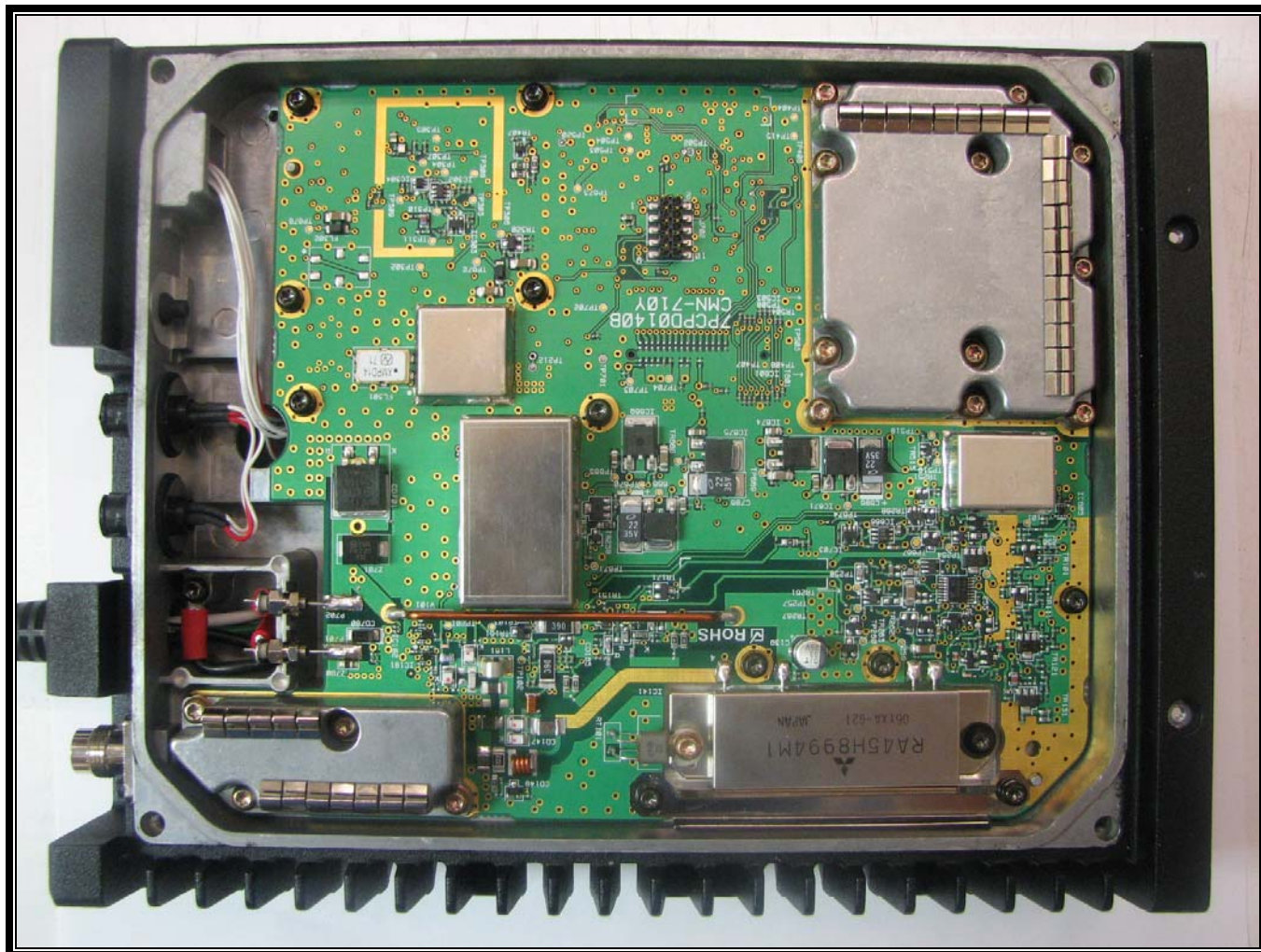
Photograph 12: Bottom View without Cover
