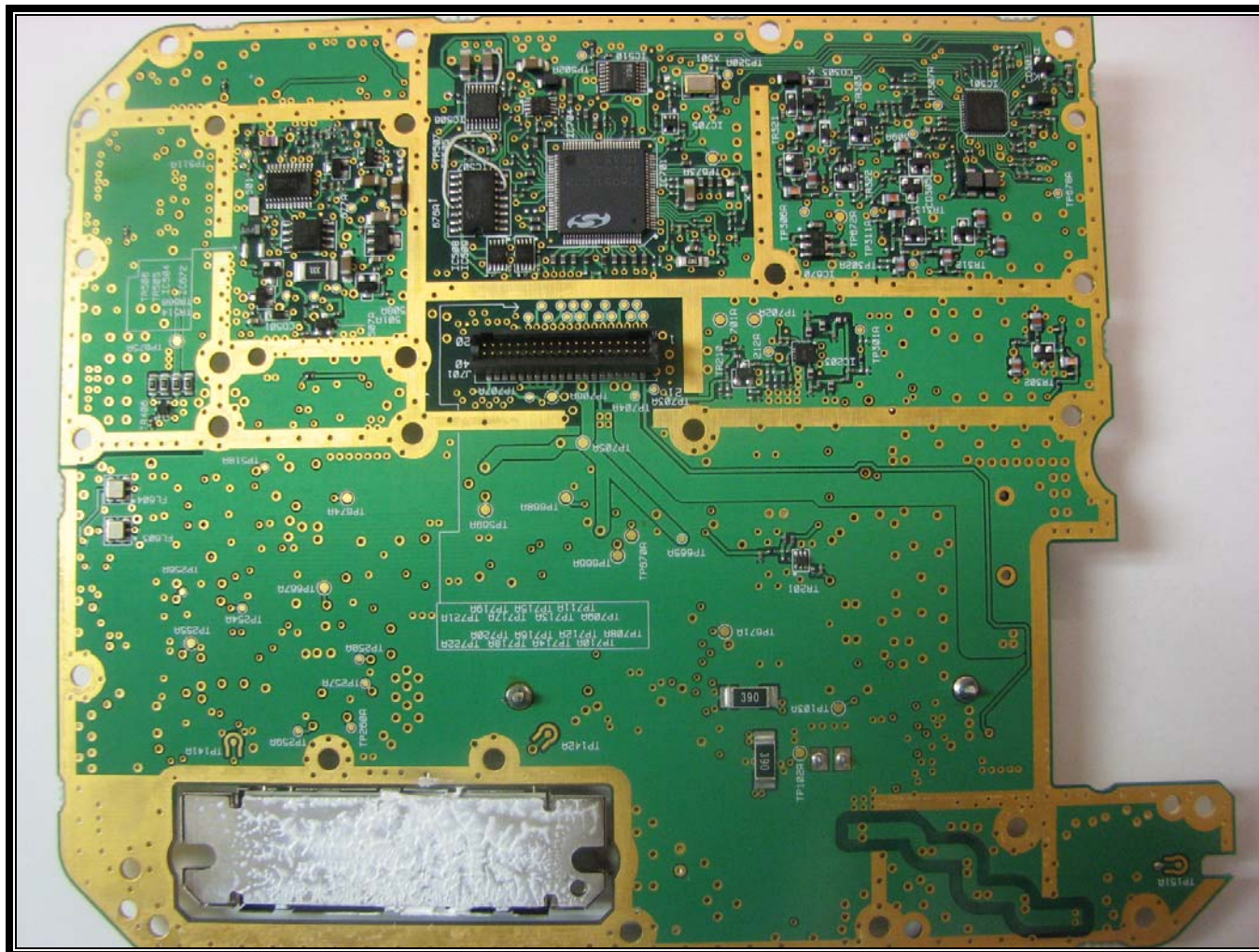
Photograph 14: RF Board Bottom View
