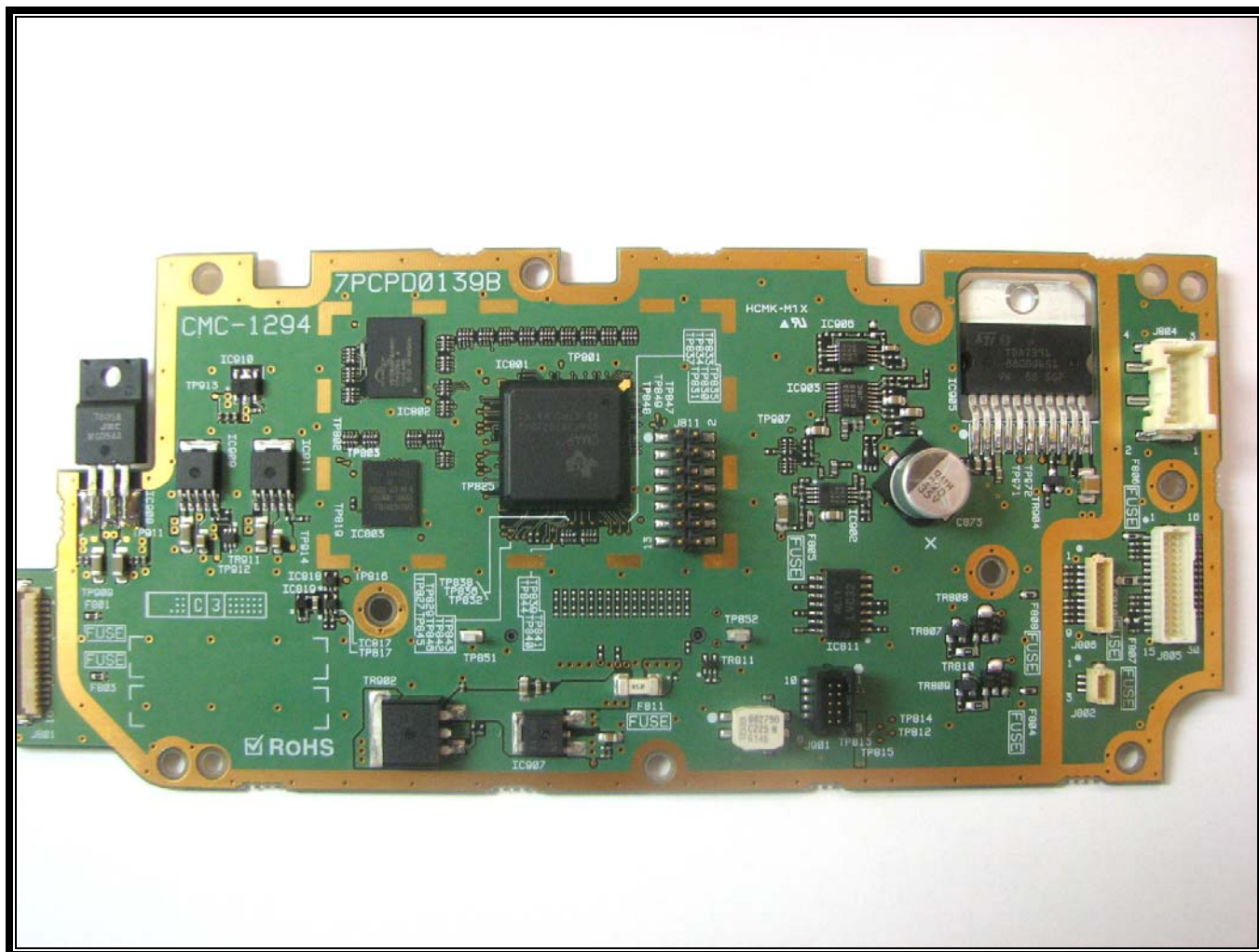
Photograph 15: Controller Board Top View
