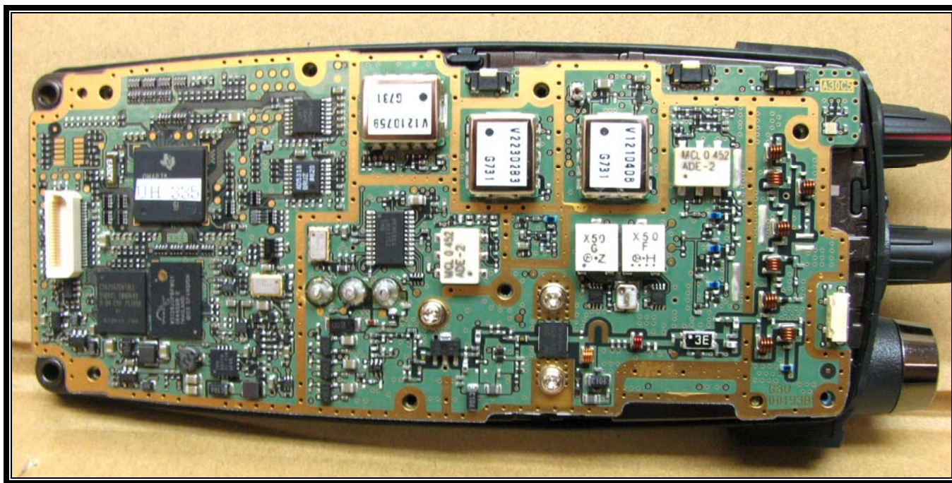
Photograph 15: Main Board in Radio
