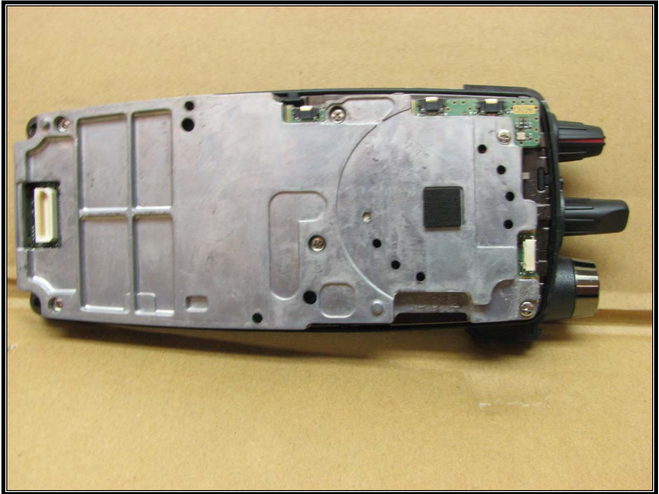
Photograph 12: RF Shield on Radio
