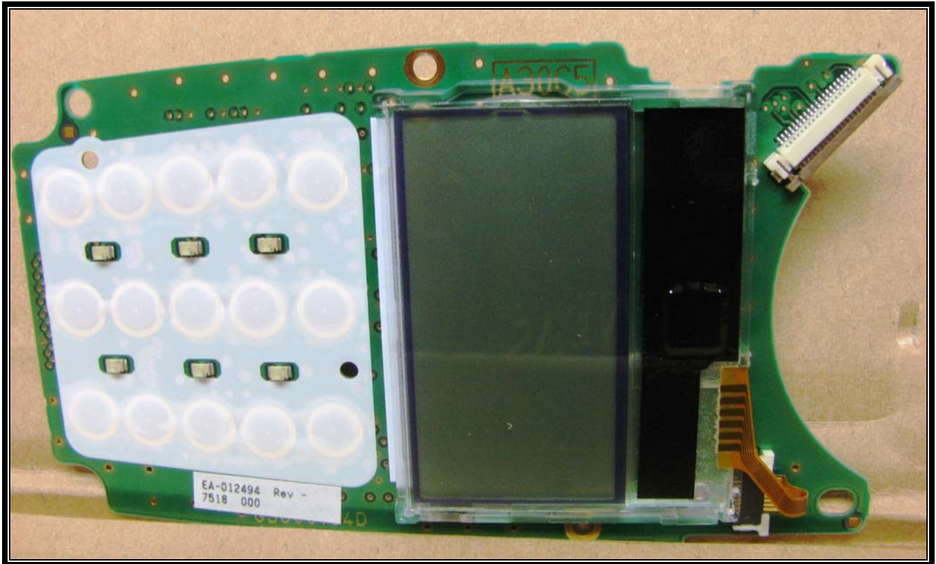
Photograph 19: Interface Board Top View
