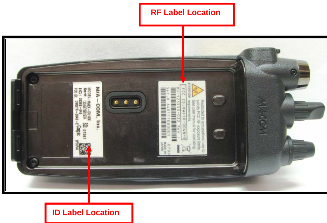
Photograph 1: ID Label and RF Label Locations
