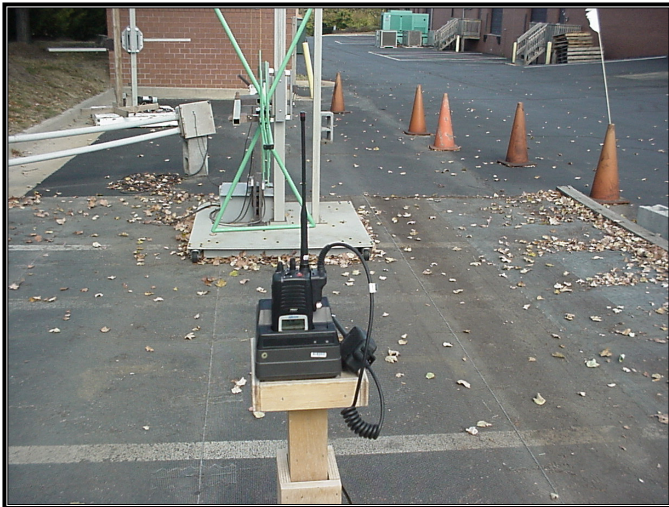
Photograph 3: Radiated TX Spurious Emissions – Front View
