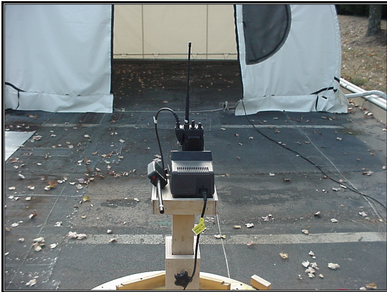
Photograph 4: Radiated TX Spurious Emissions – Rear View
