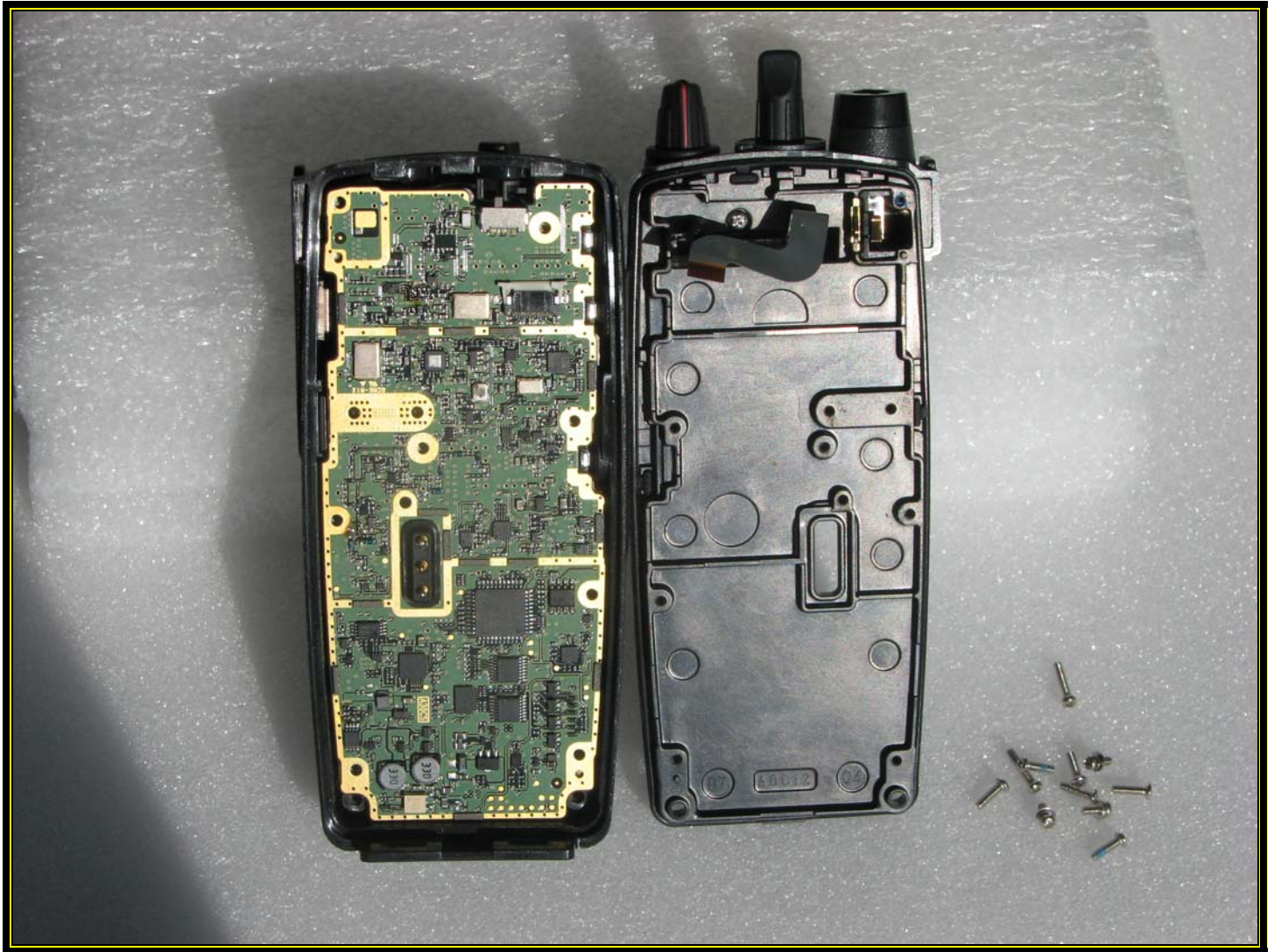
Photograph 13: Board Placement Layer 4
