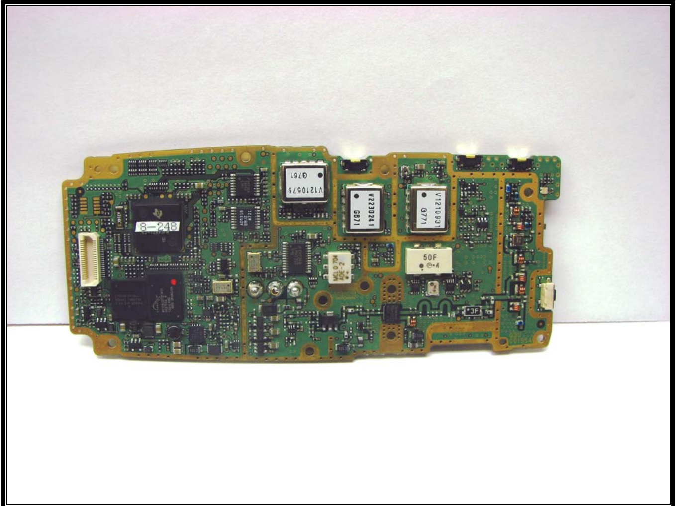
Photograph 16: Main Board Top View
