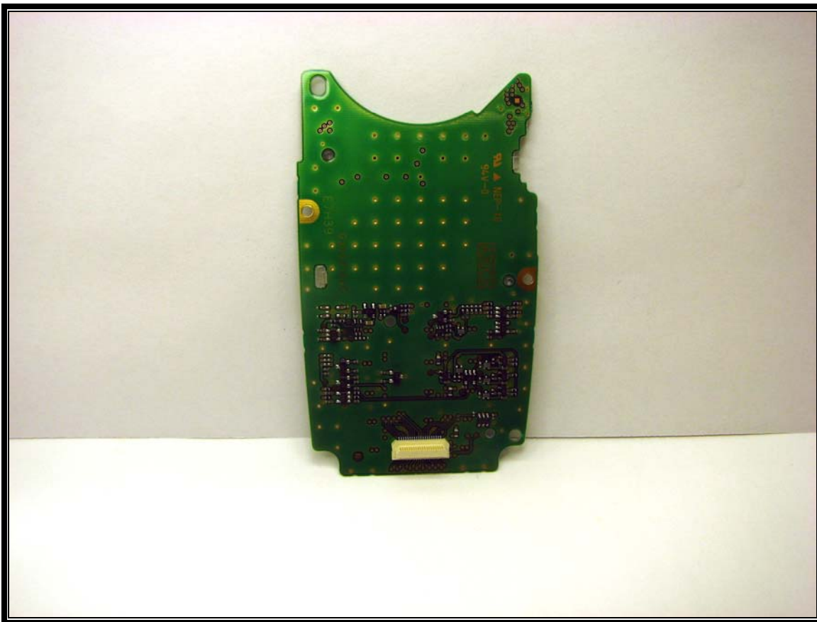
Photograph 20: Interface Board Bottom View
