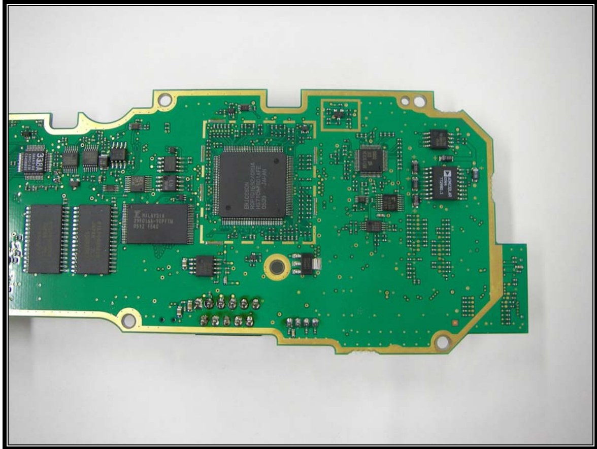
Photograph 22: Audio Logic Board Solder Side Right Side
