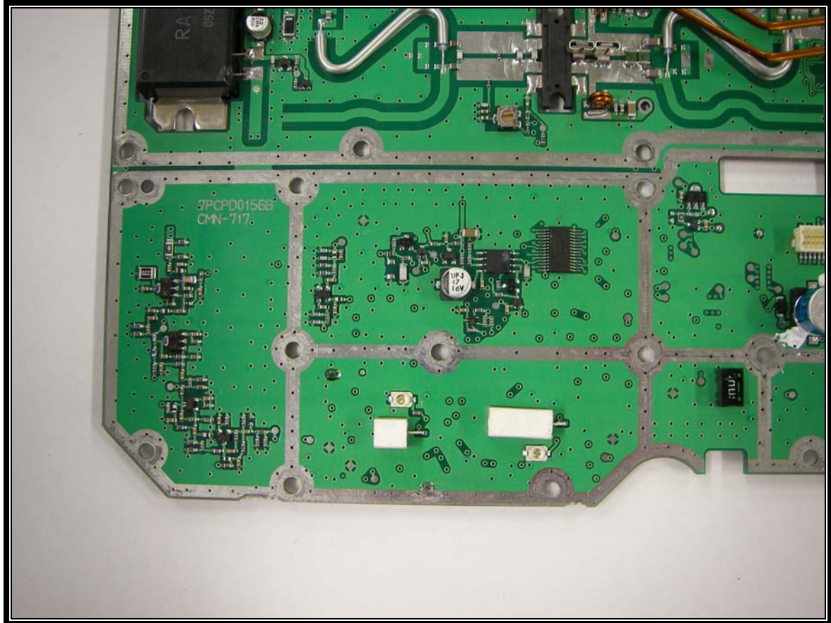
Photograph 26: TRX Syn Board Component Side Lower Left
