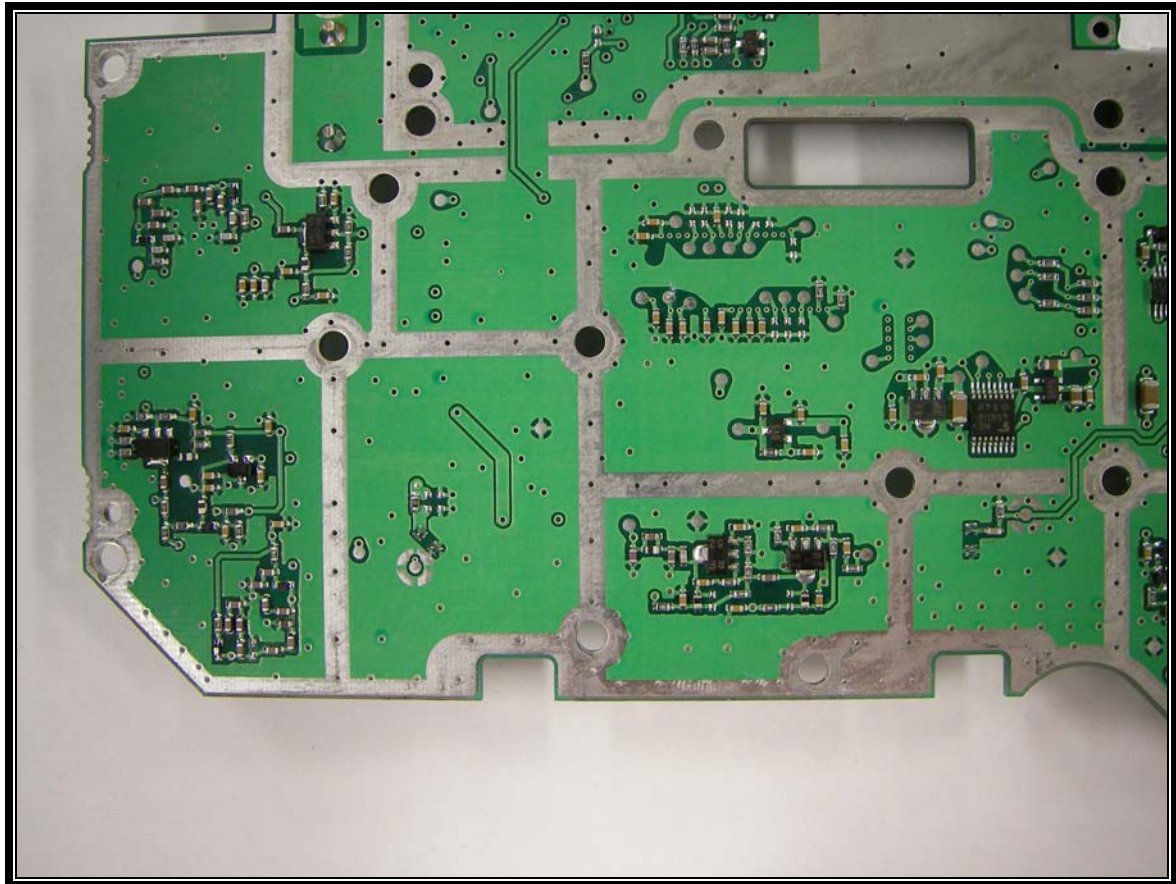
Photograph 31: TRX Syn Board Solder Side Lower Left
