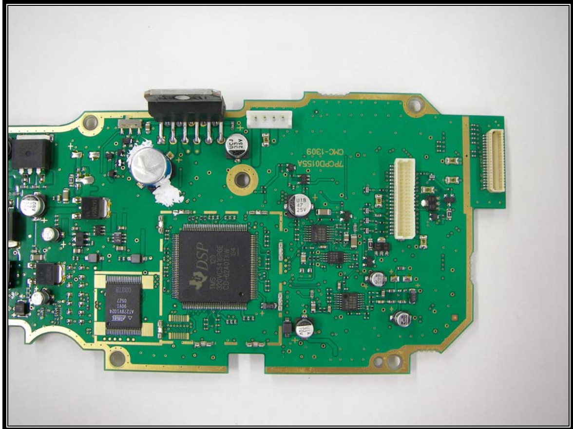
Photograph 19: Audio Logic Board Component Side Right
