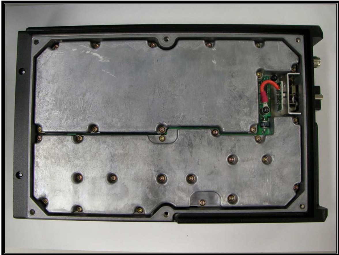
Photograph 15: Bottom Cover and Shield Removed
