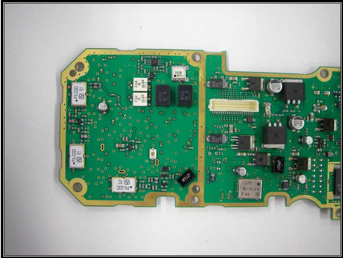
Photograph 18: Audio Logic Board Component Side Left
