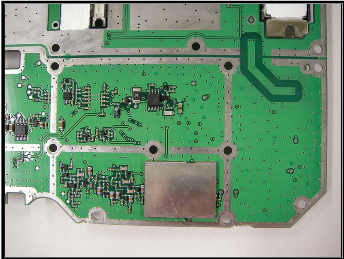
Photograph 32: TRX Syn Board Solder Side Lower Right
