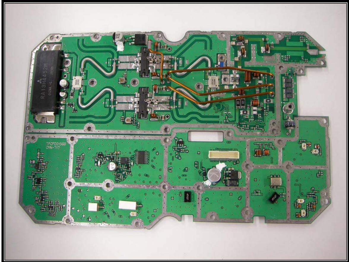
Photograph 23: TRX Syn Board Component Side Complete View
