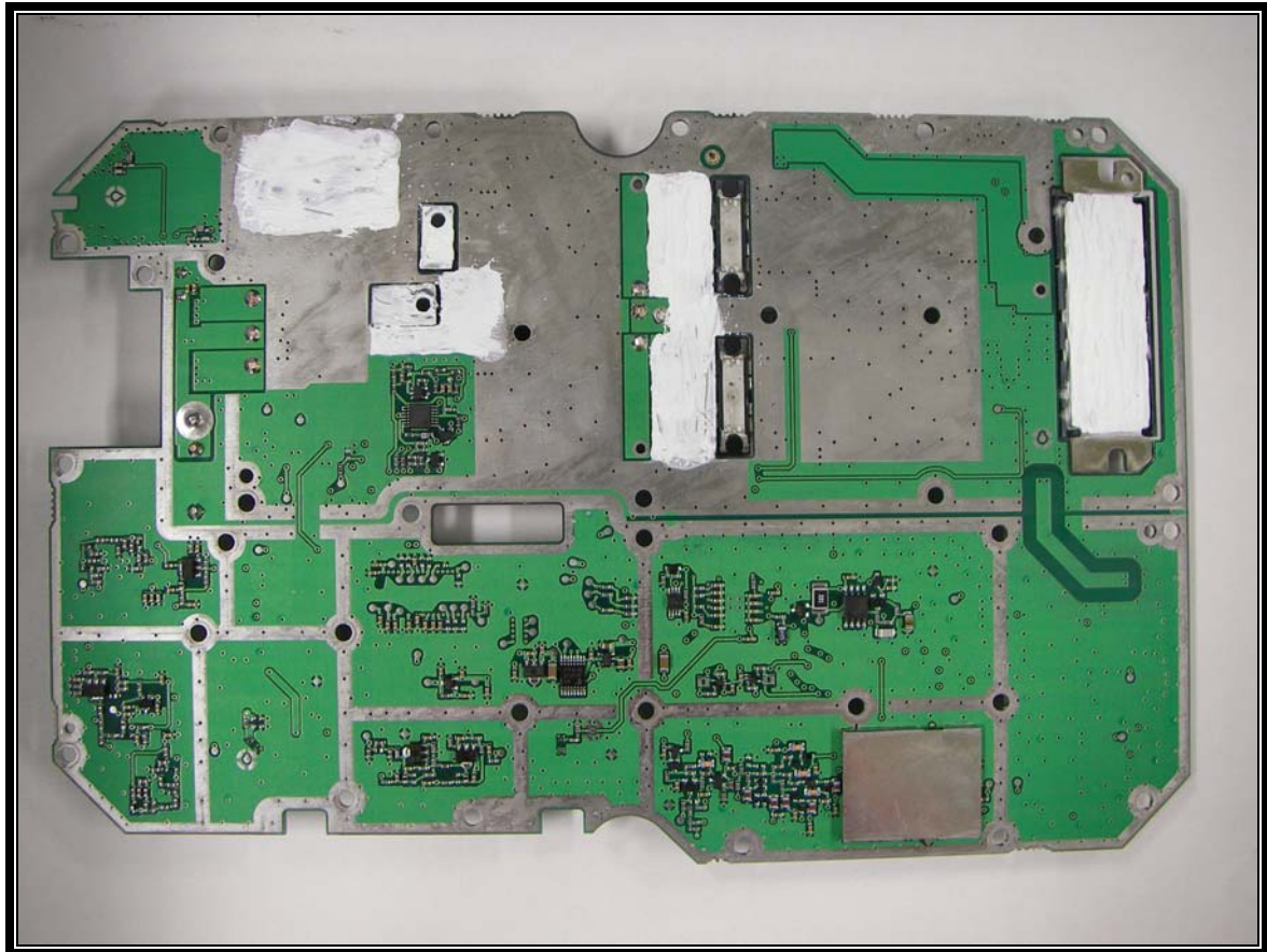
Photograph 28: TRX Syn Board Solder Side Complete View
