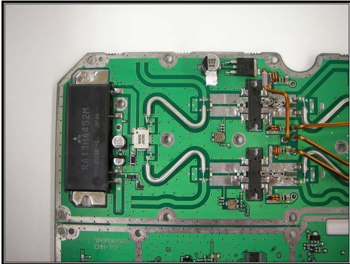
Photograph 24: TRX Syn Board Component Side Upper Left
