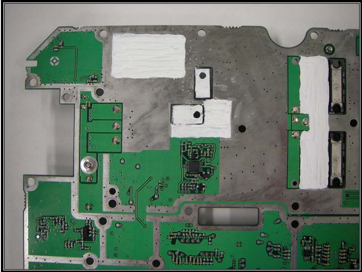
Photograph 29: TRX Syn Board Solder Side Upper Left
