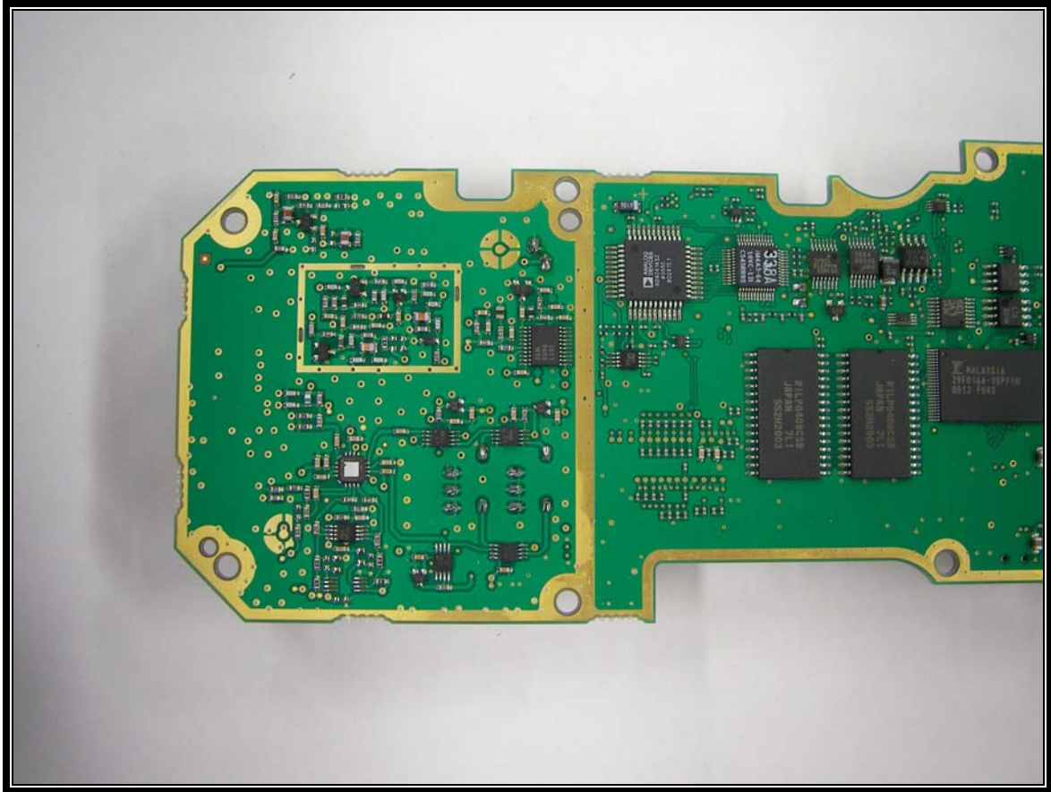
Photograph 21: Audio Logic Board Solder Side Left Side
