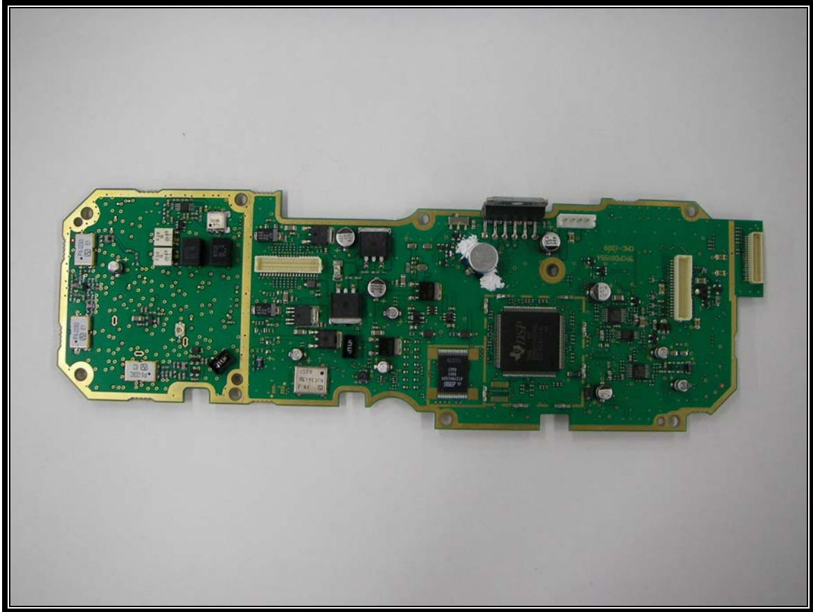
Photograph 17: Audio Logic Board Component Side Complete View
