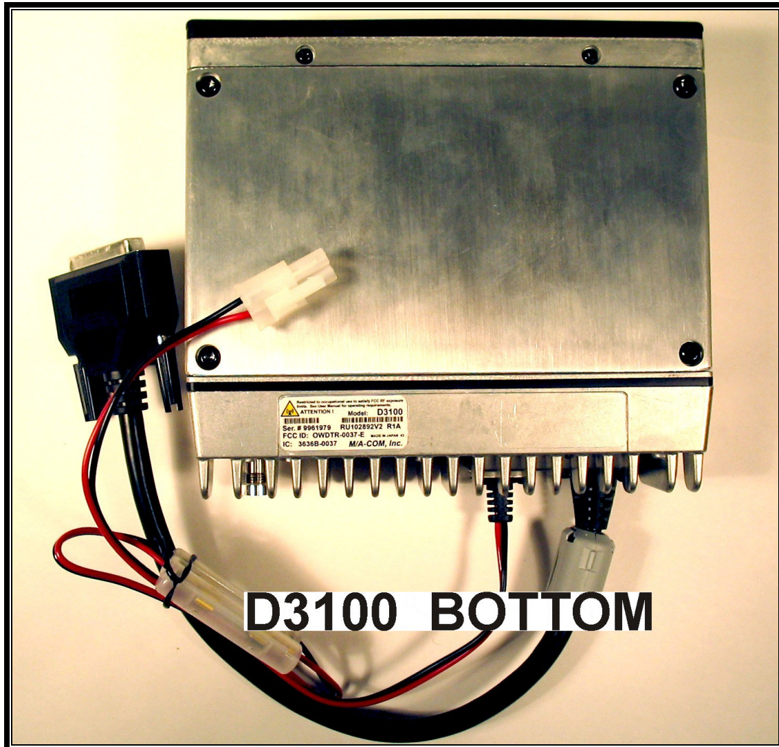
PHOTOGRAPH 6: D3100 BOTTOM VIEW
