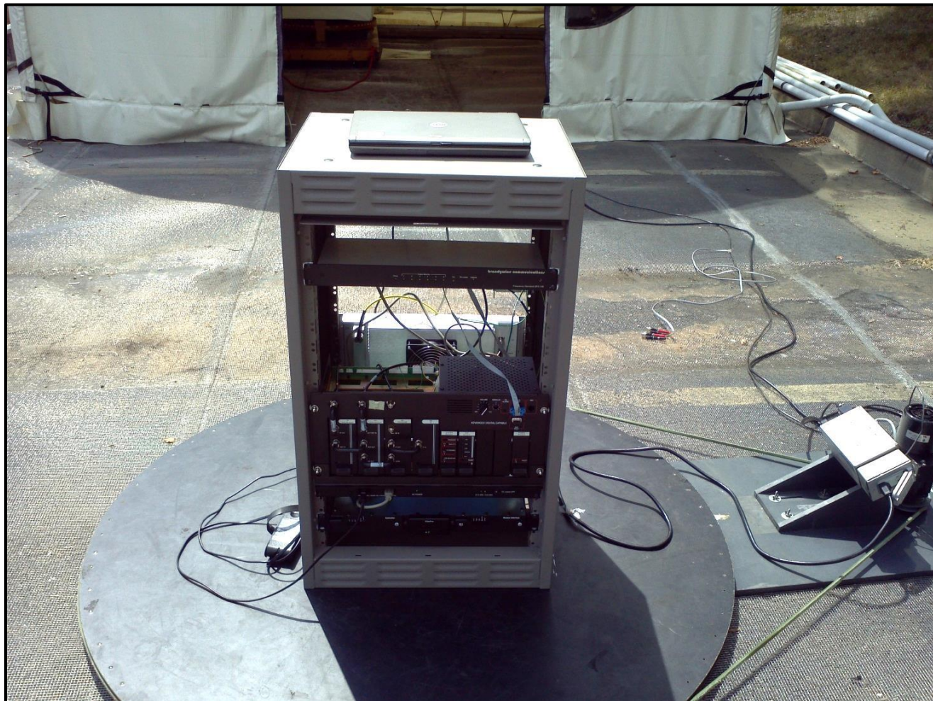
Photograph 4: Radiated Emissions (Front View)
