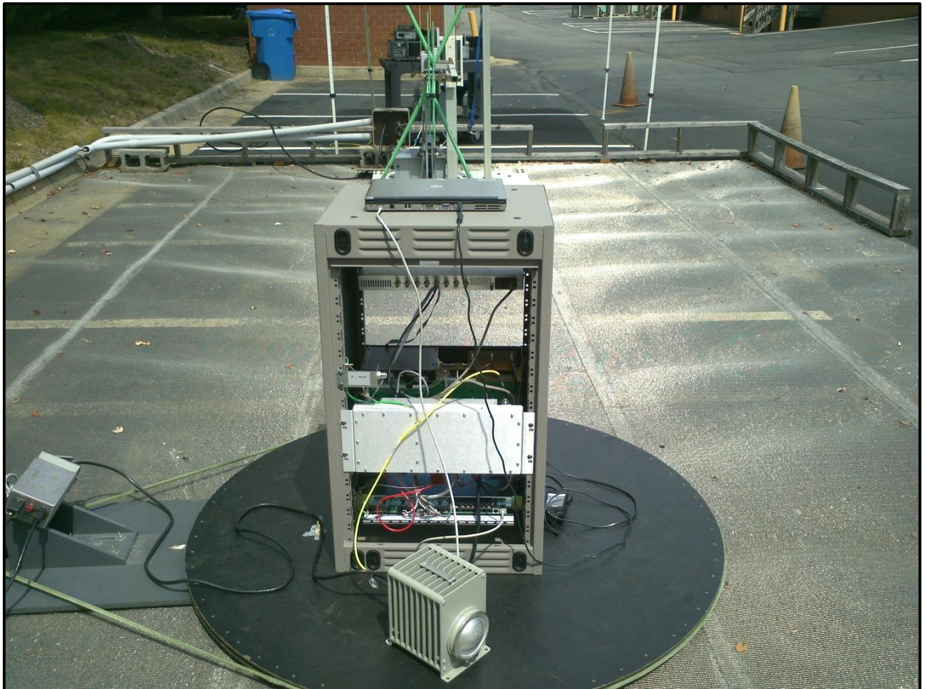
Photograph 5: Radiated Emissions (Rear View)
