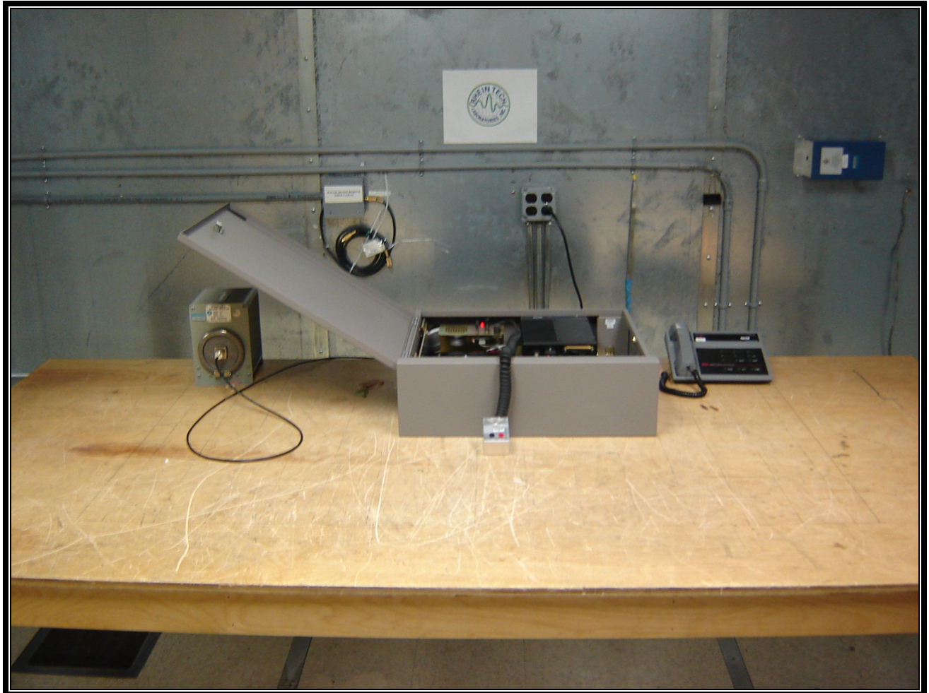
Photograph 5: Conducted Emissions (Front View) Wall Mount Configuration
