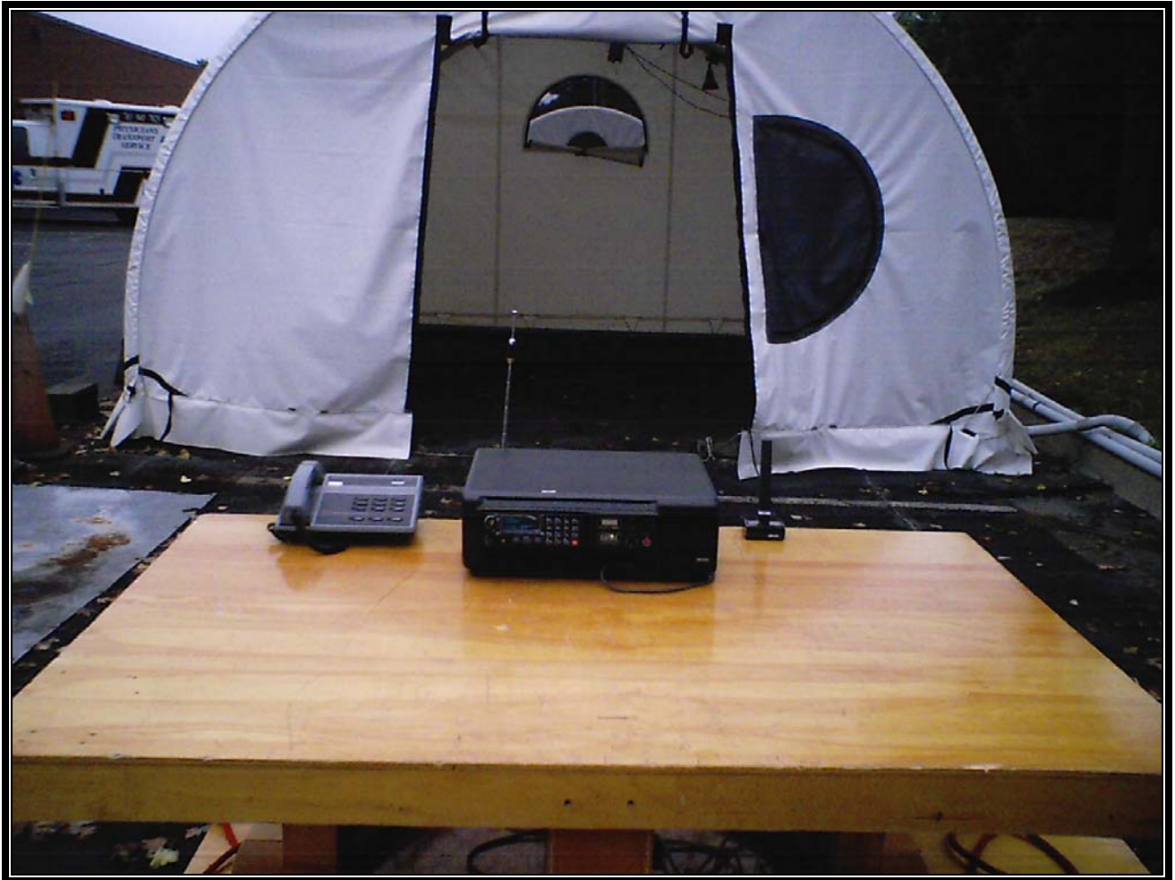
Photograph 3: Radiated Emissions (Front View) Desktop Configuration
