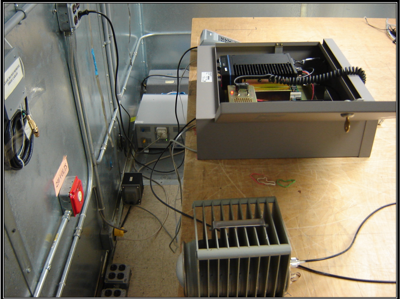
Photograph 6: Conducted Emissions (Rear View) Wall Mount Configuration
