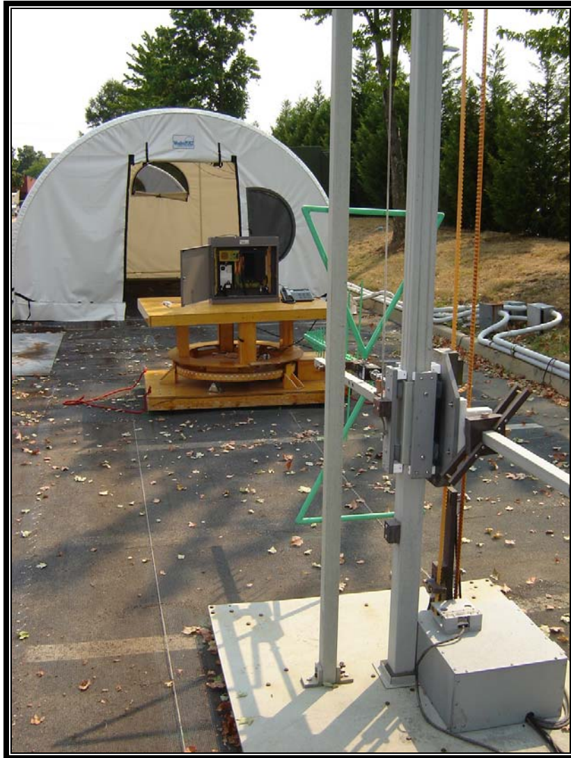
Photograph 1: Radiated Emissions (Front View) Wall Mount Configuration
