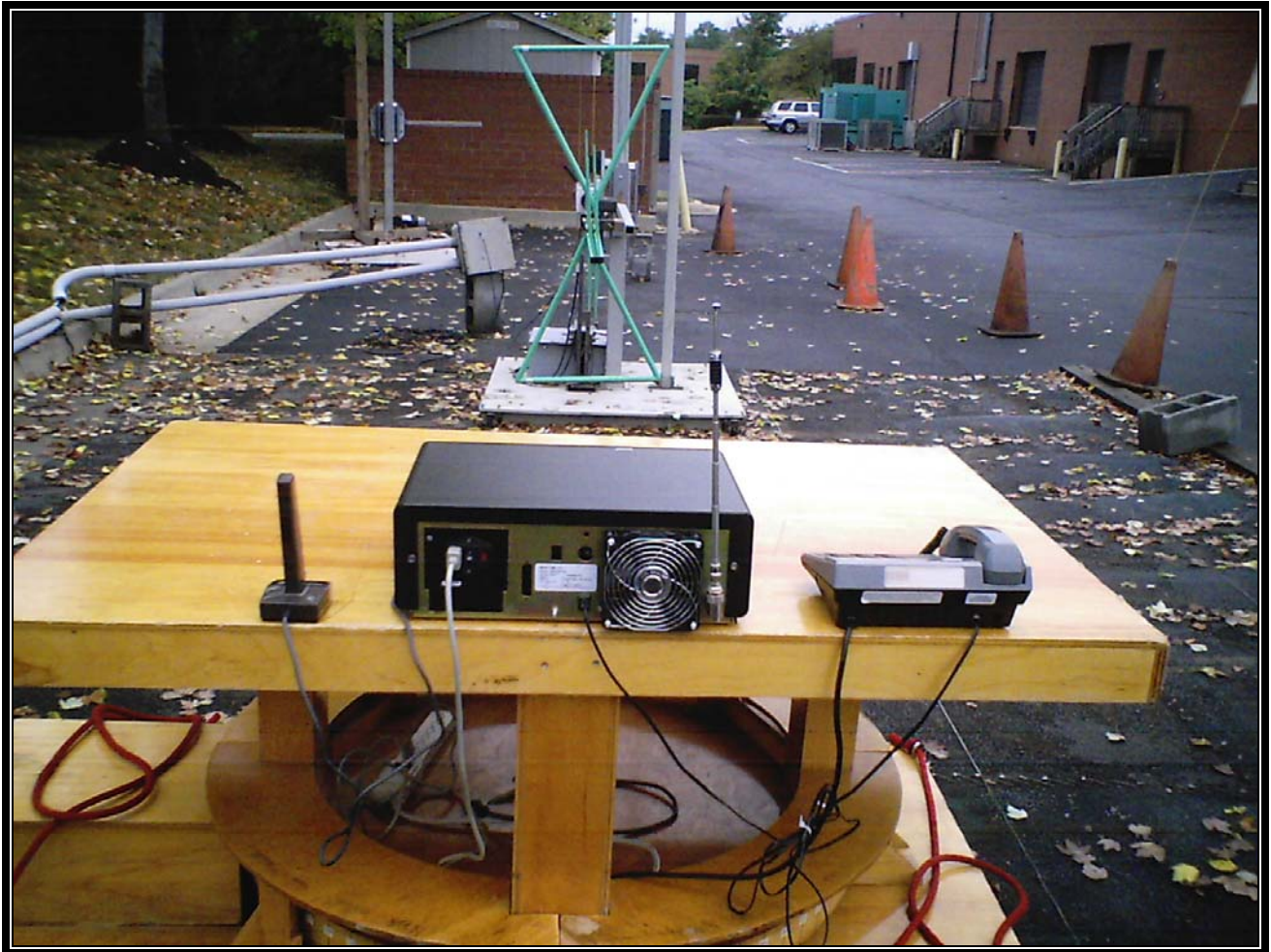
Photograph 4: Radiated Emissions (Rear View) Desktop Configuration
