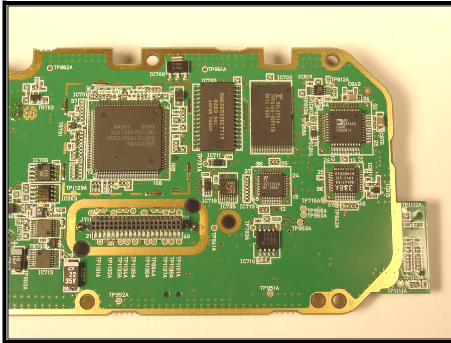
PHOTOGRAPH 20: AUDIO LOGIC BOARD SOLDER SIDE, RIGHT
