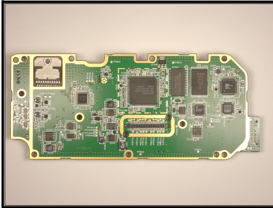
PHOTOGRAPH 18: AUDIO LOGIC BOARD SOLDER SIDE COMPLETE VIEW
