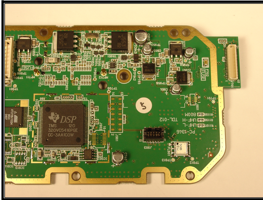
PHOTOGRAPH 17: AUDIO LOGIC BOARD COMPONENT SIDE, RIGHT
