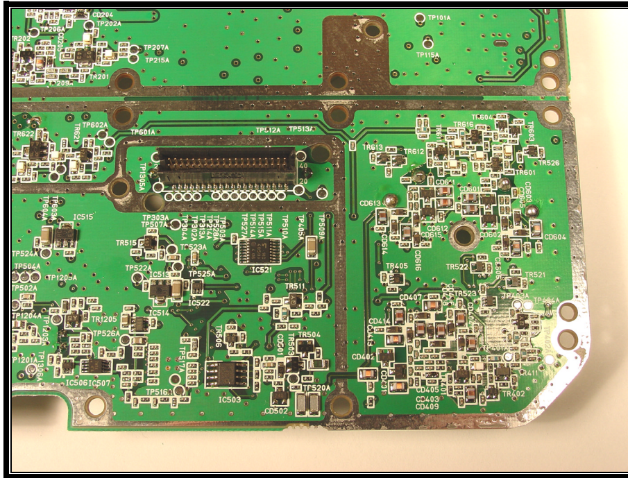
PHOTOGRAPH 12: TRX SYN BOARD SOLDER SIDE LOWER RIGHT
