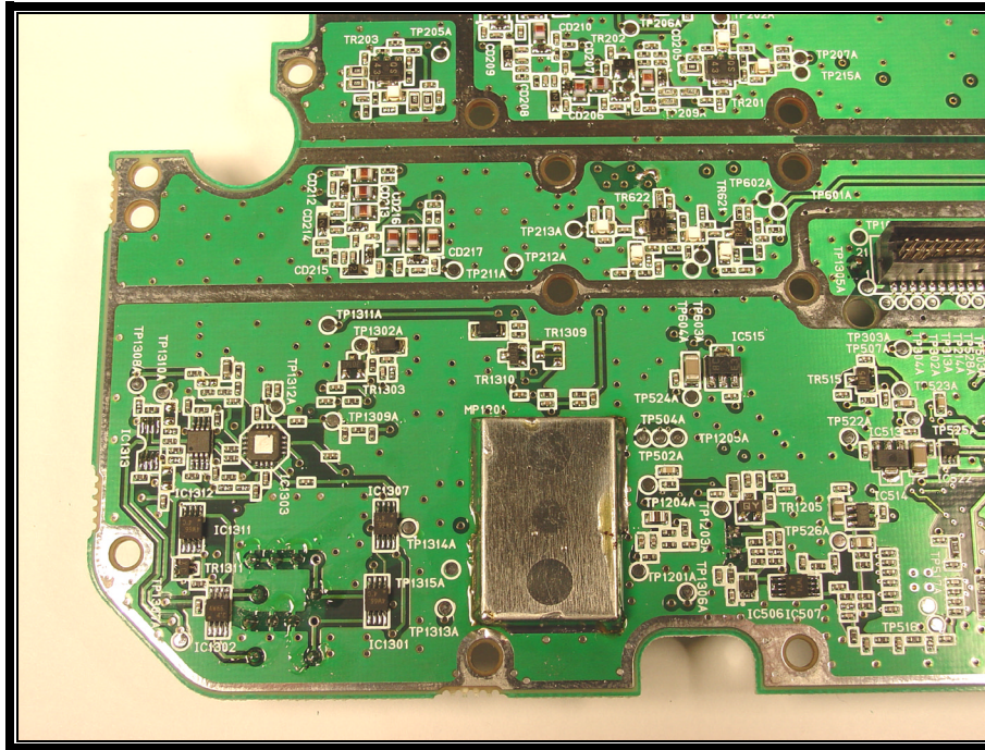
PHOTOGRAPH 11: TRX SYN BOARD SOLDER SIDE LOWER LEFT
