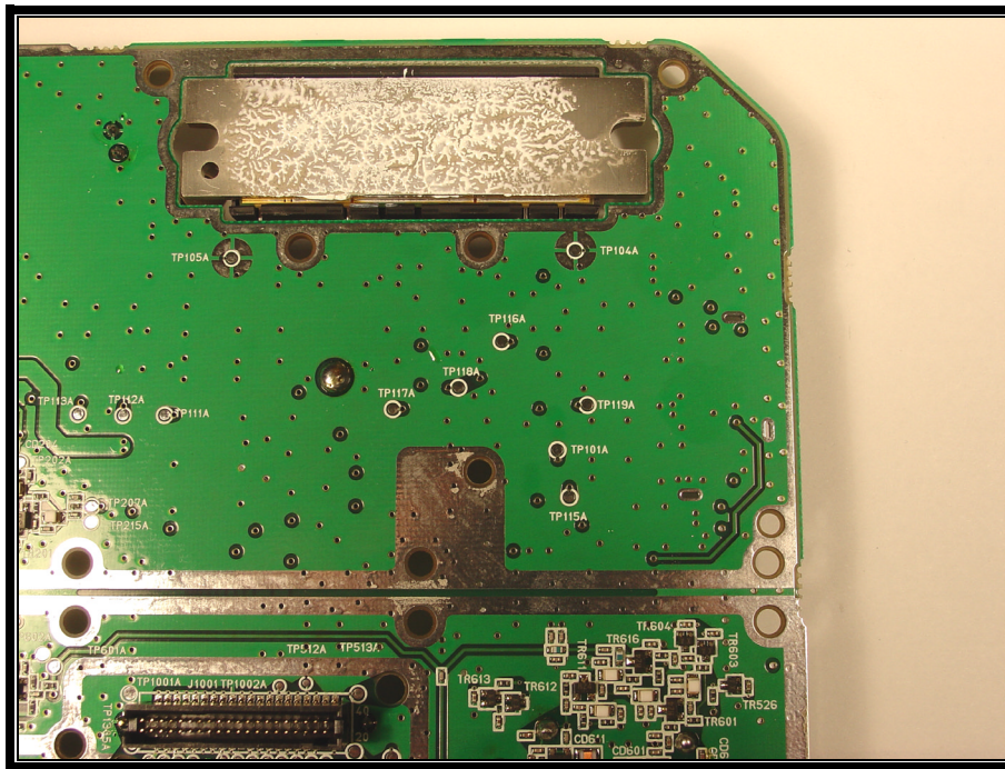
PHOTOGRAPH 14: TRX SYN BOARD SOLDER SIDE UPPER RIGHT
