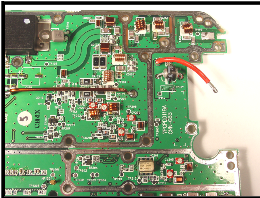
PHOTOGRAPH 9: TRX SYN BOARD COMPONENT SIDE UPPER RIGHT
