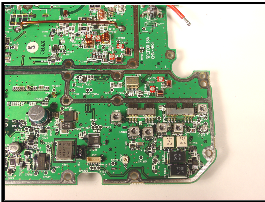
PHOTOGRAPH 7: TRX SYN BOARD COMPONENT SIDE LOWER RIGHT
