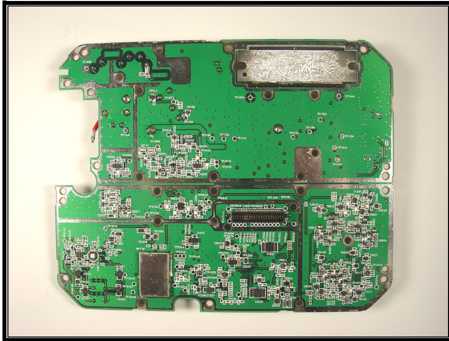
PHOTOGRAPH 10: TRX SYN BOARD SOLDER SIDE COMPLETE VIEW
