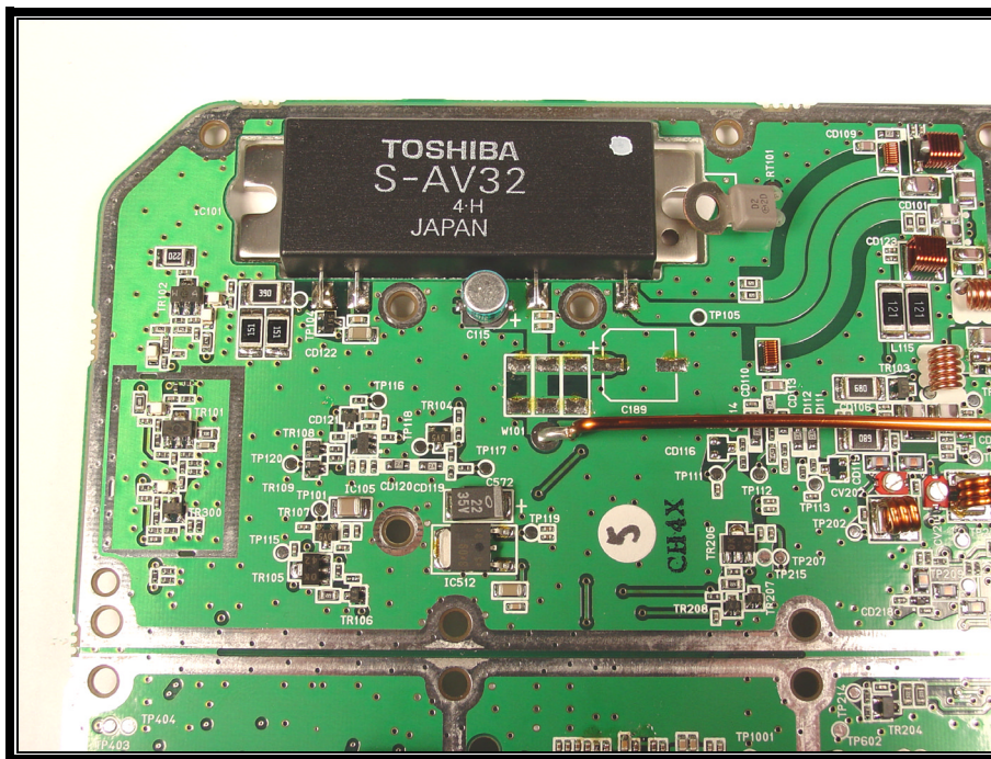
PHOTOGRAPH 8: TRX SYN BOARD COMPONENT SIDE UPPER LEFT
