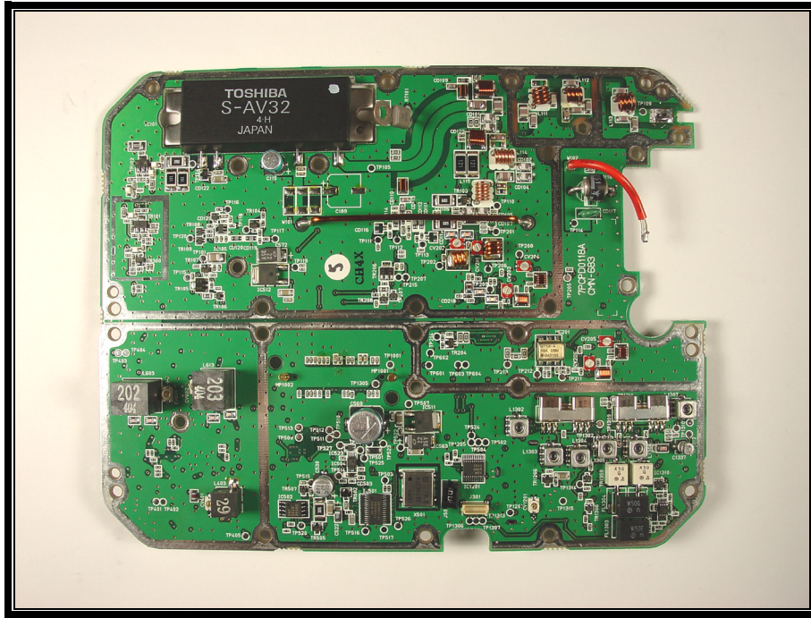
PHOTOGRAPH 5: TRX SYN BOARD COMPONENT SIDE COMPLETE VIEW
