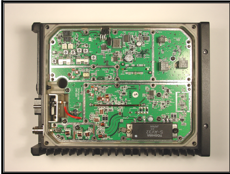
PHOTOGRAPH 4: BOTTOM COVER AND SHIELD REMOVED
