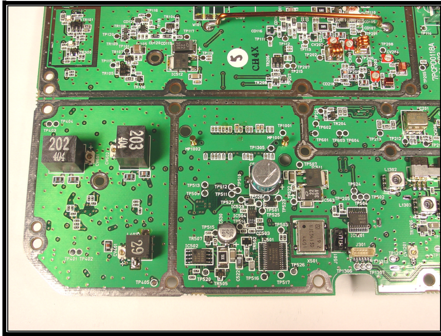
PHOTOGRAPH 6: TRX SYN BOARD COMPONENT SIDE LOWER LEFT
