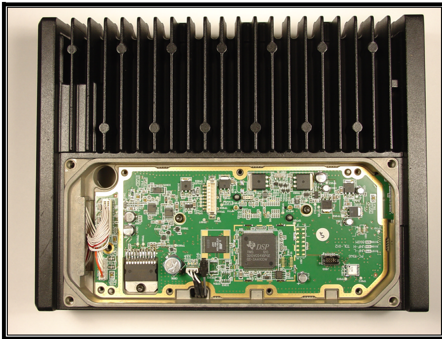
PHOTOGRAPH 2: TOP COVER AND SHIELD REMOVED
