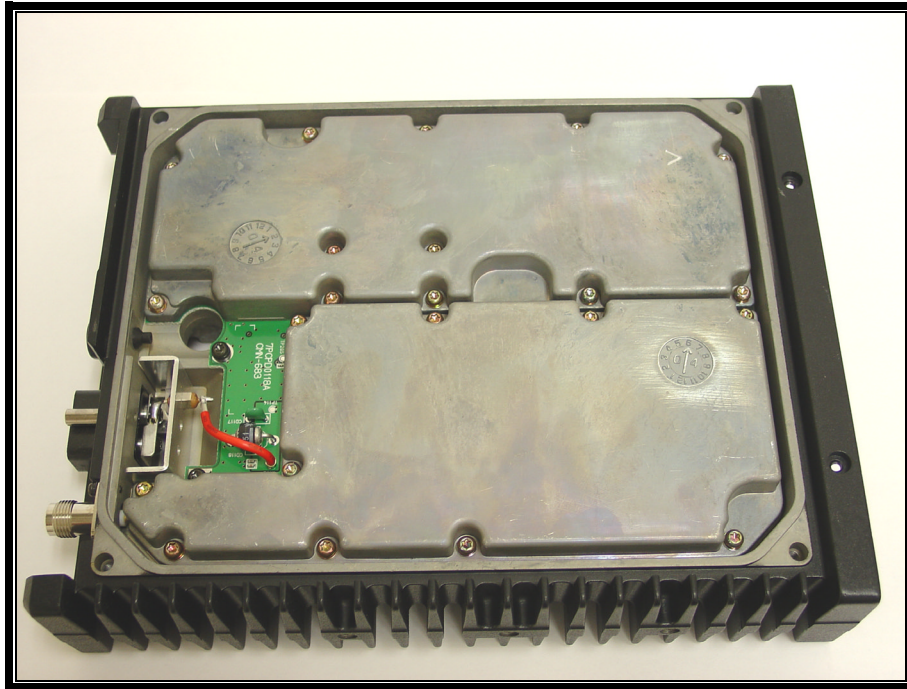
PHOTOGRAPH 3: BOTTOM COVER REMOVED
