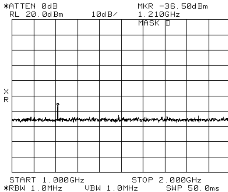
Figure 7-4: Tx at 403.025 MHz , 100 W power, 1 GHz to 2 GHz
