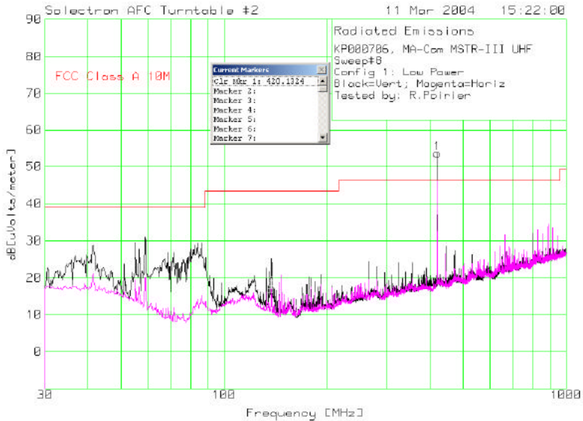
Figure 7-29: Field strength with 10 W Tx, 30 MHz to 1 GHz (Tx at 420 MHz)
