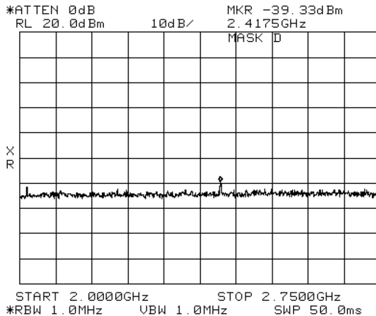
Figure 7-5: Tx at 403.025 MHz , 100 W power, 2 GHz to 2.75 GHz
