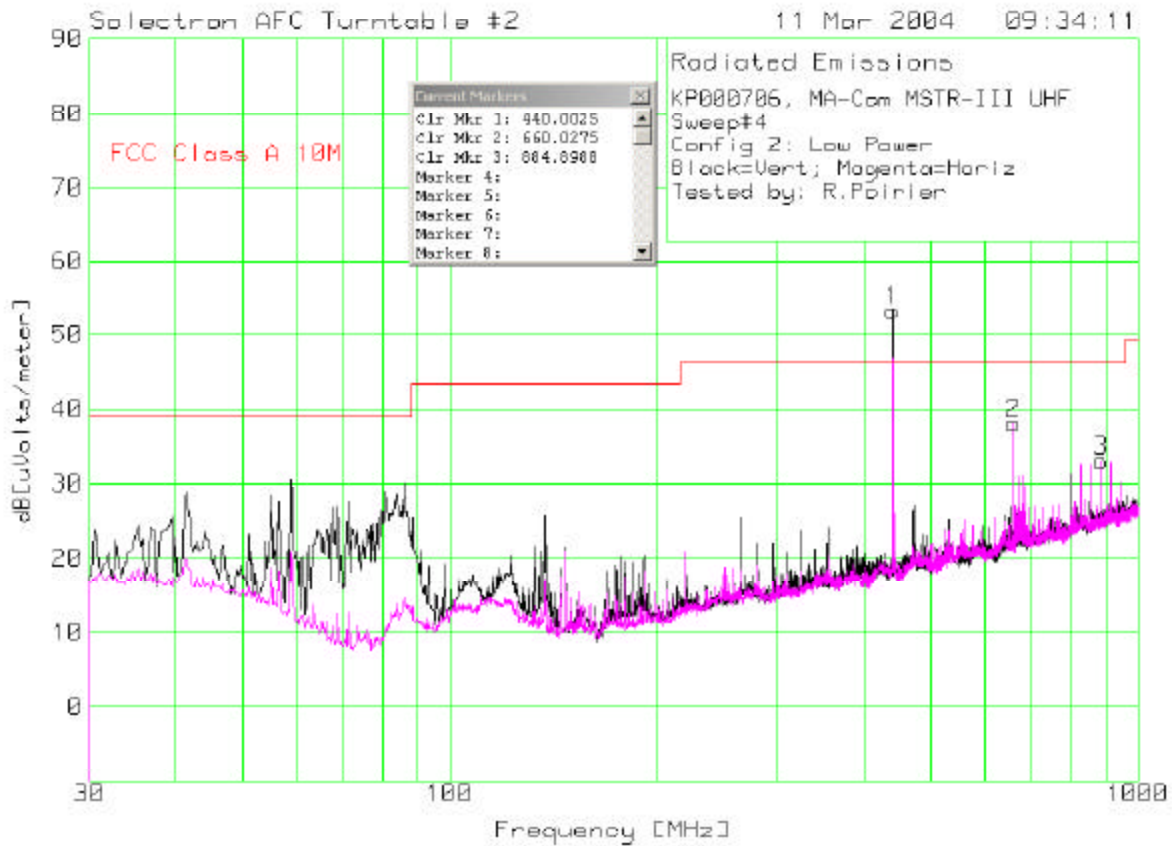
Figure 7-33: Field strength with 10 W Tx, 30 MHz to 1 GHz (Tx at 440 MHz)
