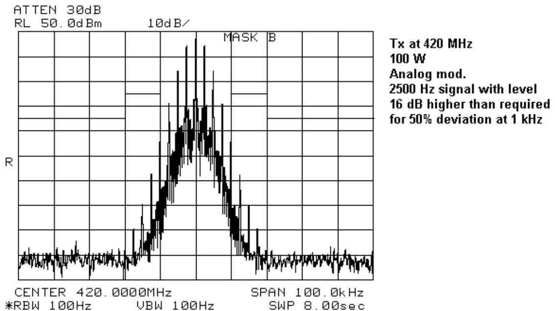
Figure 7-22: 2500 Hz audio signal Wideband, 420 MHz
