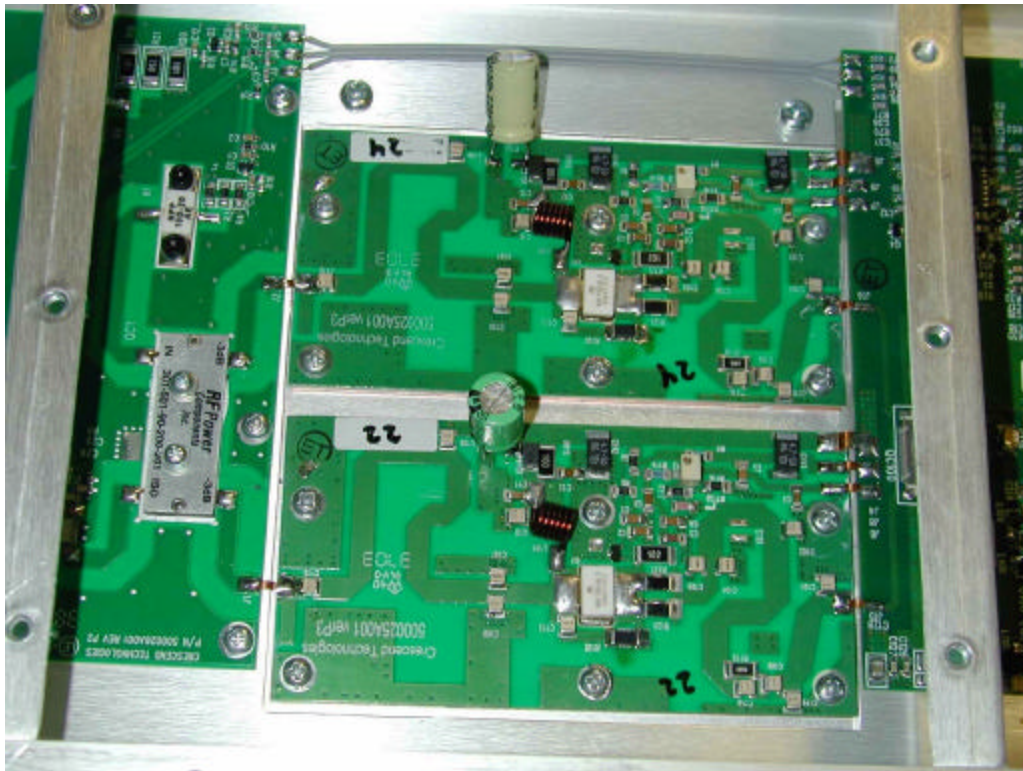
Figure 8: PA Board Middle Section
