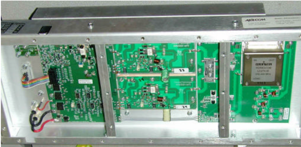
Figure 7: PA Leftmost Part of Board
