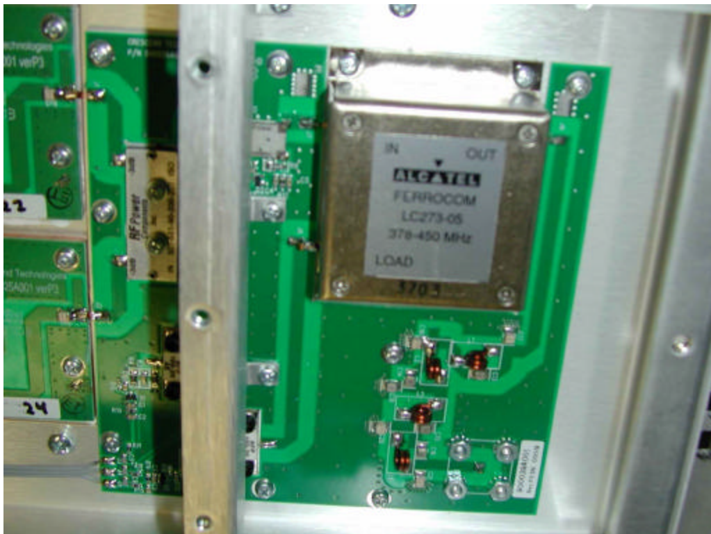
Figure 9: PA Board Rightmost section
