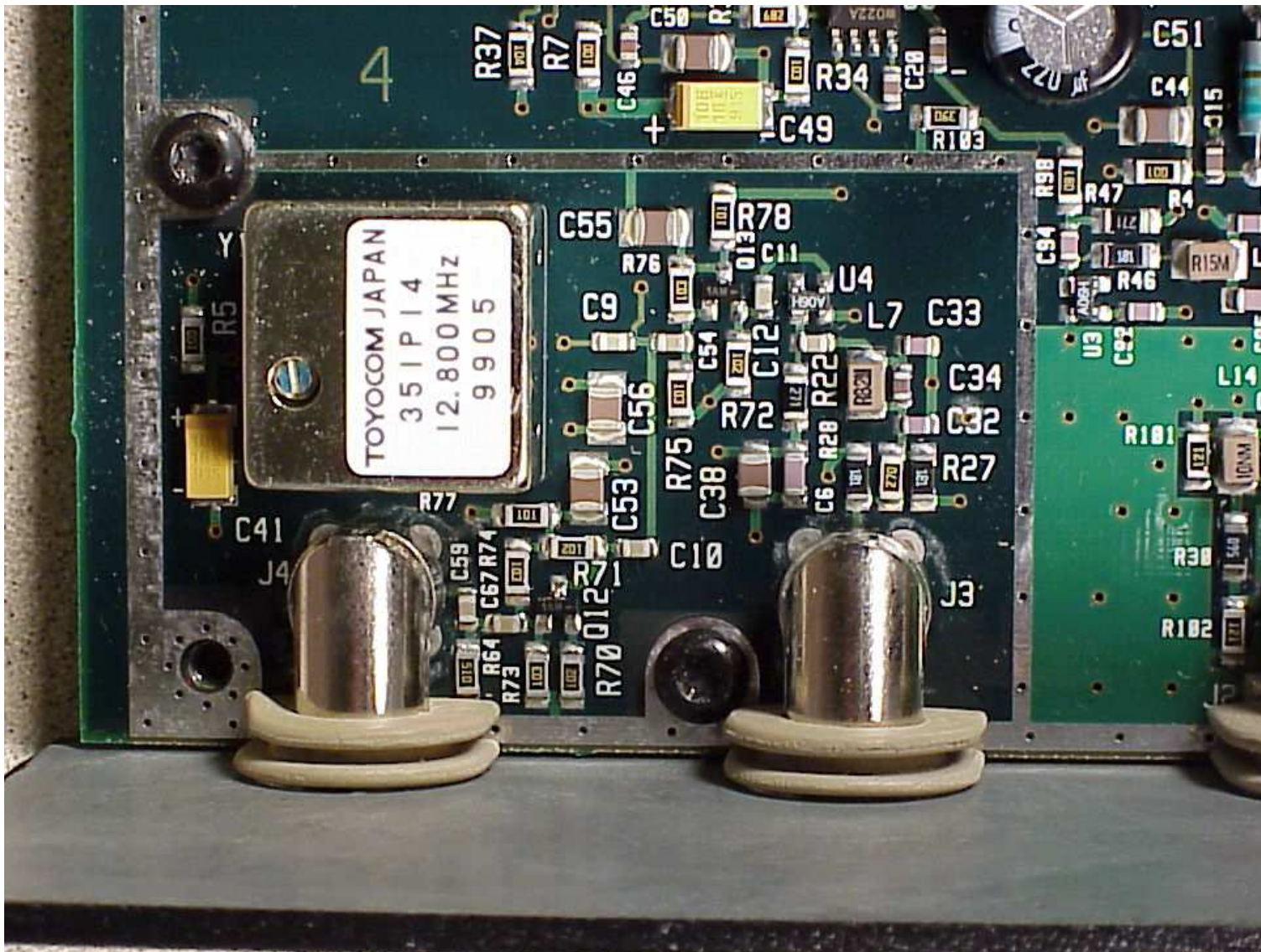
Figure 12 - Rx Synthesizer frequency reference
