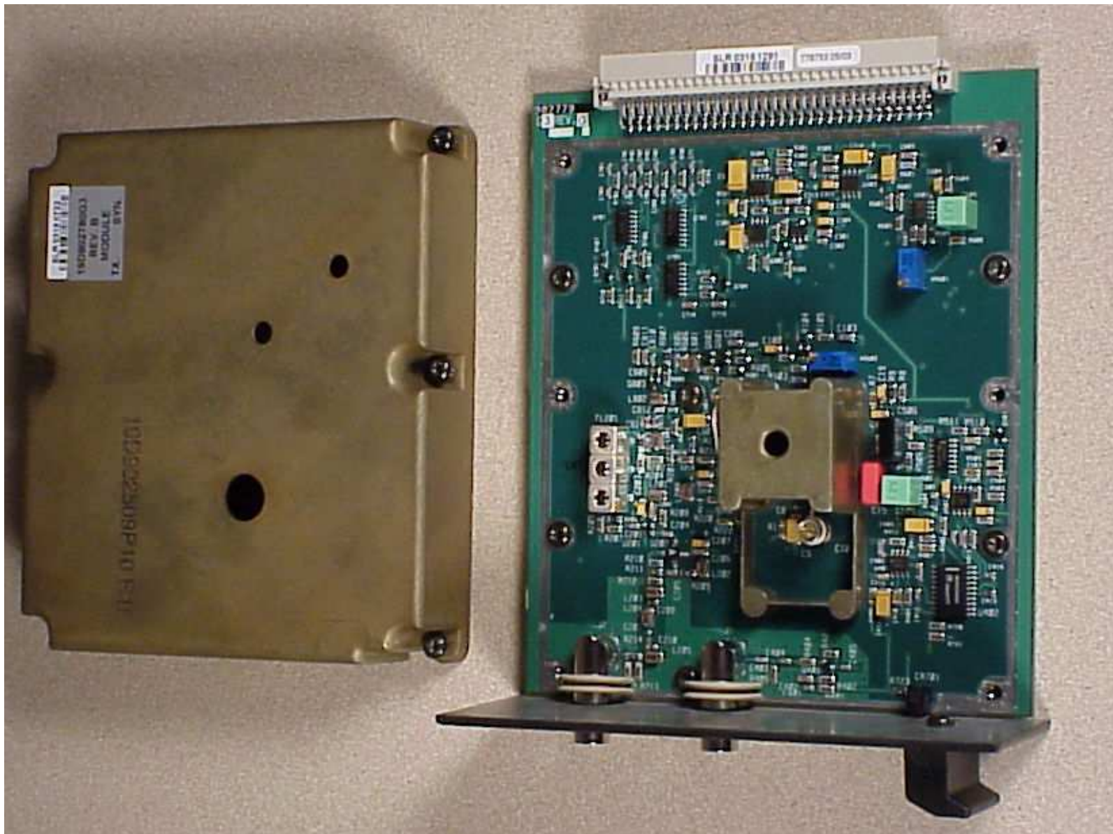
Figure 2 - Tx Synthesizer - cover removed
