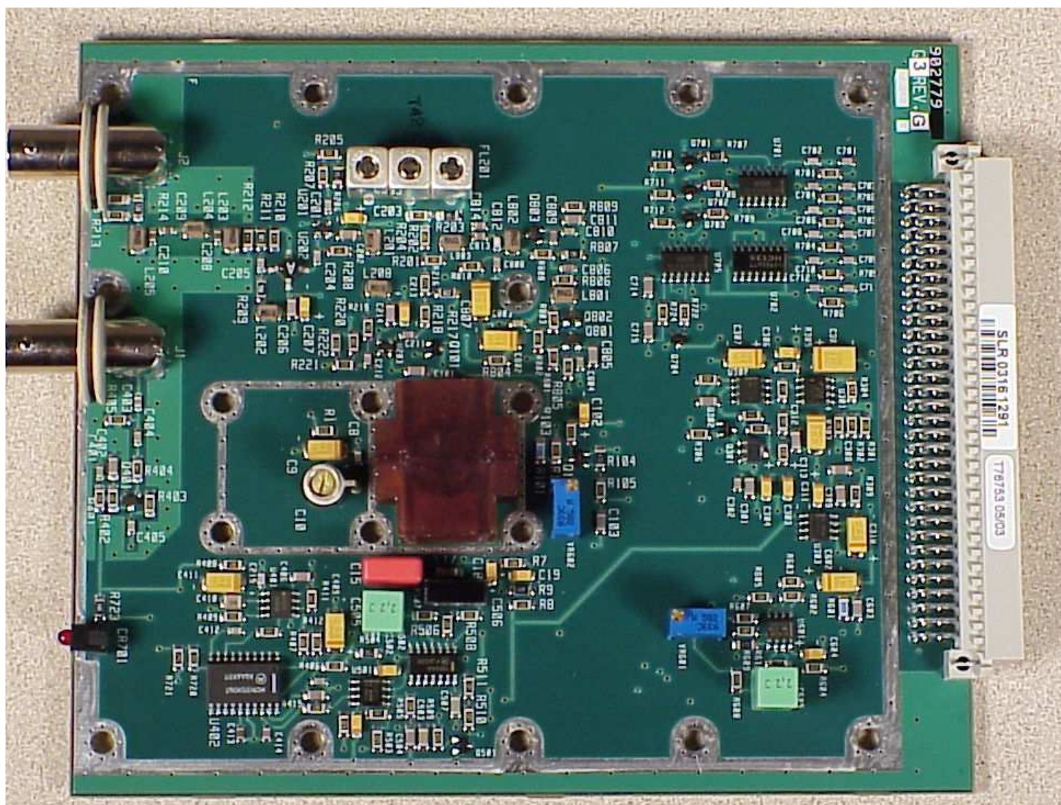
Figure 3 - Tx Synthesizer board top
