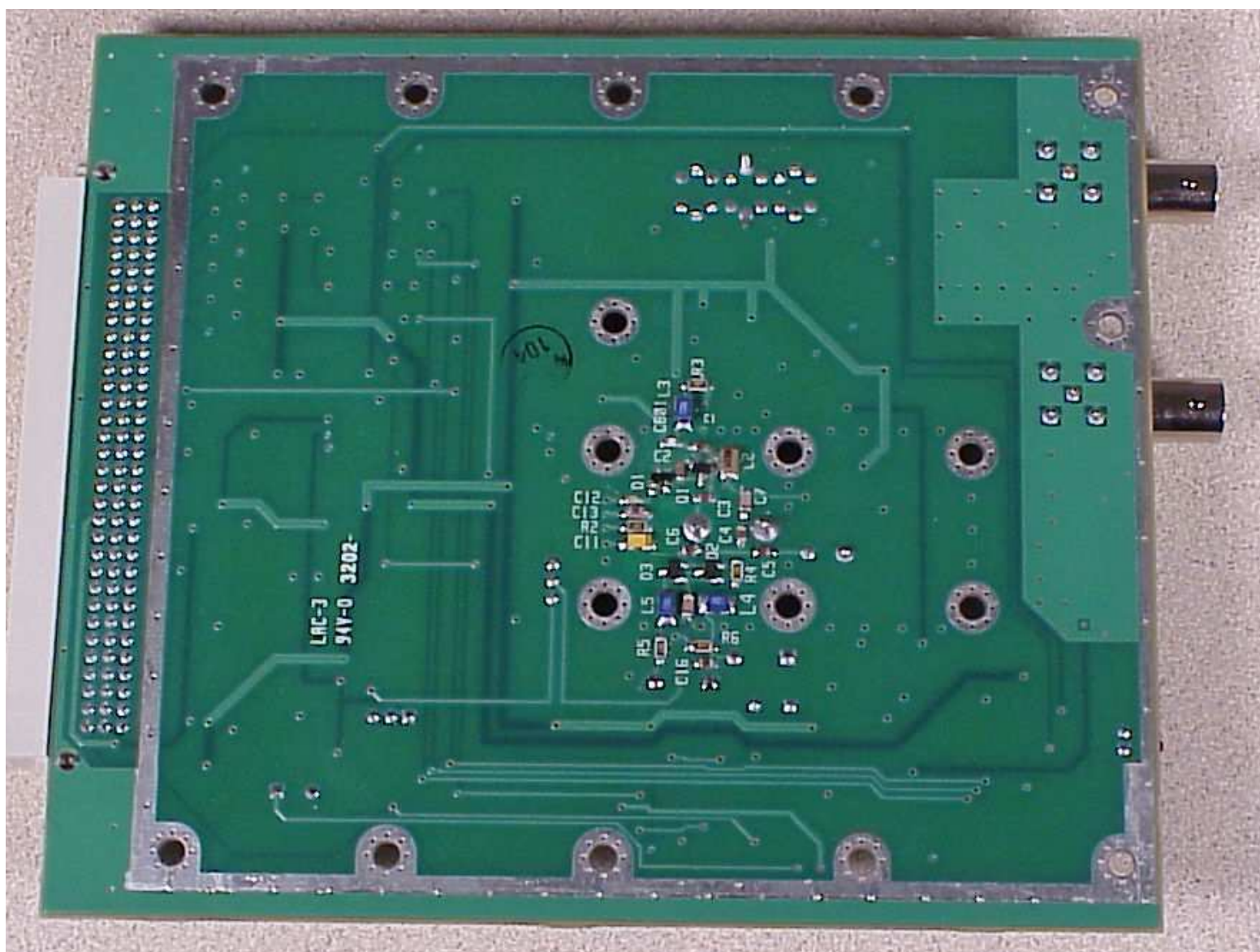
Figure 4 - Tx Synthesizer board bottom
