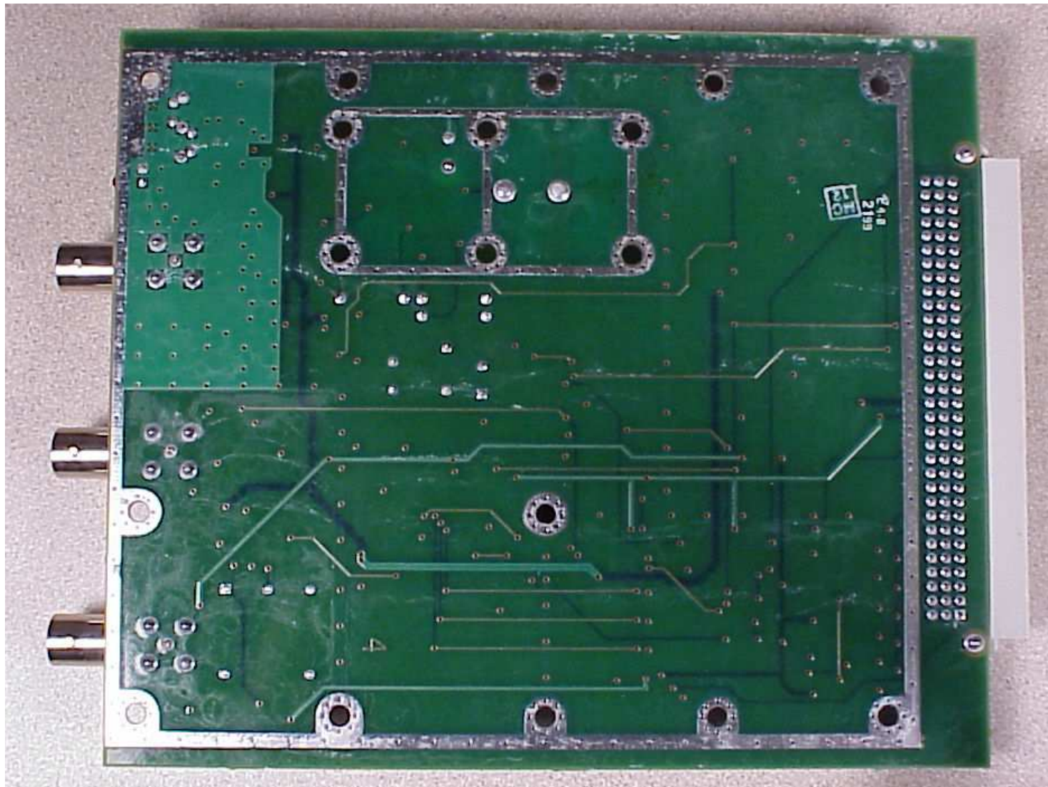
Figure 11 - Rx Synthesizer board bottom
