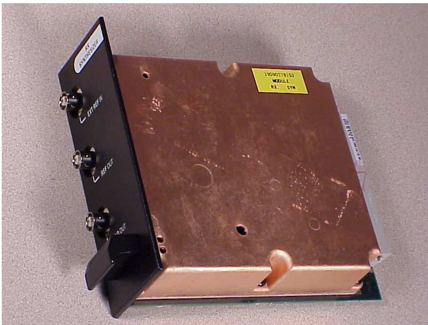
Figure 8 - Rx Synthesizer overall
