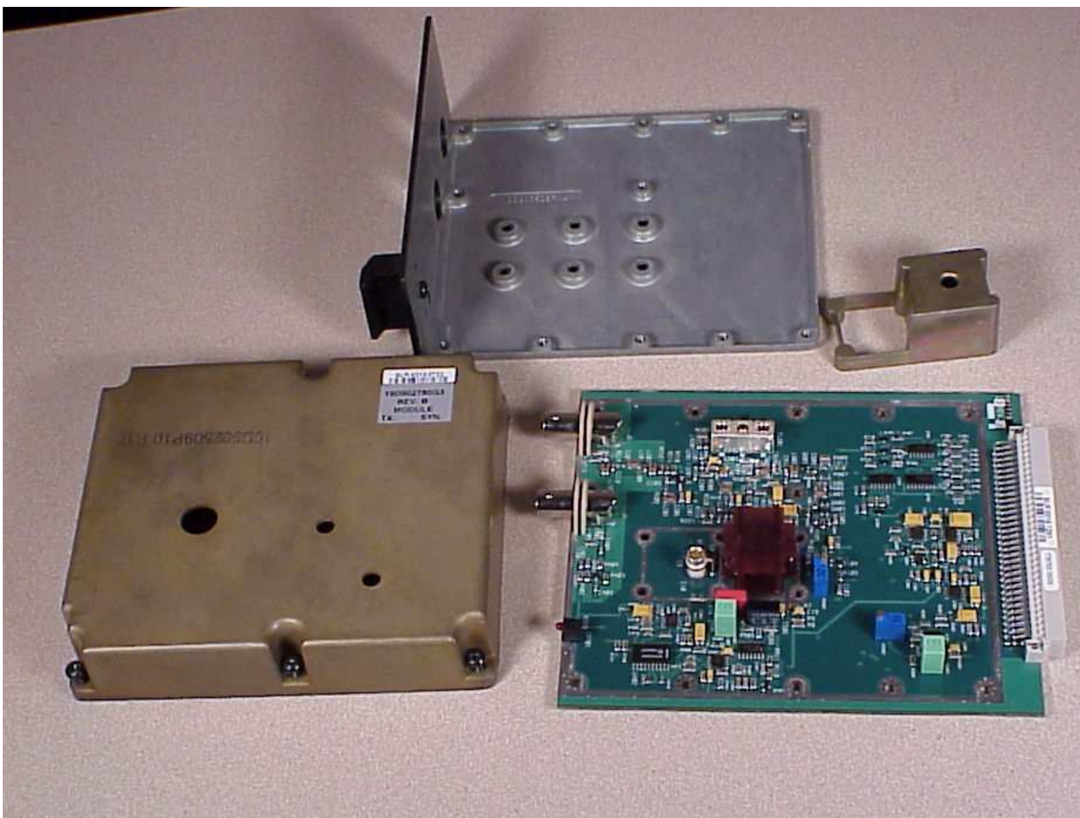
Figure 7 - Tx Synthesizer disassembled
