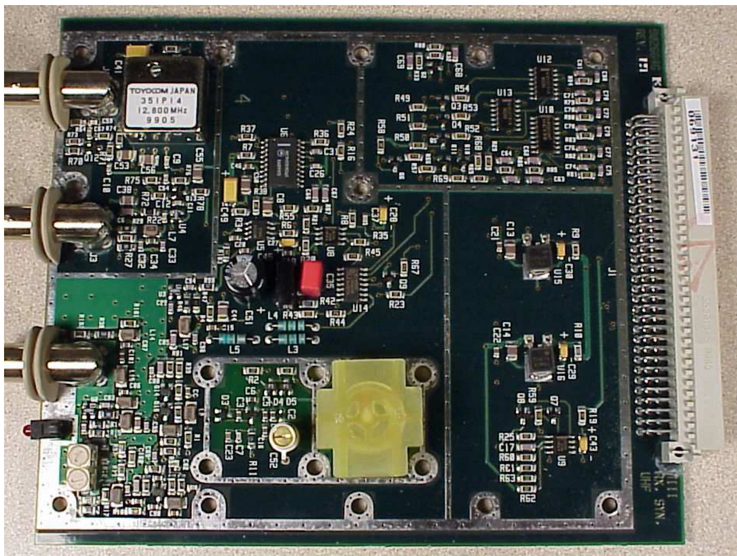
Figure 10 - Rx Synthesizer board top
