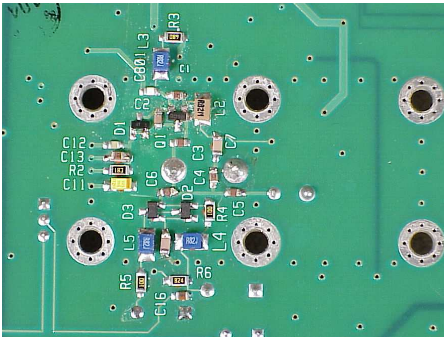
Figure 6 - Tx Synthesizer VCO bottom
