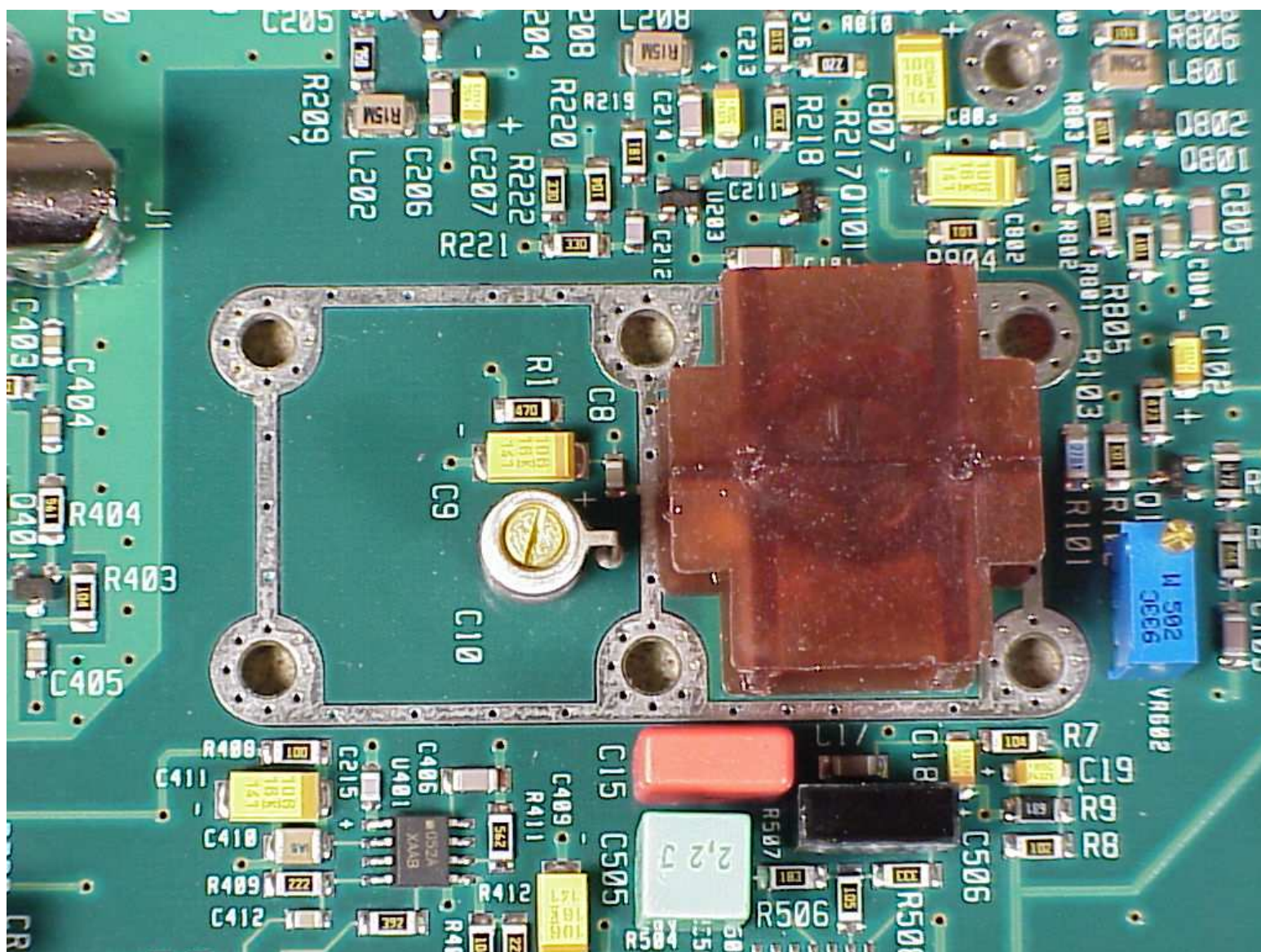
Figure 5 - Tx Synthesizer VCO top
