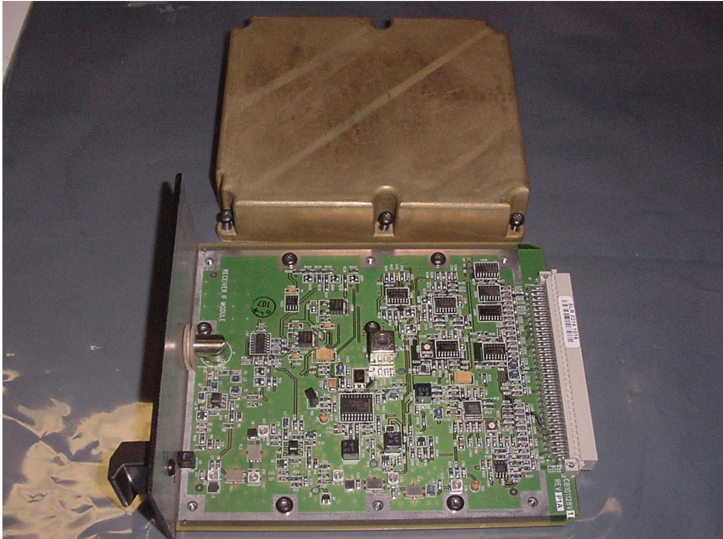
Figure 15 - Rx IF board top
