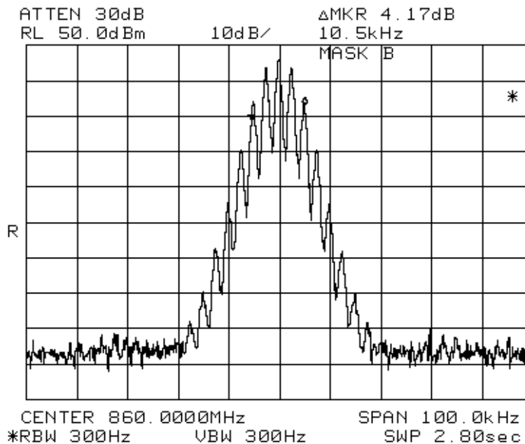
Figure 7-22: 2 Level 9600 baud Signal With 3 kHz Deviation
