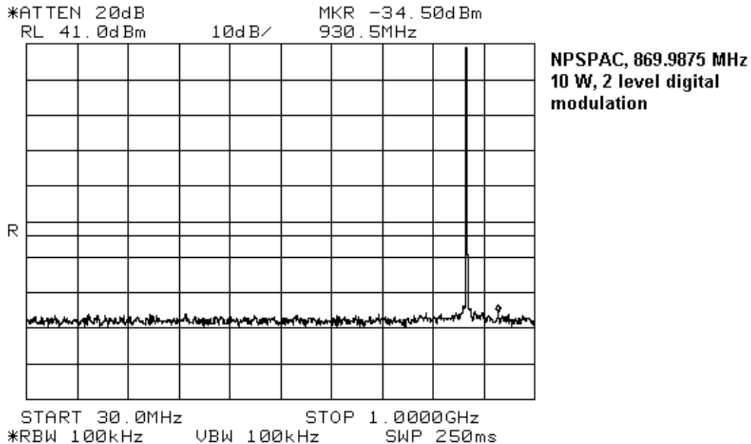
Figure 7-11: Tx at 869.9875 MHz, 10 W Power, 30 MHz to 1 GHz
