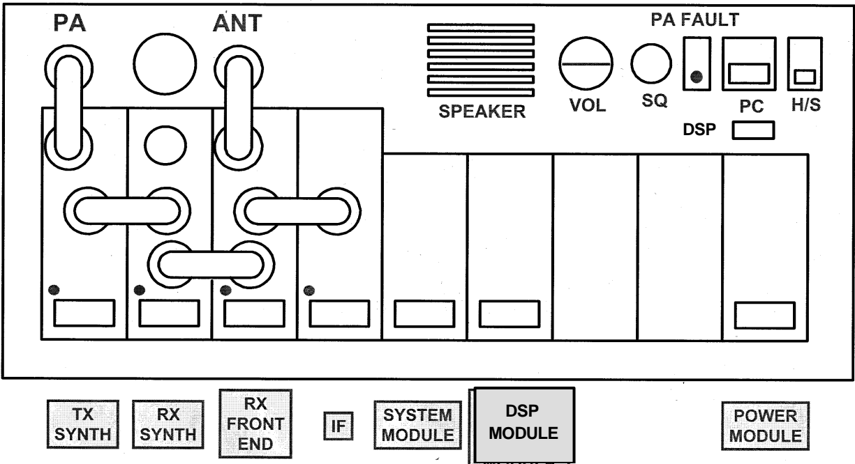
Figure 3-2: Module Configuration
