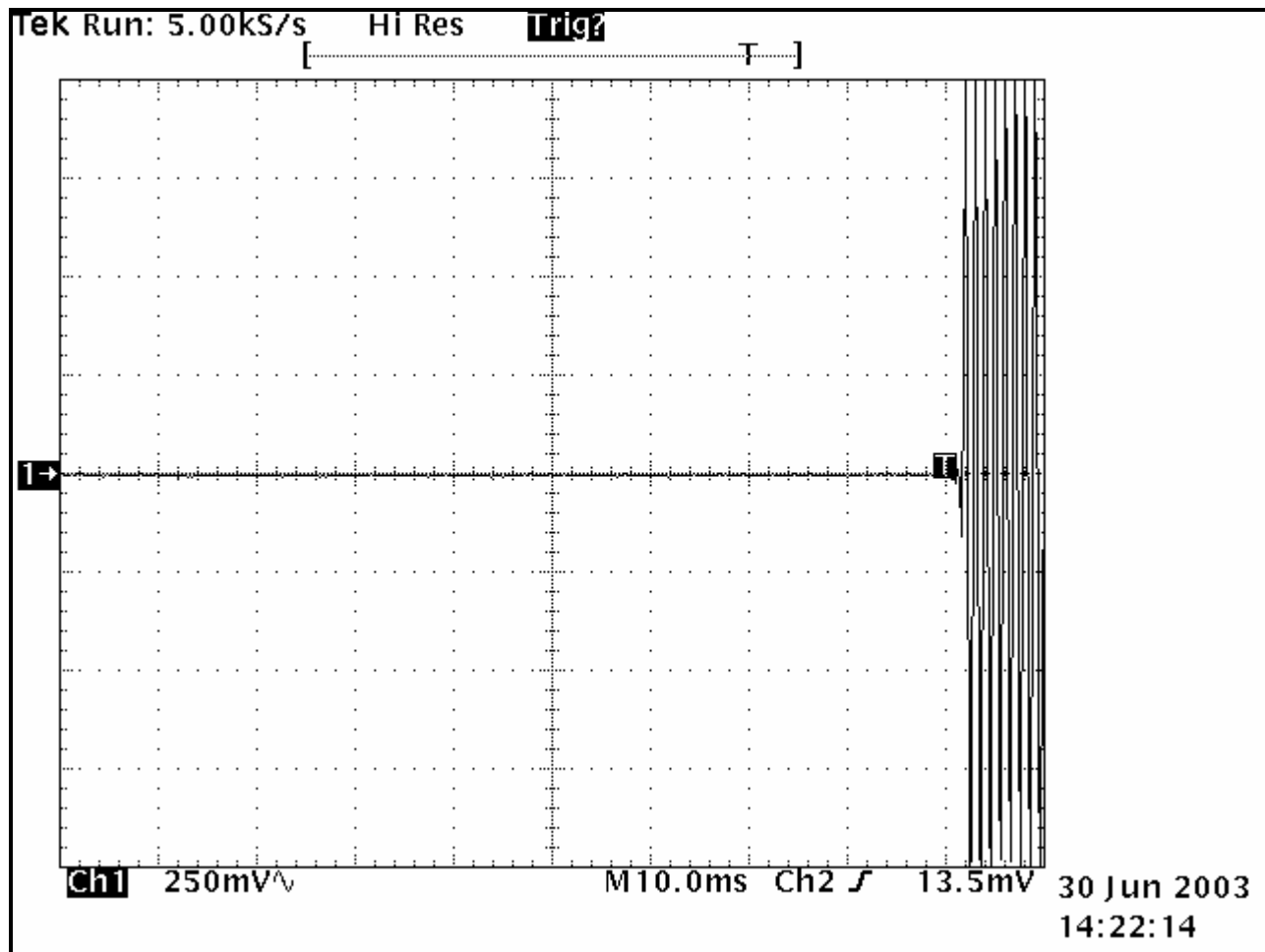
PLOT 13-4: TRANSIENT FREQUENCY BEHAVIOR – 501.525 MHZ; HIGH POWER; NARROW BAND; CARRIER OFF TIME
