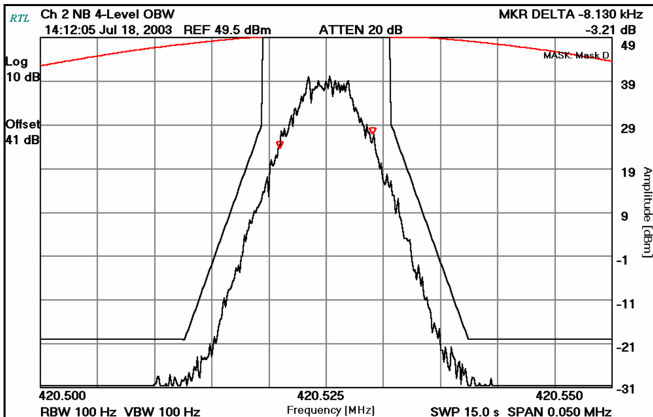
PLOT 8-6: 99% OCCUPIED BANDWIDTH - C4FM; NARROW BAND; 4800 BAUD
