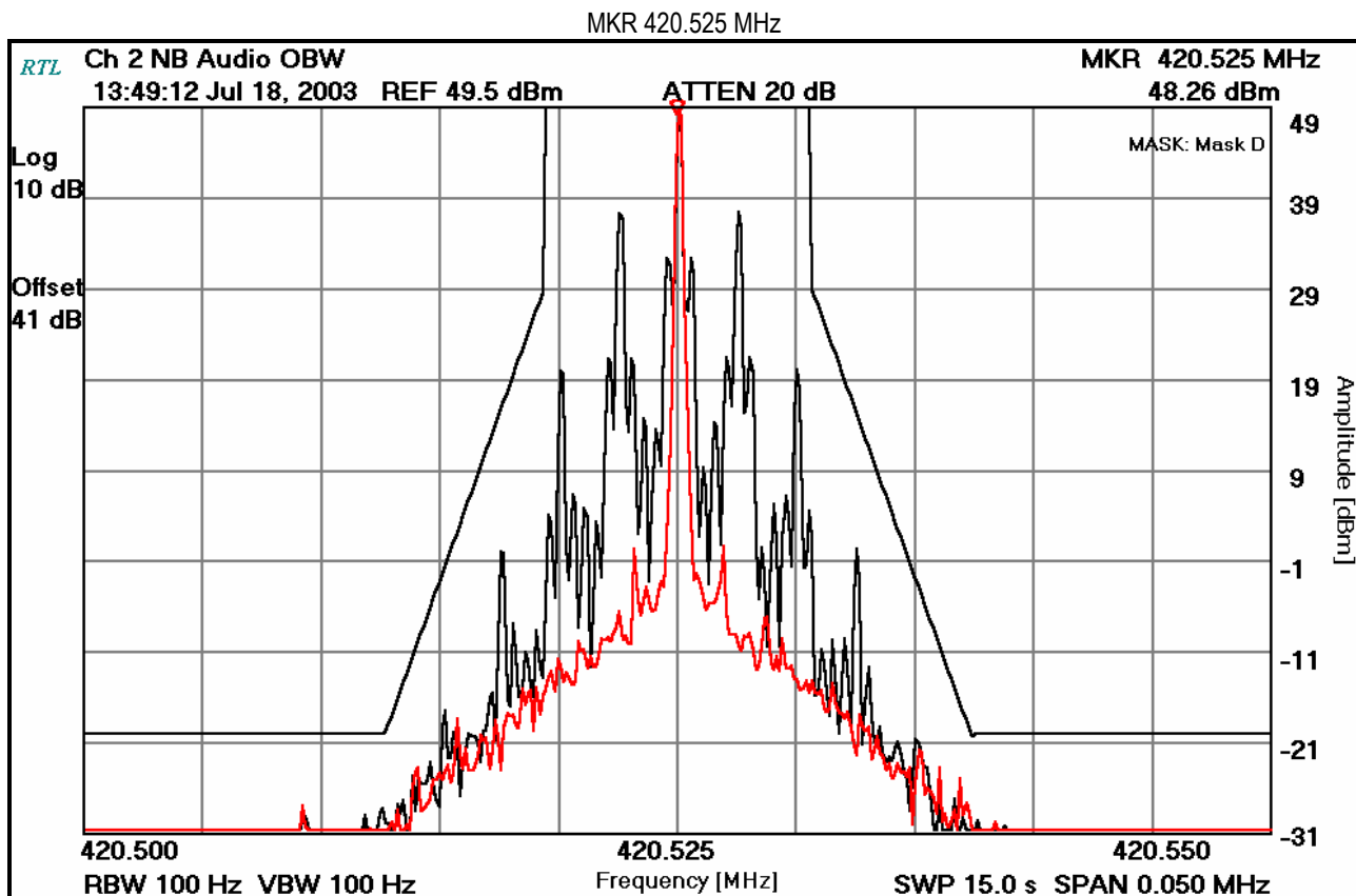
PLOT 8-2: OCCUPIED BANDWIDTH; NARROW BAND; ANALOG MODULATION: 2,500 HZ
