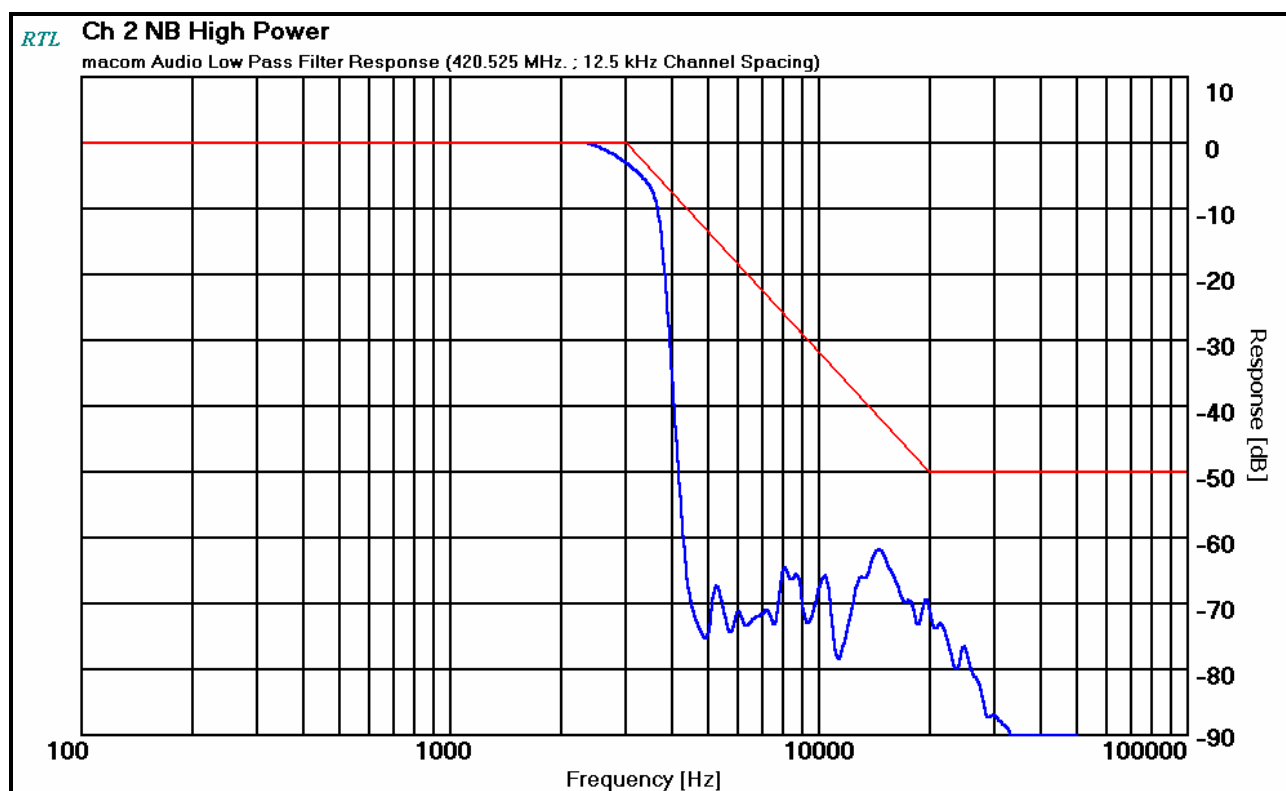
PLOT 11-1: MODULATION CHARACTERISTICS – AUDIO LOW PASS FILTER
