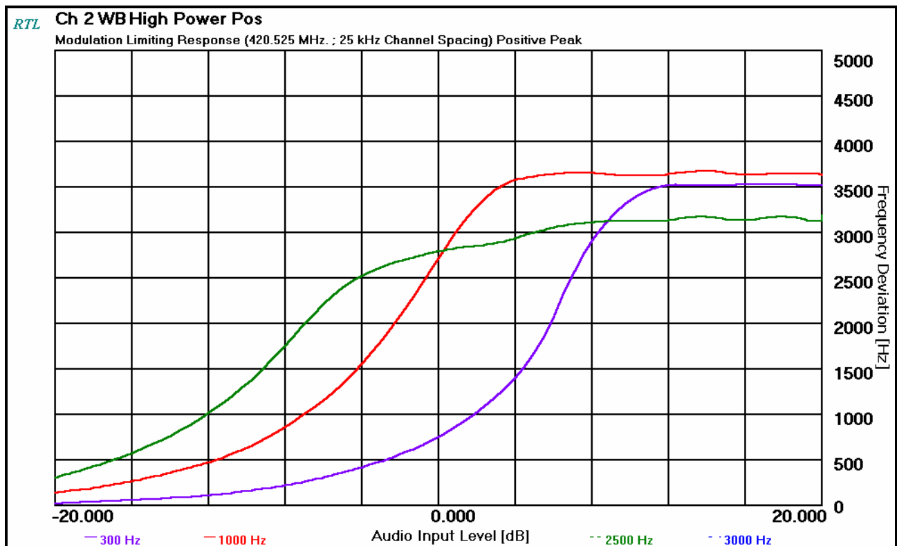
PLOT 12-1: MODULATION CHARACTERISTICS – MODULATION LIMITING: WIDE BAND; POSITIVE PEAK
