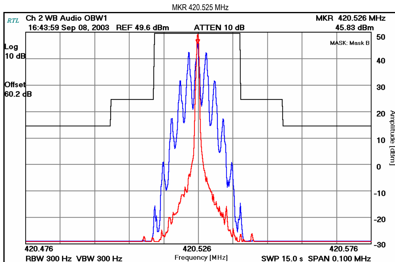
PLOT 8-1: OCCUPIED BANDWIDTH; WIDE BAND; ANALOG MODULATION: 2,500 HZ
