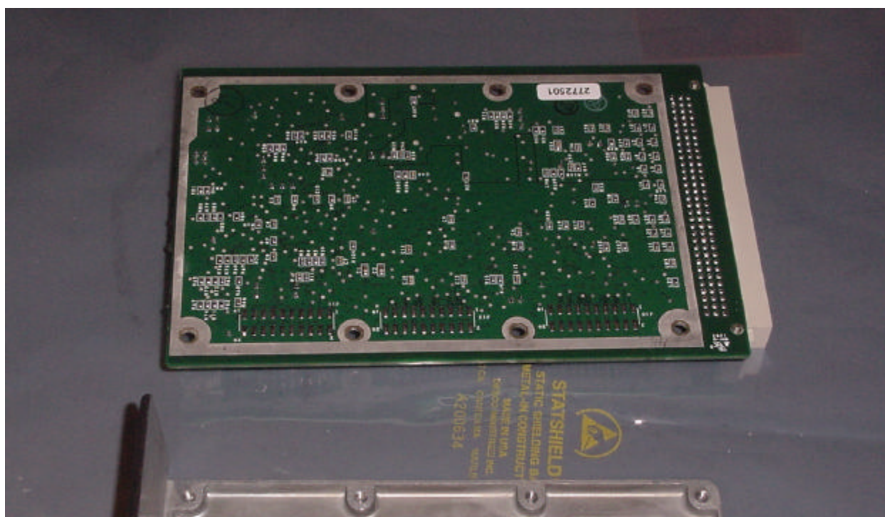
Figure 27 - Power Module board bottom
