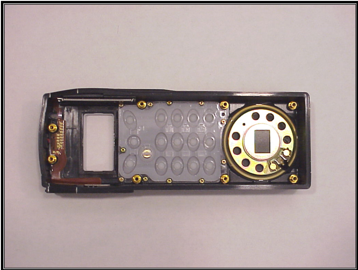
PHOTOGRAPH 4: VIEW OF INSIDE OF FRONT COVER
