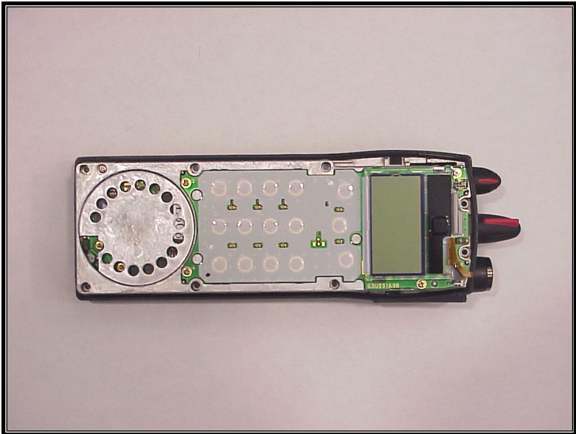
PHOTOGRAPH 5: VIEW OF TOP OF INTERFACE BOARD AND RF SHIELD
