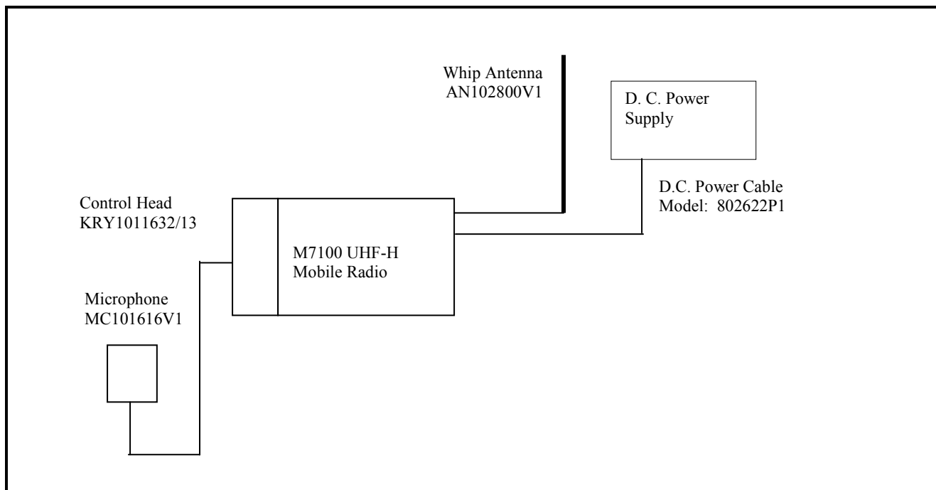
FIGURE 3-2: STANDARD CONFIGURATION
