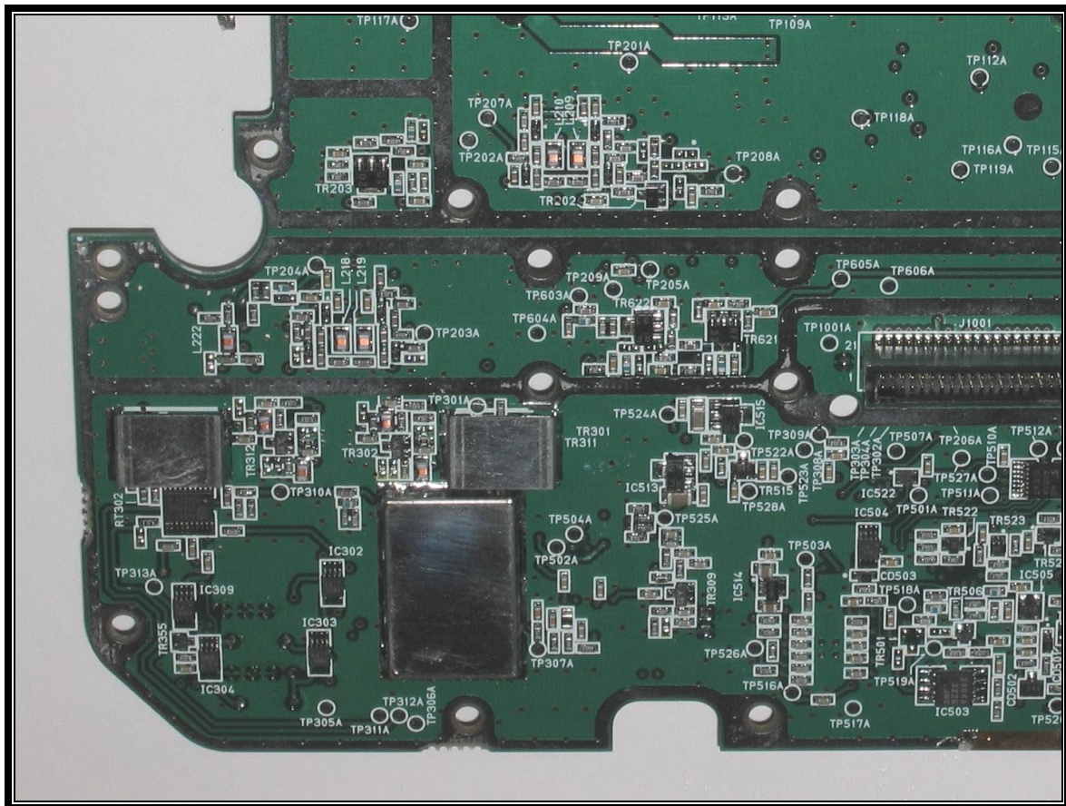
PHOTOGRAPH 23: TRX SYN BOARD SOLDER SIDE, LOWER LEFT
