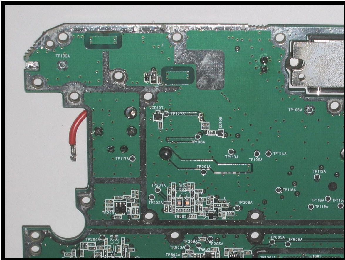
PHOTOGRAPH 25: TRX SYN BOARD SOLDER SIDE, UPPER LEFT
