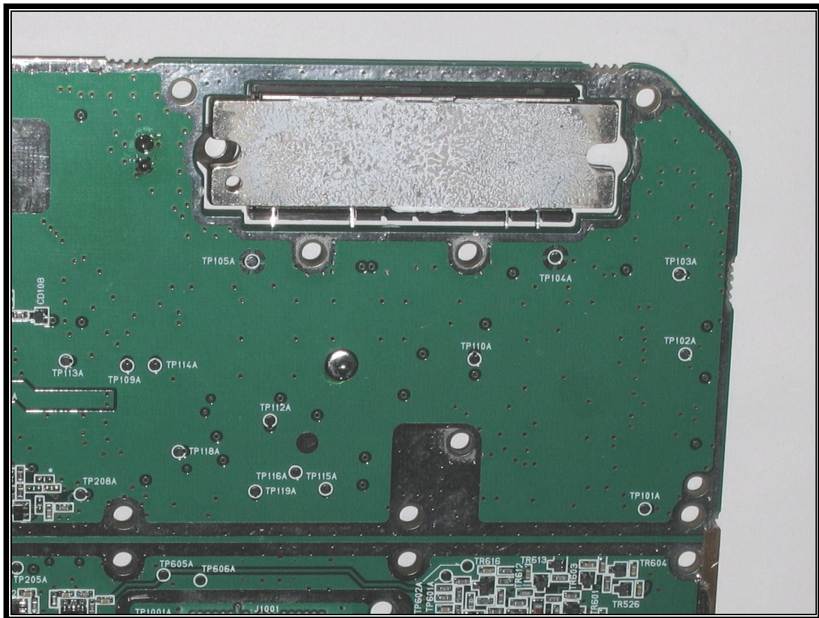
PHOTOGRAPH 26: TRX SYN BOARD SOLDER SIDE, UPPER RIGHT
