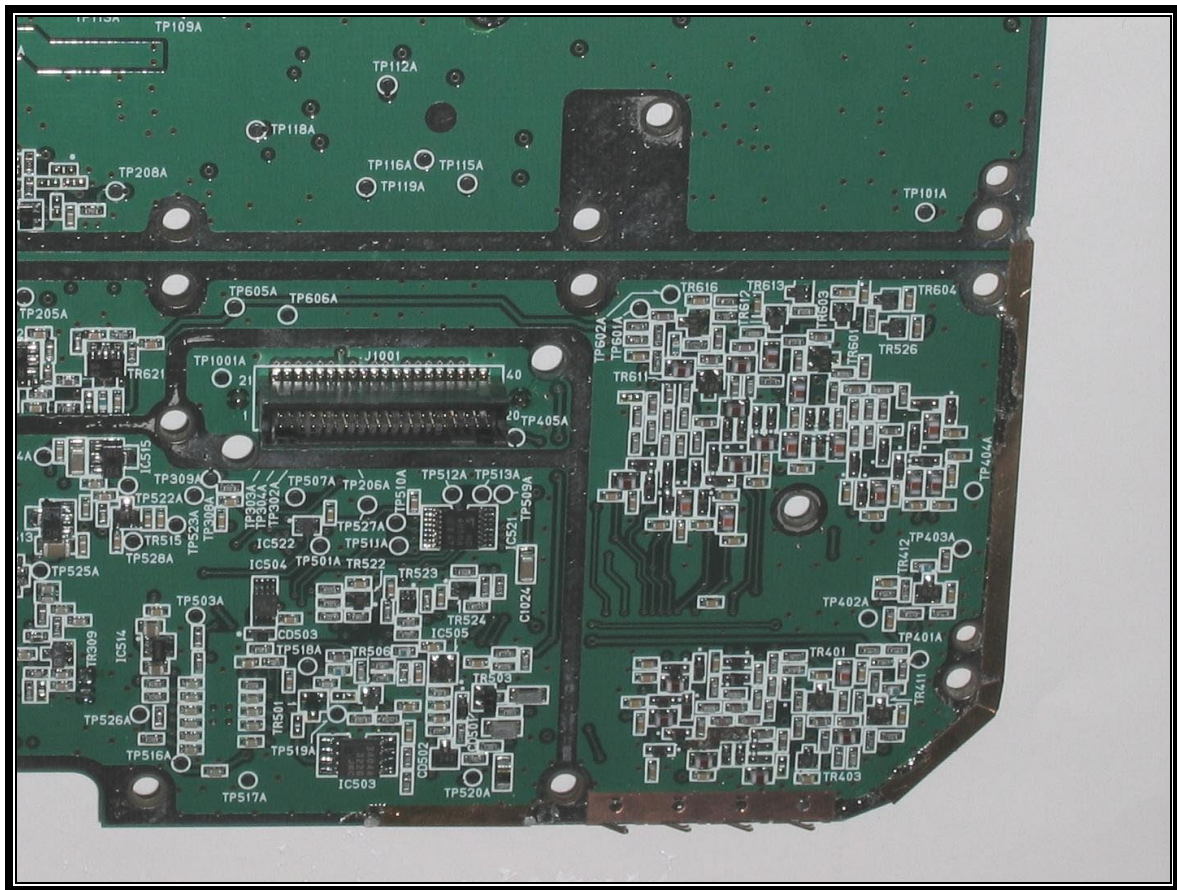
PHOTOGRAPH 24: TRX SYN BOARD SOLDER SIDE, LOWER RIGHT
