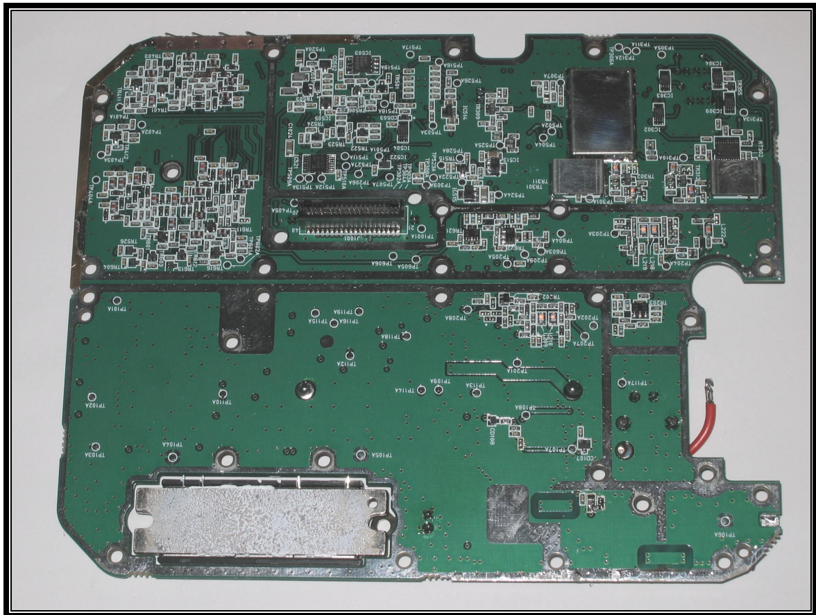
PHOTOGRAPH 22: TRX SYN BOARD SOLDER SIDE, COMPLETE VIEW
