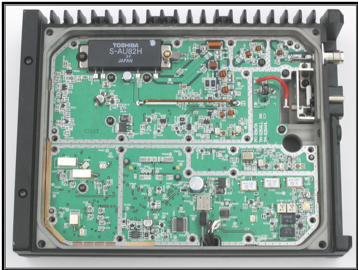
PHOTOGRAPH 9: BOTTOM COVER AND INNER SHIELD REMOVED
