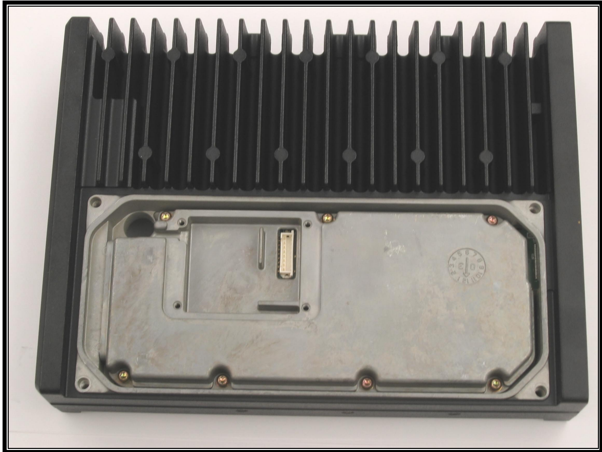
PHOTOGRAPH 7: TOP COVER REMOVED
