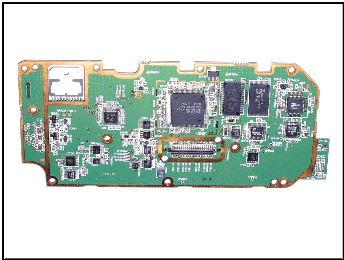
PHOTOGRAPH 13: AUDIO LOGIC BOARD SOLDER SIDE, COMPLETE VIEW
