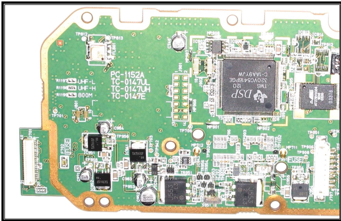
PHOTOGRAPH 11: AUDIO LOGIC BOARD COMPONENT SIDE, LEFT SIDE
