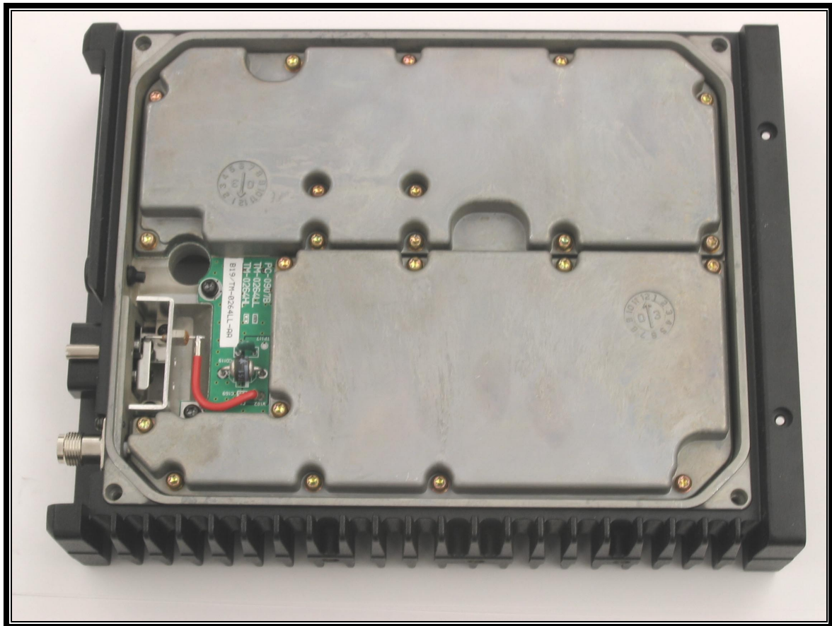
PHOTOGRAPH 8: BOTTOM COVER REMOVED
