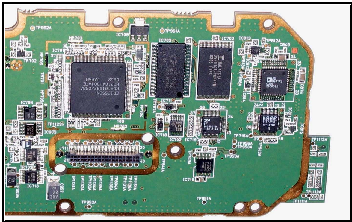
PHOTOGRAPH 15: AUDIO LOGIC BOARD SOLDER SIDE, RIGHT SIDE
