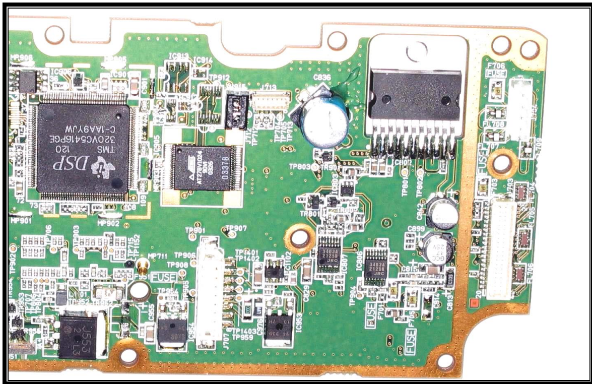
PHOTOGRAPH 12: AUDIO LOGIC BOARD COMPONENT SIDE, RIGHT SIDE
