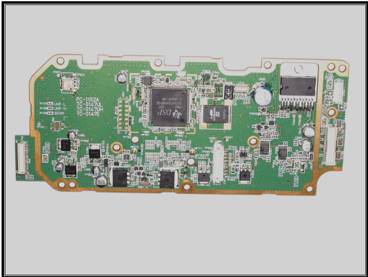
PHOTOGRAPH 10: AUDIO LOGIC BOARD COMPONENT SIDE, COMPLETE VIEW
